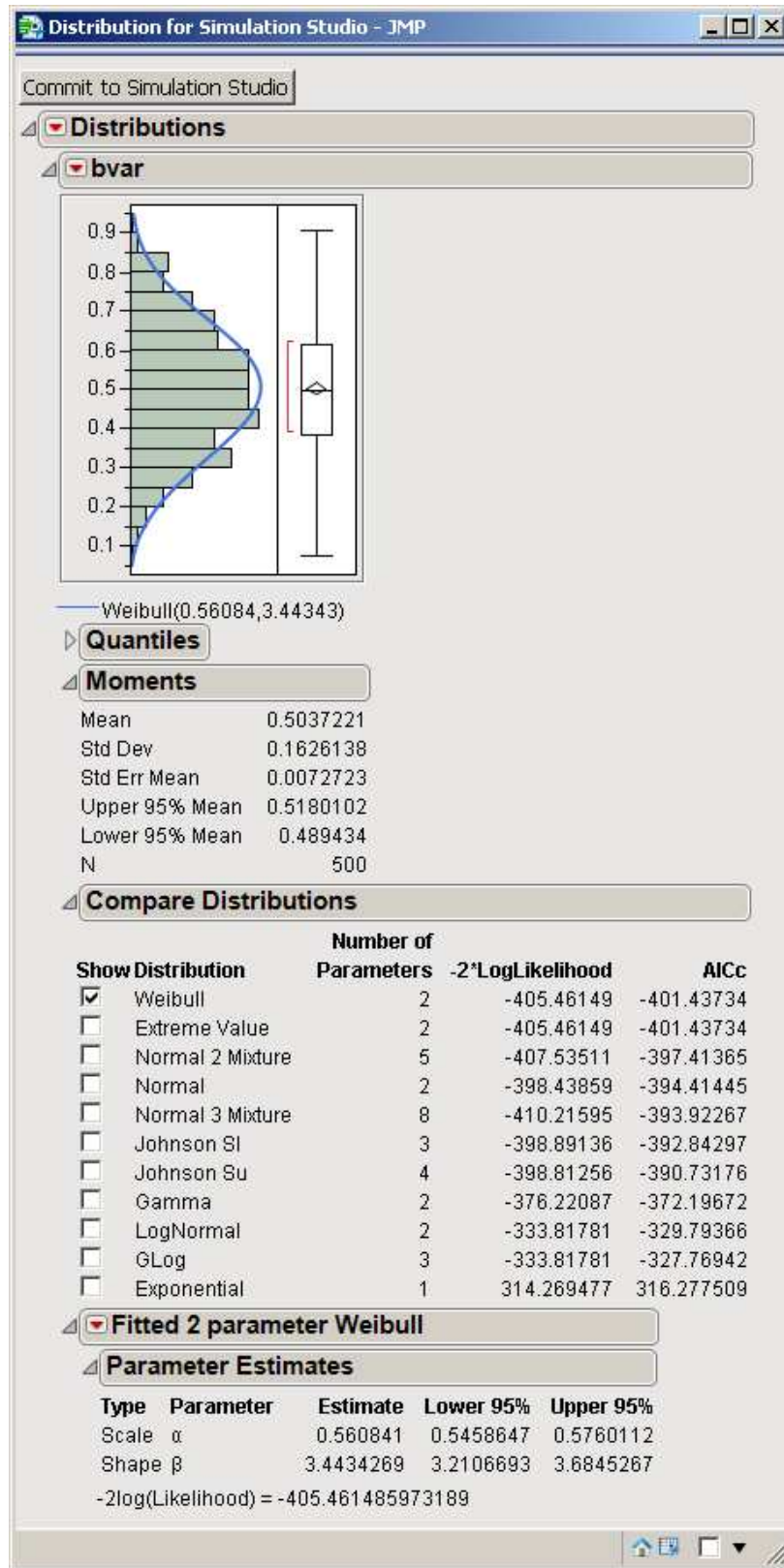
Figure 3: Automatic distribution-fitting in JMP.
