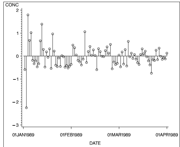
Figure 6. Residuals for Decay Model
