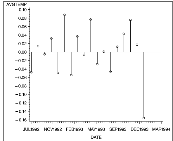
Figure 5. Residuals from OLS
