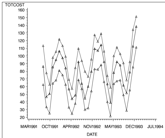
Figure 8. Prediction of TOTCOST with Error Bounds
