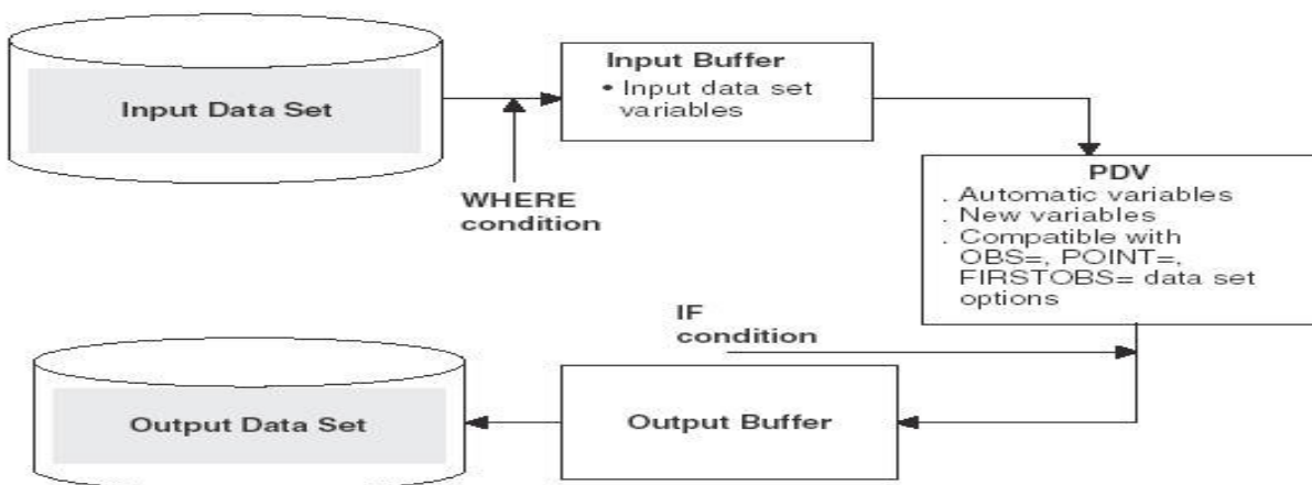
Figure 2.1 WHERE and IF conditions applied.
