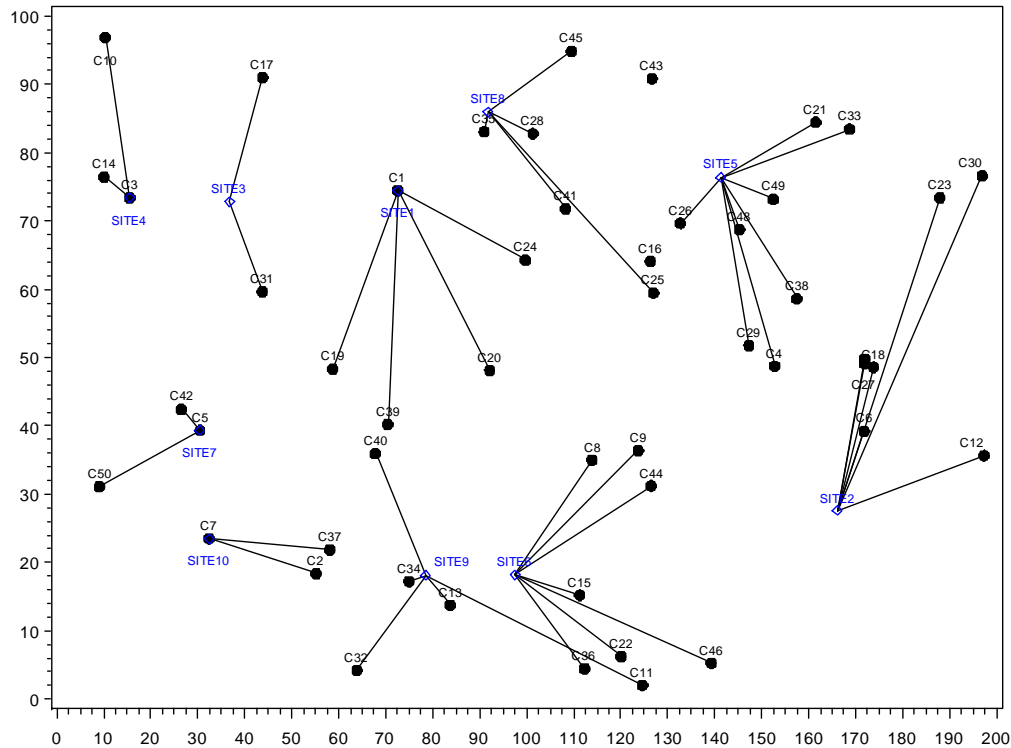
Figure 1. Facility Location Problem Solution without Fixed Charges
