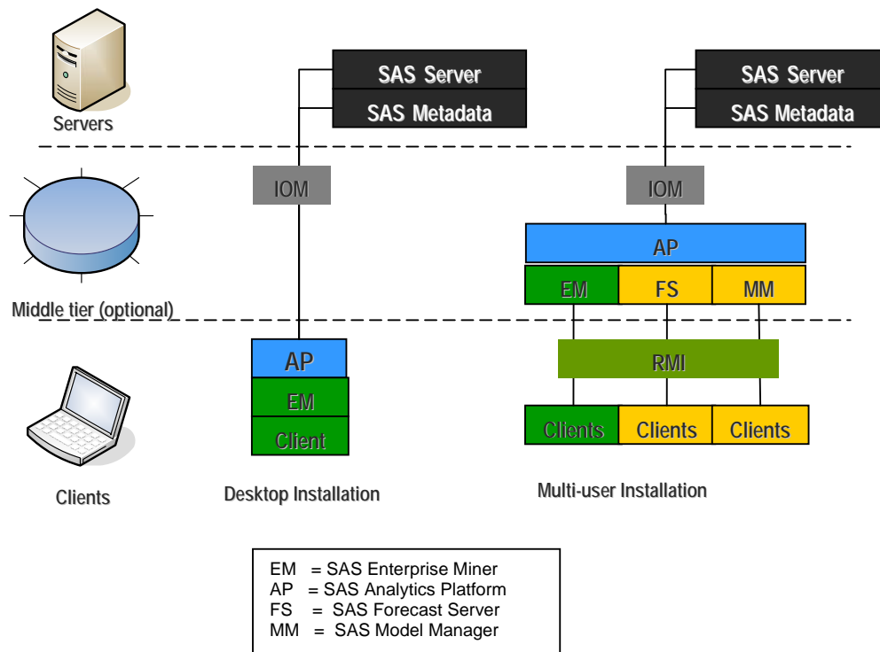
Figure 1: SAS Enterprise Miner three-tier architecture.
