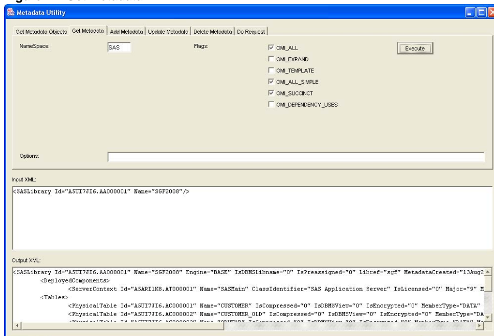
Figure 4 – Get Metadata
