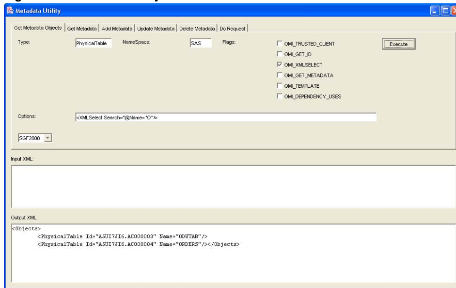
Figure 3 – Get Metadata Objects search tables
