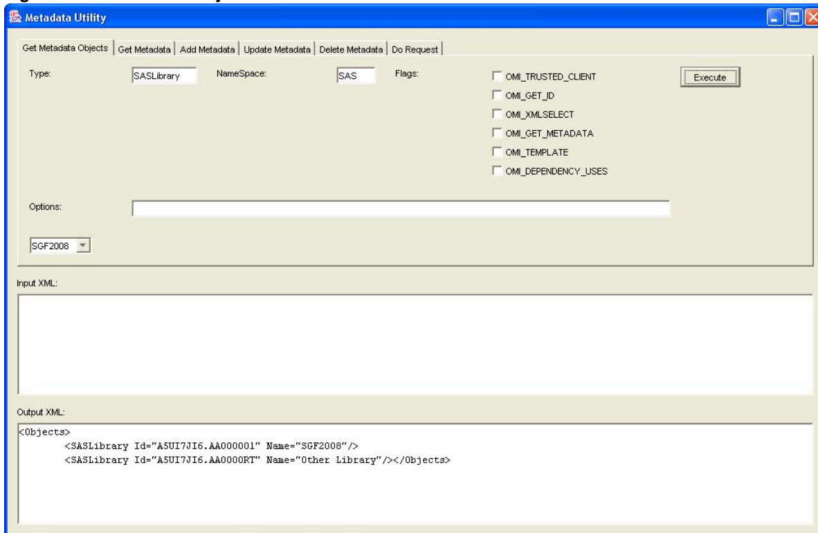
Figure 1 - Get Metadata Objects
