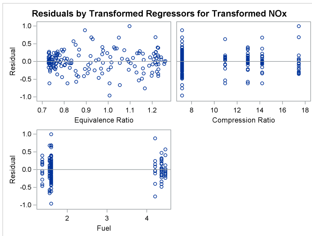
Output 93.1.1 continued
