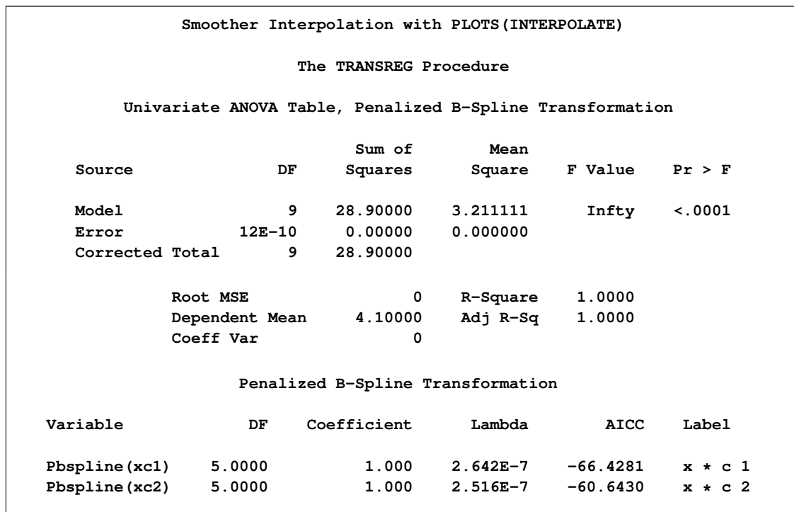
Figure 93.78 Interpolation with PLOTS(INTERPOLATE)
