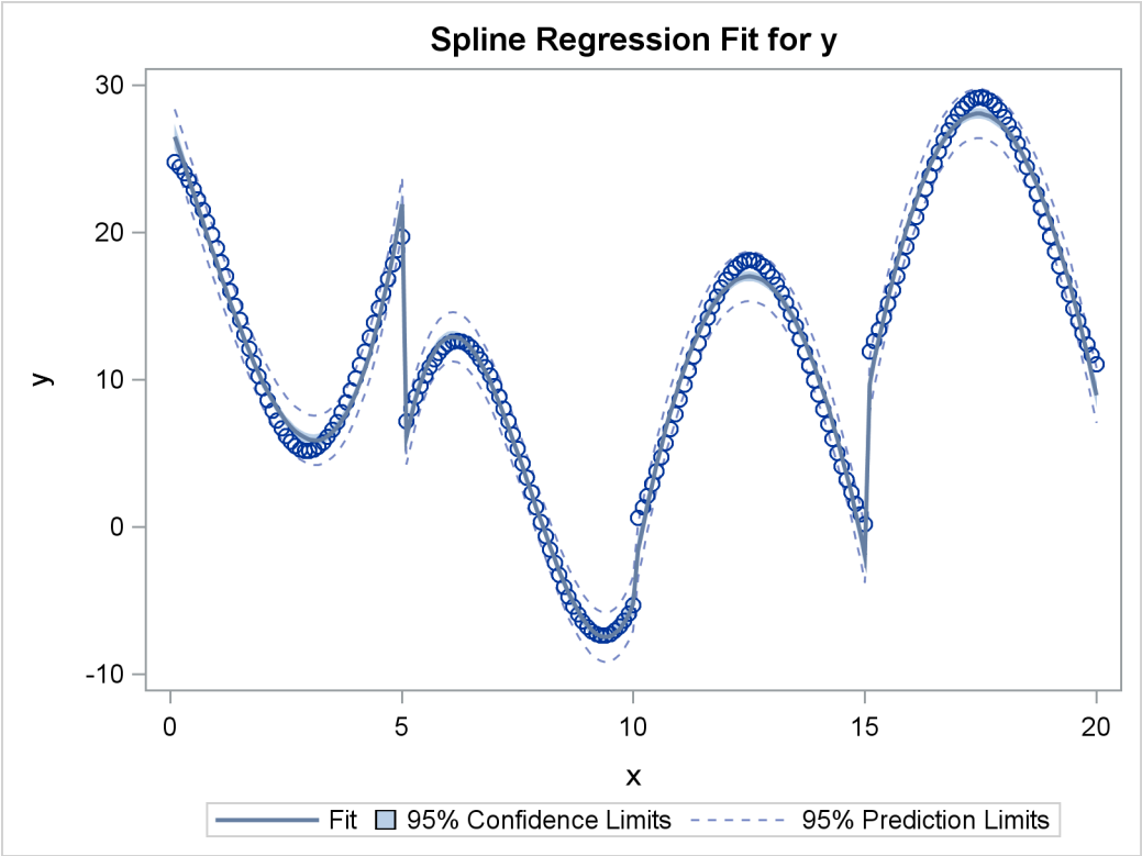
Figure 93.24 continued
