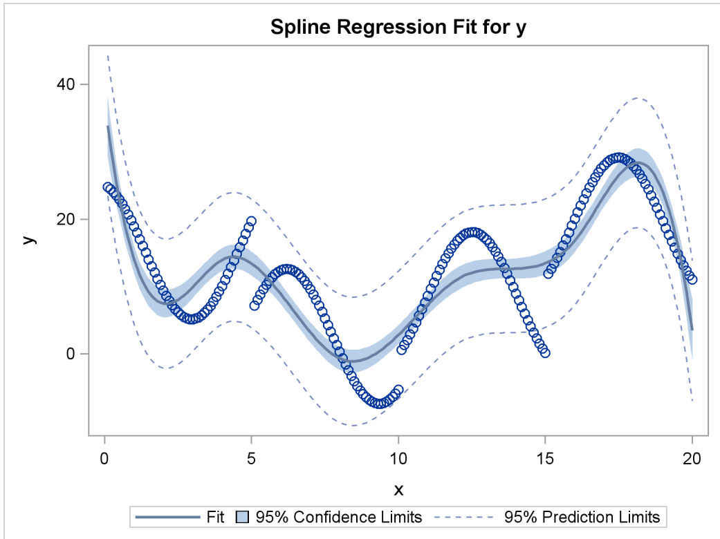
Figure 93.25 continued
