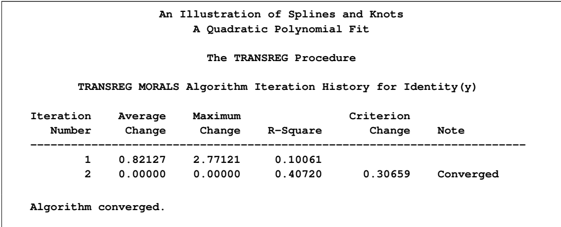
Figure 93.21 A Quadratic Polynomial Fit
