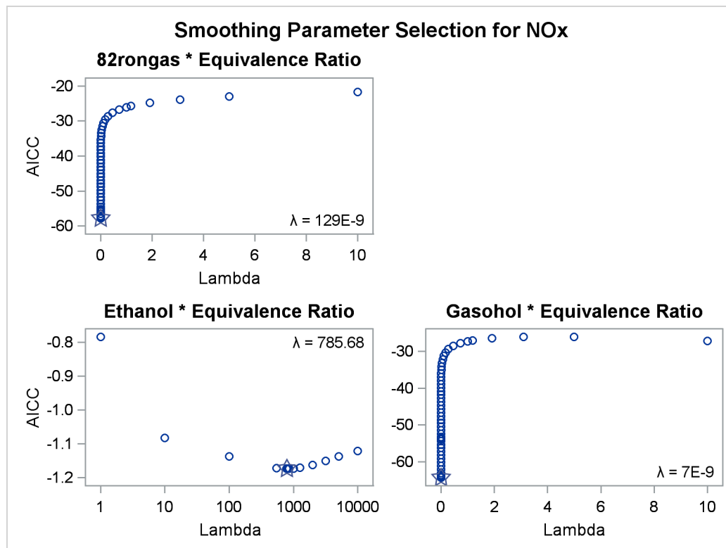
Figure 93.11 Penalized B-Splines
