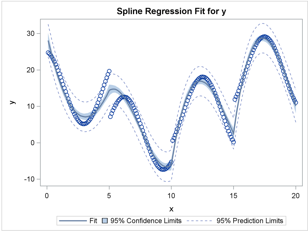
Figure 93.23 continued
