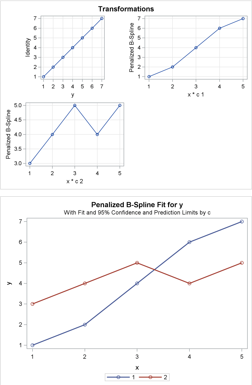
Figure 93.77 continued
