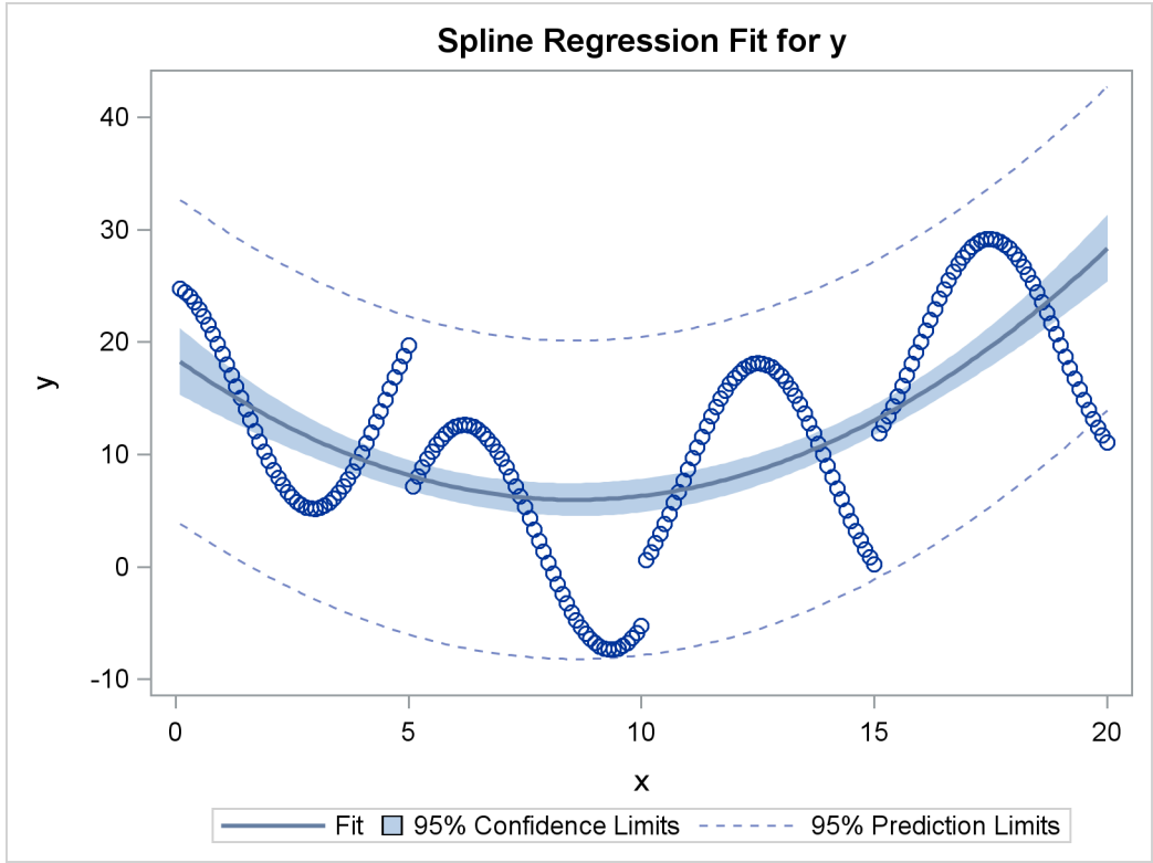
Figure 93.21 continued
