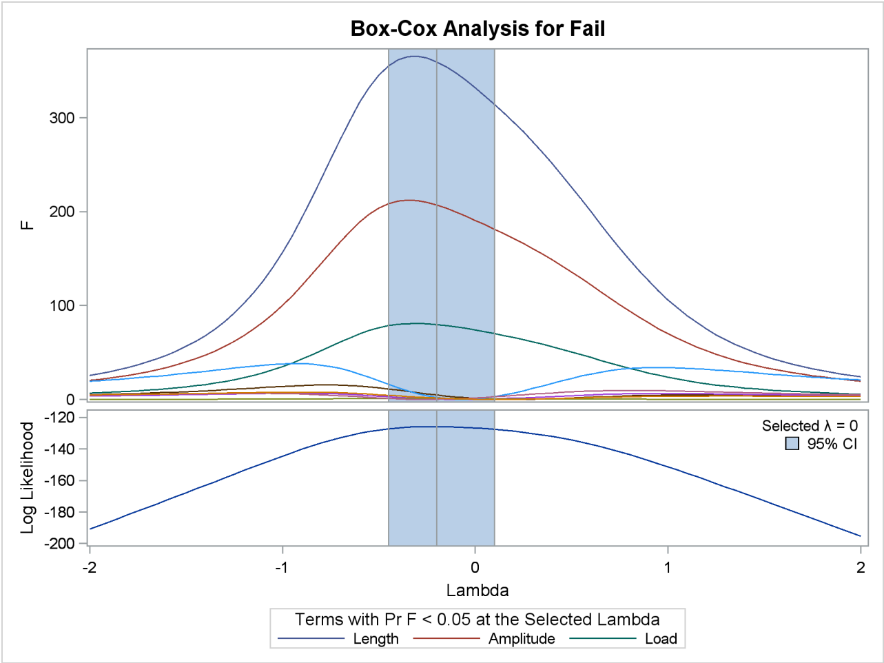
Output 93.2.1 Box-Cox Yarn Data
