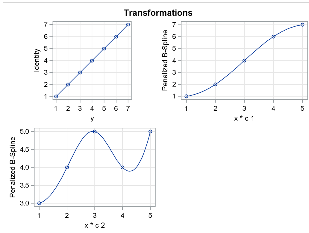
Figure 93.78 continued
