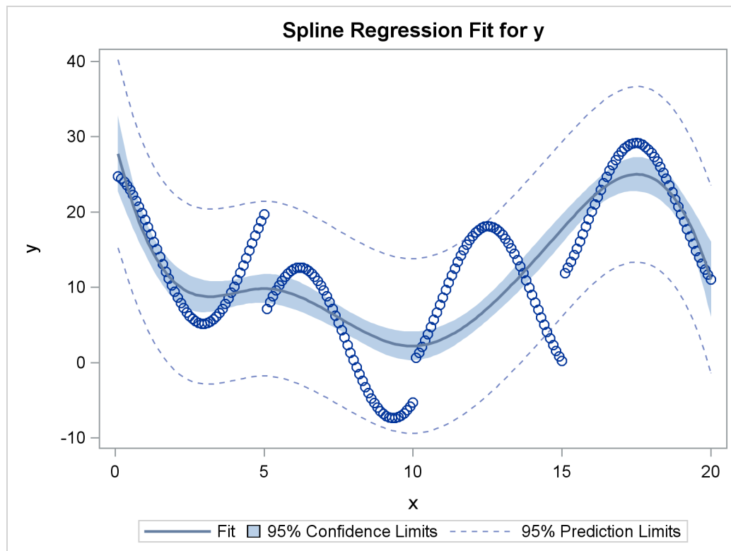
Figure 93.22 continued
