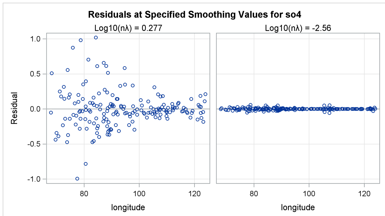
Output 92.3.7 Panel of Residuals by Longitude Plots
