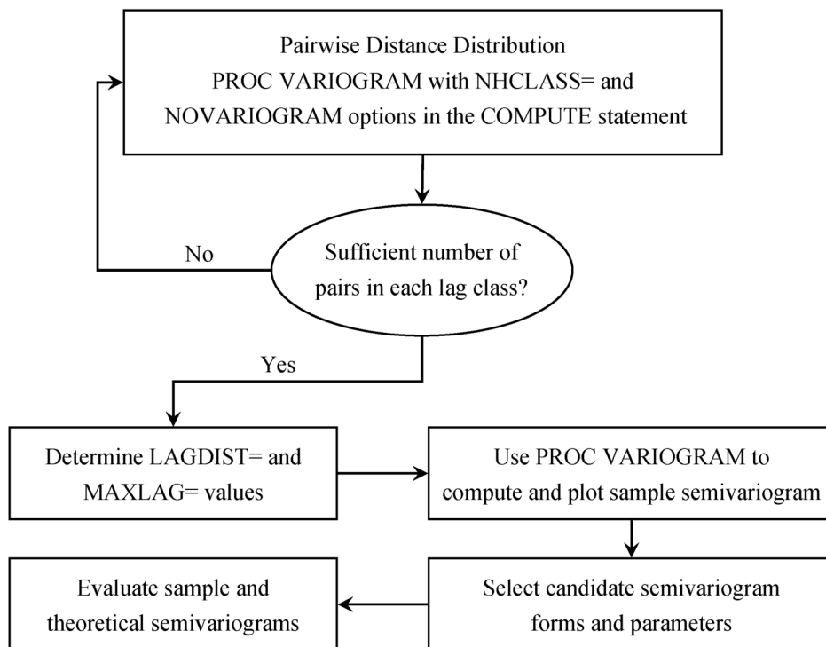
Figure 48.5 Flowchart for Semivariogram Selection
