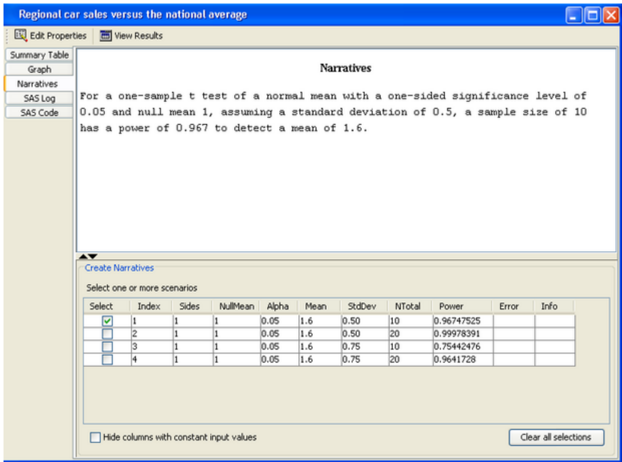
Figure 71.32 Narrative Selector and Display
