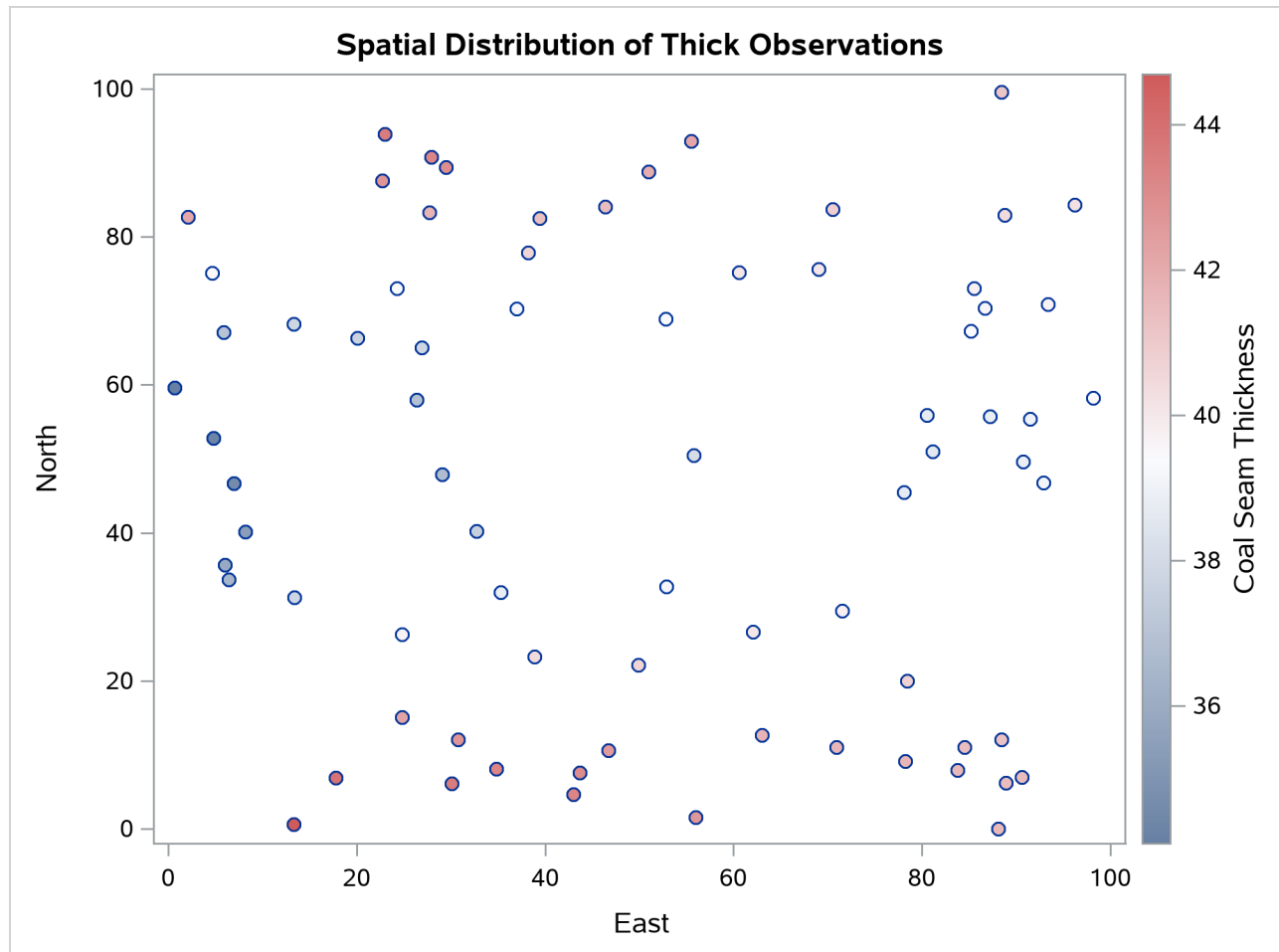
Figure 128.2 Scatter Plot of the Observations Spatial Distribution
