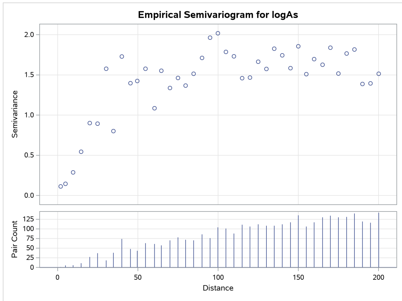
Output 128.1.4 Empirical Semivariogram for logAs Data
