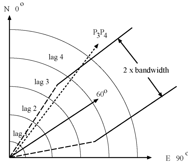
Figure 128.23 Selected Pair P_3P_4 Falls outside Bandwidth Limit
