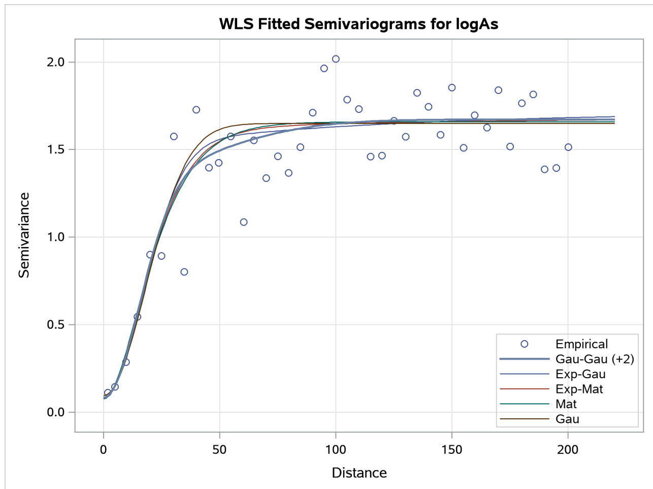
Output 128.1.9 Fitted Theoretical and Empirical logAs Concentration Semivariograms for the Specified Models
