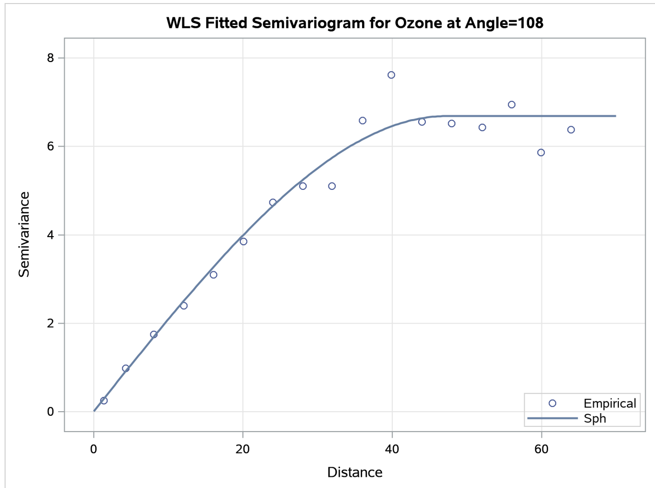
Output 128.3.6 Fitted Theoretical and Empirical Semivariogram for the Ozone Data in \theta = 108^\circ
