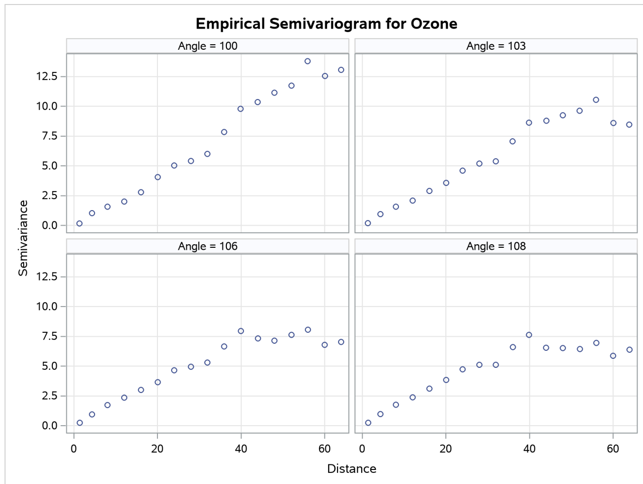
Output 128.3.2 Ozone Empirical Semivariograms in 100^\circ , 103^\circ , 106^\circ , and 108^\circ
