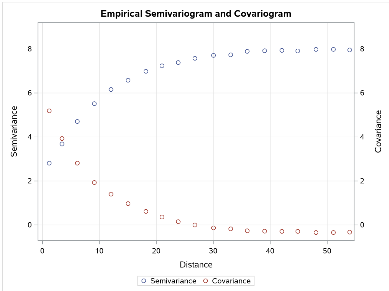
Output 128.4.1 Average Empirical Semivariogram and Covariogram from 500 Simulations
