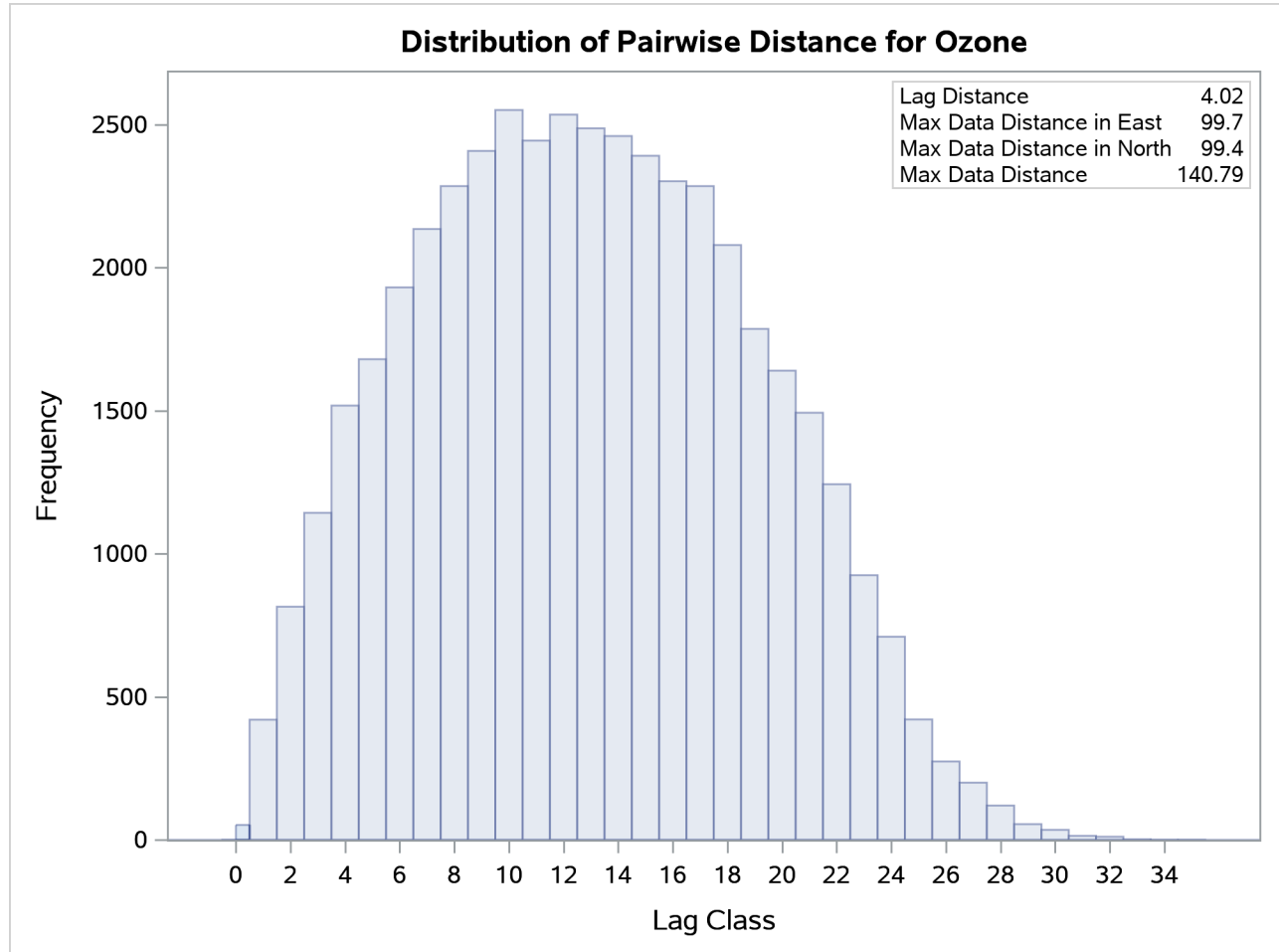
Output 128.2.3 Distribution of Pairwise Distances for Ozone Observation Data
