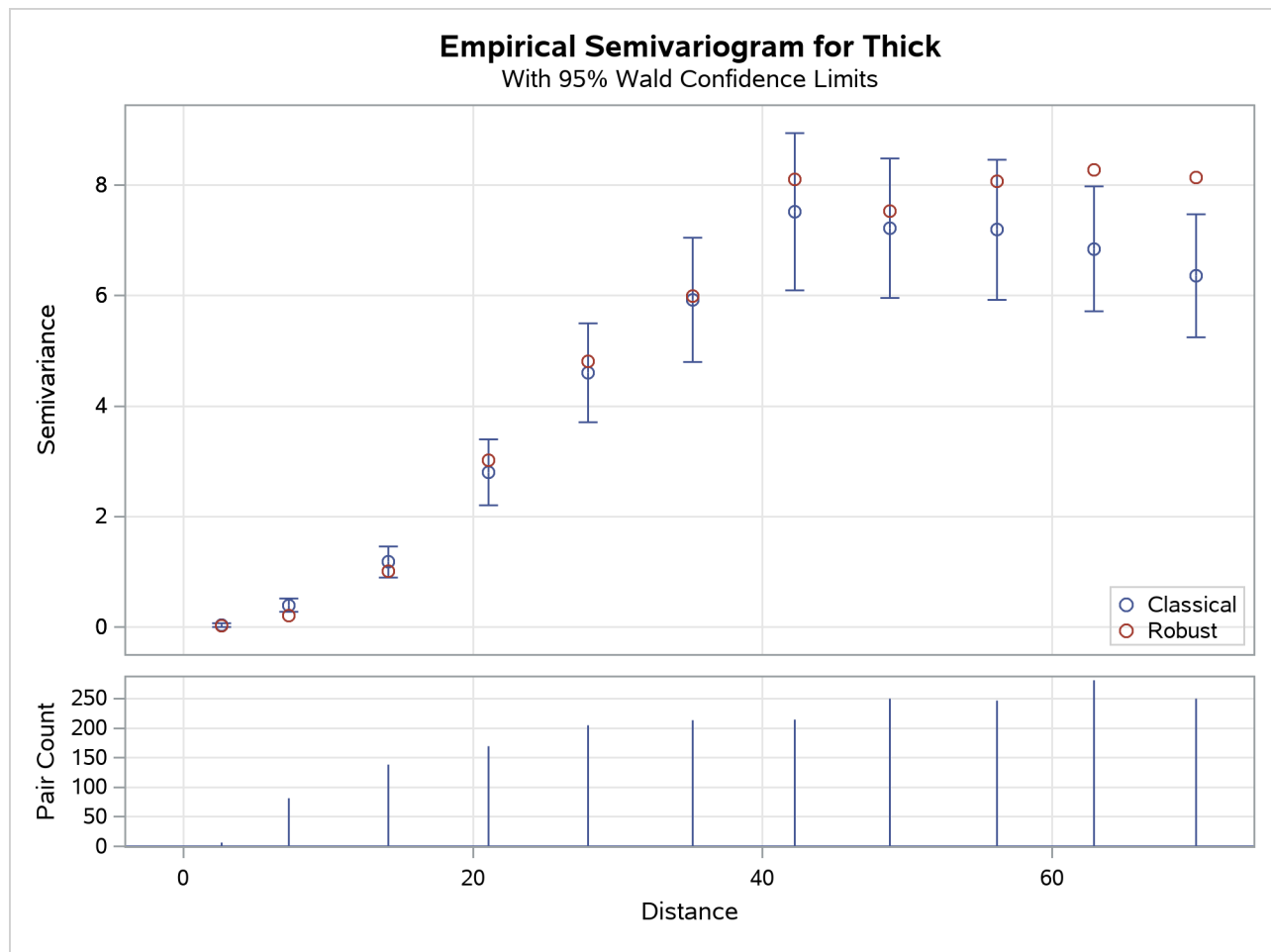
Figure 128.7 Classical and Robust Empirical Semivariograms for Coal Seam Thickness Data
