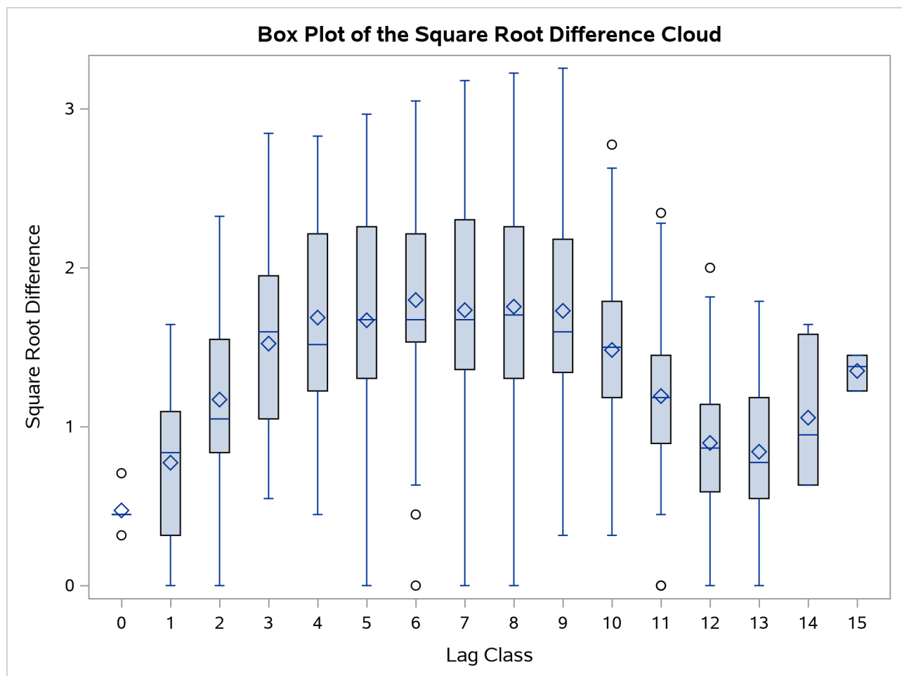
Output 128.5.2 Box Plot of the Square Root Difference Cloud
