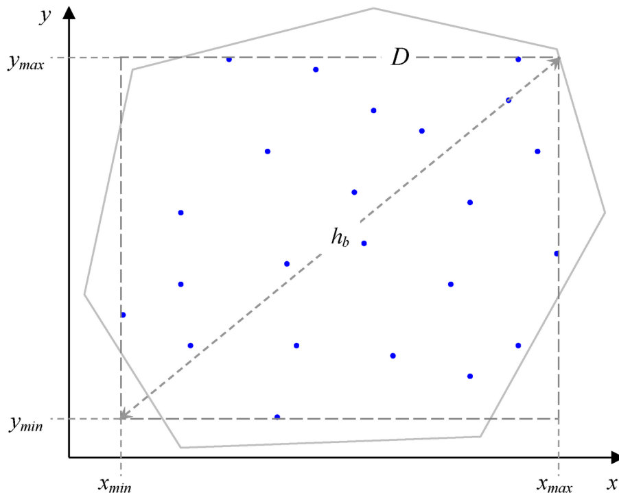
Figure 128.24 Bounding Rectangle to Determine Maximum Pairwise Distance in Domain D
