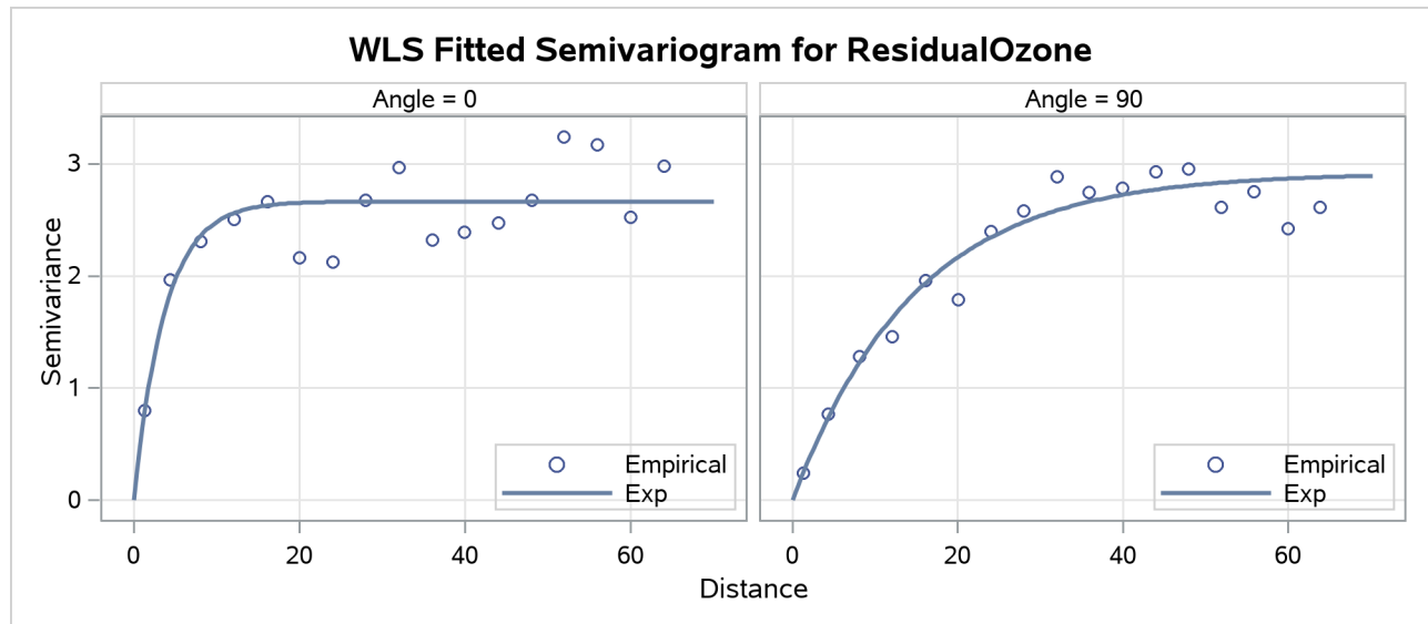
Output 128.2.12 Fitted Theoretical and Empirical Semivariogram for the Ozone Data in the \theta = 0^\circ and \theta = 90^\circ Directions
