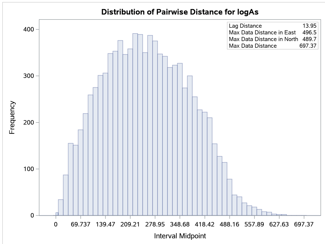
Output 128.1.2 Distribution of Pairwise Distances for logAs Data
