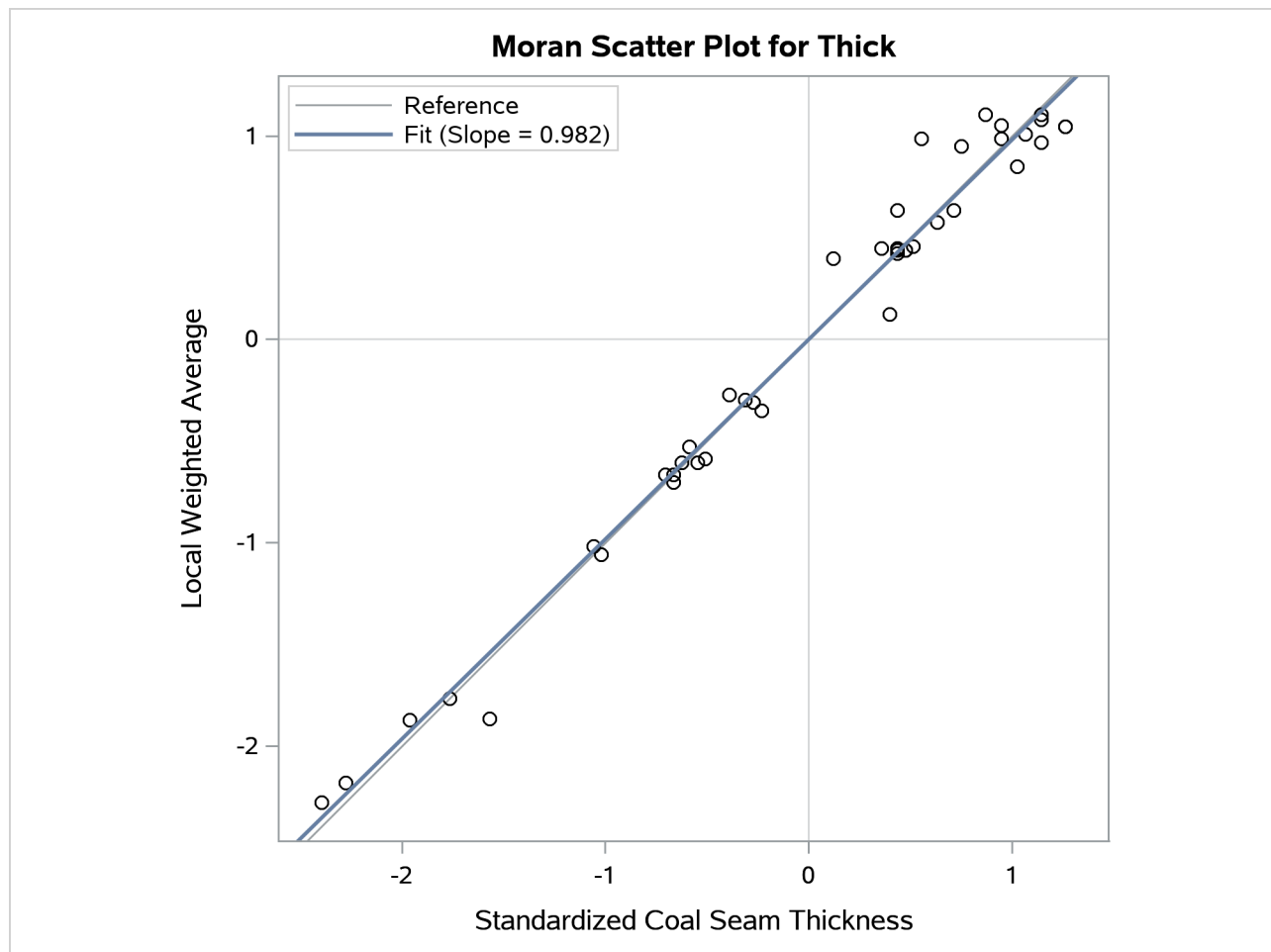
Figure 128.9 Moran Scatter Plot for Coal Seam Thickness Data
