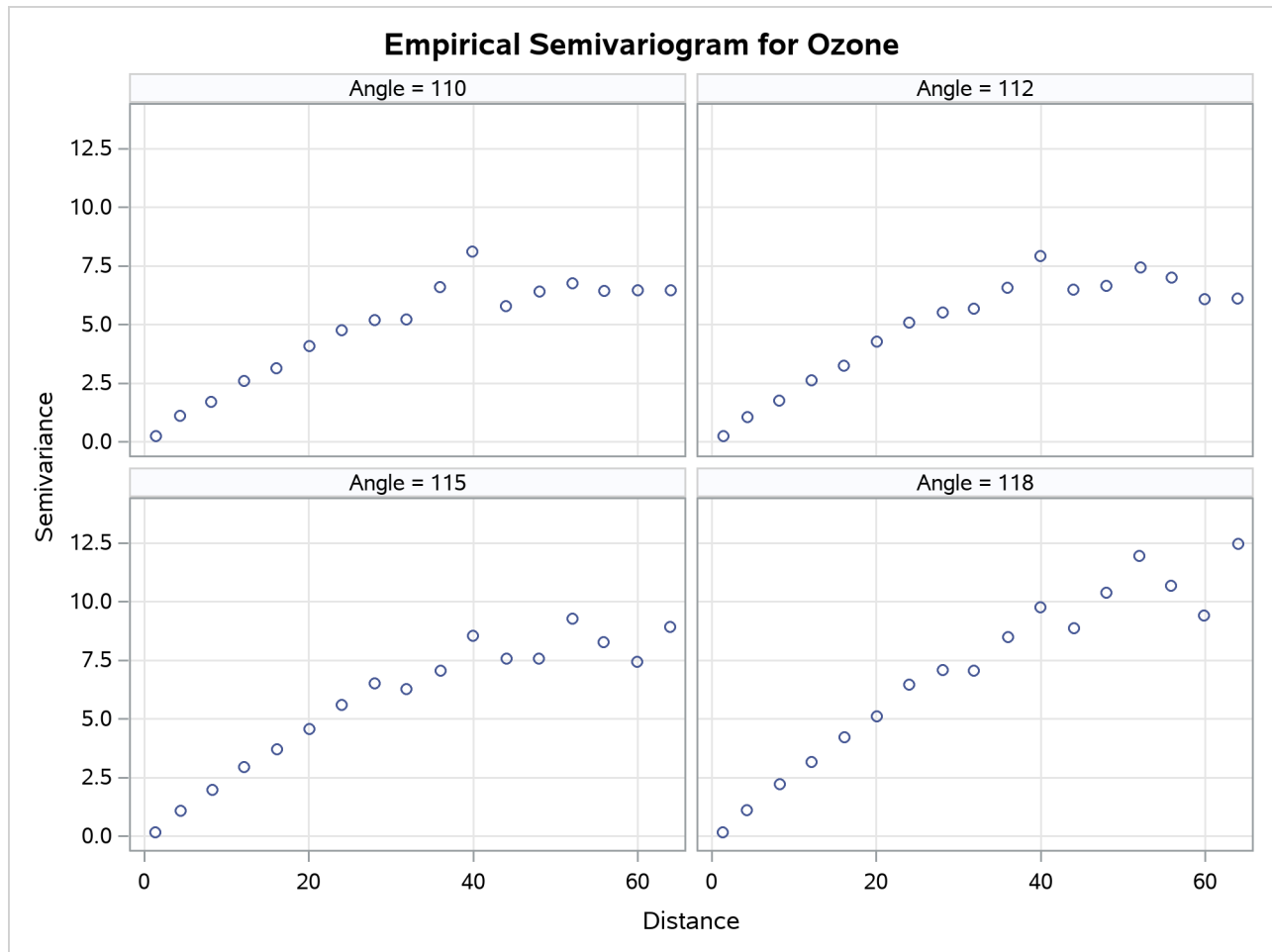
Output 128.3.3 Ozone Empirical Semivariograms in 110°, 112°, 115°, and 118°
