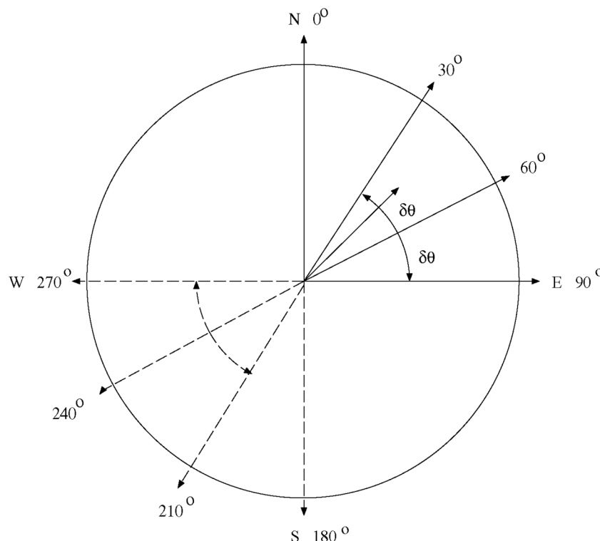
Figure 128.20 Selected Pair P_1 P_2 Falls within the Second Angle Class
