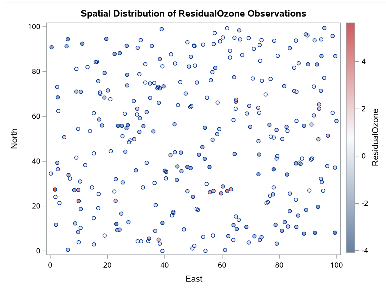
Output 128.2.5 Ozone Residual Observation Data Scatter Plot
