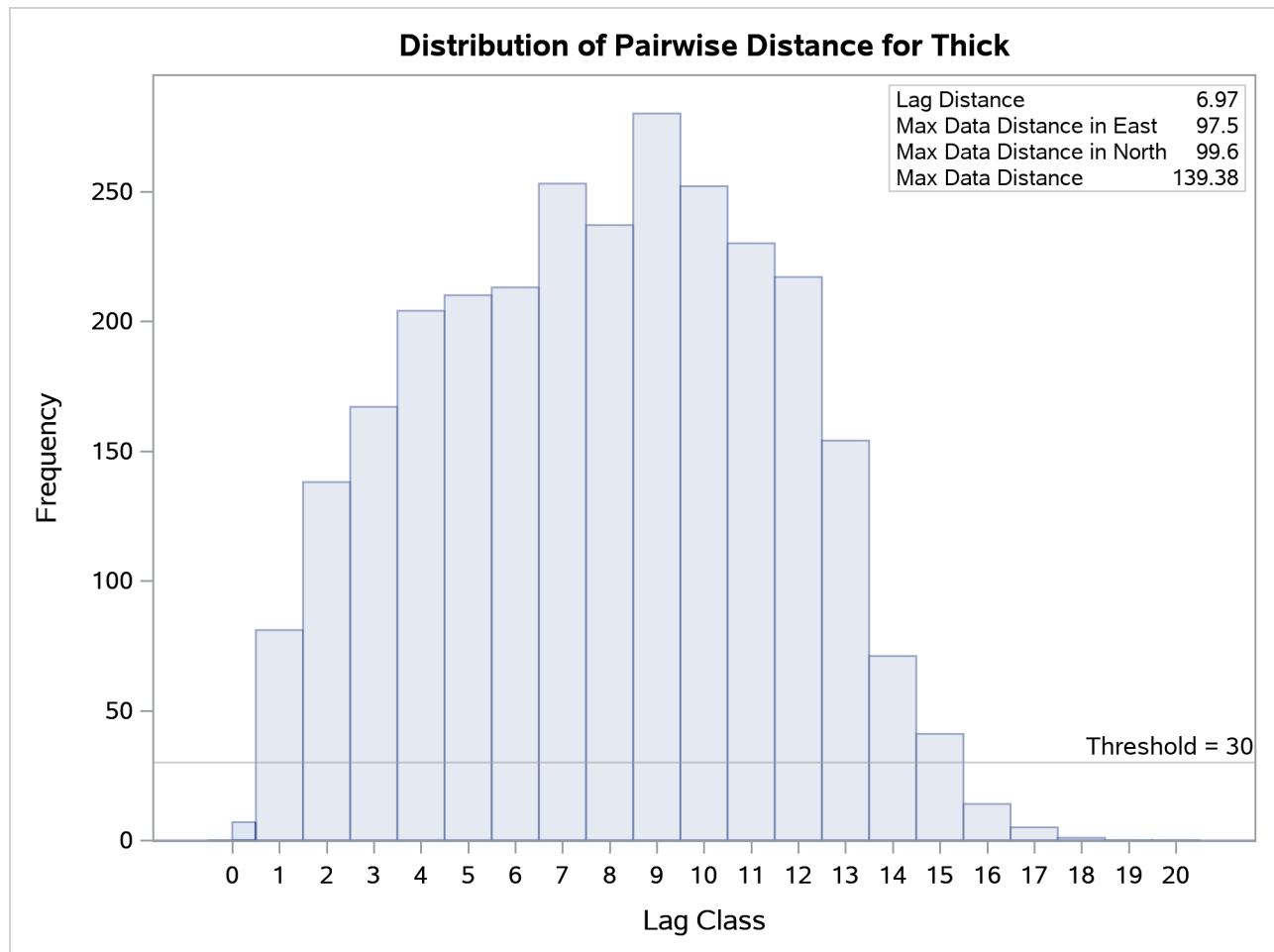
Figure 128.4 Distribution of Pairwise Distances
