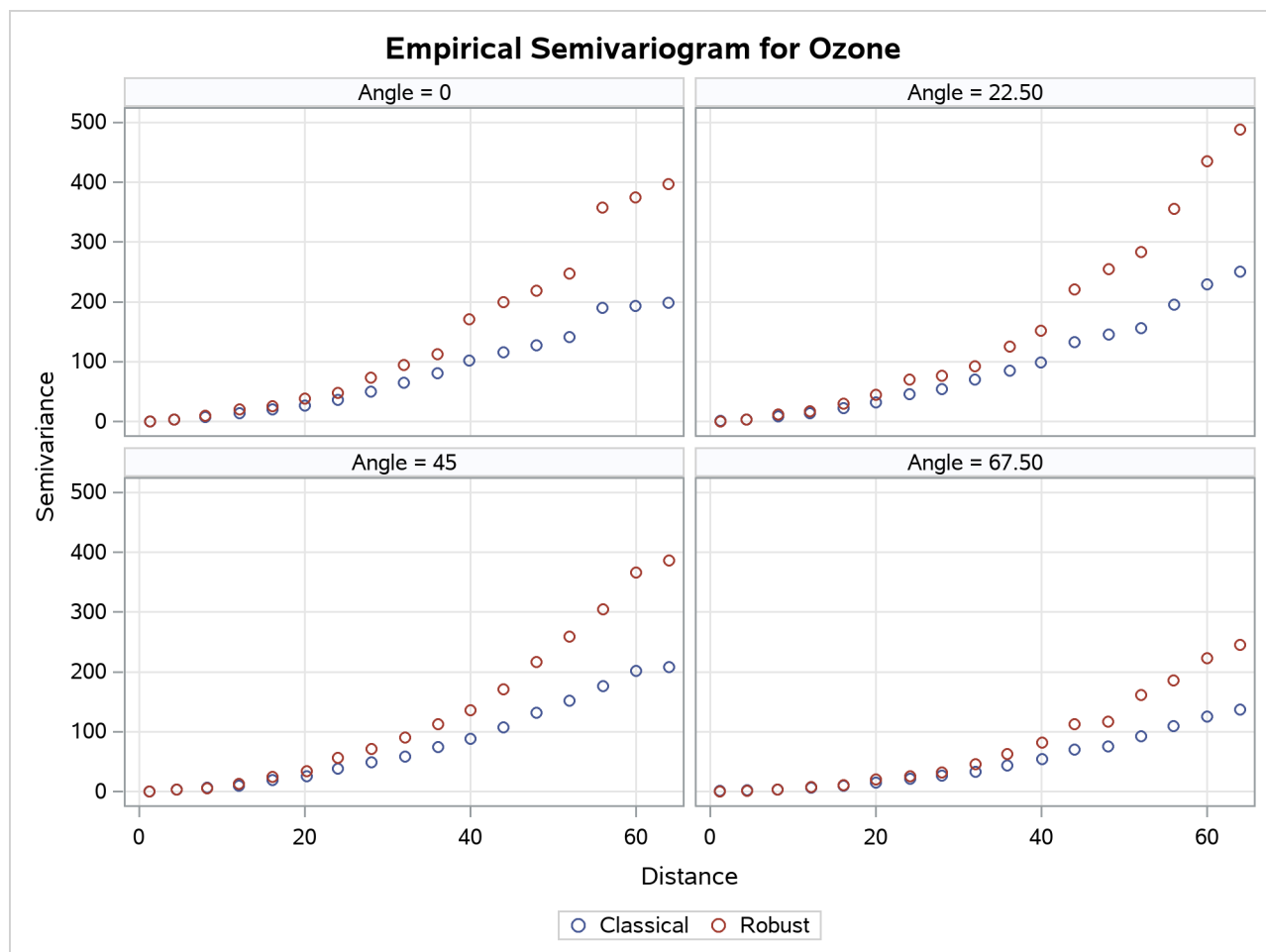
Output 128.3.1 Ozone Empirical Semivariograms with 0^\circ \leq \theta < 180^\circ and \delta\theta = 22.5^\circ
