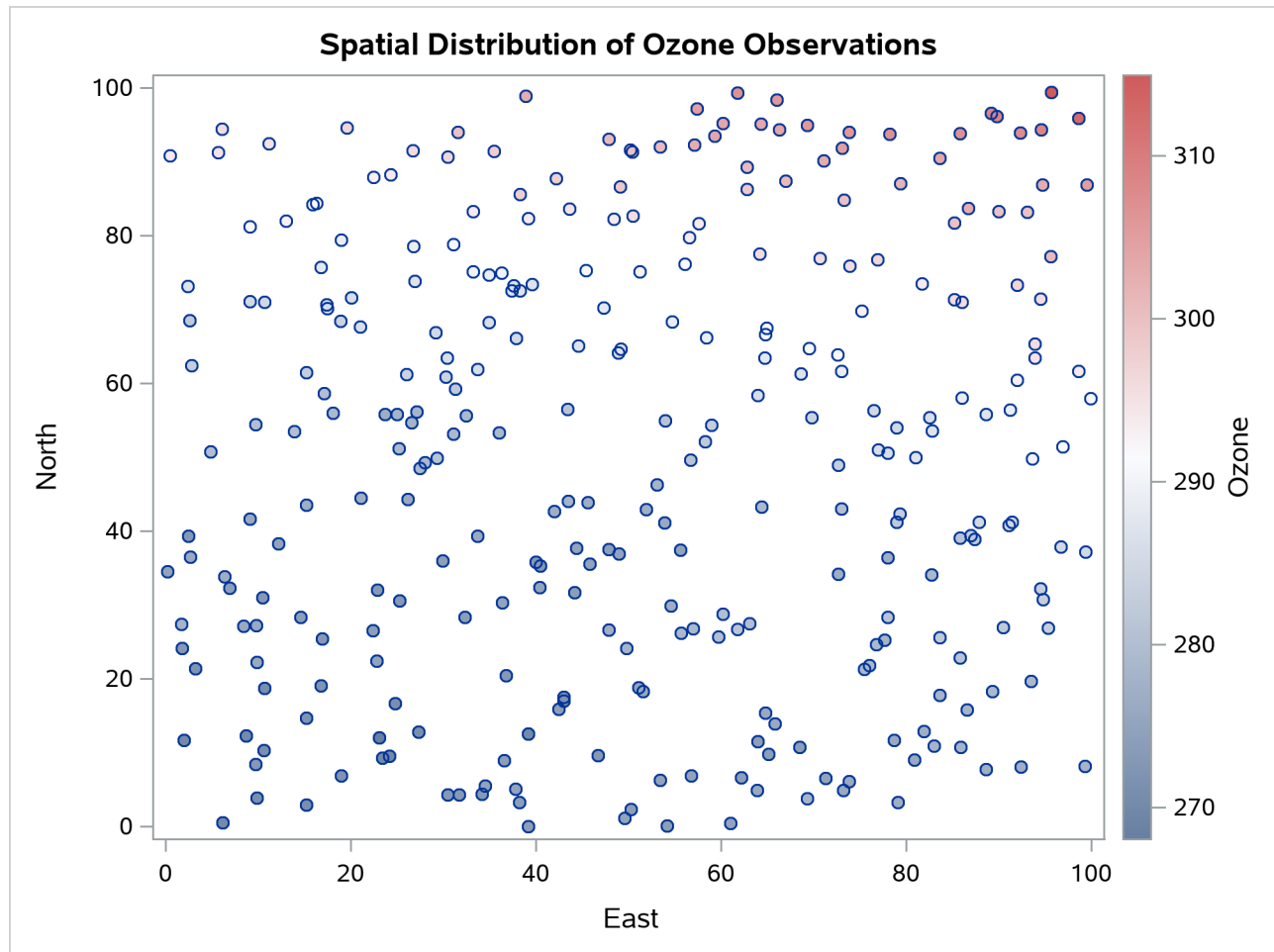
Output 128.2.1 Ozone Observation Data Scatter Plot
