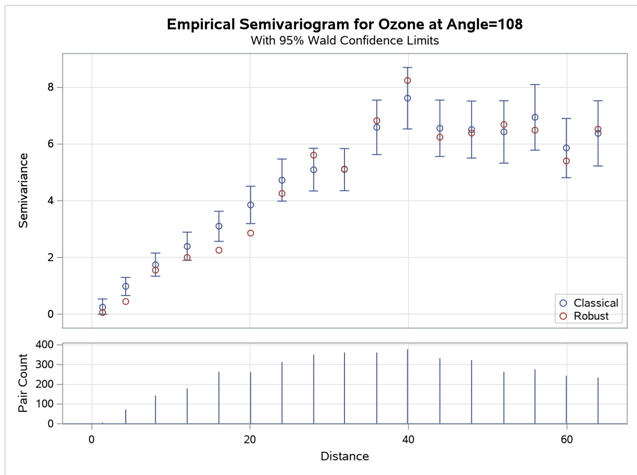
Output 128.3.4 Ozone Classical and Robust Empirical Semivariograms in \theta = 108^\circ
