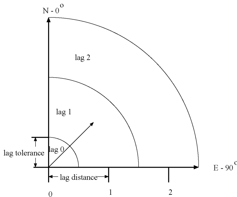
Figure 128.21 Selected Pair P_1 P_2 Falls within the First Lag Class
