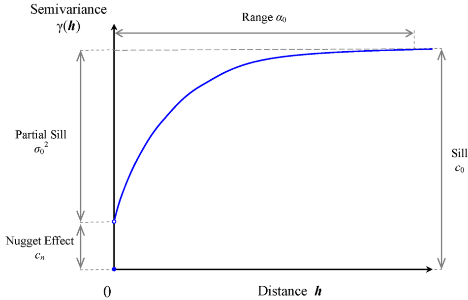
Figure 128.18 A Theoretical Semivariogram of Spherical Type and Its Characteristics
