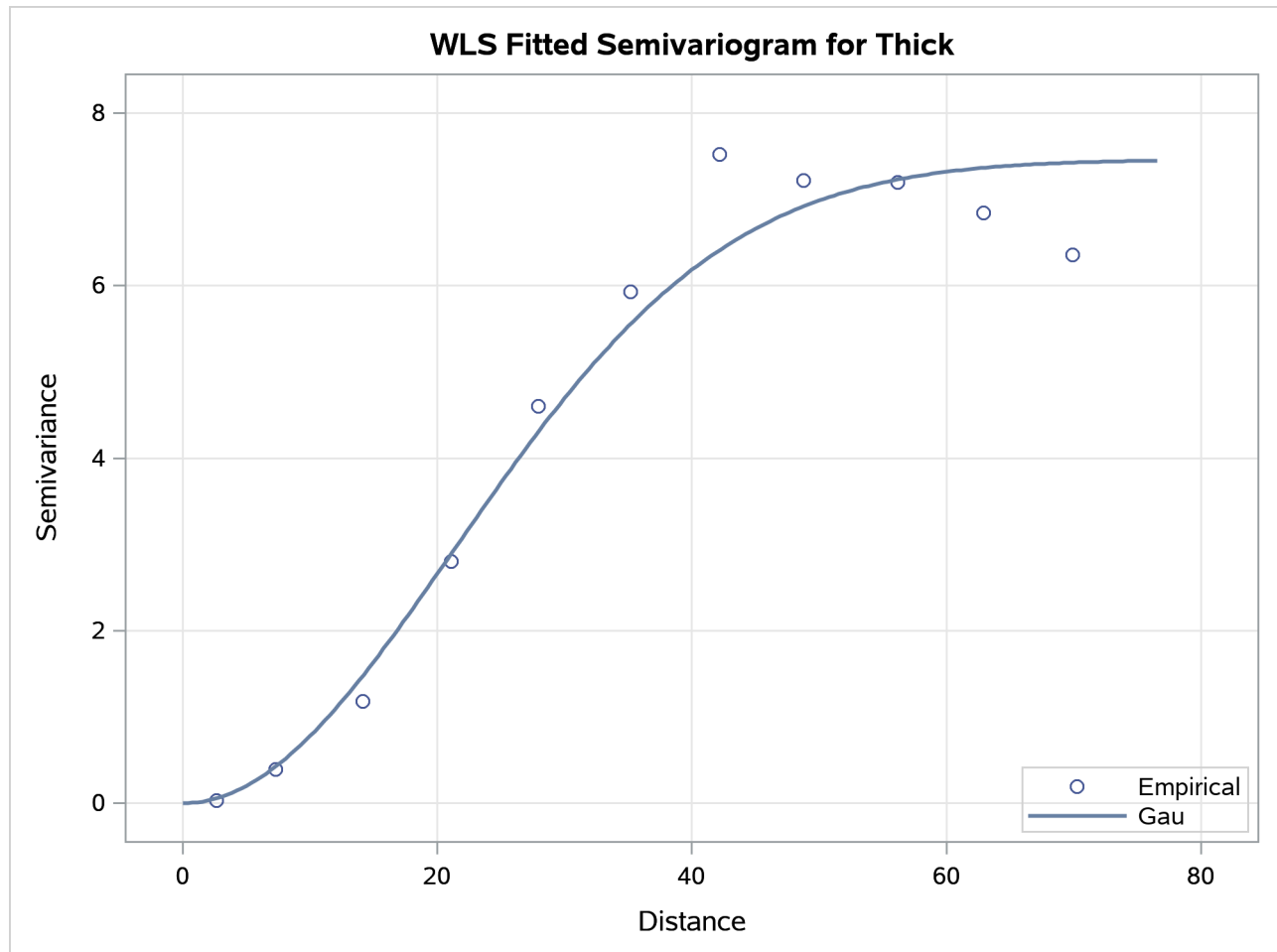
Figure 128.16 Fitted Theoretical and Empirical Semivariogram for Coal Seam Thickness
