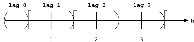
Figure 128.22 Lag Distance Axis Showing Lag Classes
