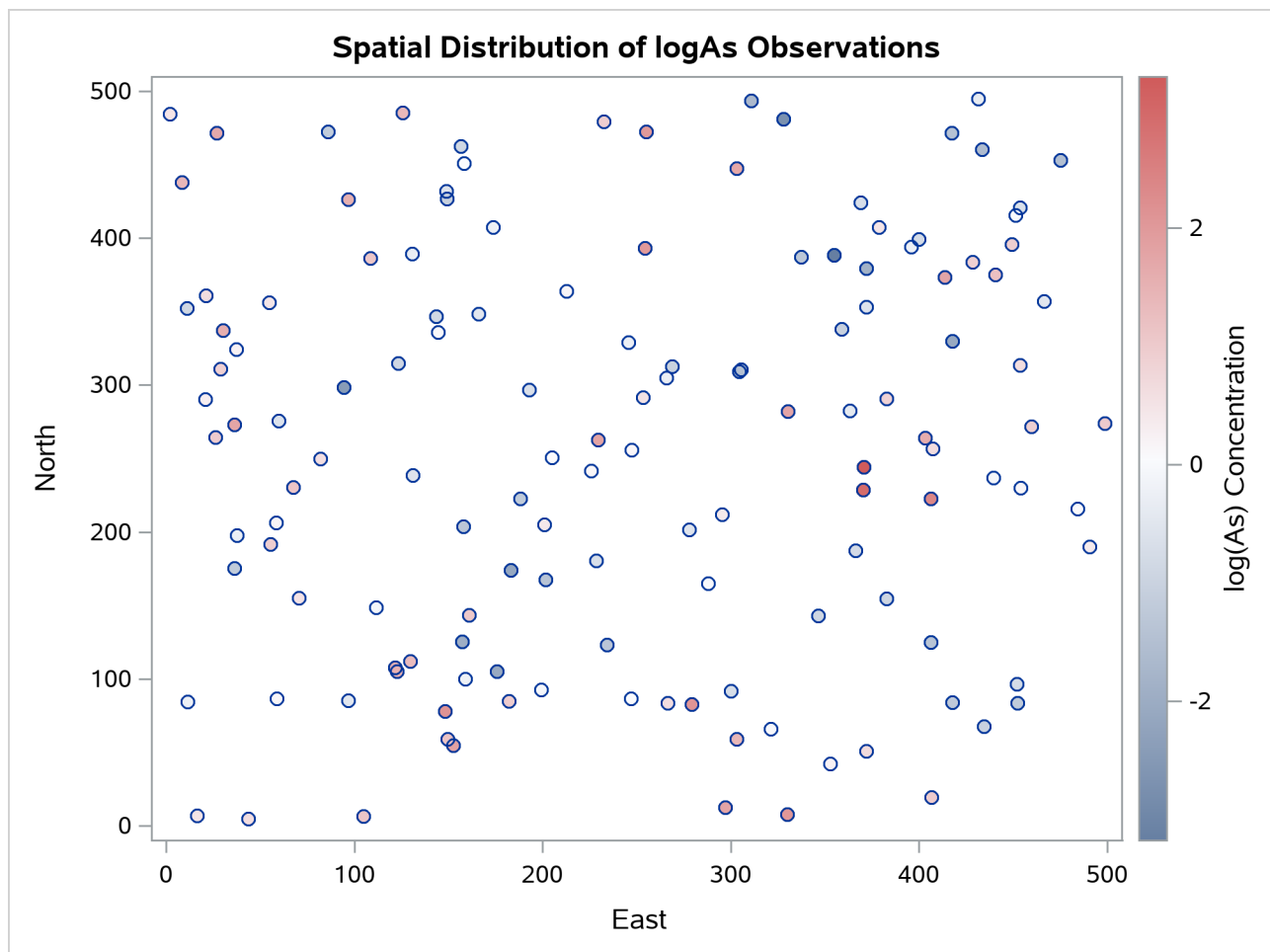
Output 128.1.1 logAs Observation Data Scatter Plot
