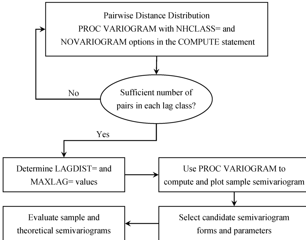
Figure 128.17 Flowchart for Semivariogram Selection
