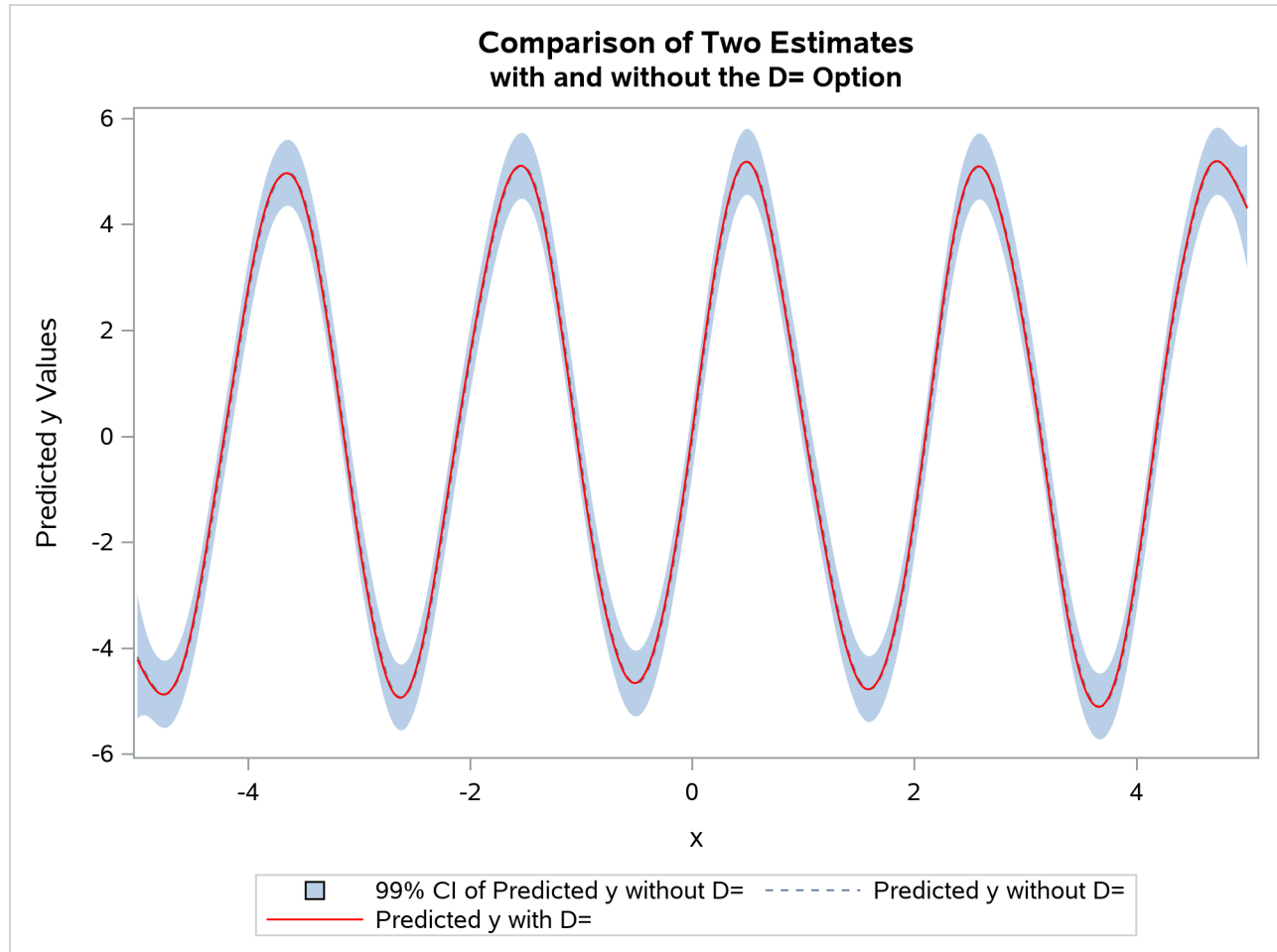
Output 122.4.3 Comparison of Two PROC TPSPLINE Fits with and without the D= Option
