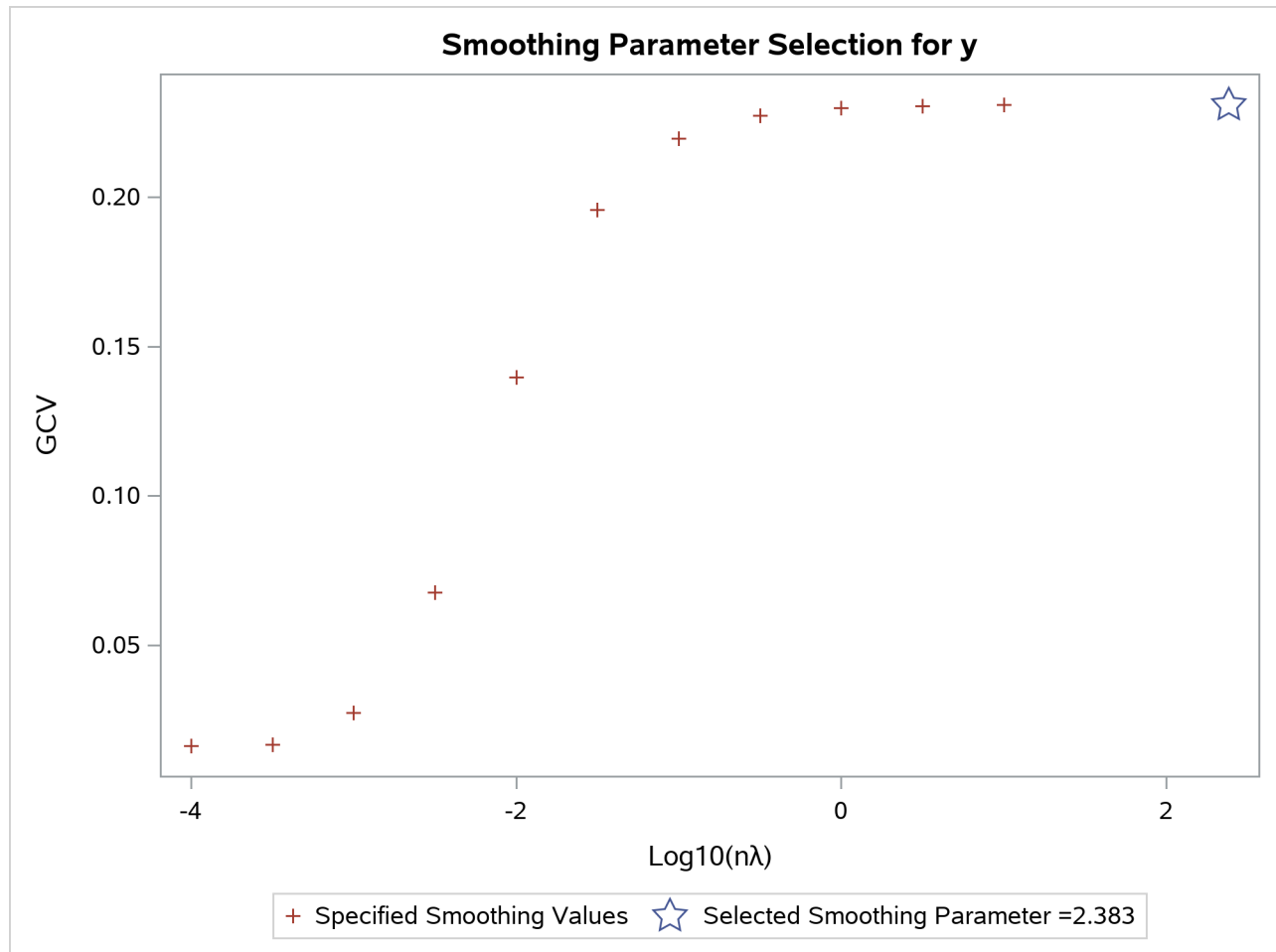
Output 122.2.4 Criterion Plot
