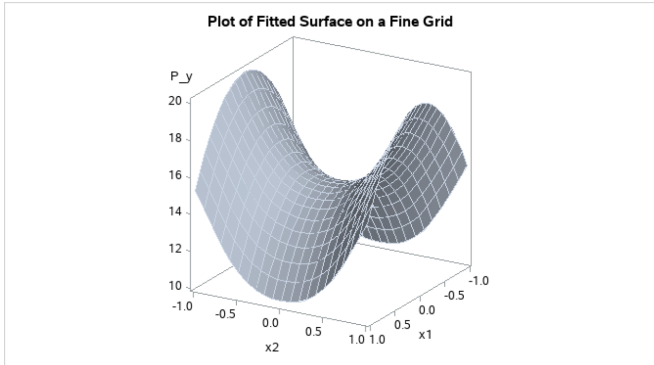
Output 122.1.2 Plot of PROC TPSPLINE Fit from the Partial Spline Model
