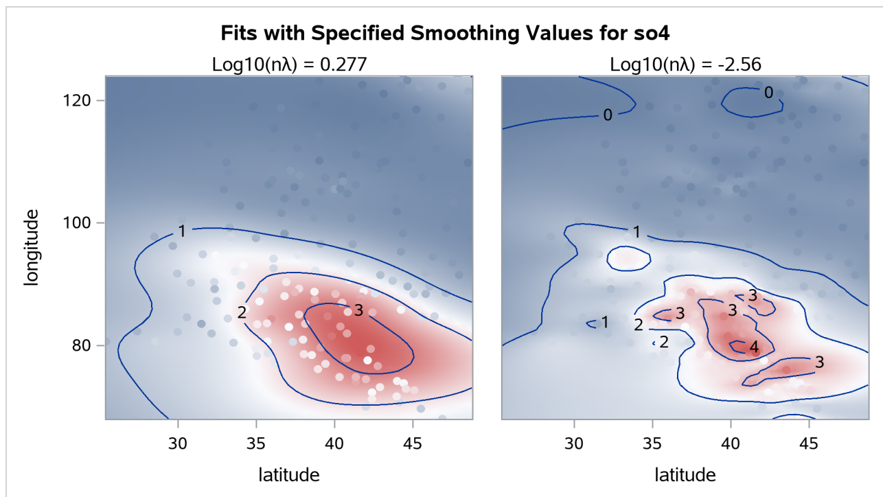
Output 122.3.5 Panel of Contour Fit Plots by 0.277 and -2.56
