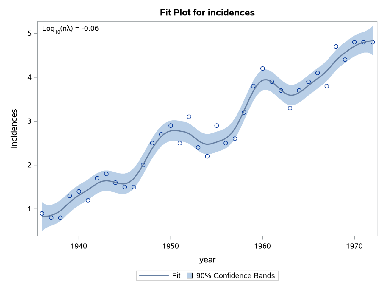
Output 122.5.2 PROC TPSPLINE Estimate and 90% Confidence Interval of Data Set MELANOMA
