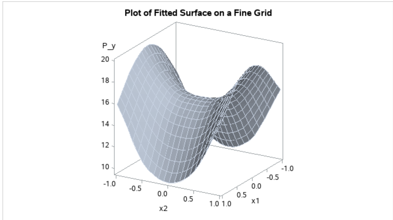
Figure 122.6 Plot of TPSPLINE Fit
