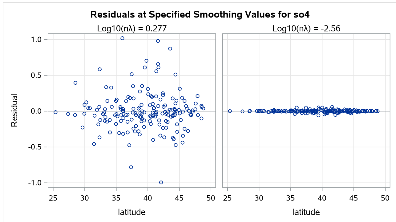
Output 122.3.6 Panel of Residuals by Latitude Plots
