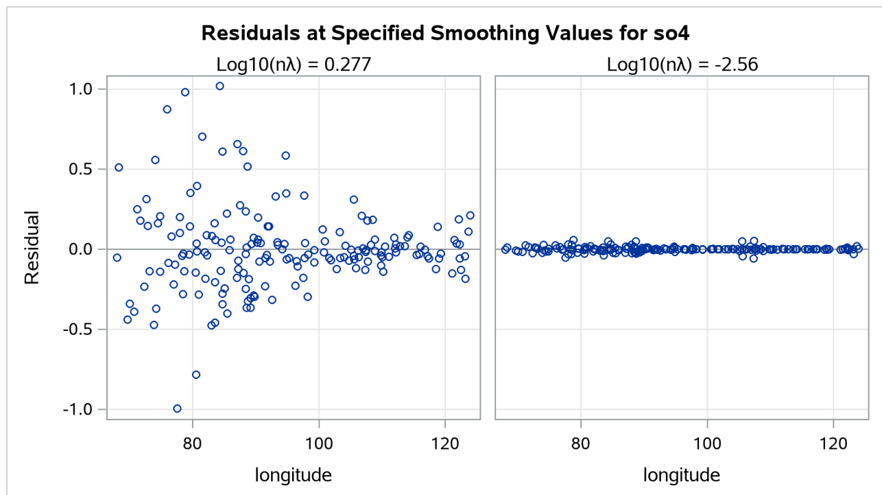
Output 122.3.7 Panel of Residuals by Longitude Plots
