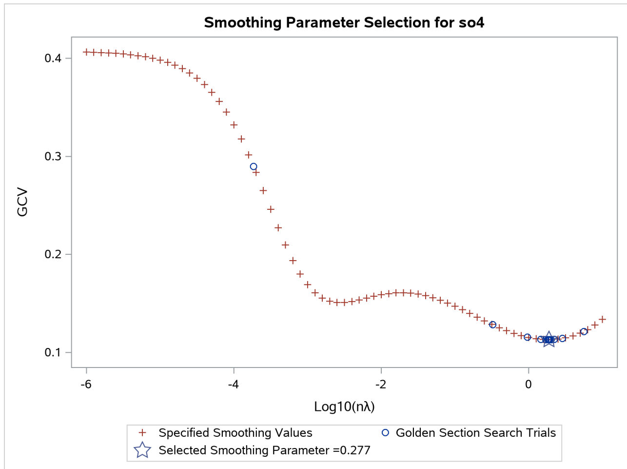
Output 122.3.3 GCV Function of SO 4 Data Set
