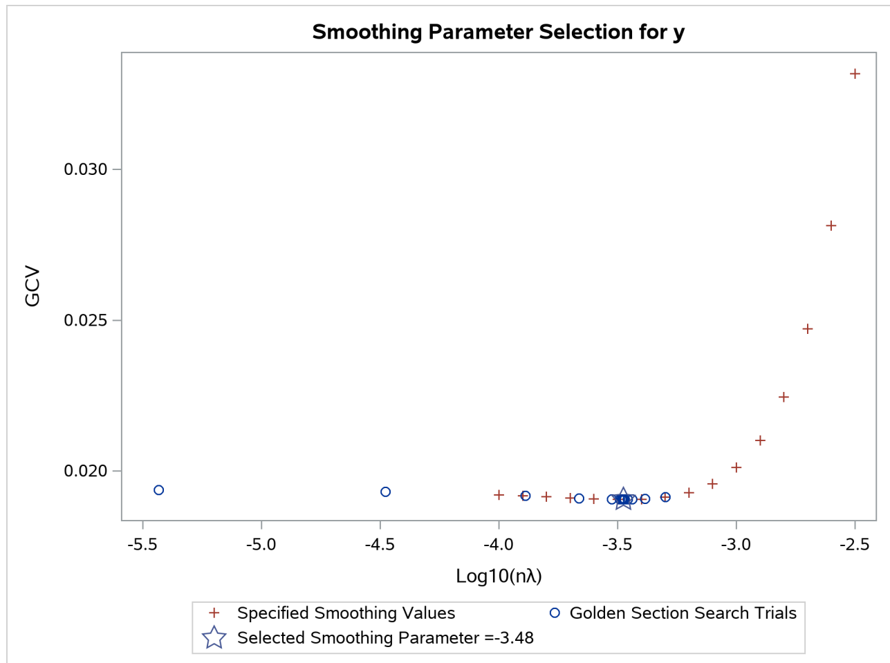
Figure 122.3 The GCV Criterion by \log_{10}(n\lambda)
