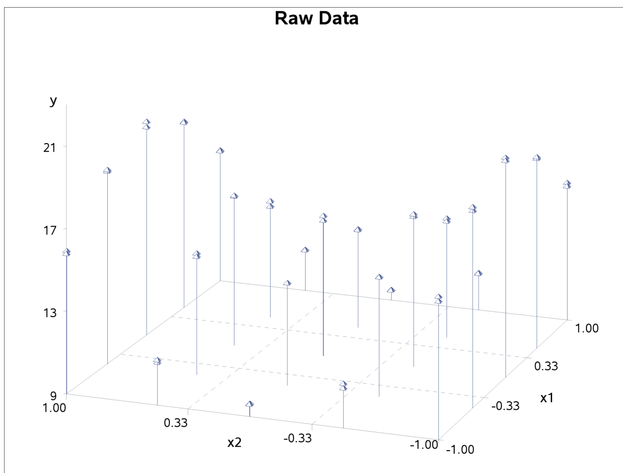
Figure 122.1 Plot of Data Set MEASURE
