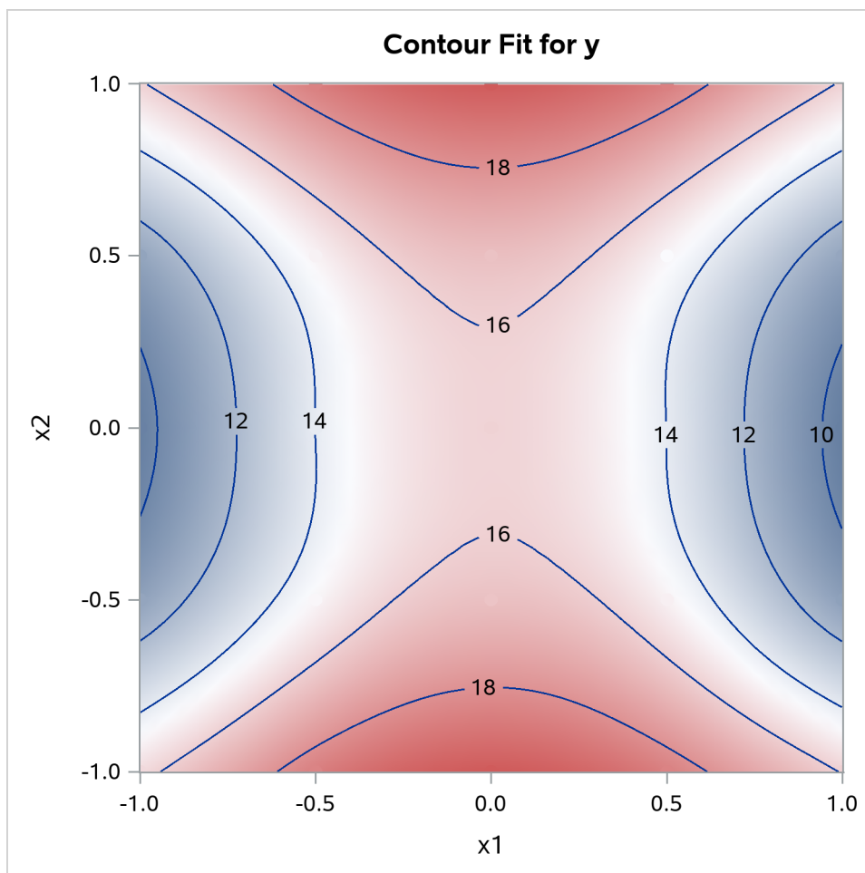
Figure 122.2 Fitted Surface from PROC TPSPLINE
