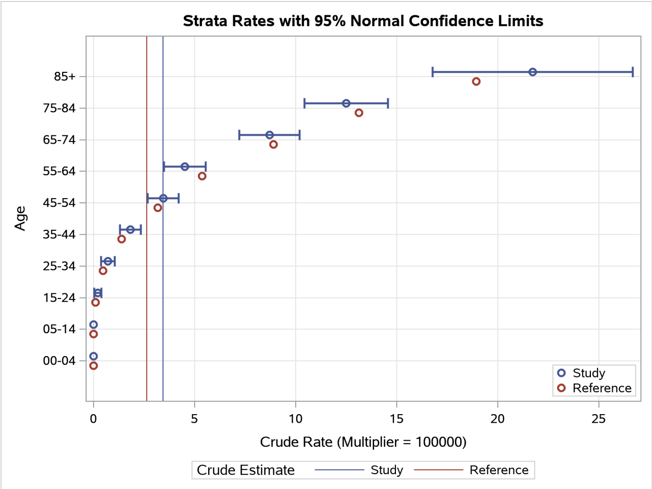
Figure 113.4 Strata Rate Plot
