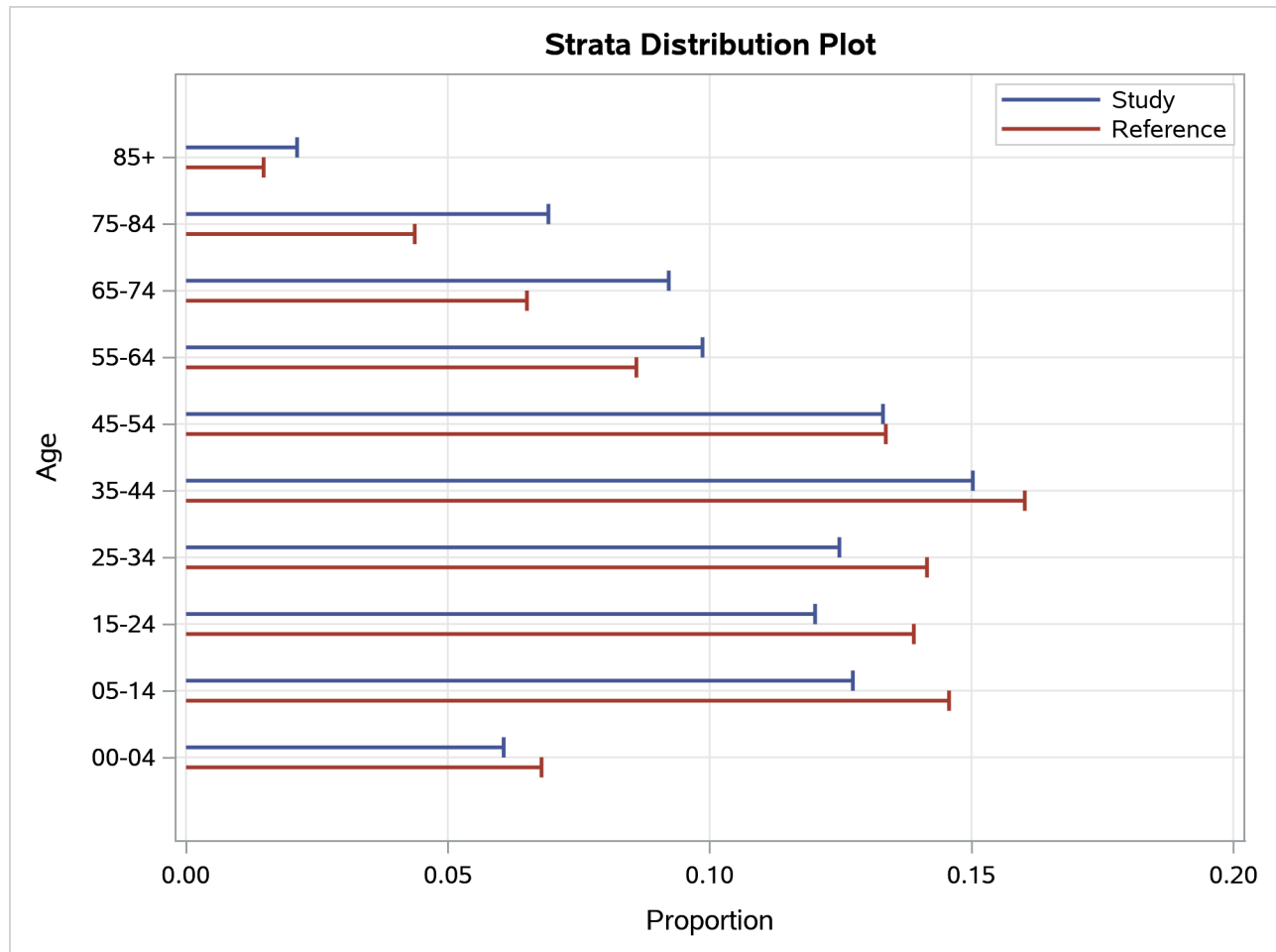
Figure 113.3 Strata Distribution Plot
