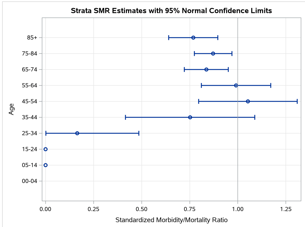
Output 113.4.7 Strata SMR Plot
