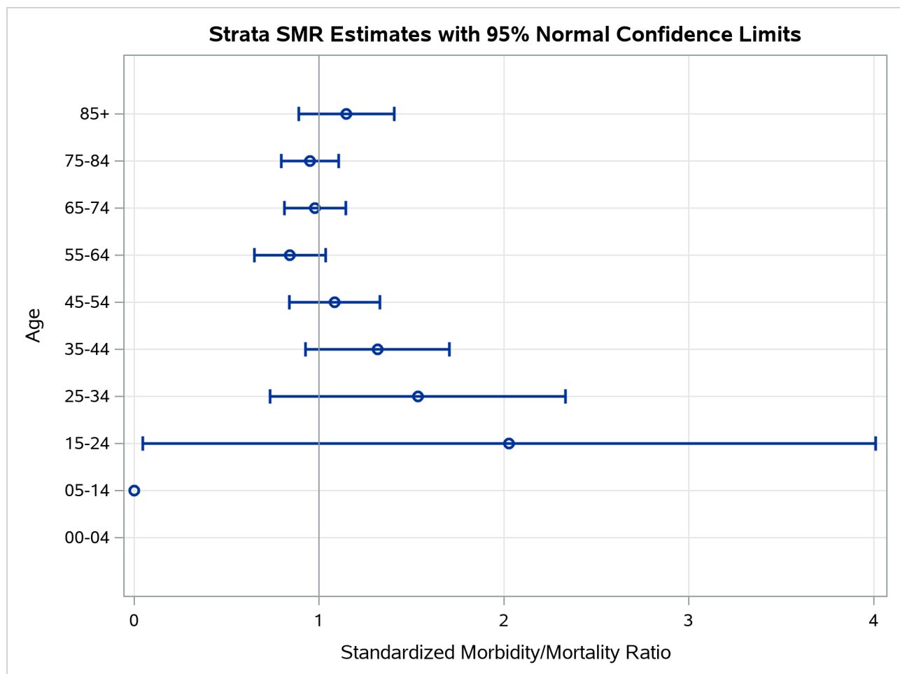
Output 113.4.4 Strata SMR Plot
