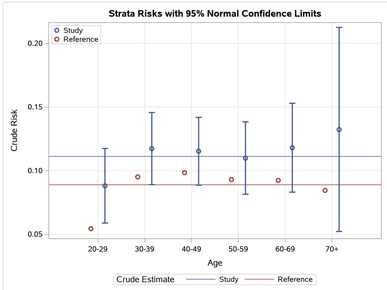
Output 113.3.3 Strata Risk Plot
