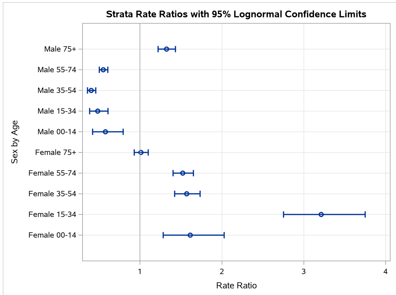
Output 113.1.4 Strata Effect Measure Plot
