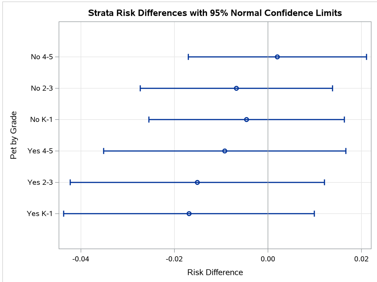
Output 113.2.6 Strata Risk Plot
