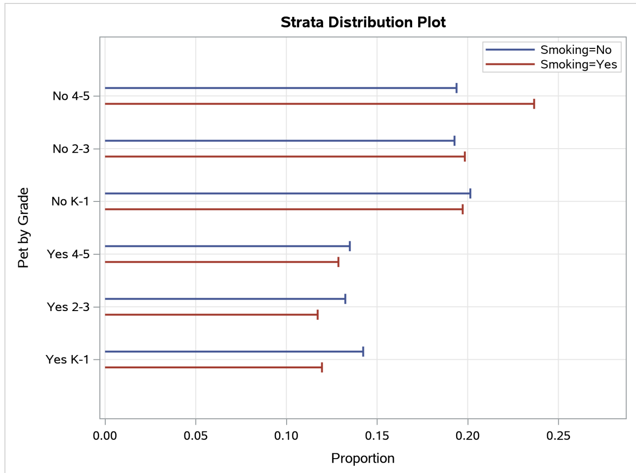
Output 113.2.3 Strata Distribution Plot
