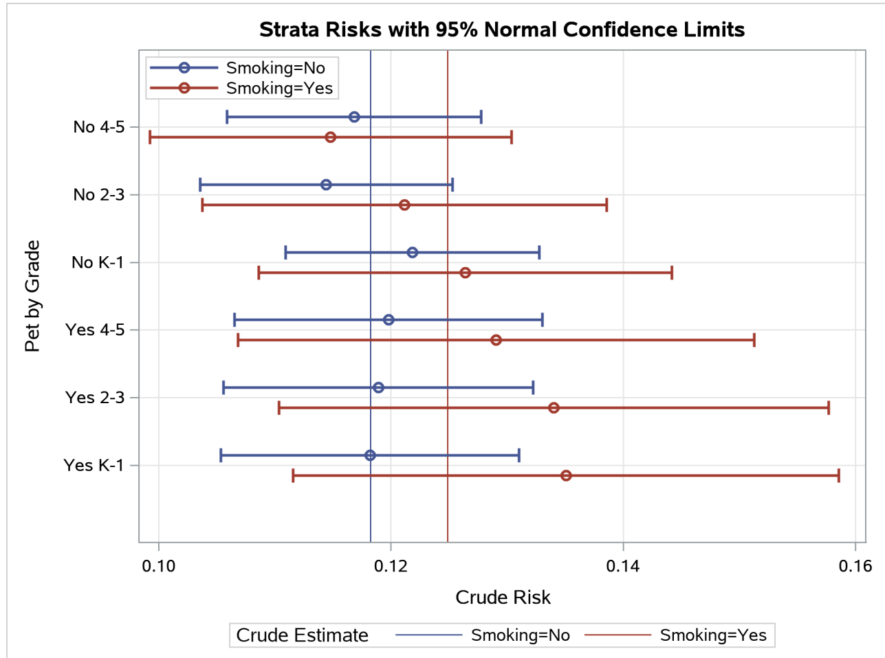
Output 113.2.4 Strata Risk Plot
