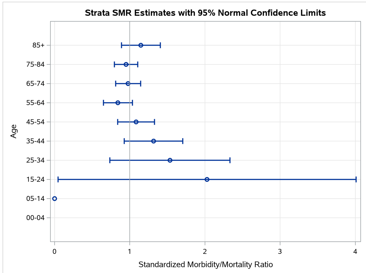
Figure 113.6 Strata SMR Plot
