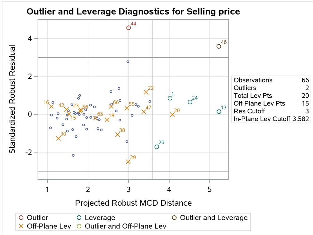
Output 104.5.6 Projected RD Plot
