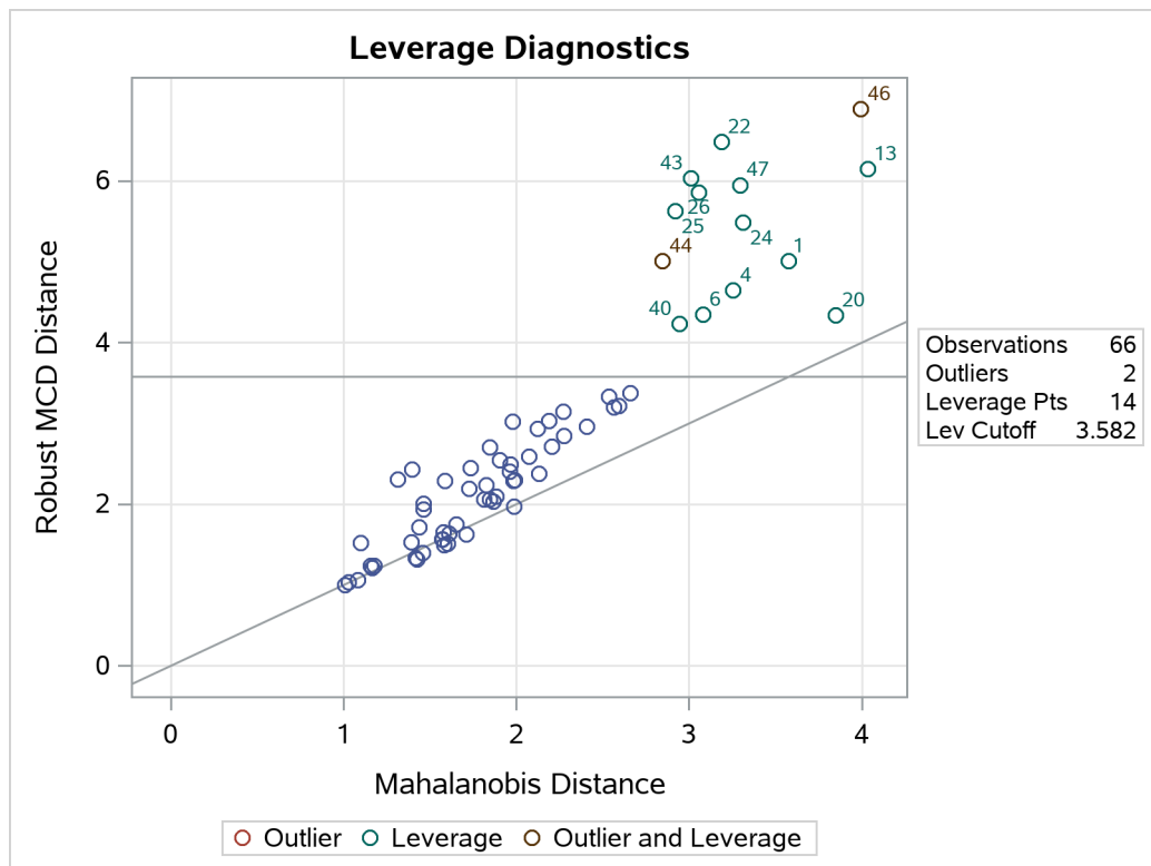
Output 104.5.10 DD Plot for the Reduced Model
