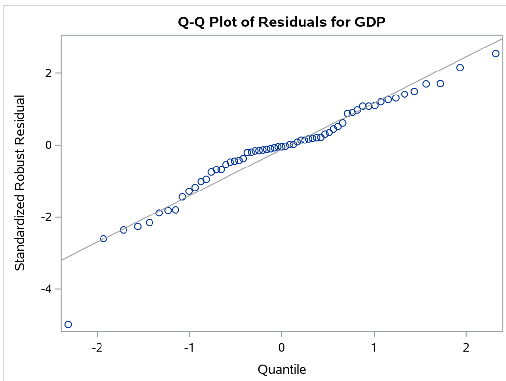
Output 104.3.9 Q-Q Plot
