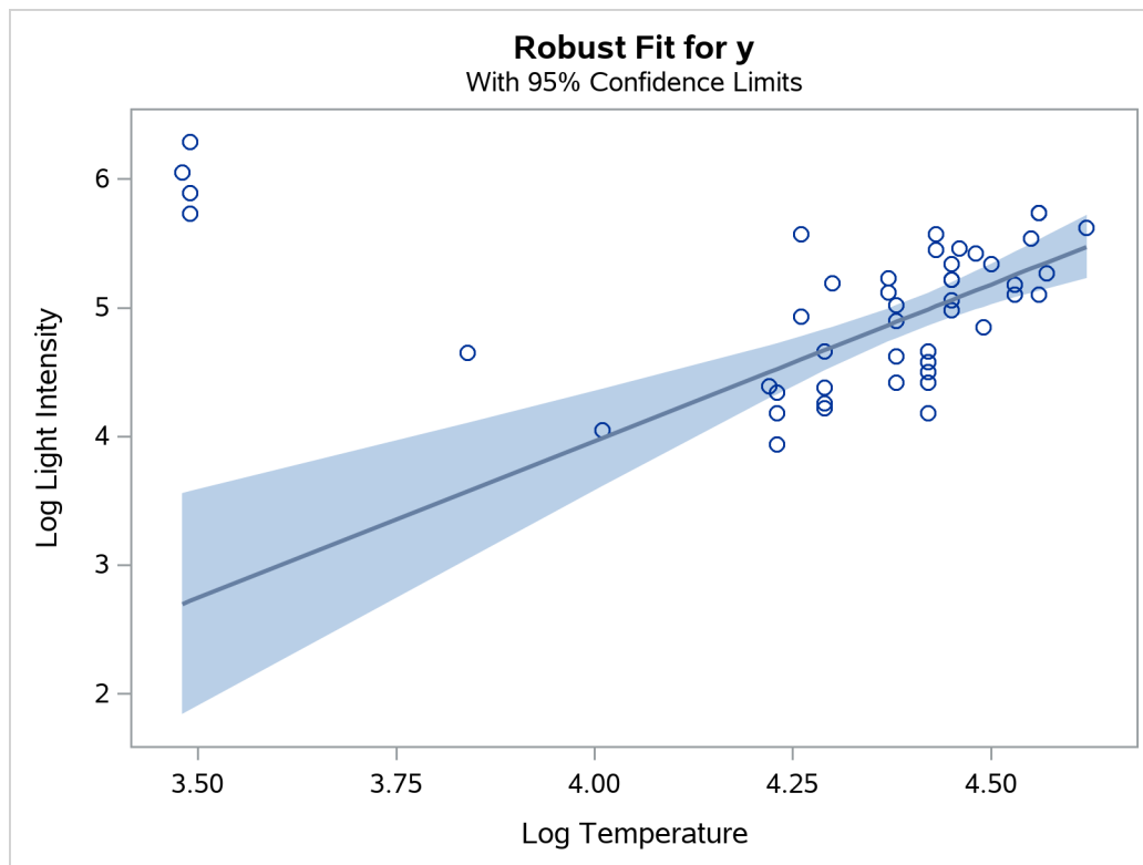
Figure 104.22 Robust Fit
