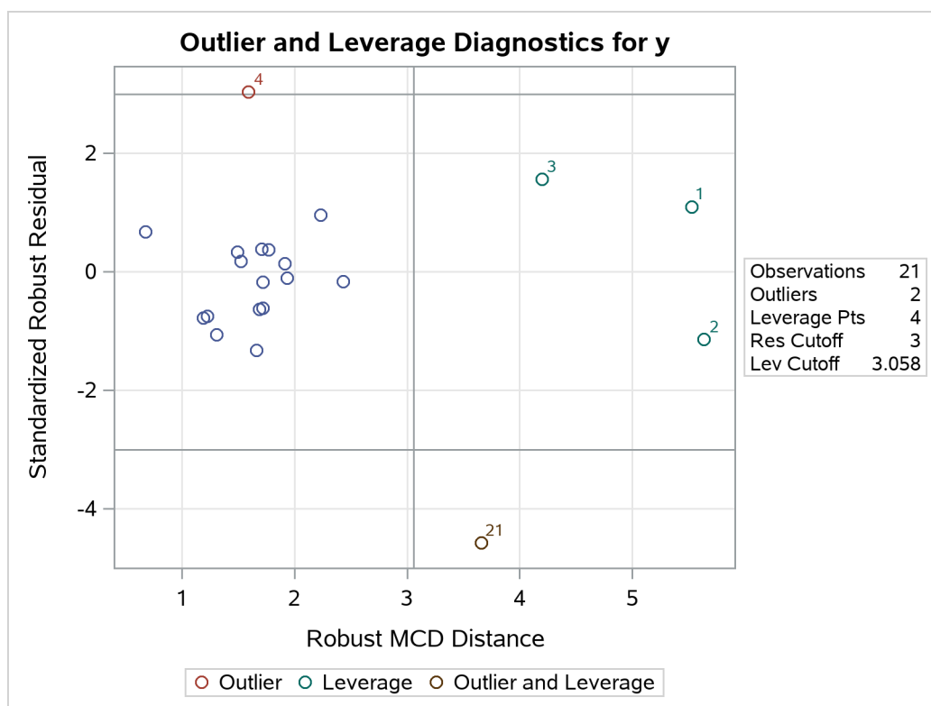
Figure 104.4 RD Plot for Stack Loss Data
