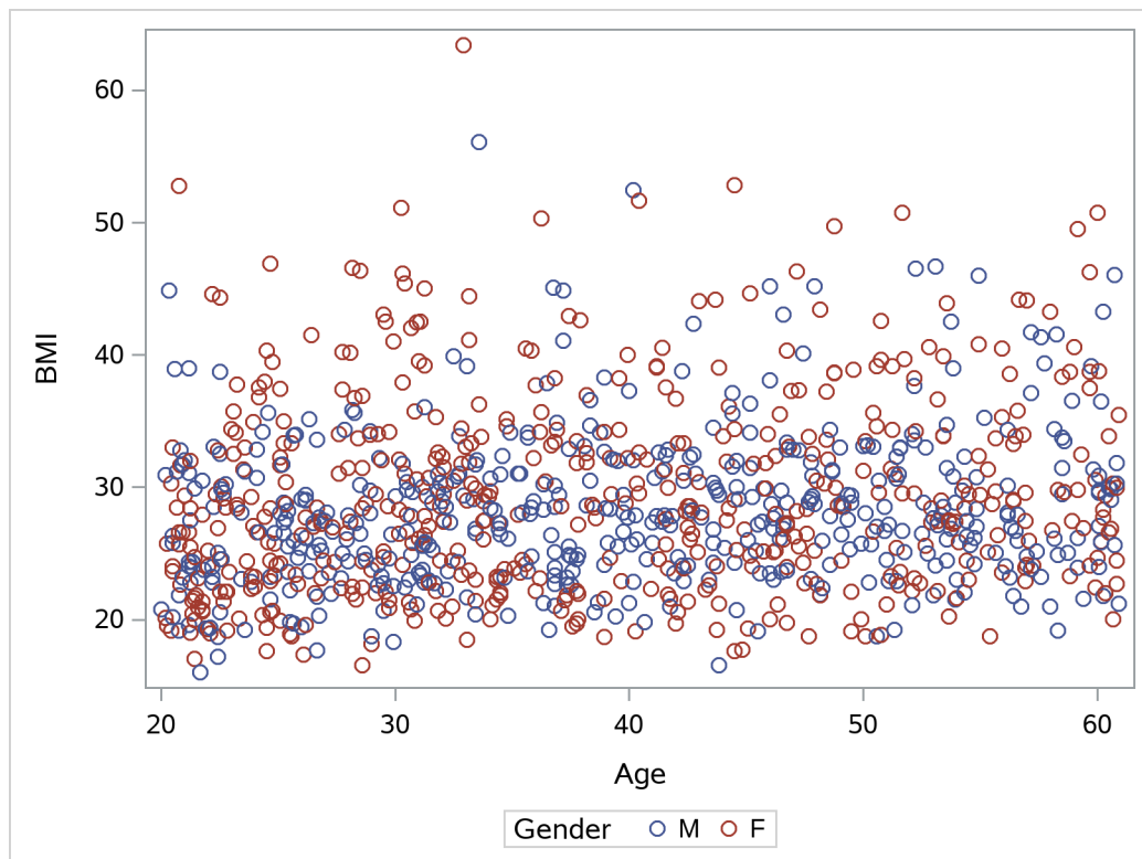
Output 104.4.1 Scatter Plot for BMI Data
