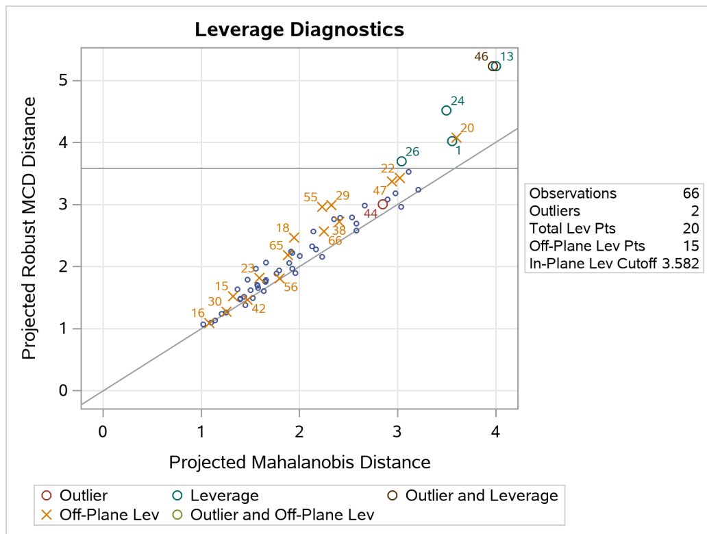
Output 104.5.7 Projected DD Plot
