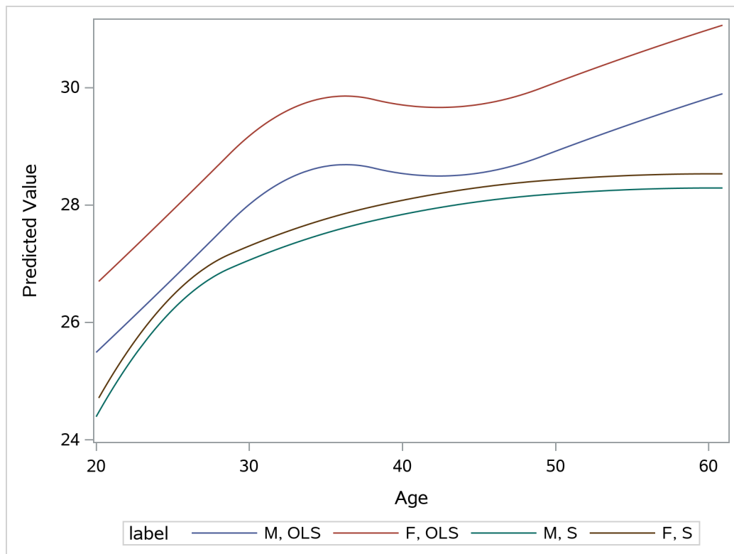
Output 104.4.4 OLS and S Predictions
