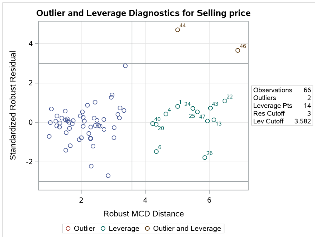
Output 104.5.9 RD Plot for the Reduced Model
