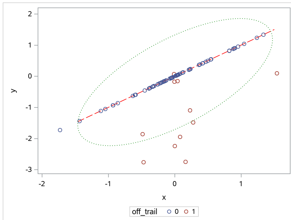
Figure 104.17 Scatter Plot for Children Data
