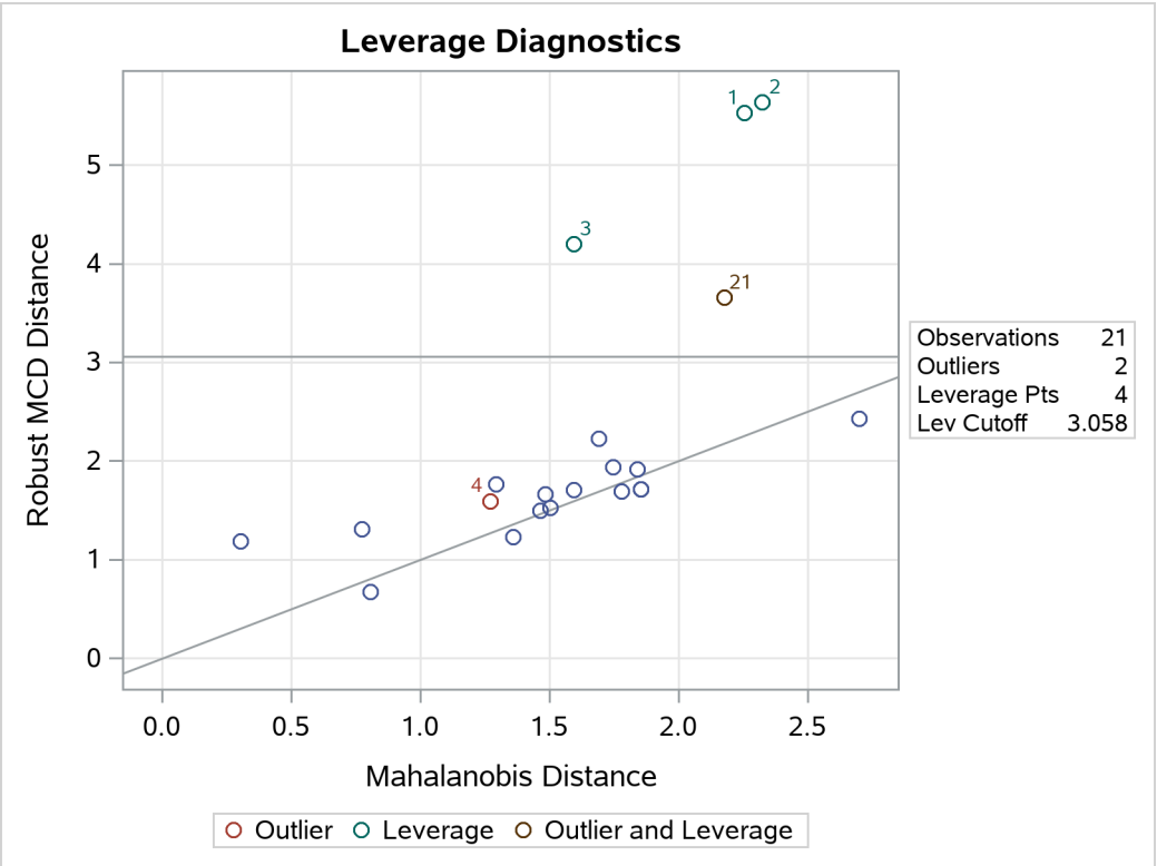
Figure 104.5 DD Plot for Stack Loss Data
