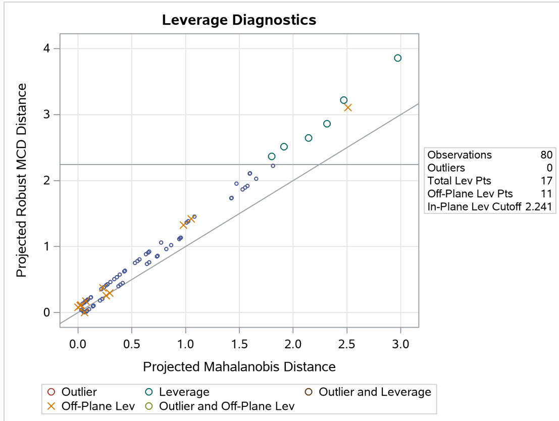
Figure 104.19 DD Plot for Children Data
