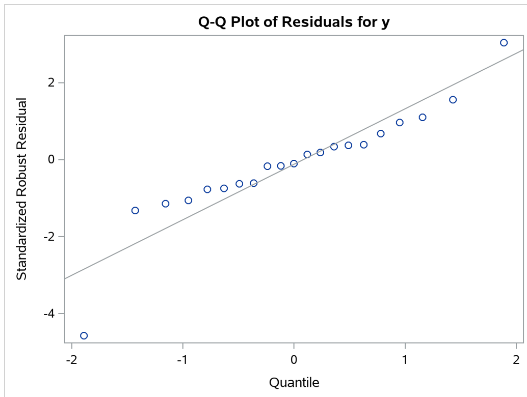
Figure 104.7 Q-Q Plot
