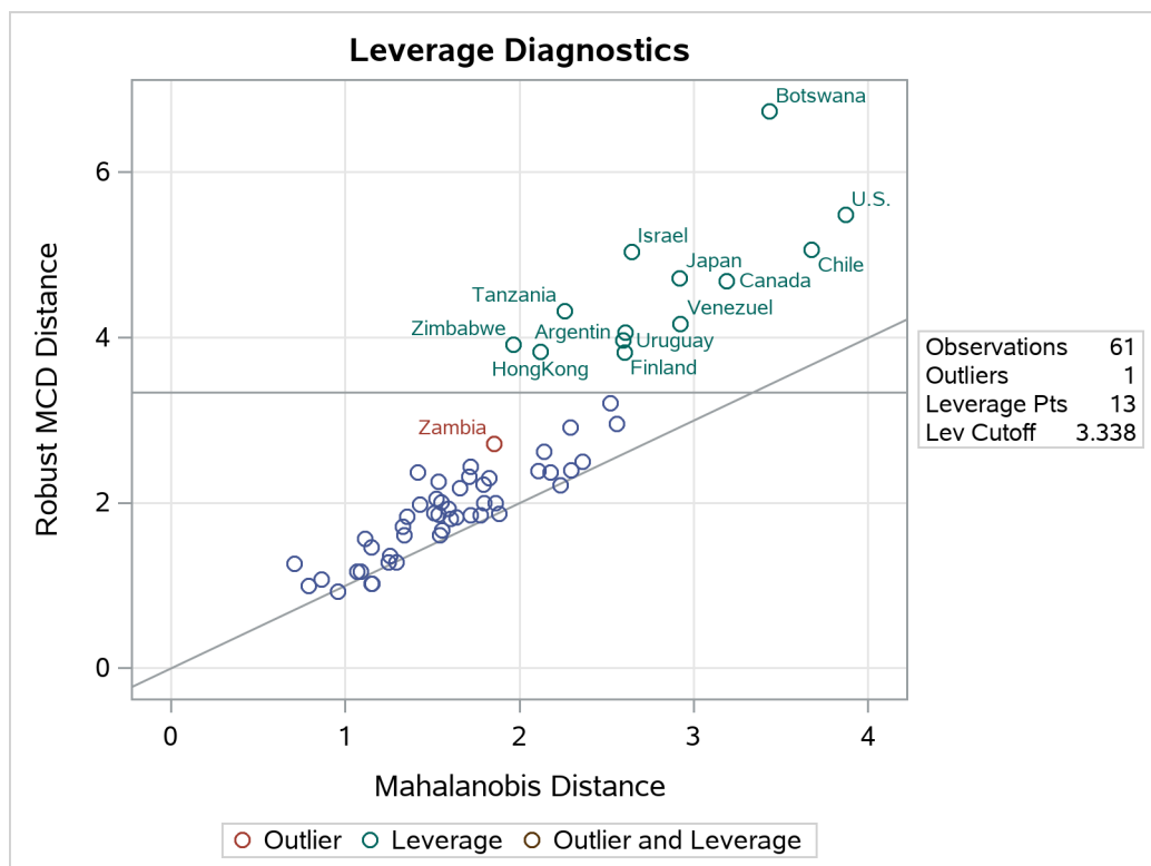
Output 104.3.7 DD Plot for Growth Data
