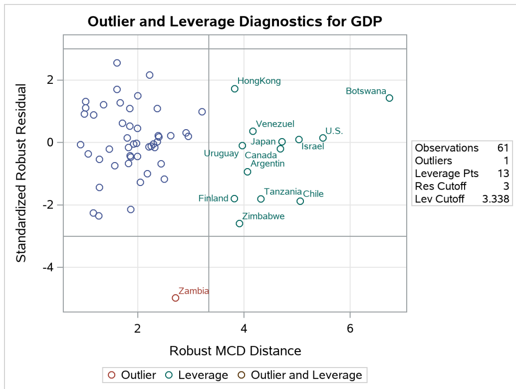
Output 104.3.6 RD Plot for Growth Data
