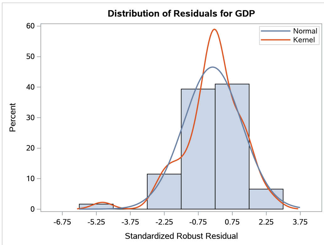
Output 104.3.8 Histogram
