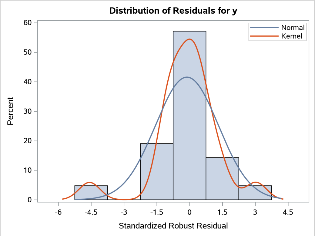
Figure 104.6 Histogram
