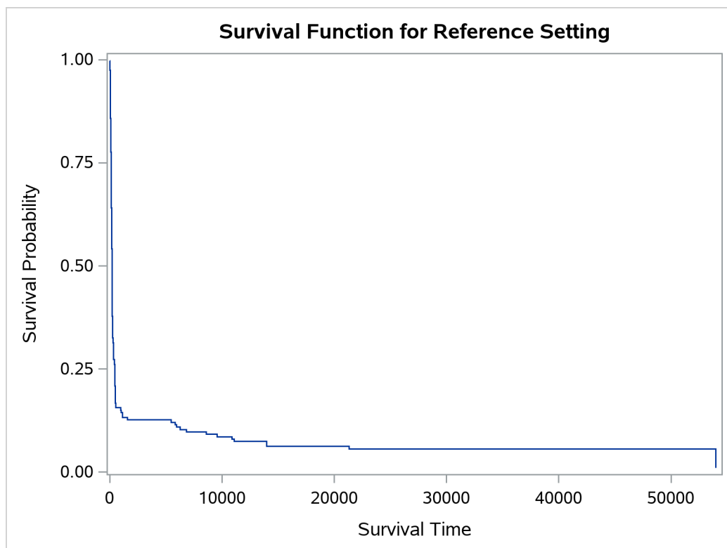
Output 99.2.3 Survival Function
