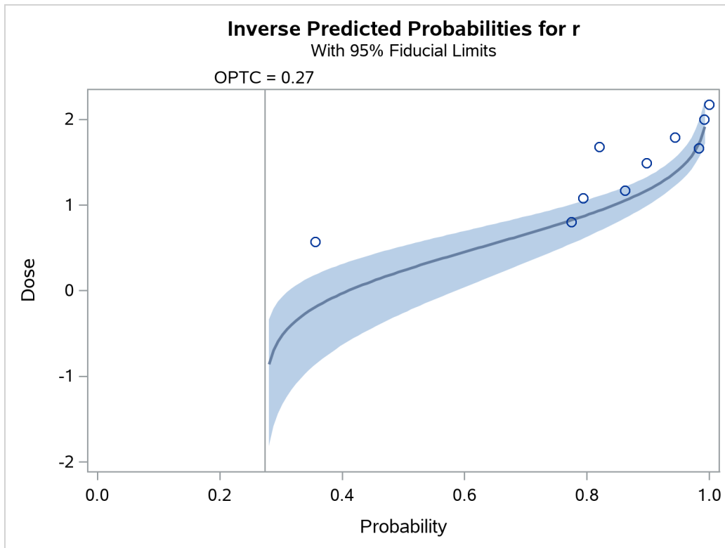
Output 97.4.12 Inverse Predicted Probability Plot
