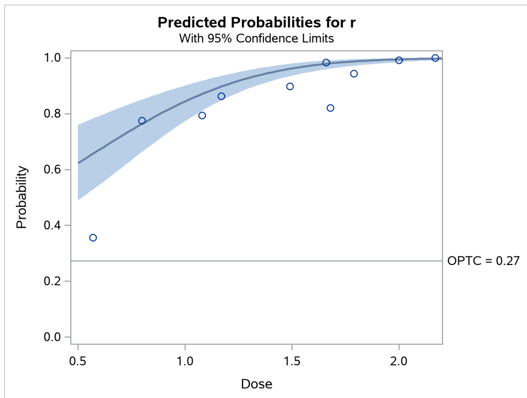
Output 97.4.11 Predicted Probability Plot
