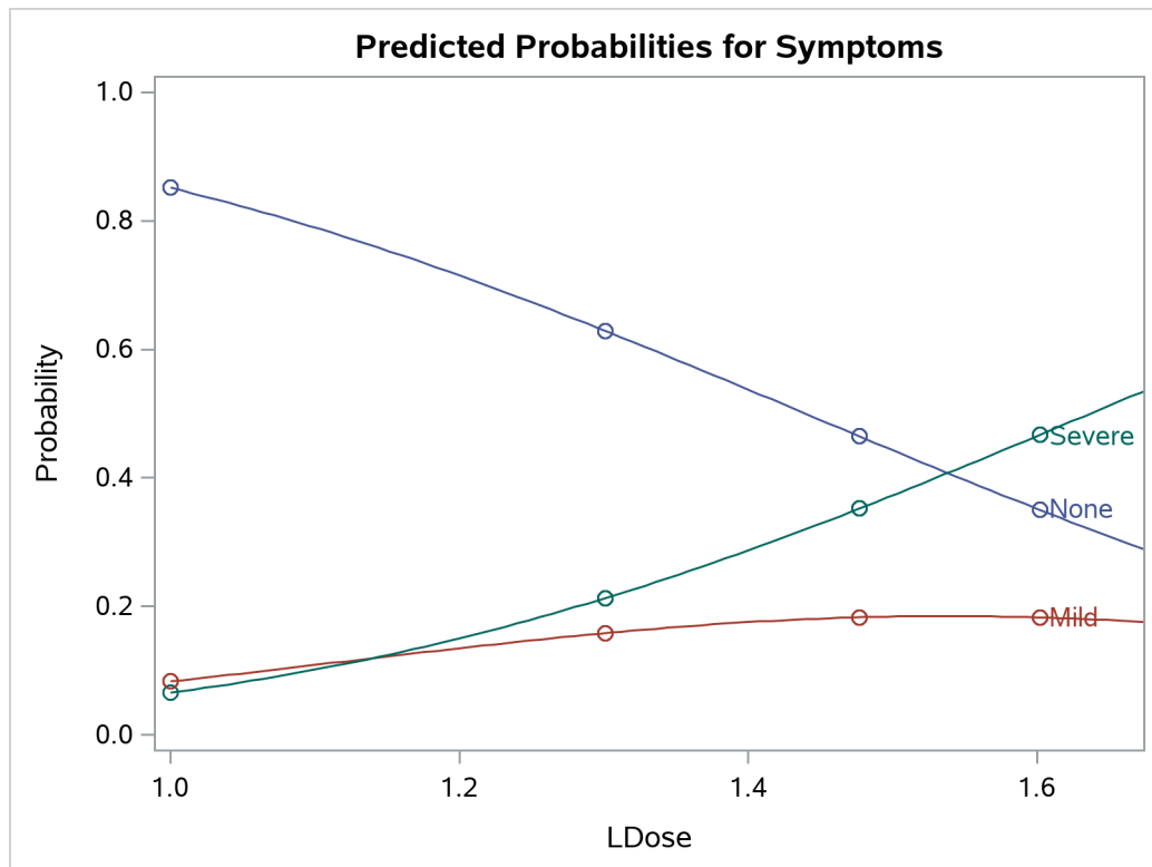
Output 97.2.3 Plot of Predicted Probabilities for the Test Preparation Group
