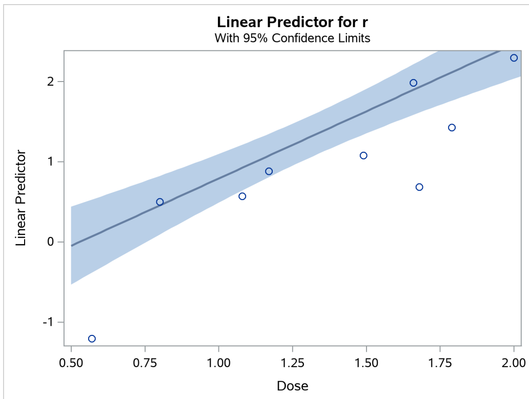
Output 97.4.13 Linear Predictor Plot
