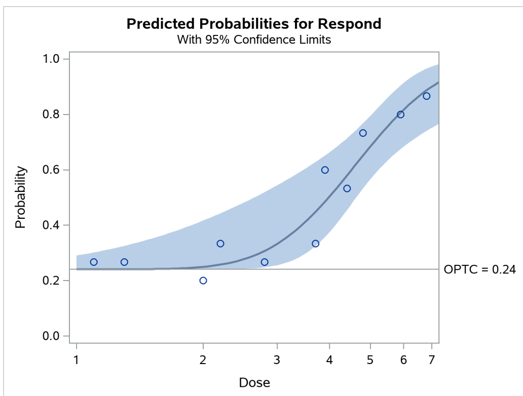
Figure 97.4 Plot of Observed and Fitted Probabilities versus Dose Level
