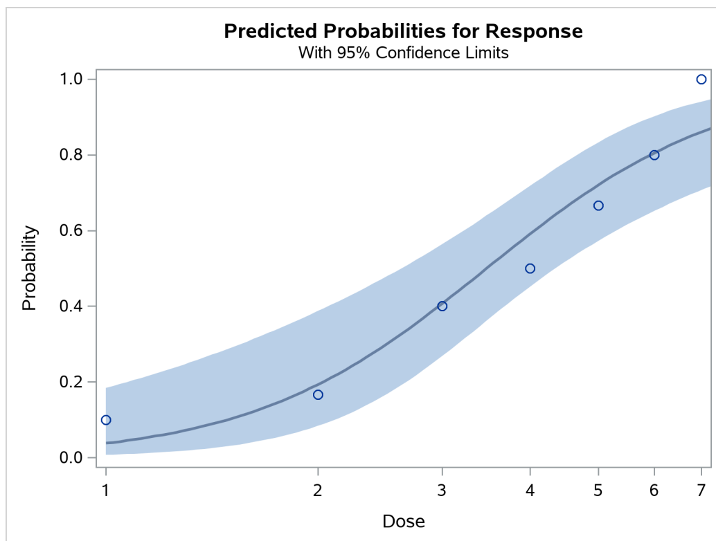
Output 97.1.7 Plot of Observed and Fitted Probabilities
