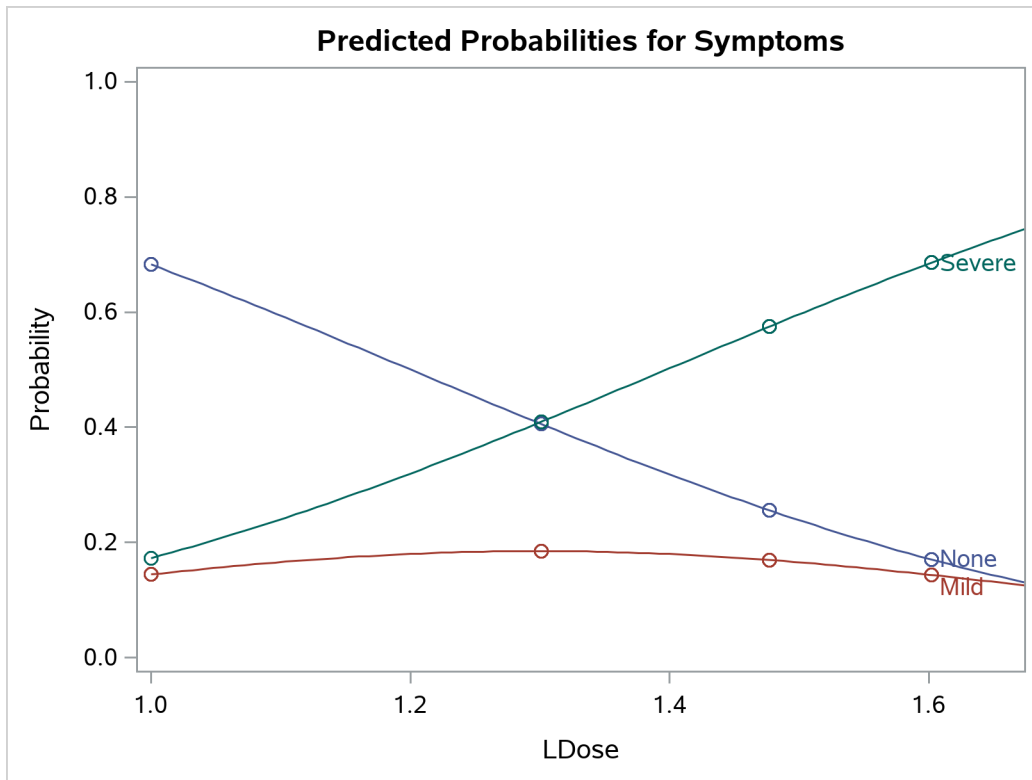
Output 97.2.5 Plot of Predicted Probabilities for the Standard Preparation Group
