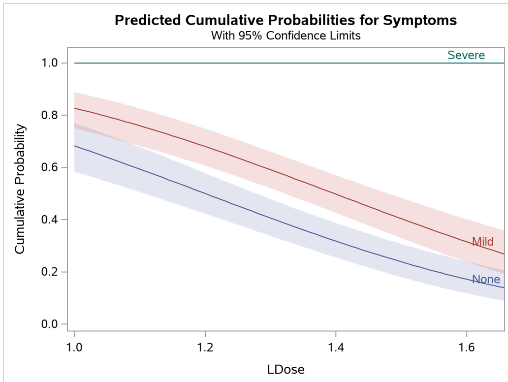
Output 97.2.6 Plot of Predicted Cumulative Probabilities for the Standard Preparation Group
