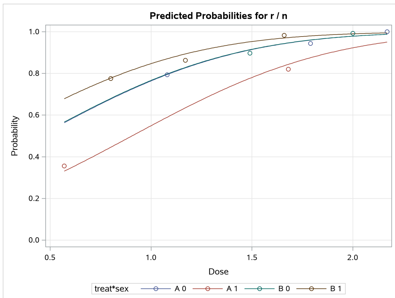
Output 97.5.3 Predicted Probability versus Dose Level by treat*sex
