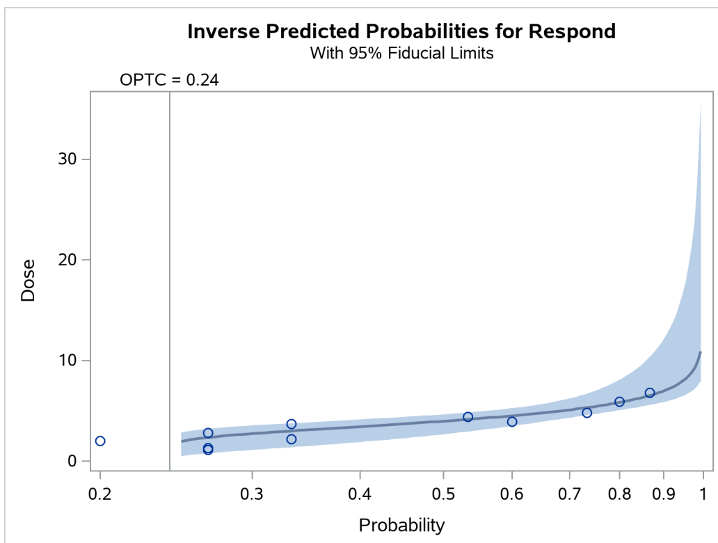
Figure 97.5 Inverse Predicted Probability Plot with Fiducial Limits
