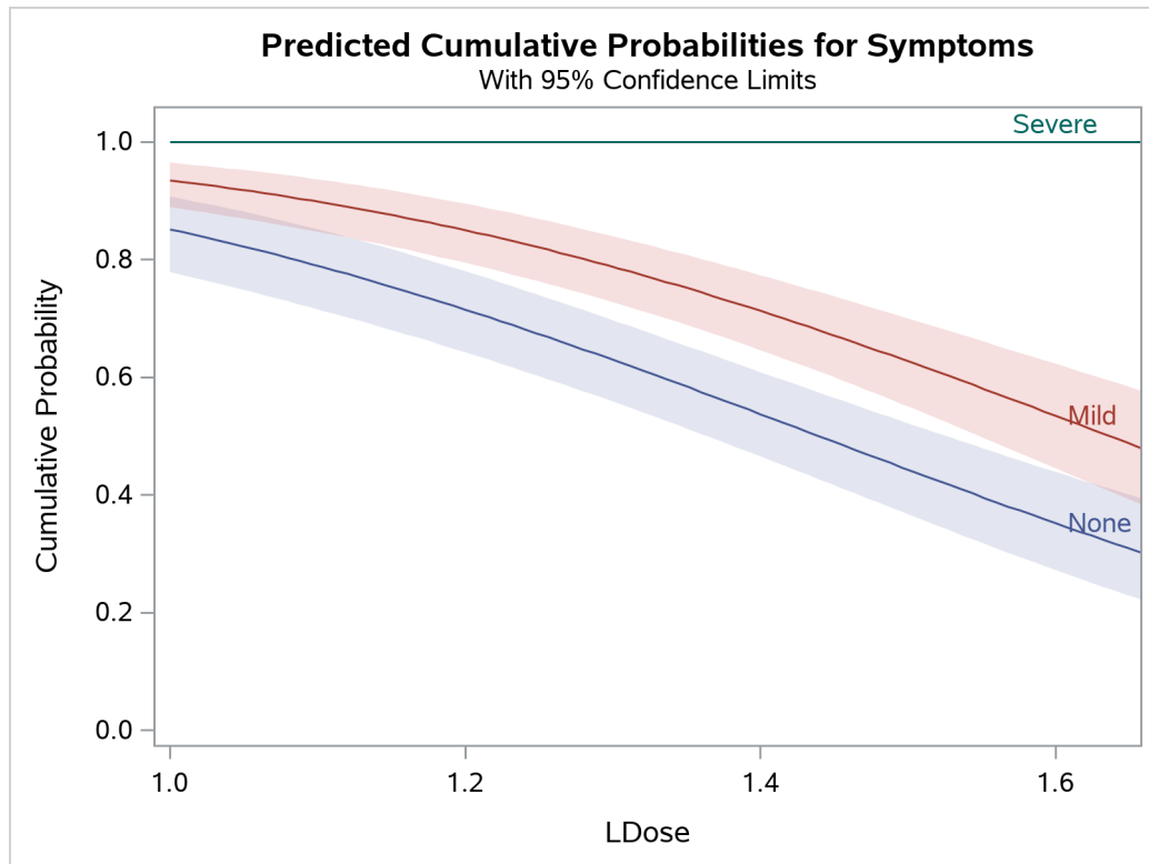
Output 97.2.4 Plot of Predicted Cumulative Probabilities for the Test Preparation Group
