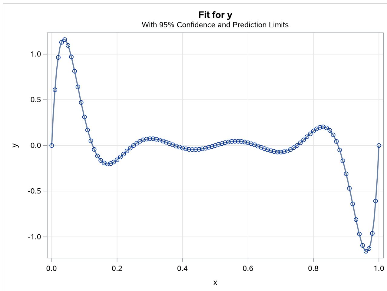
Output 88.3.2 PROC ORTHOREG Fit Plot for Ninth-Degree Polynomial
