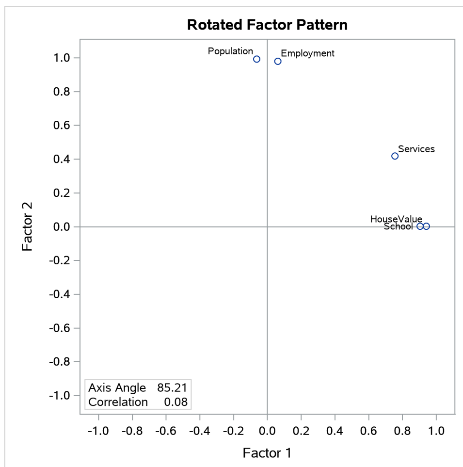
Output 41.2.20 Harris-Kaiser Rotation: Factor Loading Plot
