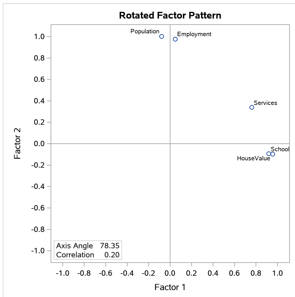
Output 41.2.12 Promax Rotation: Factor Loading Plot
