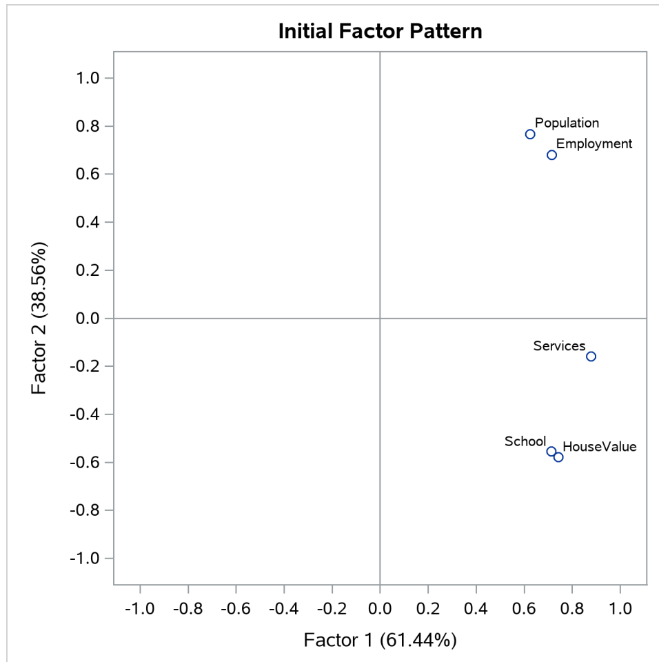
Output 41.2.6 Unrotated Factor Loading Plot
