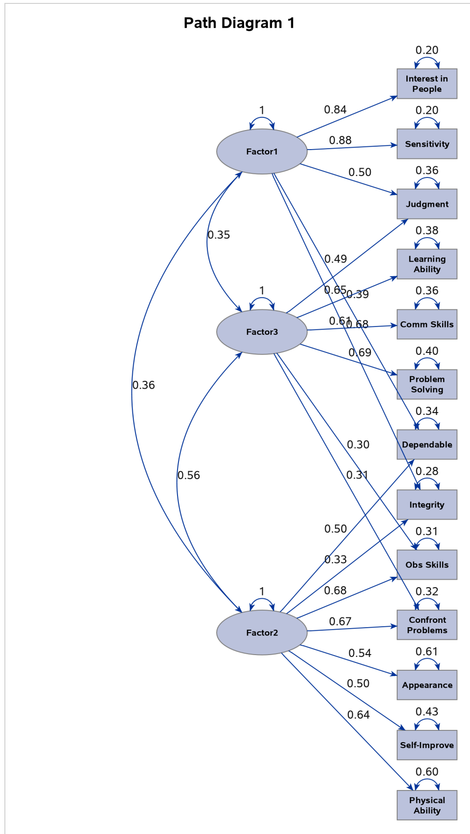
Output 41.6.3 Default Path Diagram for the Quartimin-Rotated Solution
