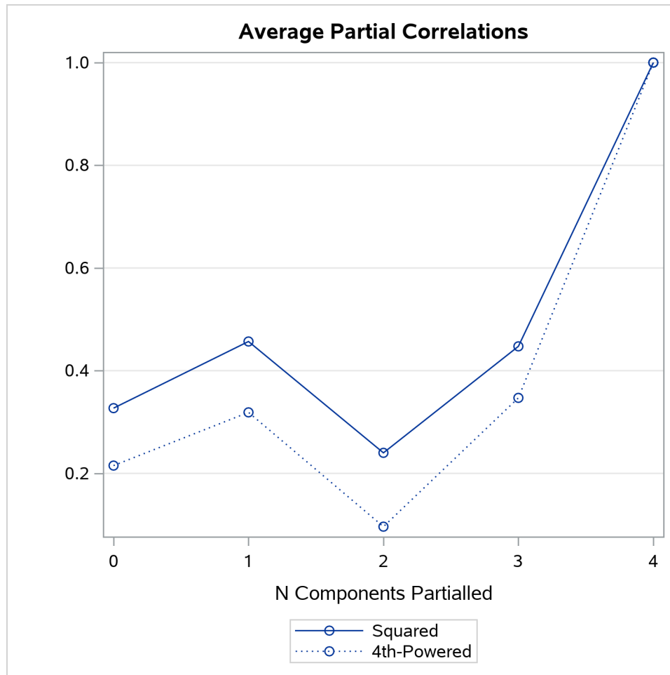
Output 41.3.4 Graphical Summary of the MAP
