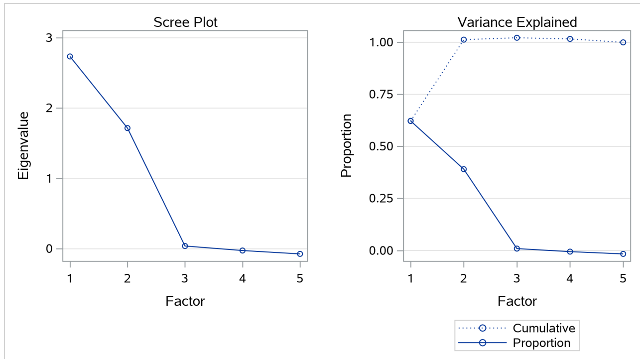
Output 41.2.3 Scree and Variance Explained Plots
