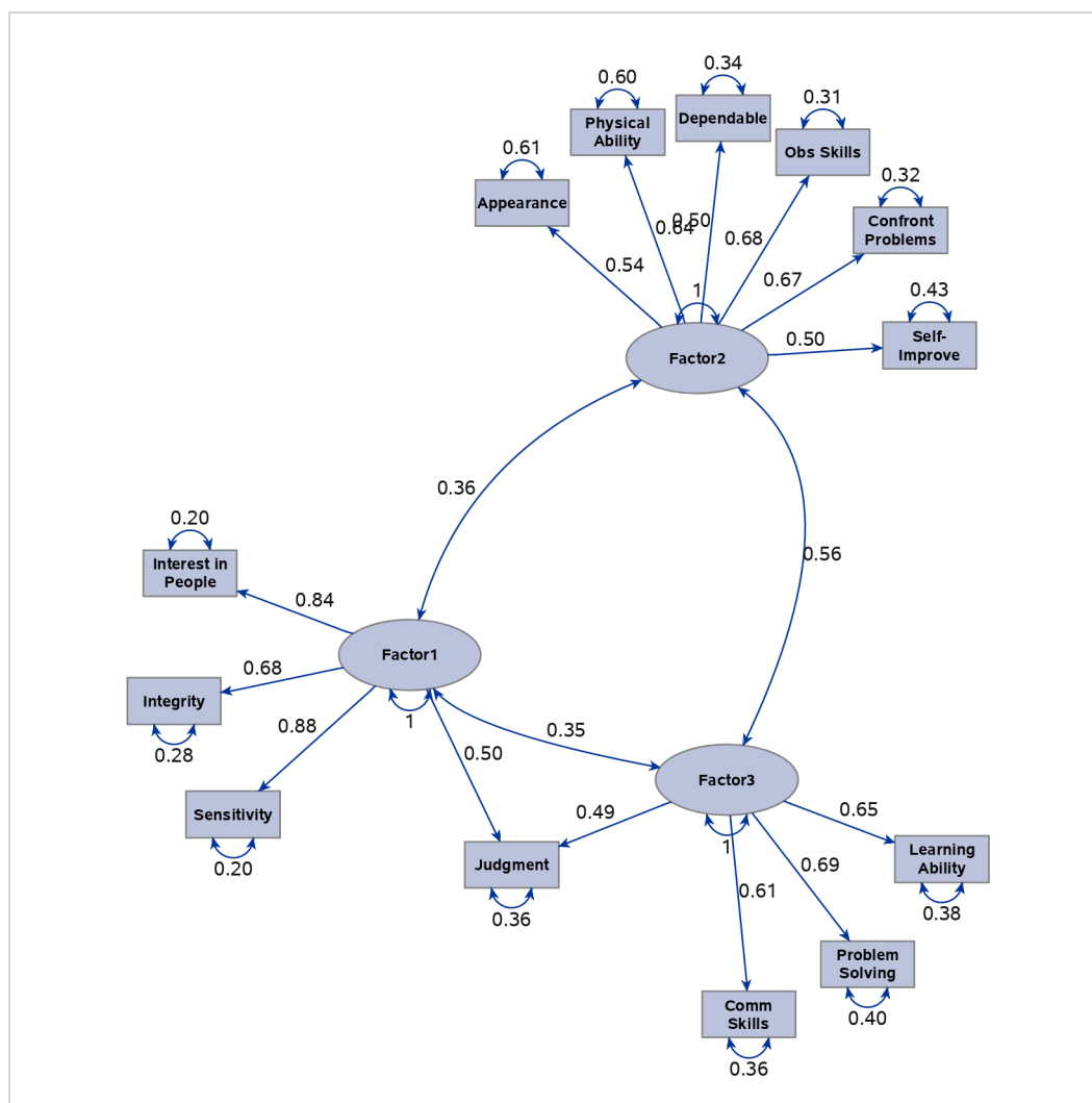
Output 41.6.5 Path Diagram Showing Strong Links by Using the ARRANGE=GRIP Algorithm
