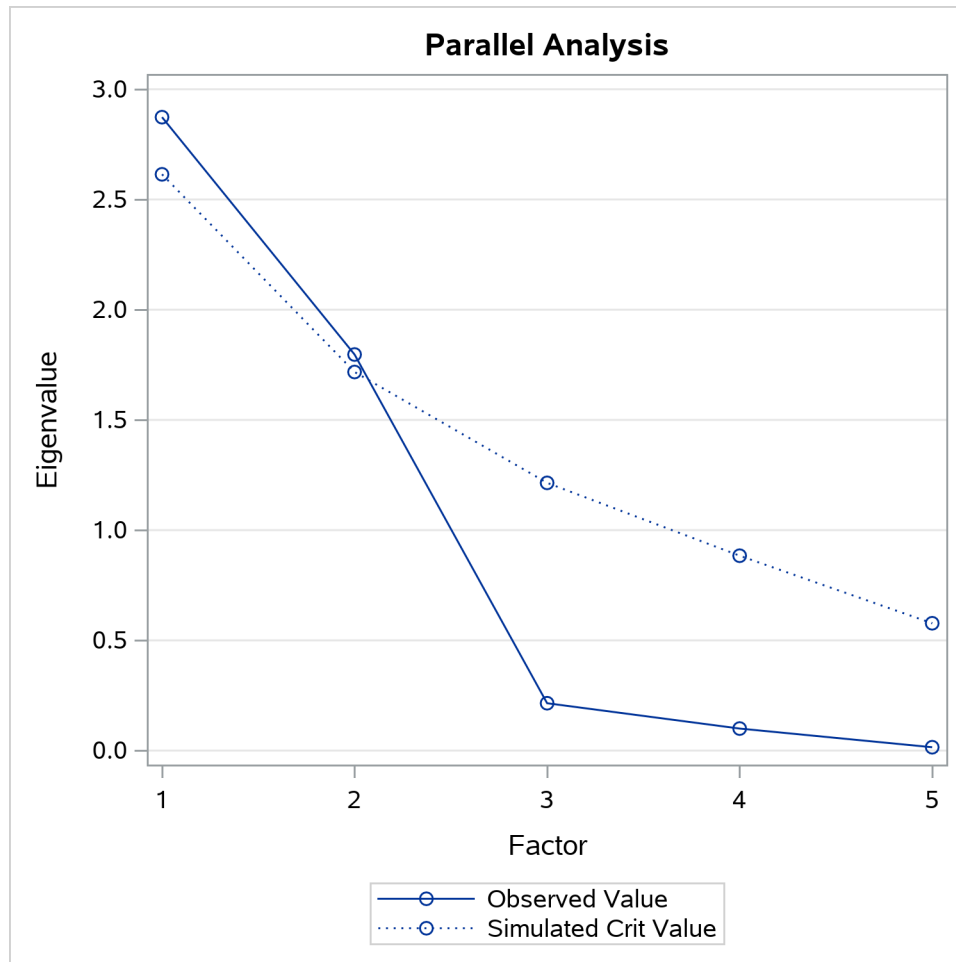
Output 41.3.2 Graphical Summary of the Parallel Analysis
