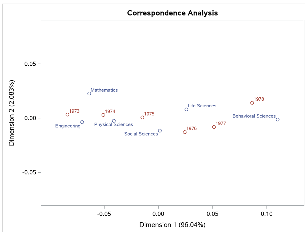
Figure 38.2 Correspondence Analysis of Ph.D. Data
