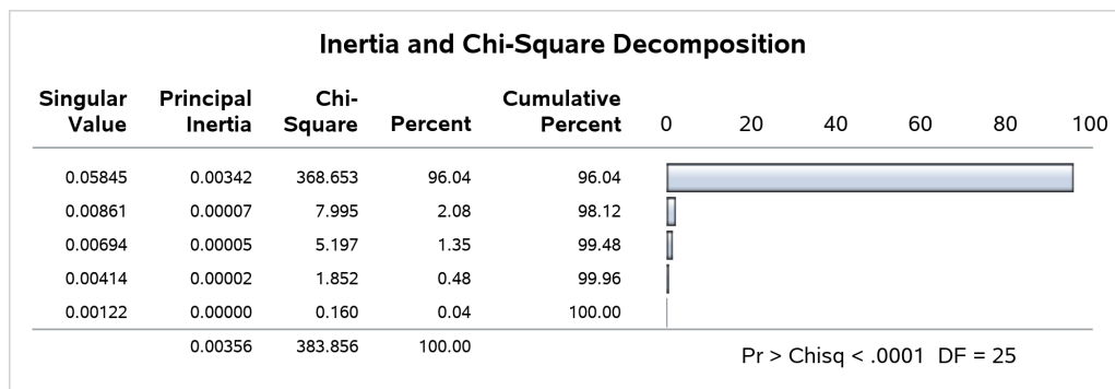
Figure 38.1 Inertia and Chi-Square Decomposition
