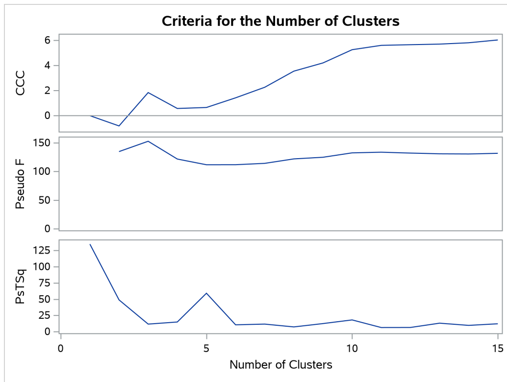
Figure 37.3 Plot of Statistics for Estimating the Number of Clusters
