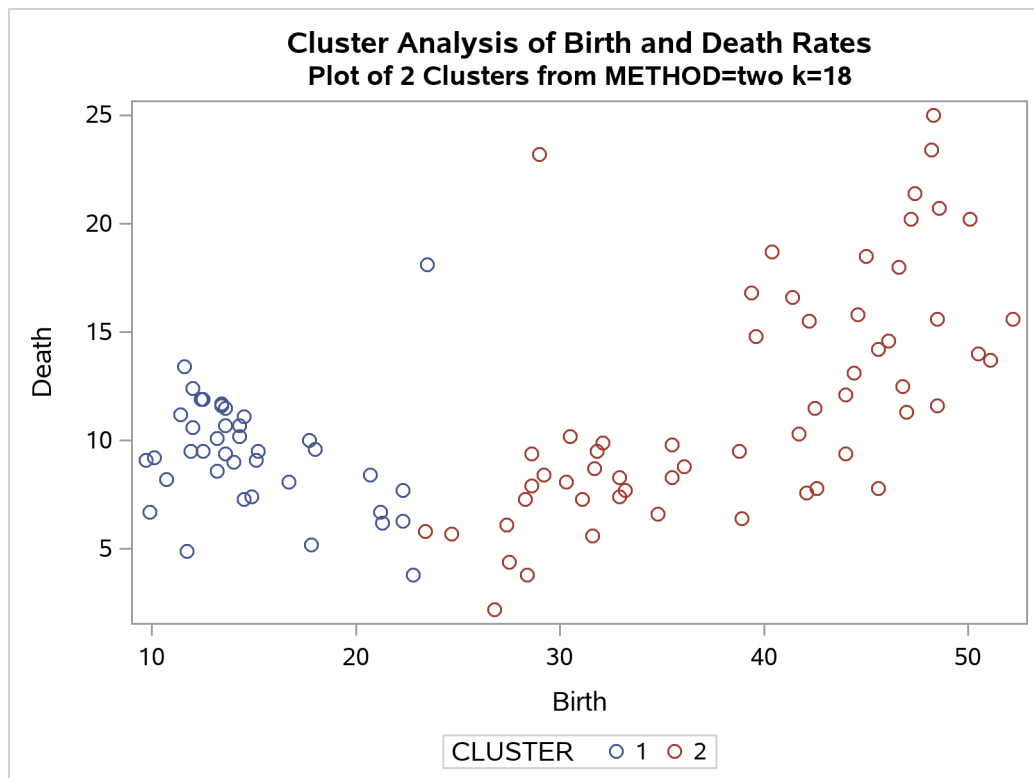
Output 37.2.14 Plot of Clusters for METHOD=TWOSTAGE K=18
