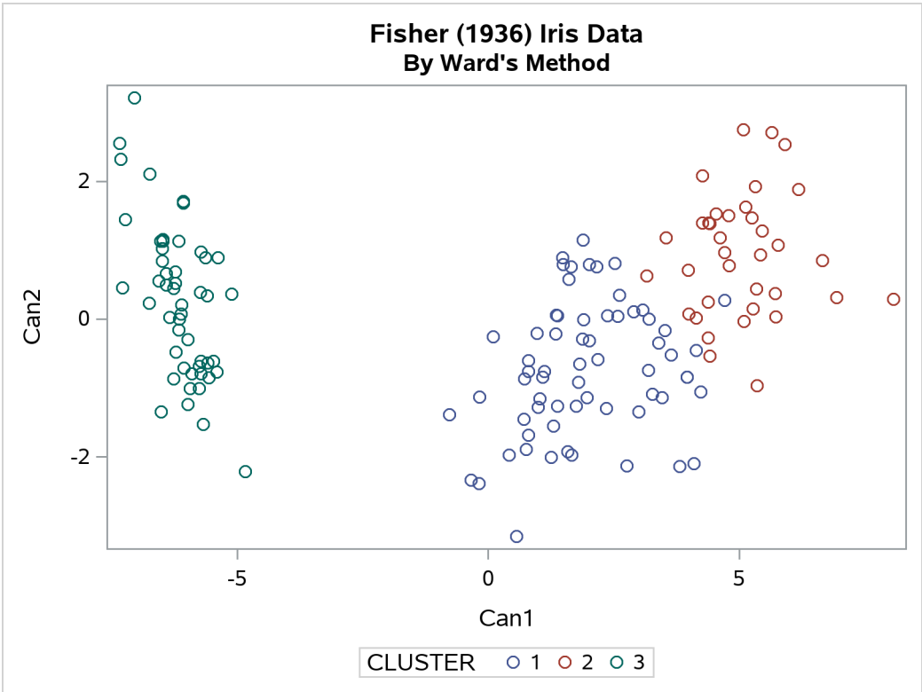
Output 37.3.4 Scatter Plot of Clusters for METHOD=WARD
