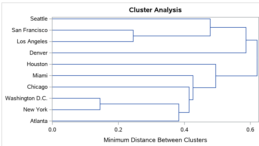
Output 37.1.9 Dendrogram Using METHOD=SINGLE
