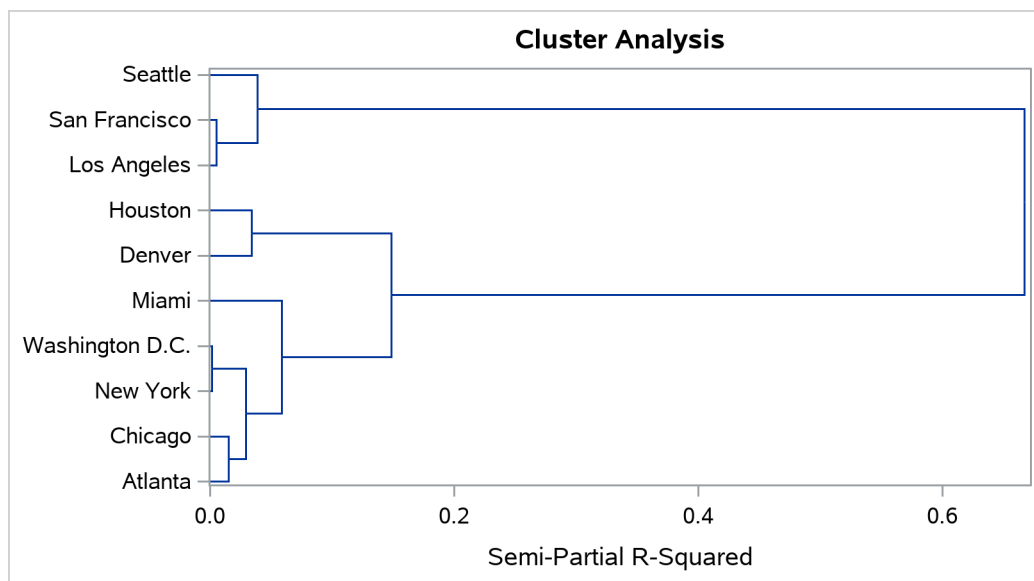
Output 37.1.13 Dendrogram Using METHOD=WARD
