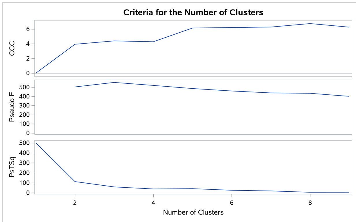
Output 37.3.12 Criteria for the Number of Clusters for Clustering Clusters from Ward's Method
