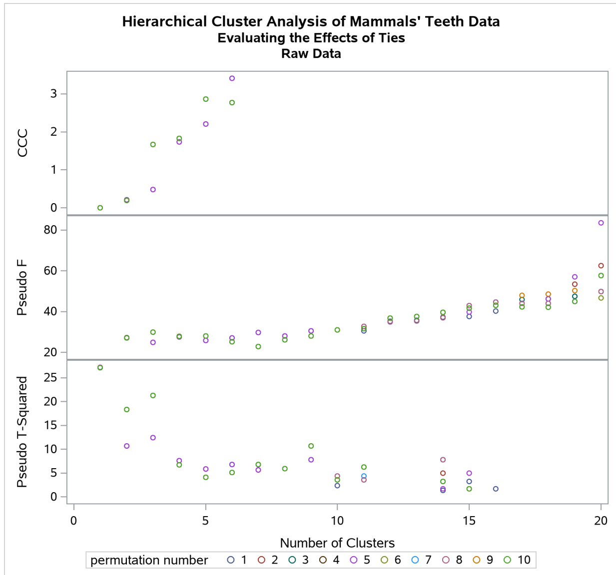
Output 37.4.3 Analysis of 10 Random Permutations of Raw Mammals' Teeth Data
