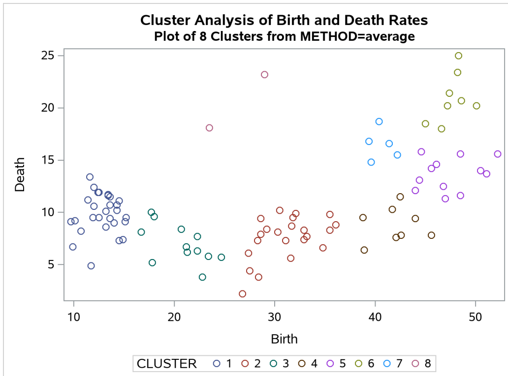
Output 37.2.4 Plot of Eight Clusters: METHOD=AVERAGE
