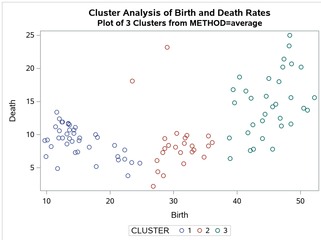
Output 37.2.3 Plot of Three Clusters: METHOD=AVERAGE
