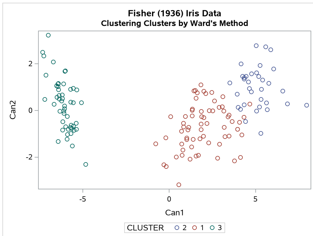
Output 37.3.14 Scatter Plot for Clustering Clusters using Ward's Method
