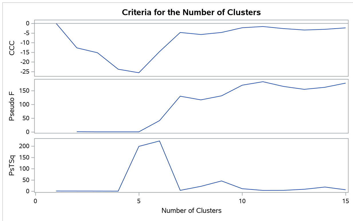
Output 37.2.9 Criteria for the Number of Clusters: METHOD=SINGLE
