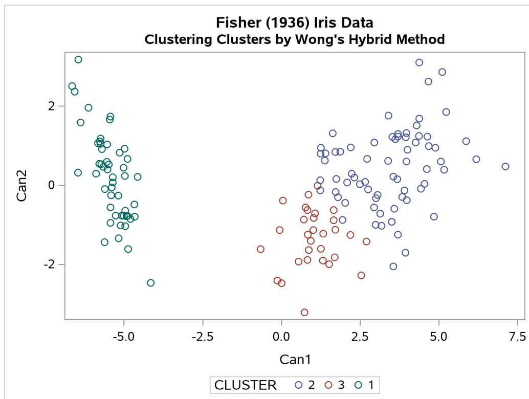
Output 37.3.17 Scatter Plot for Clustering Clusters using Wong's Hybrid Method
