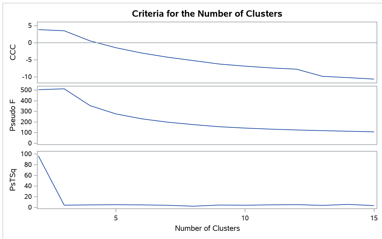
Output 37.3.6 Criteria for the Number of Clusters with METHOD=TWOSTAGE
