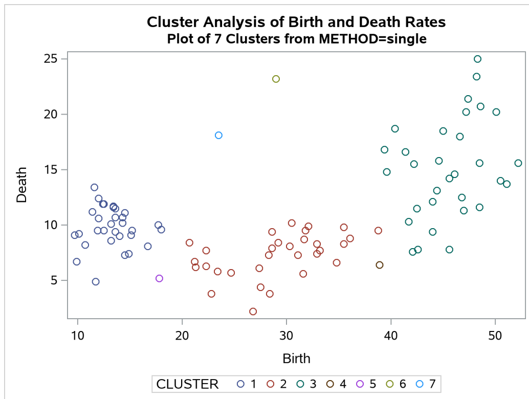
Output 37.2.10 Plot of Clusters for METHOD=SINGLE
