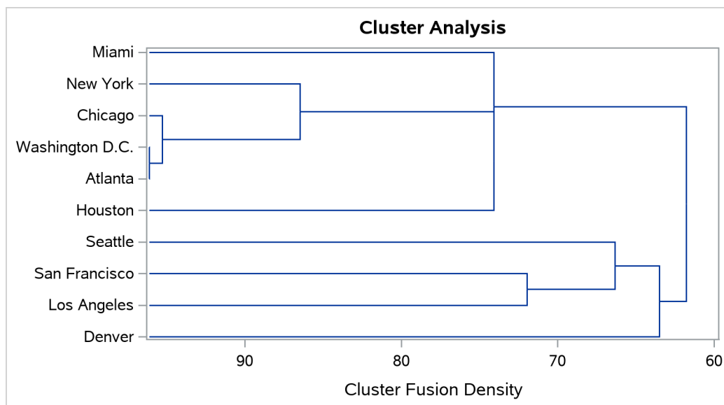
Output 37.1.7 Dendrogram Using METHOD=DENSITY K=3
