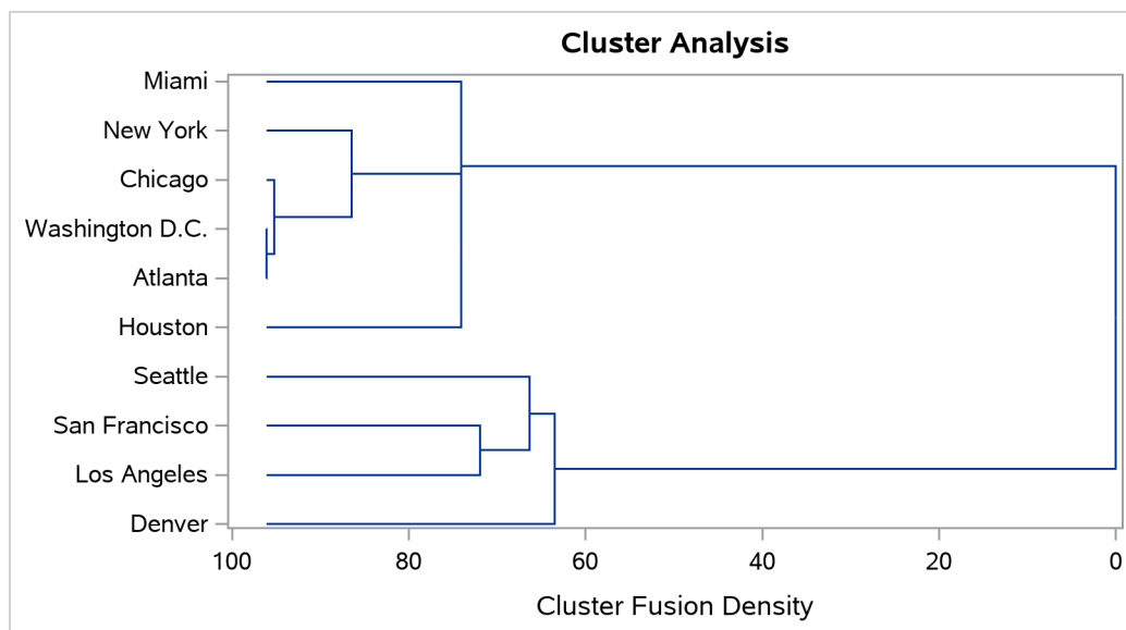
Output 37.1.11 Dendrogram Using METHOD=TWOSTAGE K=3
