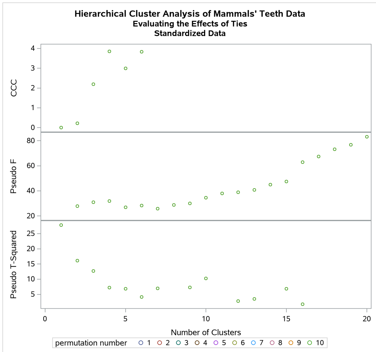
Output 37.4.5 Analysis of 10 Random Permutations of Standardized Mammals' Teeth Data
