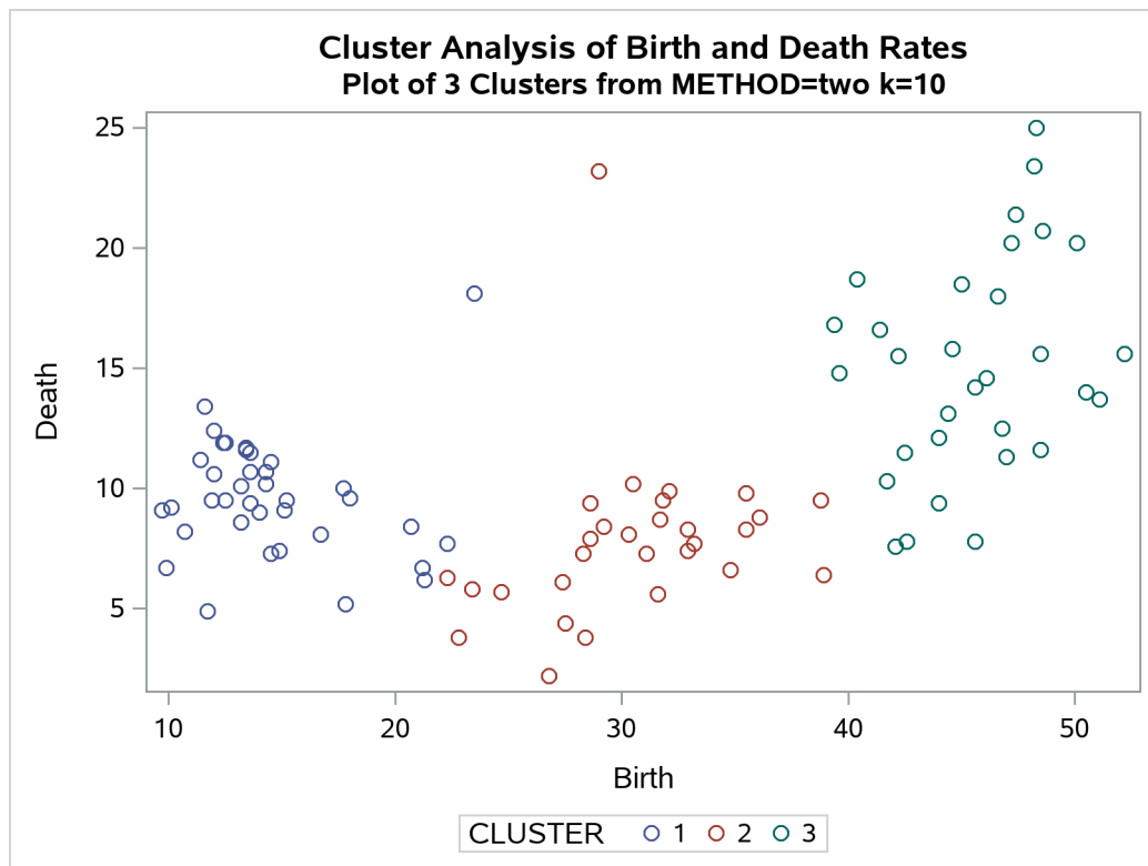
Output 37.2.13 Plot of Clusters for METHOD=TWOSTAGE K=10
