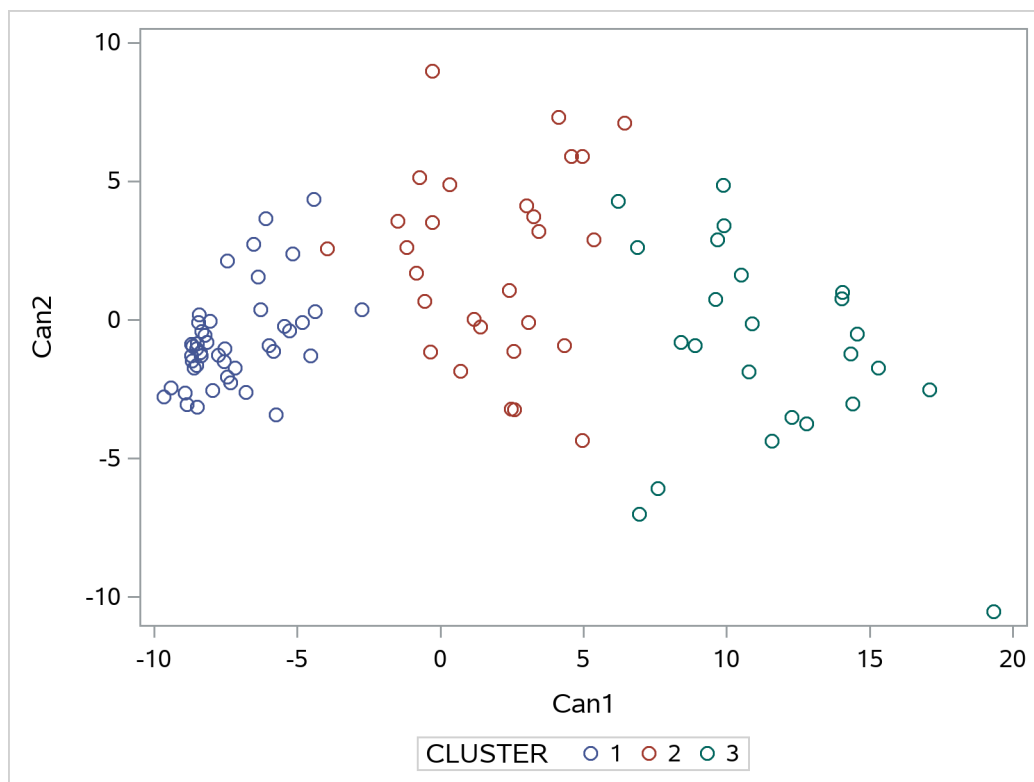
Figure 37.5 Plot of Canonical Variables and Cluster for Three Clusters
