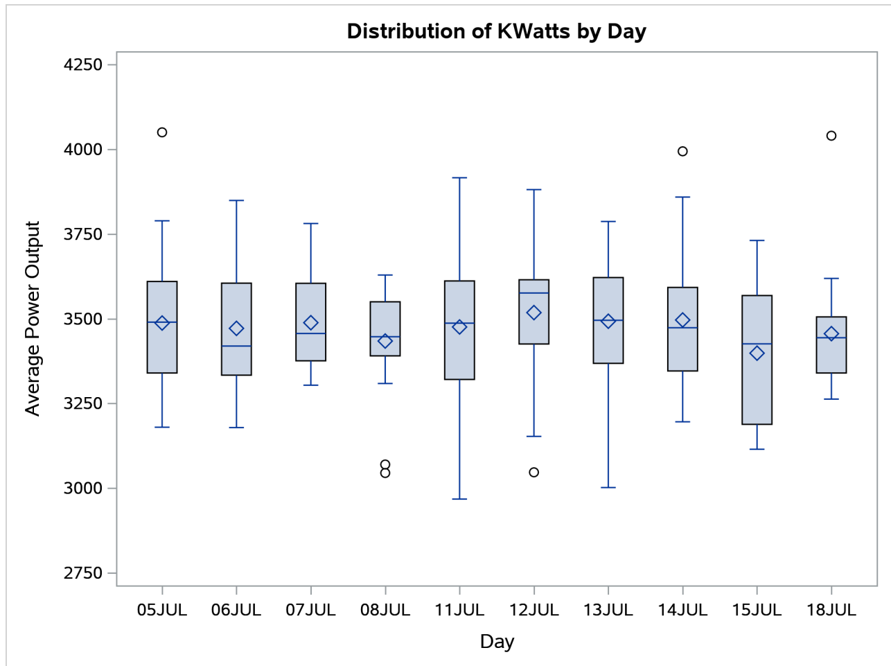
Figure 29.4 Schematic Box Plot of Power Output
