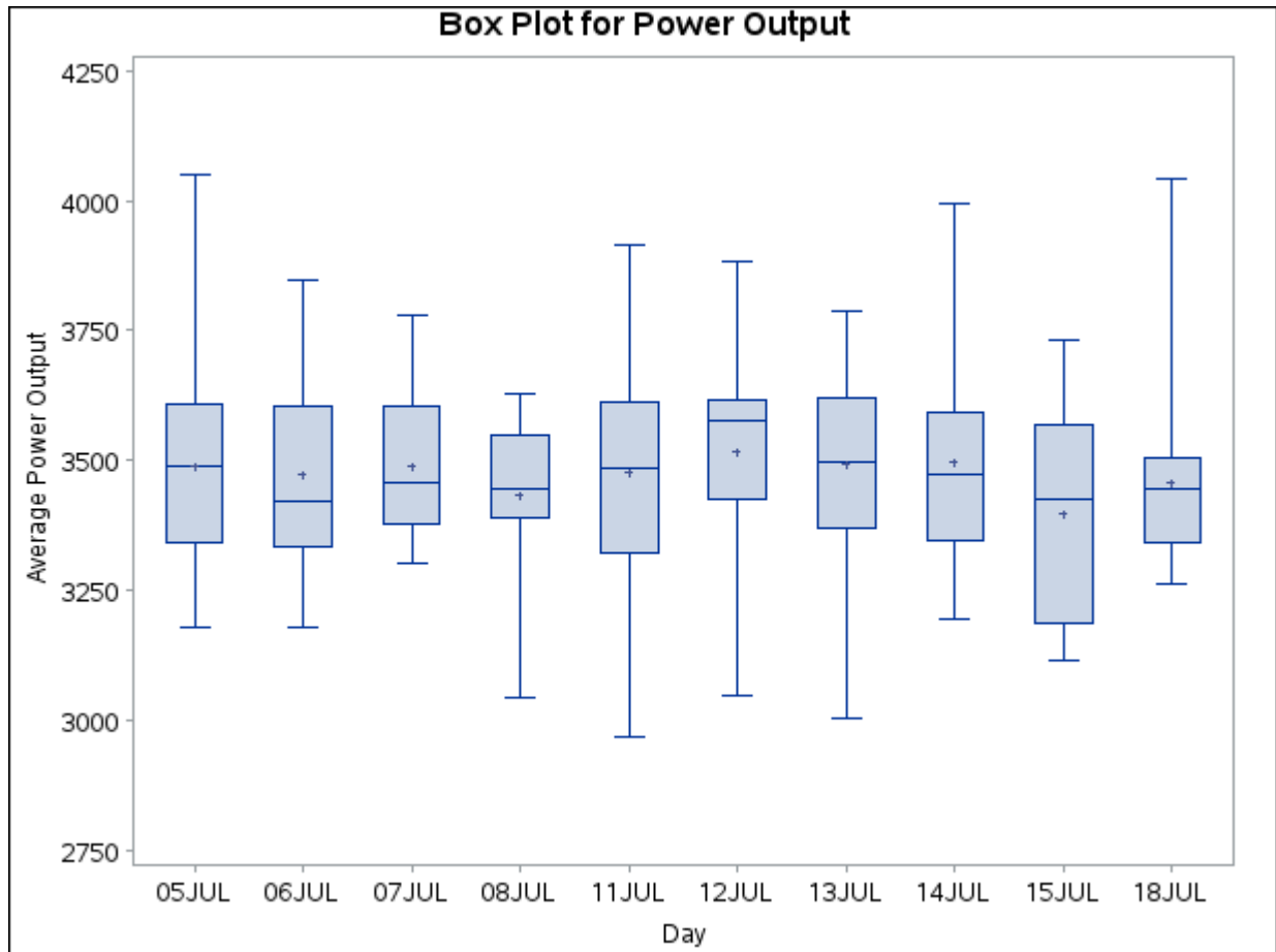
Figure 29.1 Box Plot for Power Output Data
