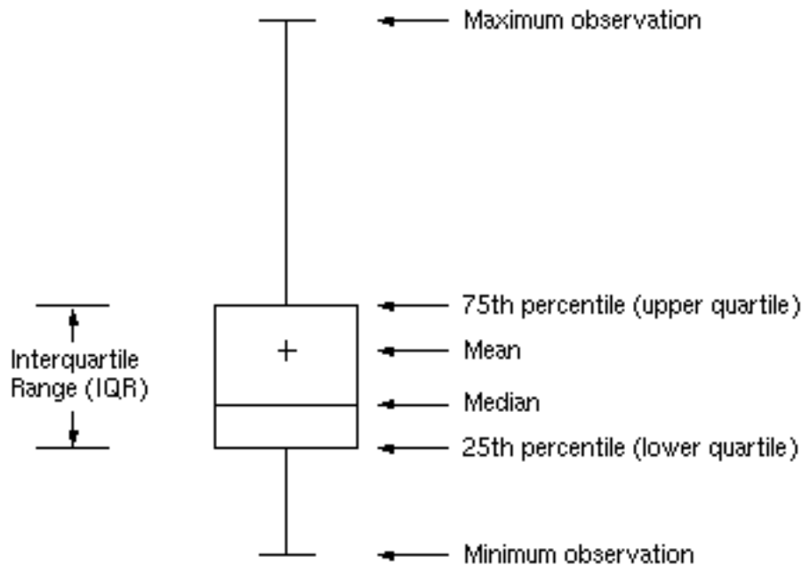
Figure 29.6 Skeletal Box-and-Whiskers Plot
