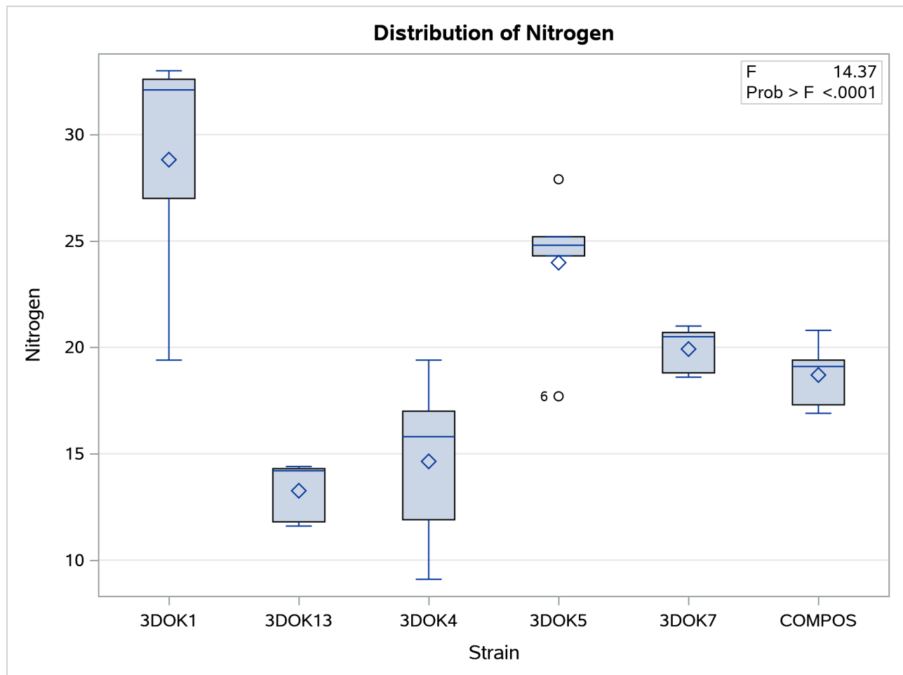
Figure 26.3 Box Plot of Nitrogen Content for Each Treatment
