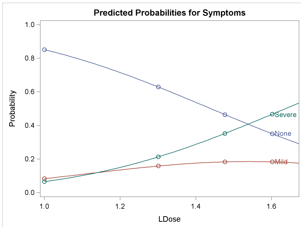
Output 95.2.3 Plot of Predicted Probabilities for the Test Preparation Group
