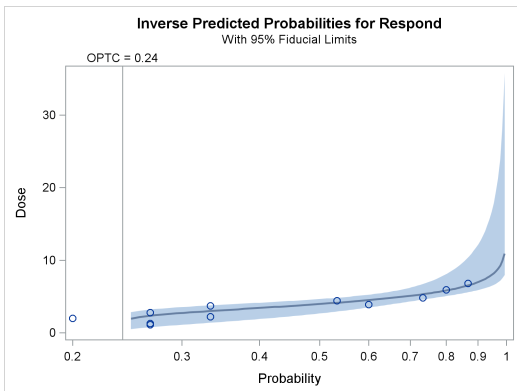
Figure 95.5 Inverse Predicted Probability Plot with Fiducial Limits
