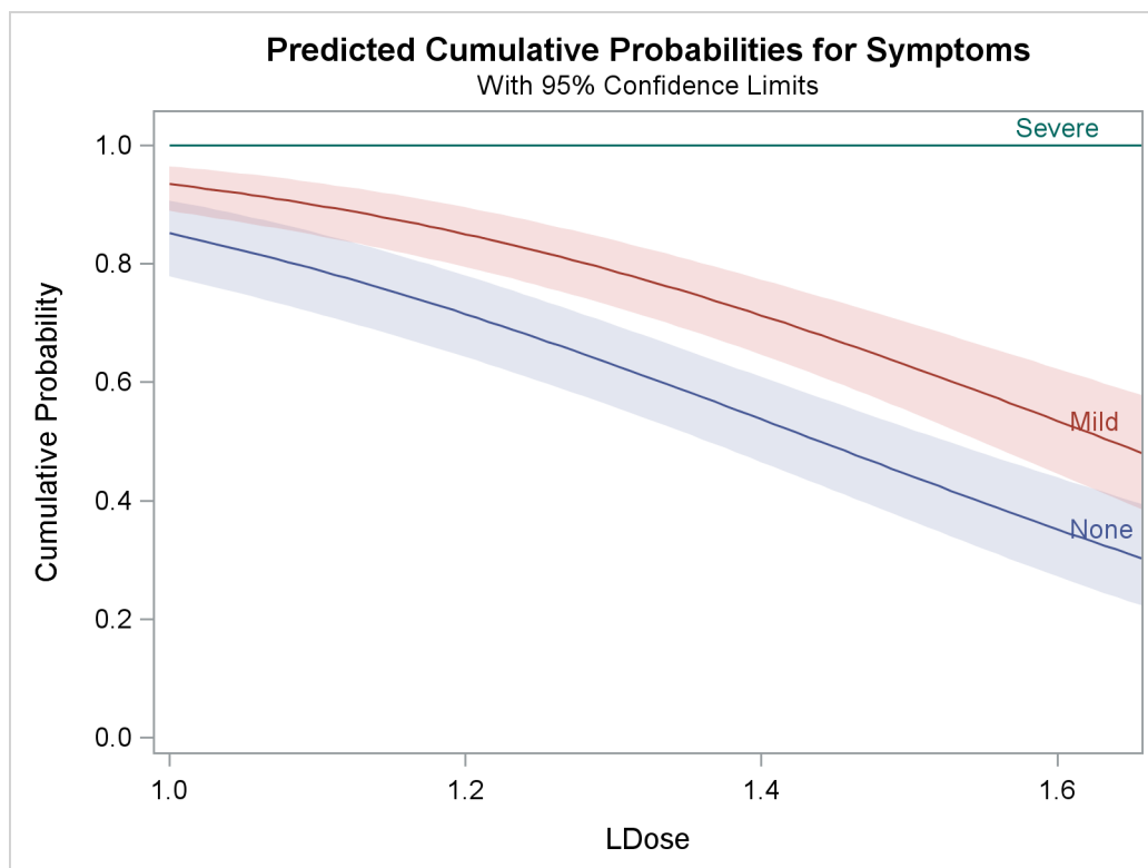
Output 95.2.4 Plot of Predicted Cumulative Probabilities for the Test Preparation Group
