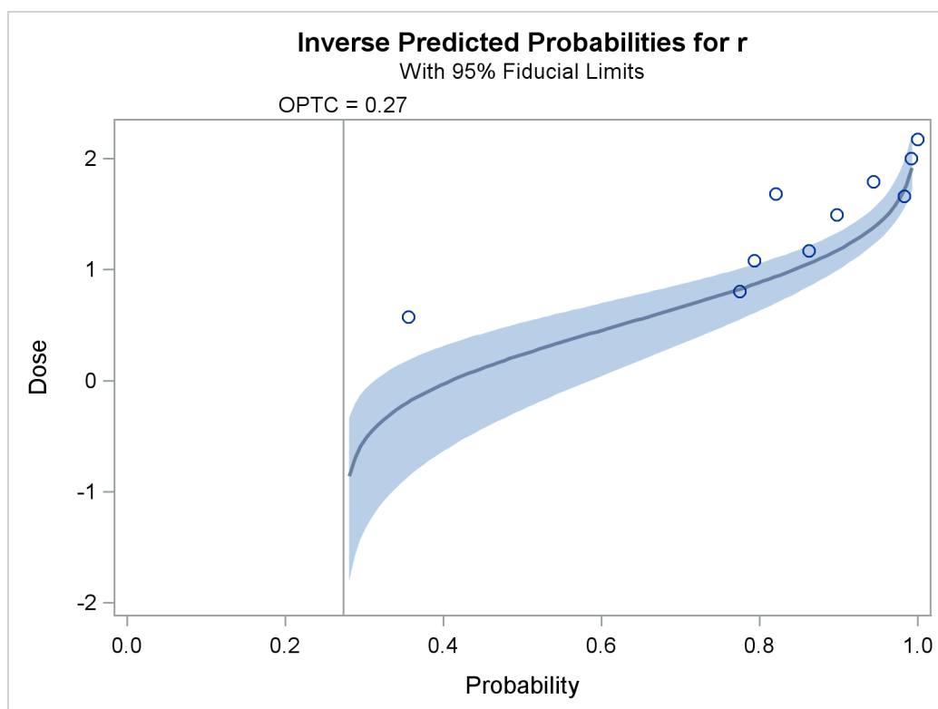
Output 95.4.12 Inverse Predicted Probability Plot
