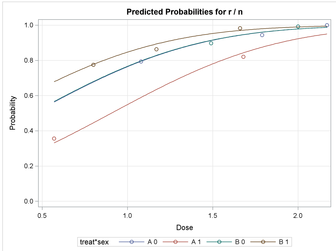
Output 95.5.3 Predicted Probability versus Dose Level by treat*sex
