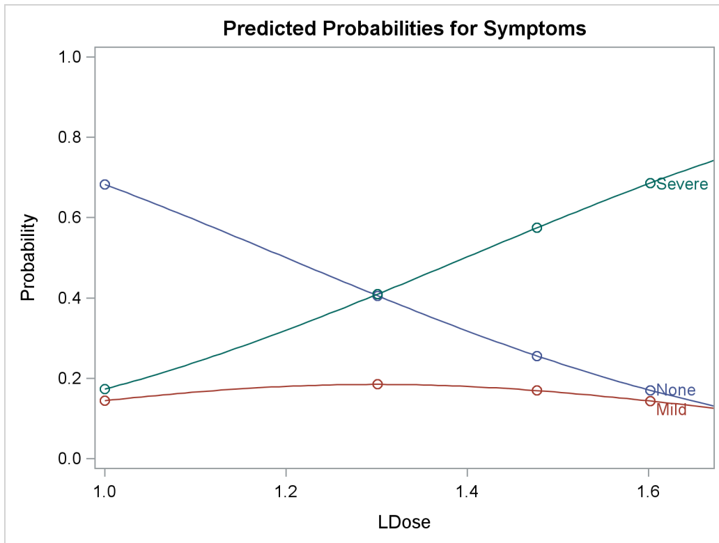
Output 95.2.5 Plot of Predicted Probabilities for the Standard Preparation Group
