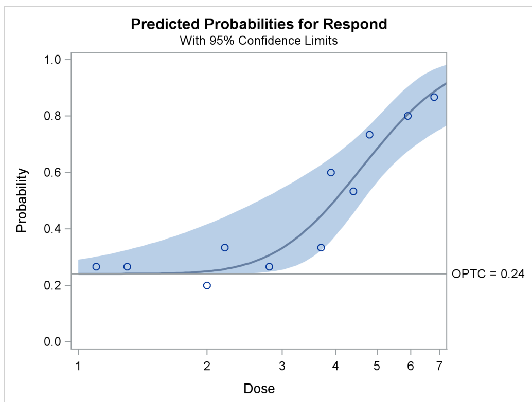
Figure 95.4 Plot of Observed and Fitted Probabilities versus Dose Level
