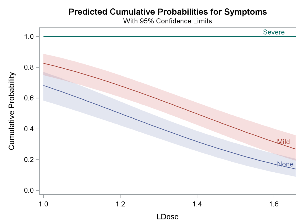
Output 95.2.6 Plot of Predicted Cumulative Probabilities for the Standard Preparation Group
