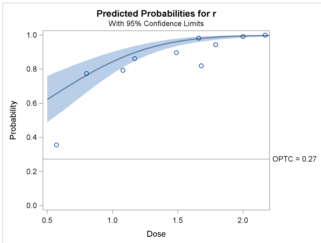
Output 95.4.11 Predicted Probability Plot
