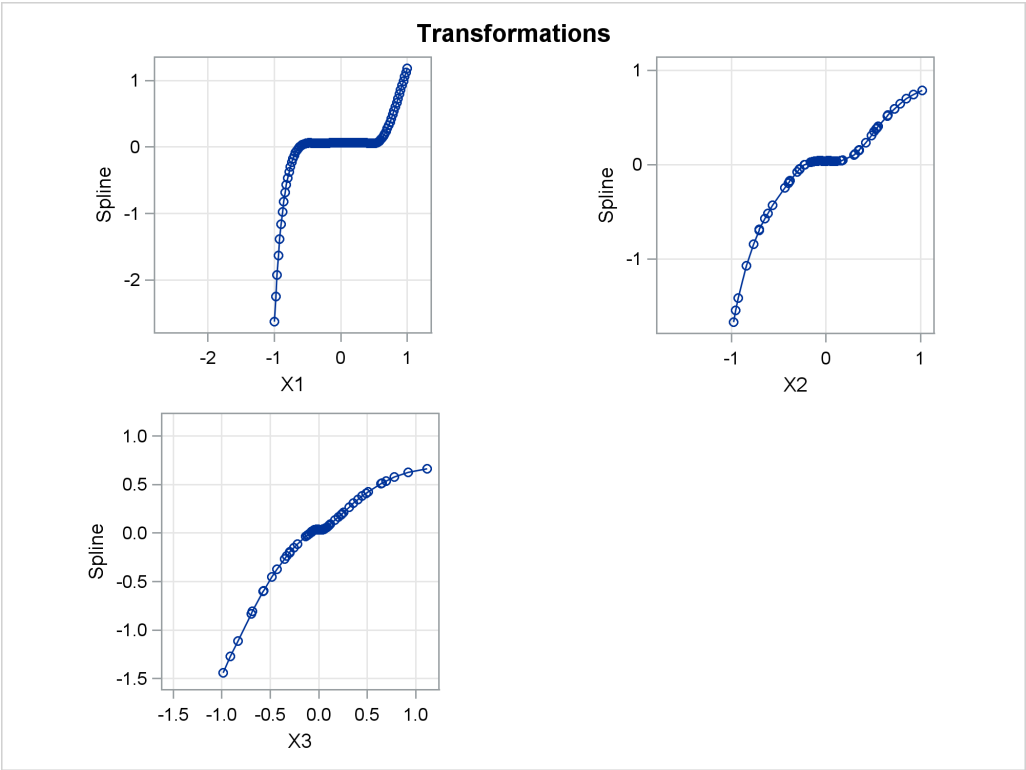
Figure 94.6 Transformations
