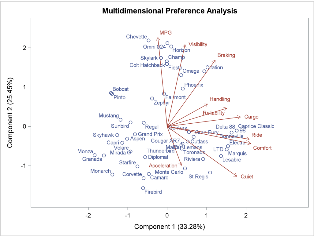
Figure 94.2 Automobile Ratings PCA Biplot
