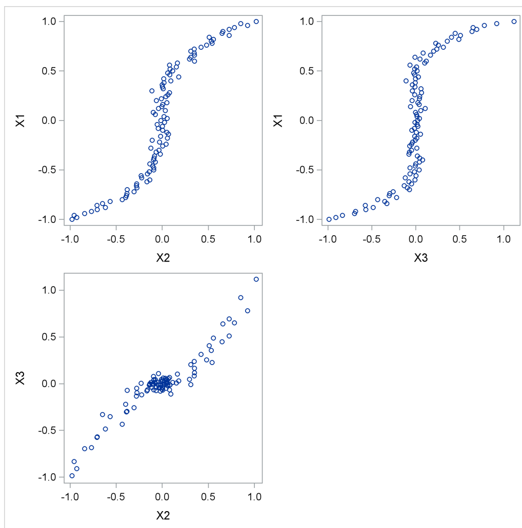
Figure 94.4 Three-Dimensional Scatter Plot
