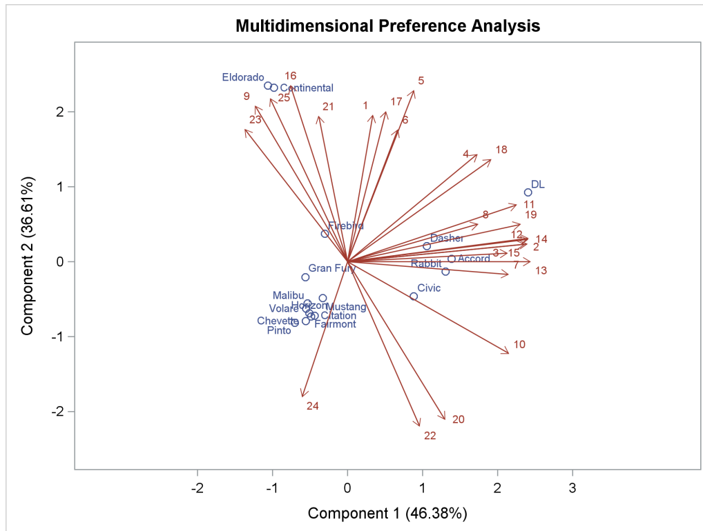
Output 94.1.3 Biplot Made with PRINQUAL
