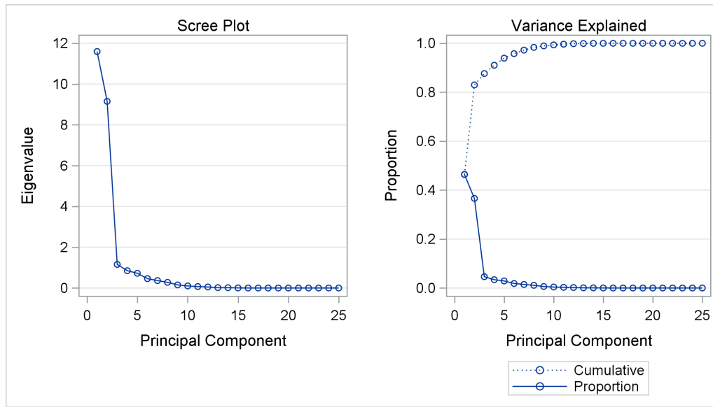
Output 94.1.4 Transformed Data Eigenvalue Plot
