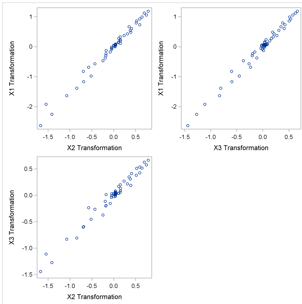
Figure 94.7 Linearized Scatter Plot
