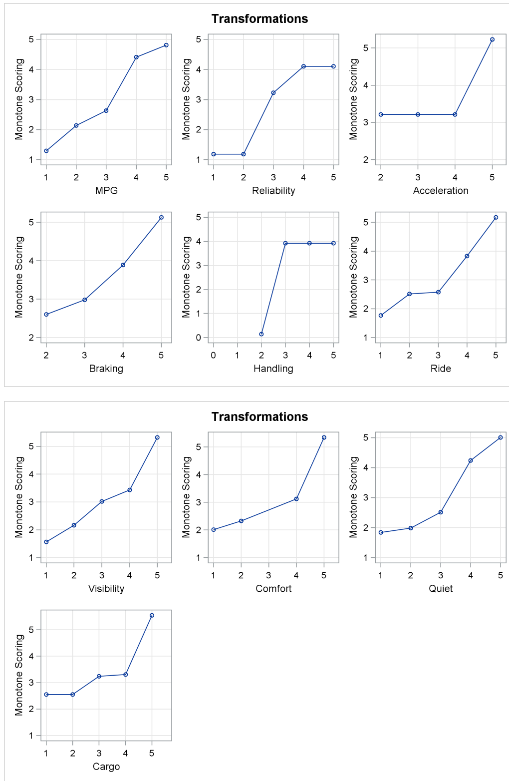
Figure 94.3 Automobile Ratings Transformations
