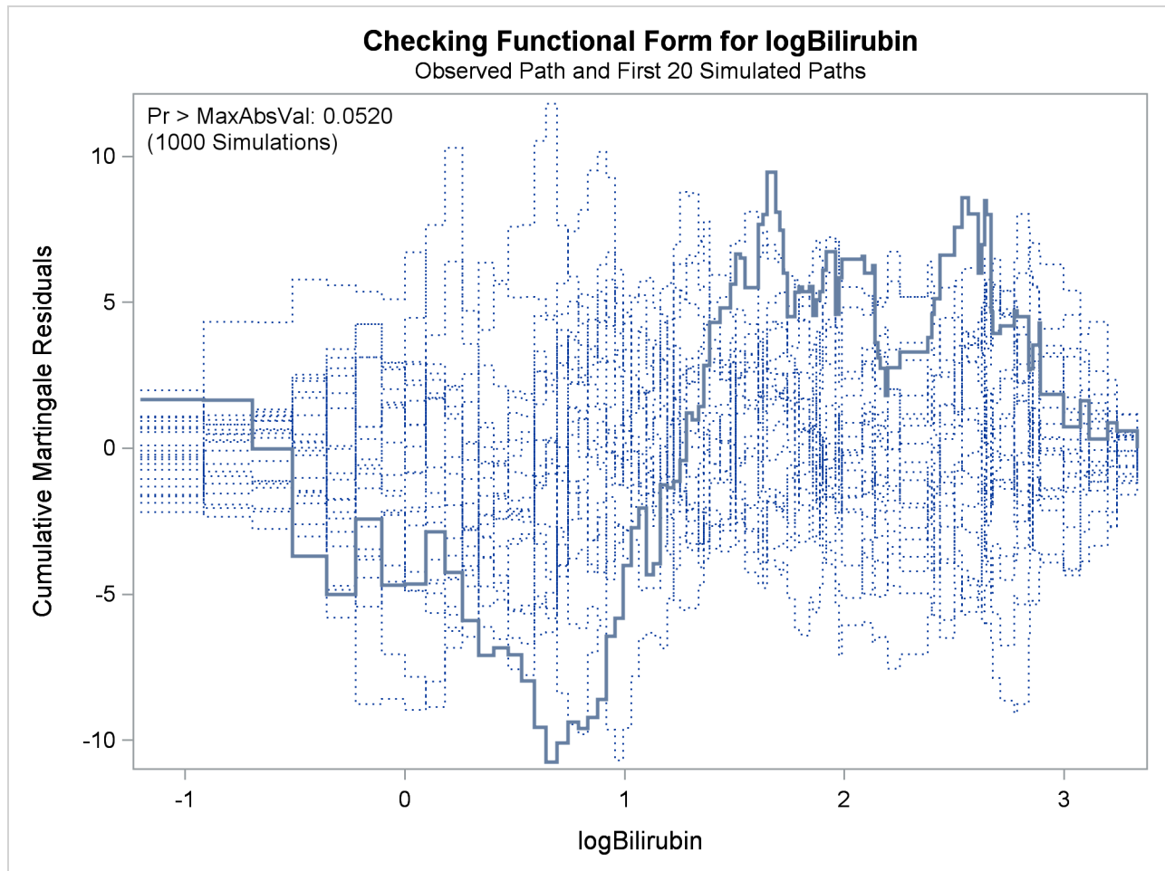
Output 87.12.6 Cumulative Martingale Residuals versus log(Bilirubin)
