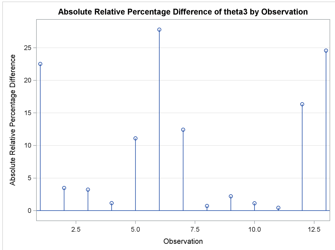
Output 83.7.6 Observation Influence on Parameter Estimate
