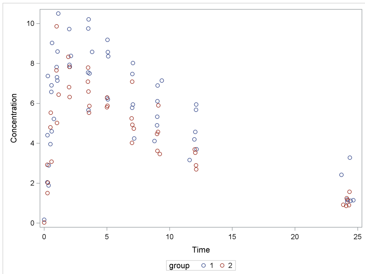
Output 83.5.1 Observed Responses in Two Groups
