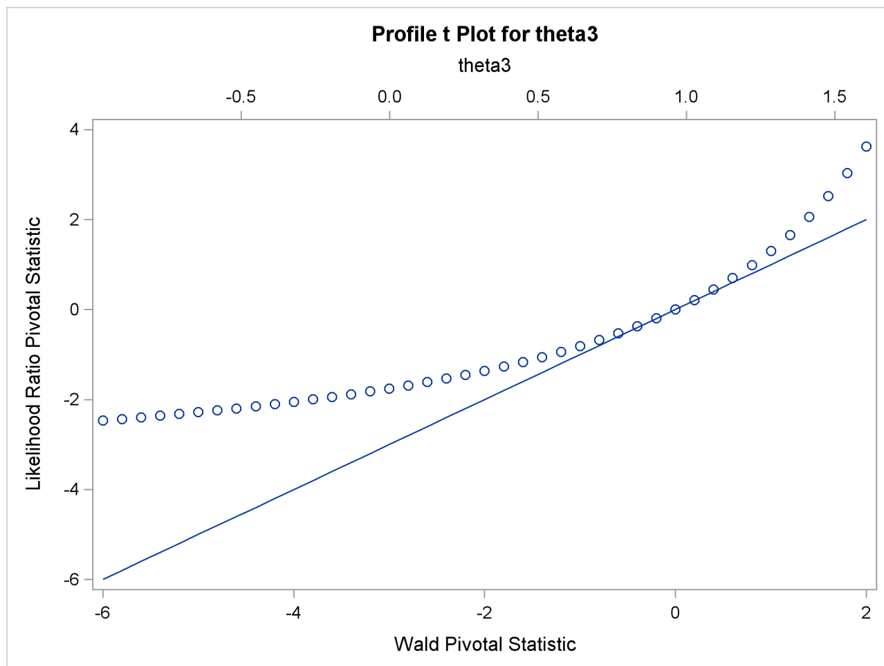
Output 83.7.3 Profile t Plot
