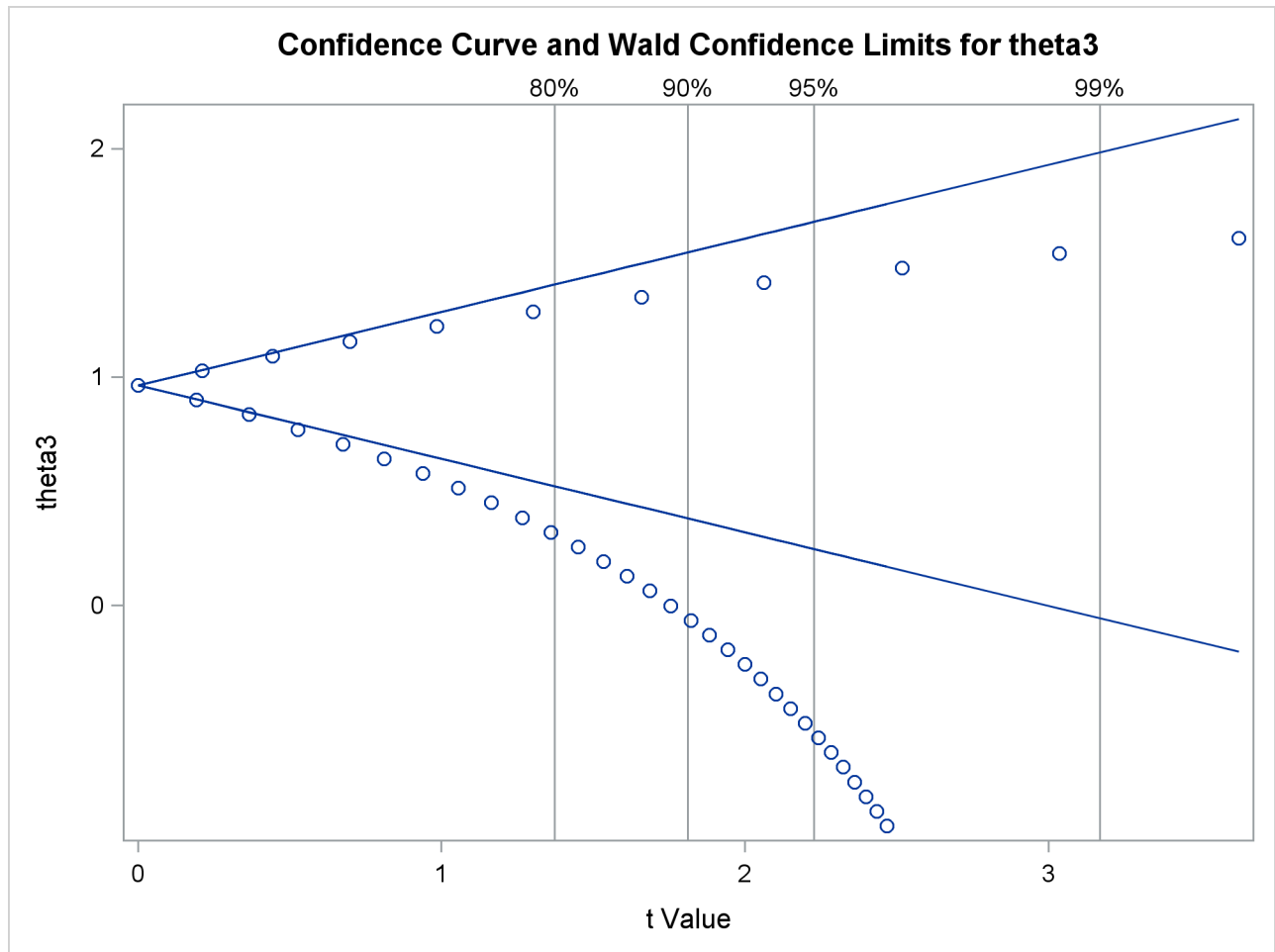
Output 83.7.5 Confidence Curve
