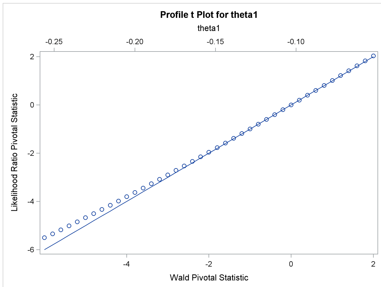
Output 83.7.2 Profile t Plot
