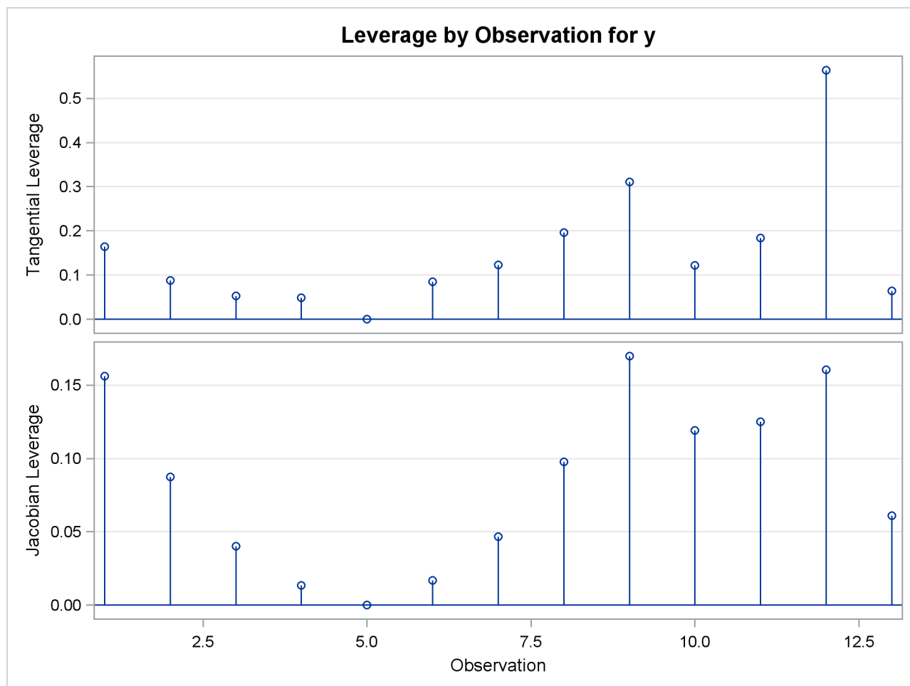
Output 83.6.3 Leverage Plots
