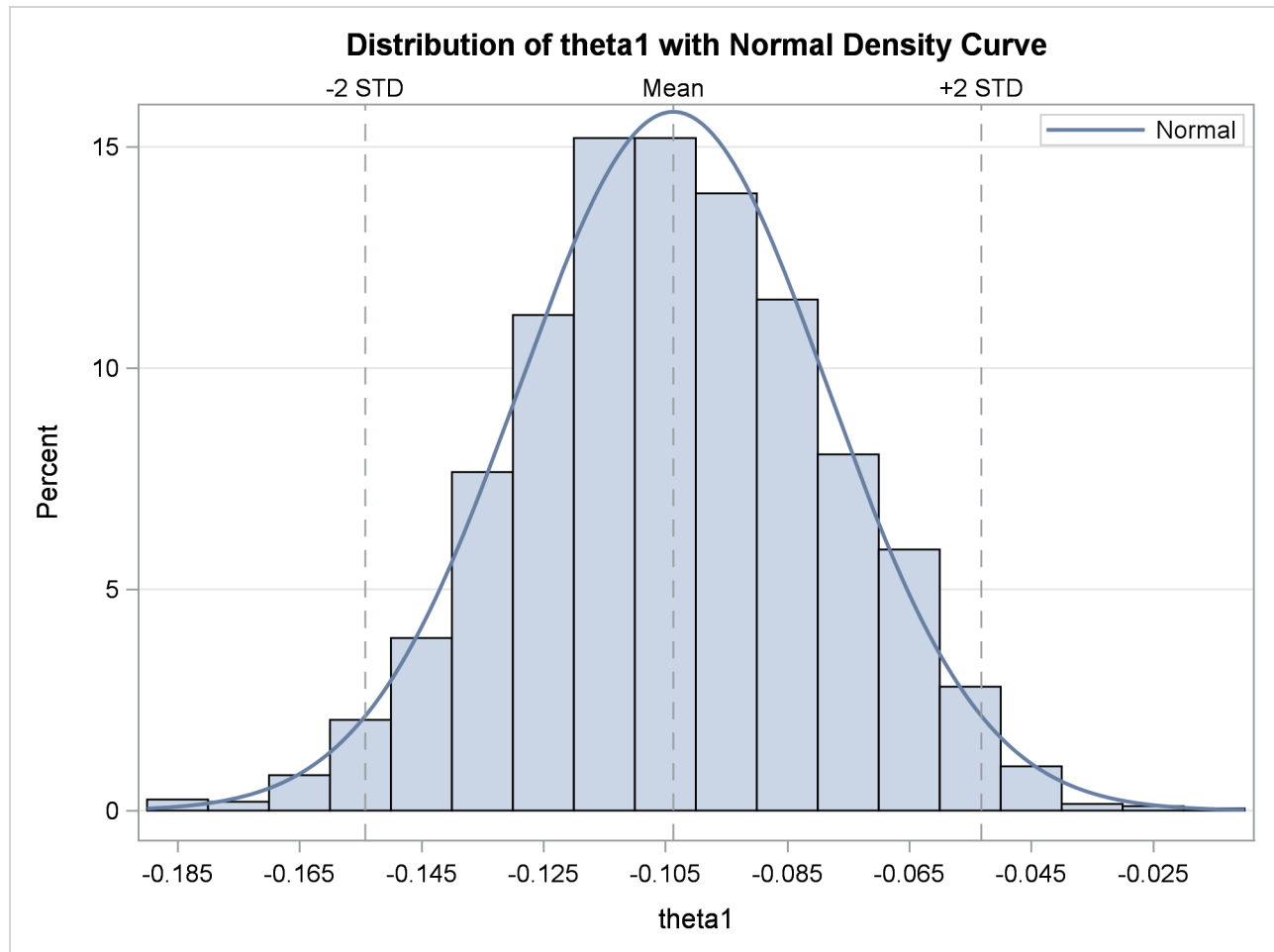
Output 83.7.8 Histogram of Bootstrap Parameter Estimates
