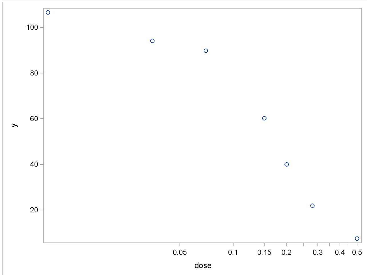
Output 83.4.1 Observed Data in Dose-Response Experiment
