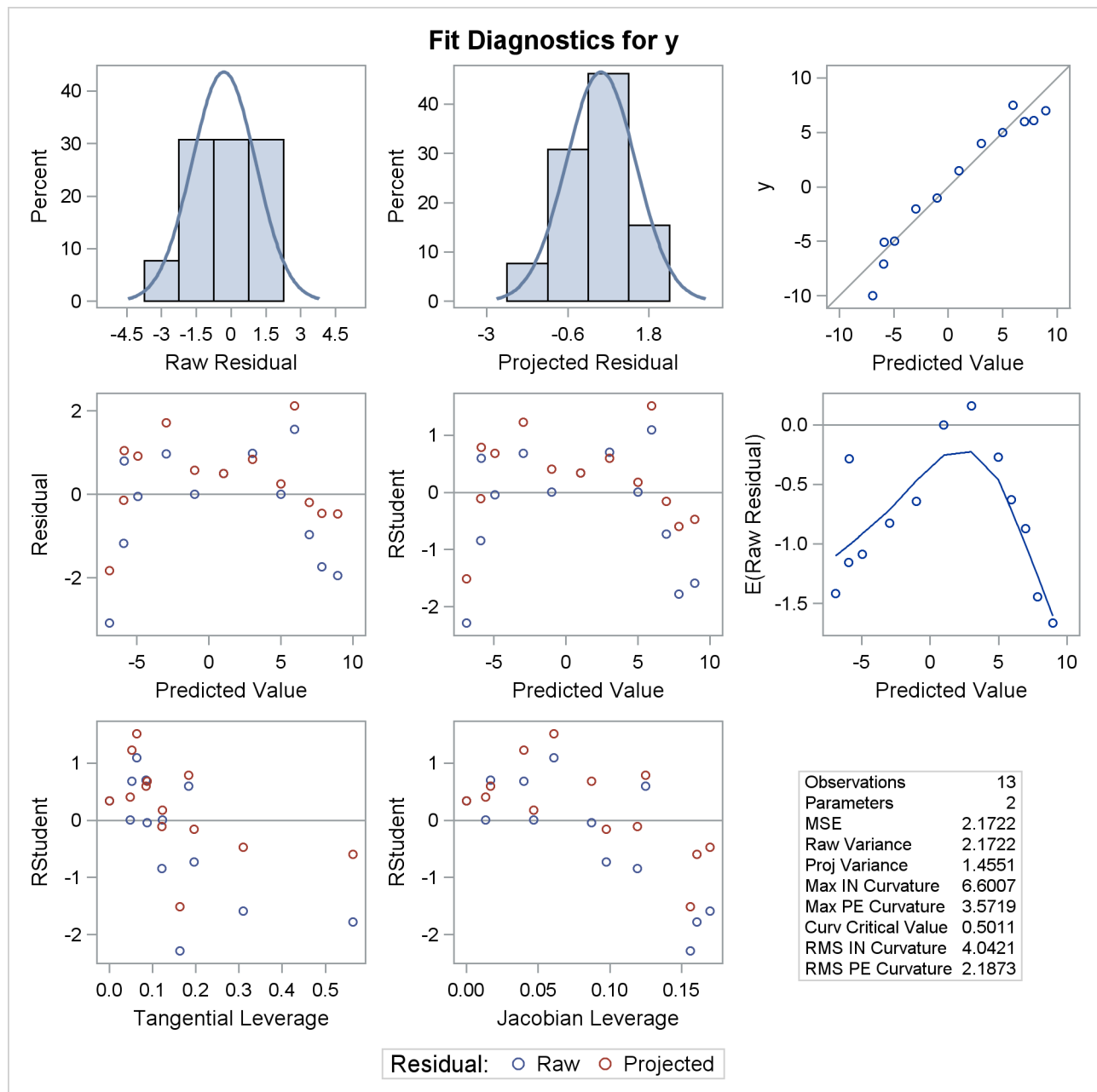
Output 83.6.2 Diagnostics Panel
