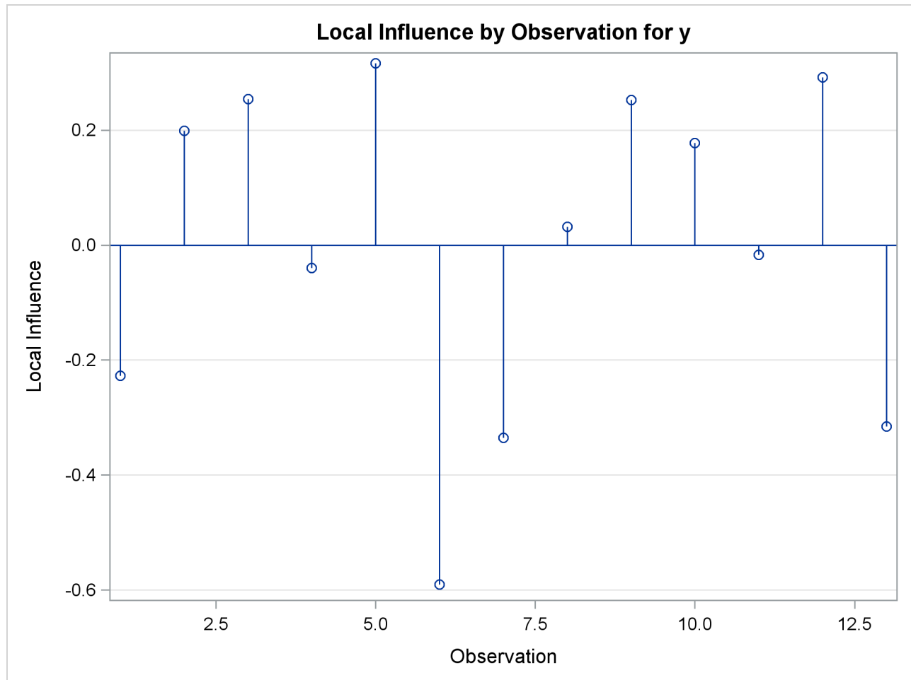
Output 83.7.7 Local Influence Plot
