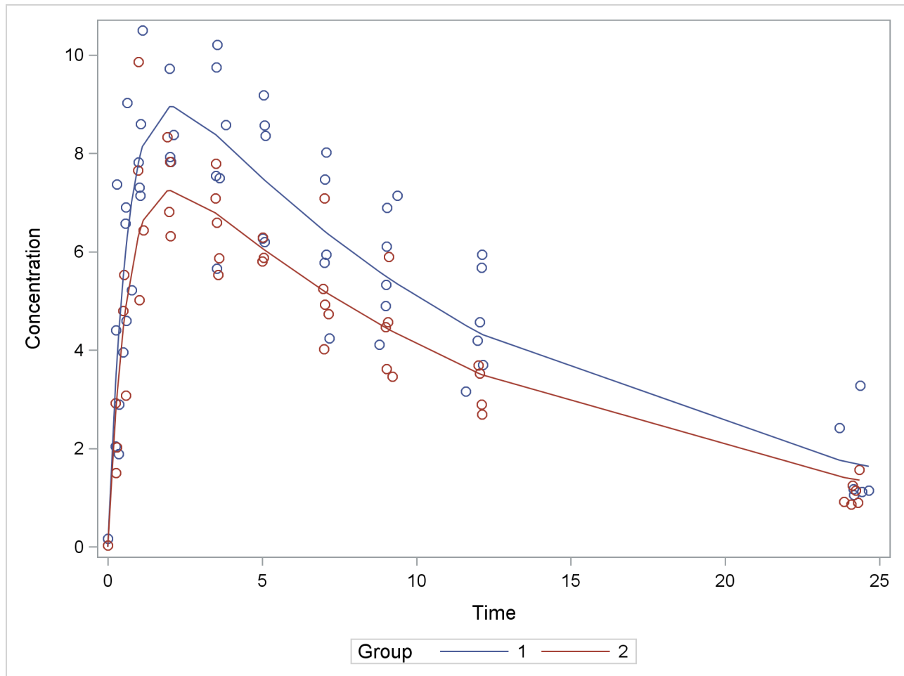
Output 83.5.8 Observed and Fitted Values for Theophylline Data
