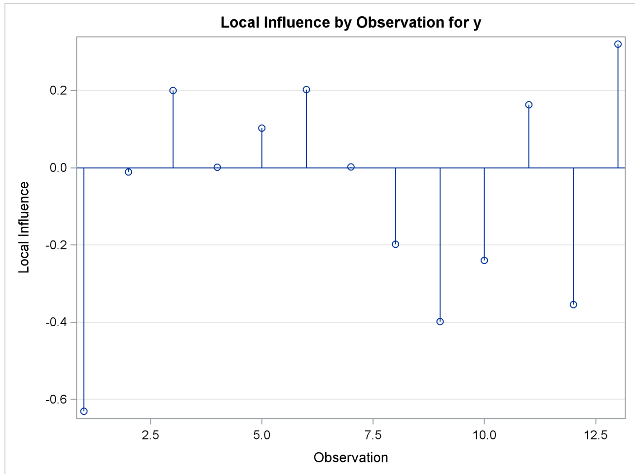
Output 83.6.4 Local Influence Plot
