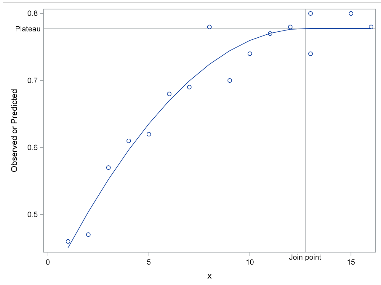
Output 83.1.4 Observed and Predicted Values for the Quadratic Model
