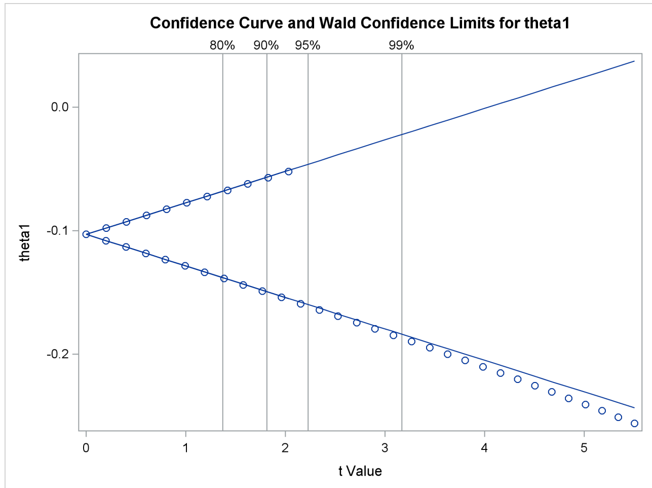
Output 83.7.4 Confidence Curve
