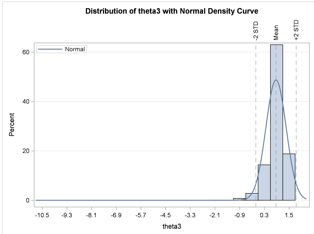
Output 83.7.9 Histogram of Bootstrap Parameter Estimates
