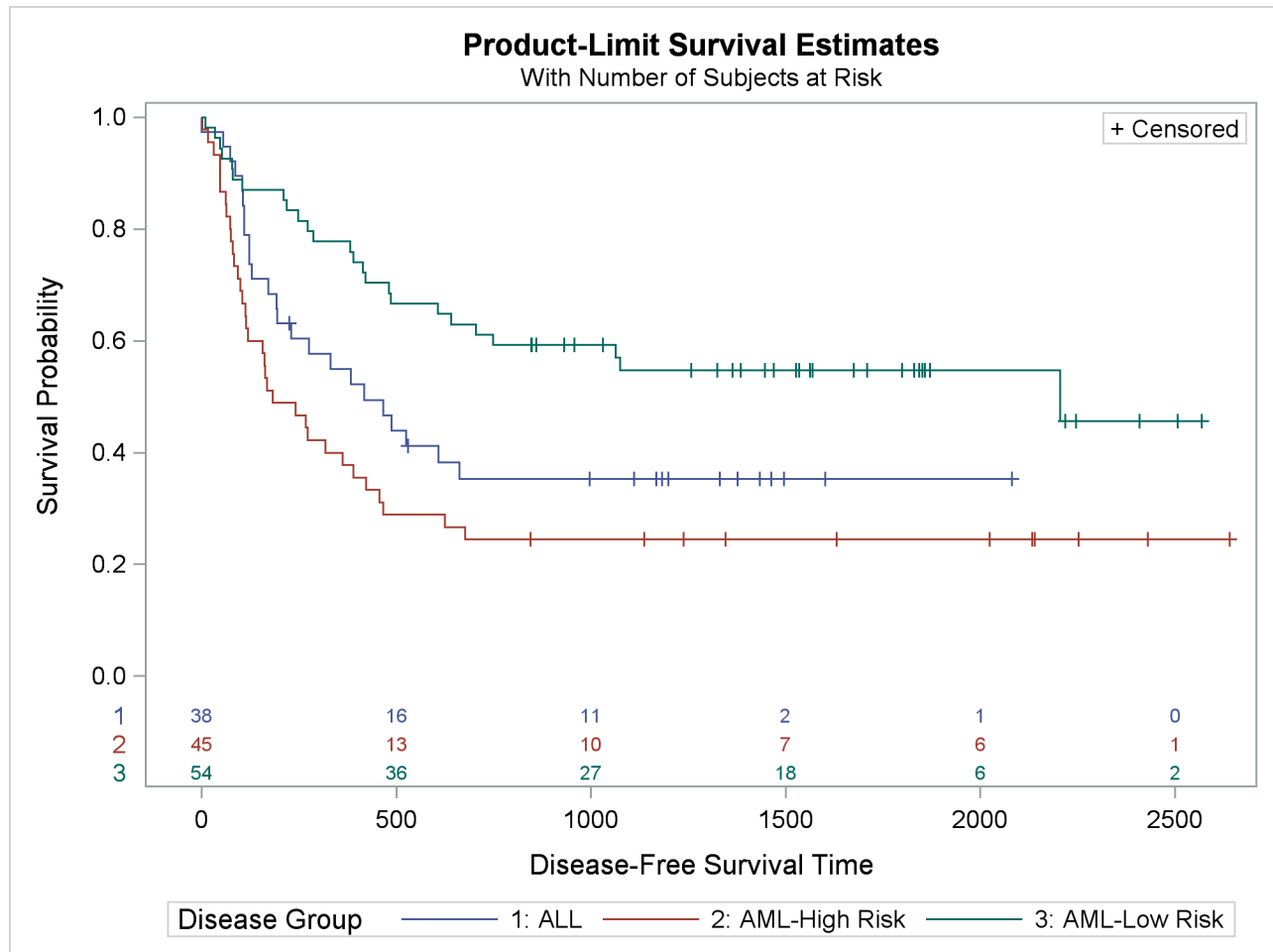
Output 72.2.2 Estimated Disease-Free Survival for 137 Bone Marrow Transplant Patients
