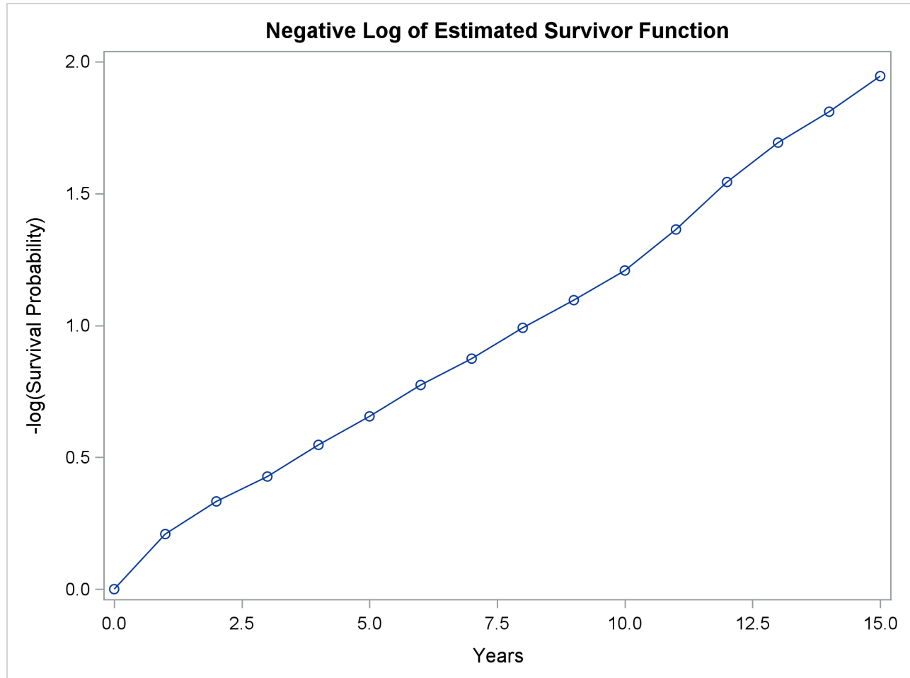
Output 72.3.4 Negative Log of Survivor Function Estimate
