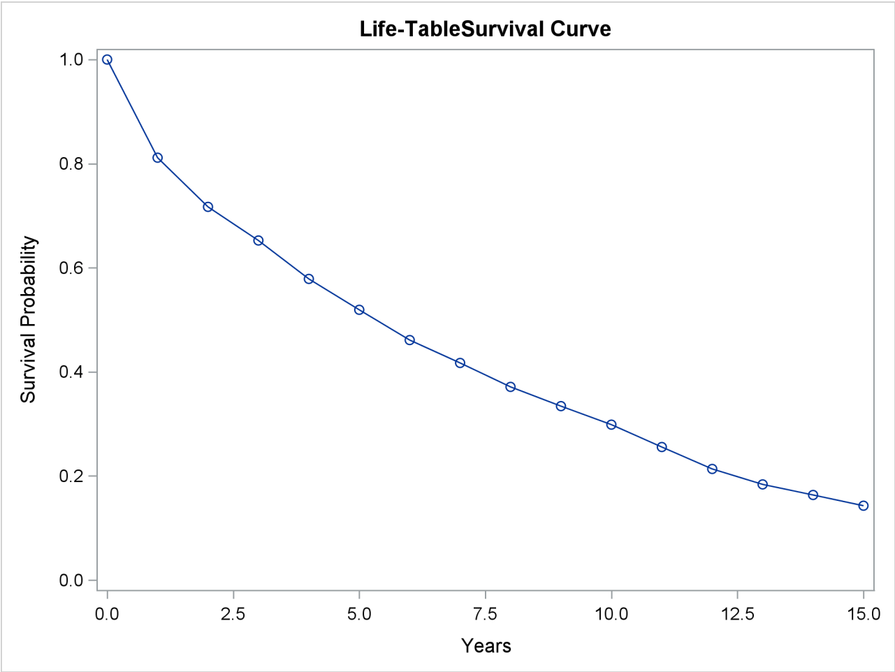
Output 72.3.3 Life-Table Survivor Function Estimate
