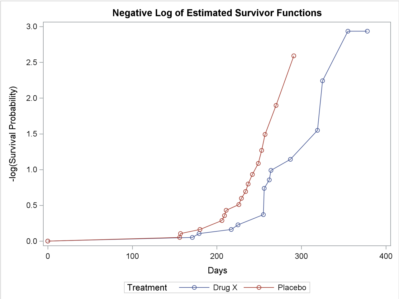
Figure 72.7 Plot of Estimated Negative Log Survivor Functions
