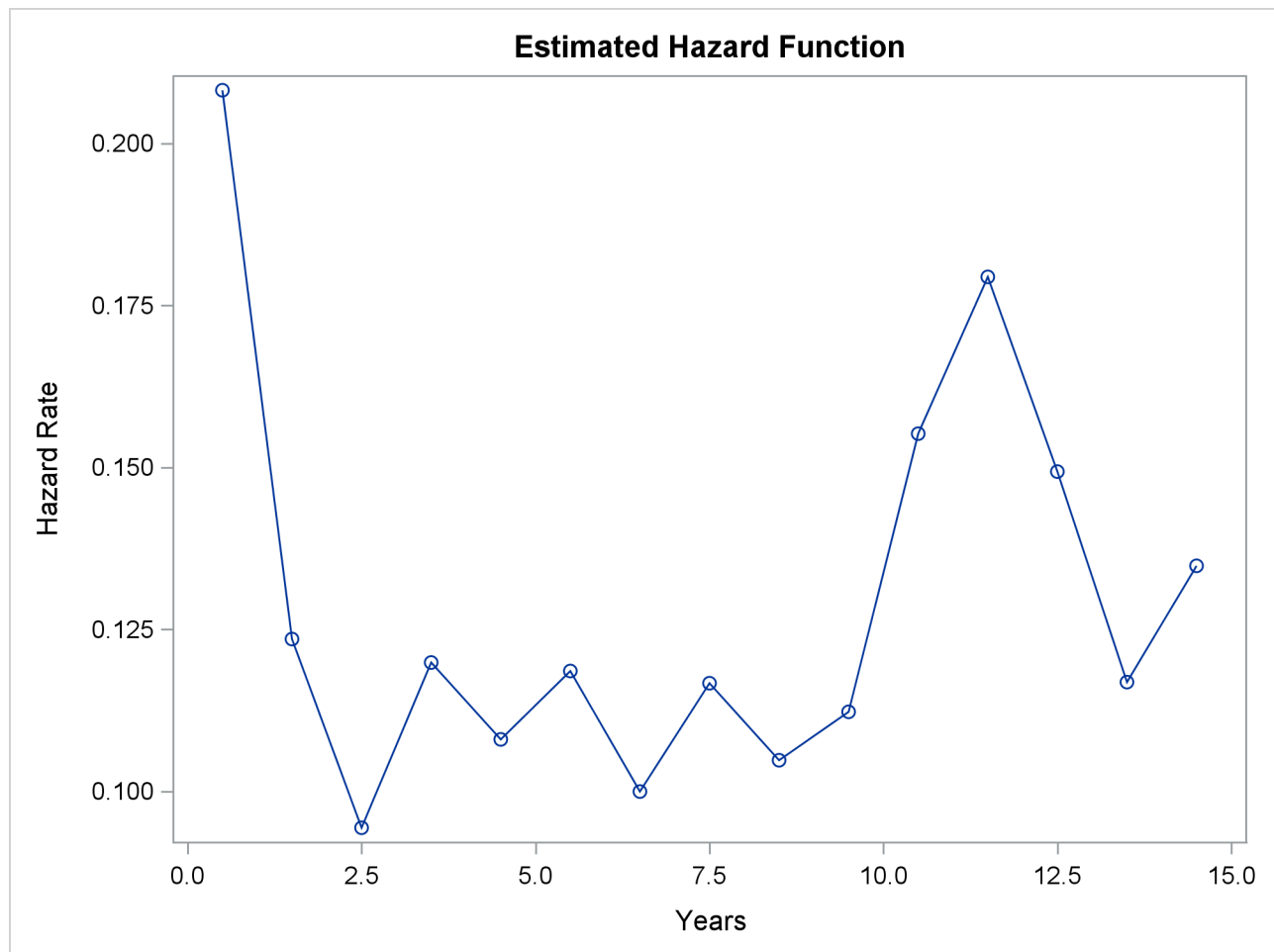
Output 72.3.6 Hazard Function Estimate
