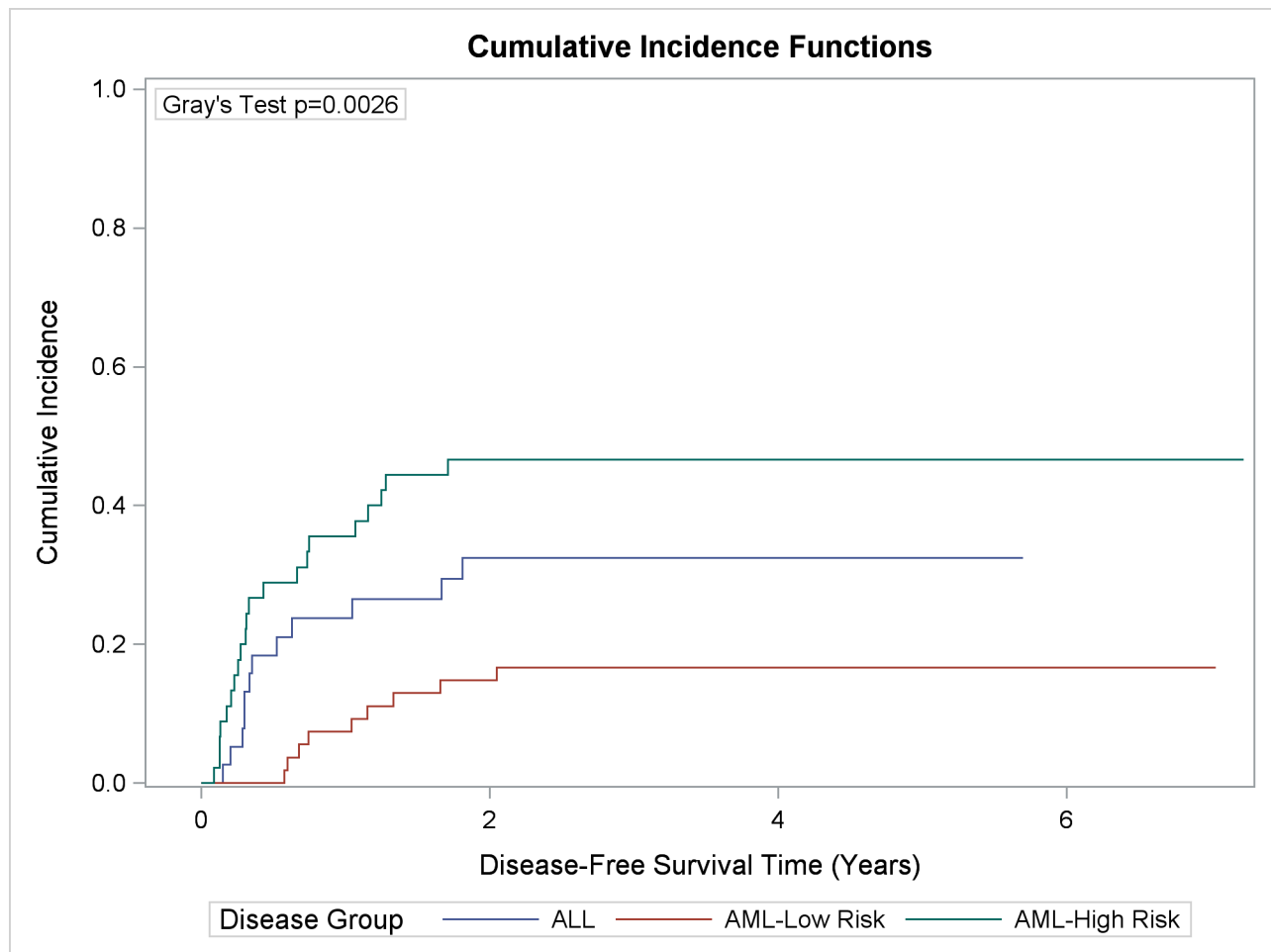
Output 72.4.6 CIF Estimates of Relapse in Bone Marrow Transplant Study
