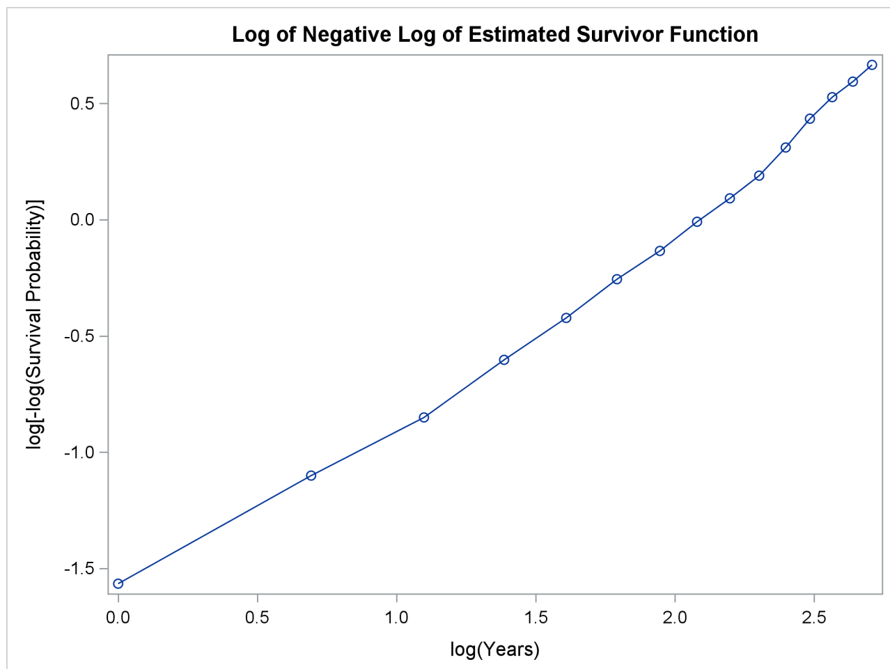
Output 72.3.5 Log of Negative Log of Survivor Function Estimate
