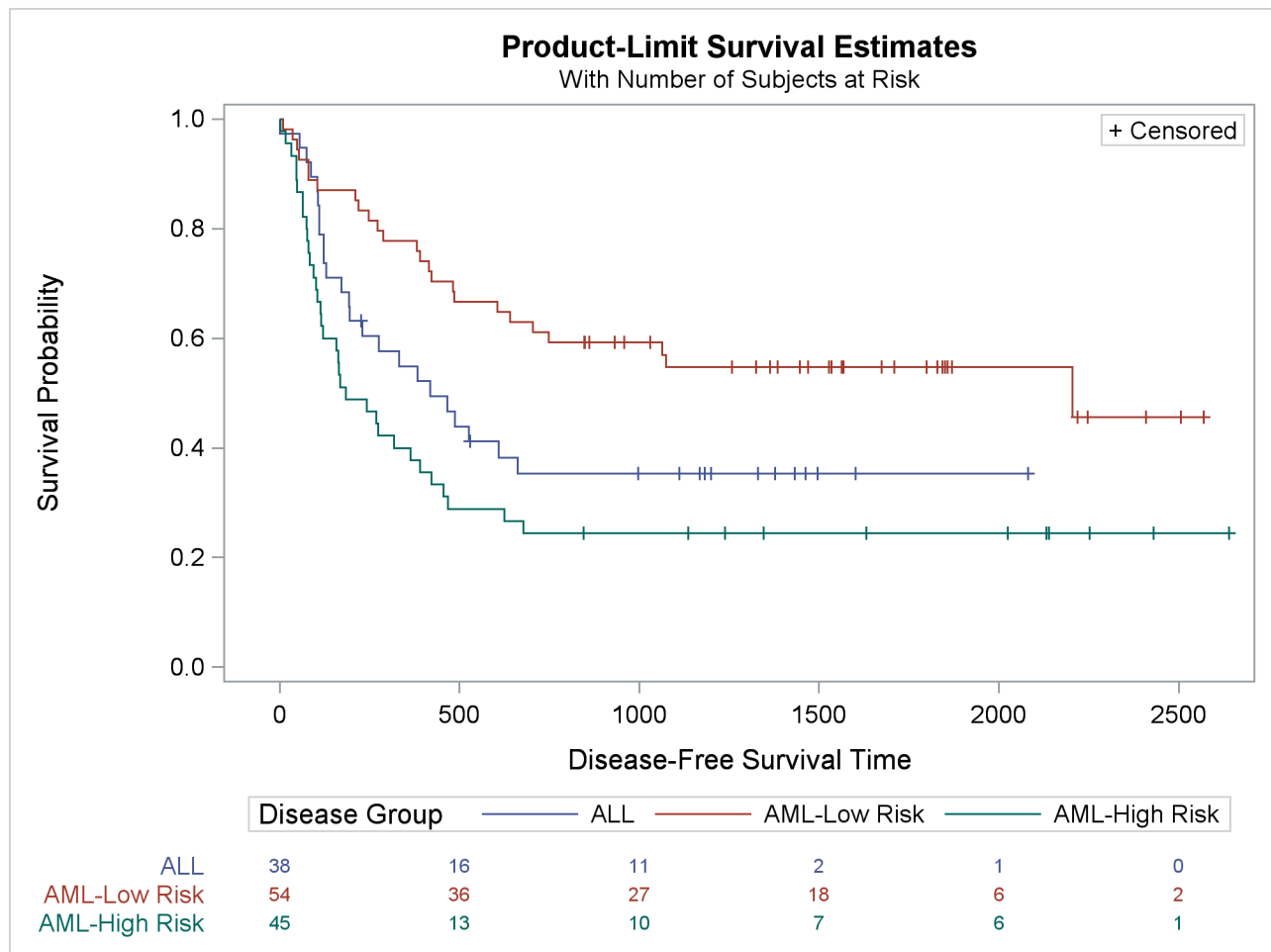
Output 72.2.6 Modified Disease-Free Survival for Bone Marrow Transplant Patients
