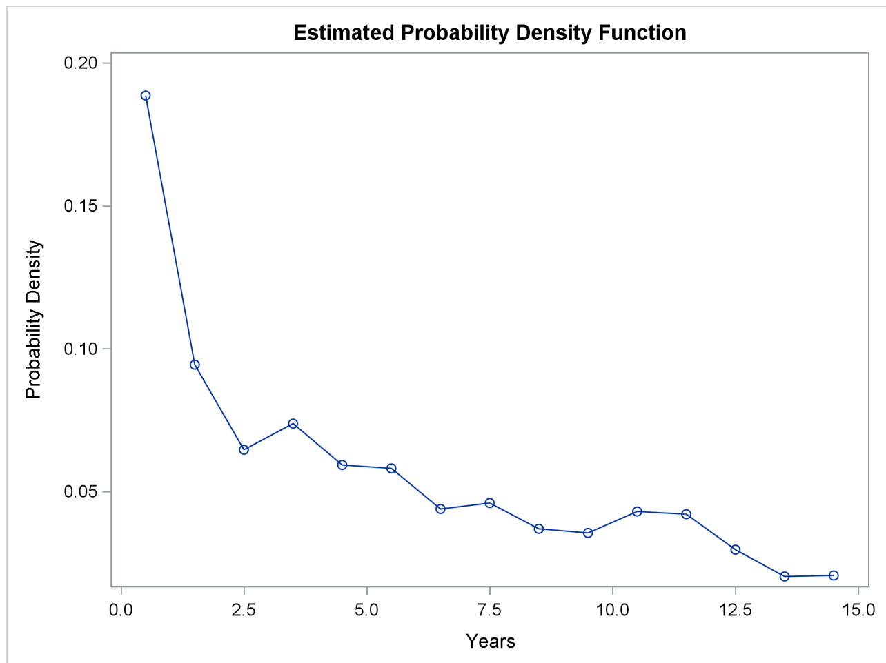
Output 72.3.7 Density Function Estimate
