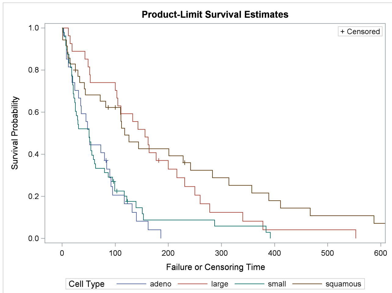
Output 72.1.6 Graph of the Estimated Survivor Functions
