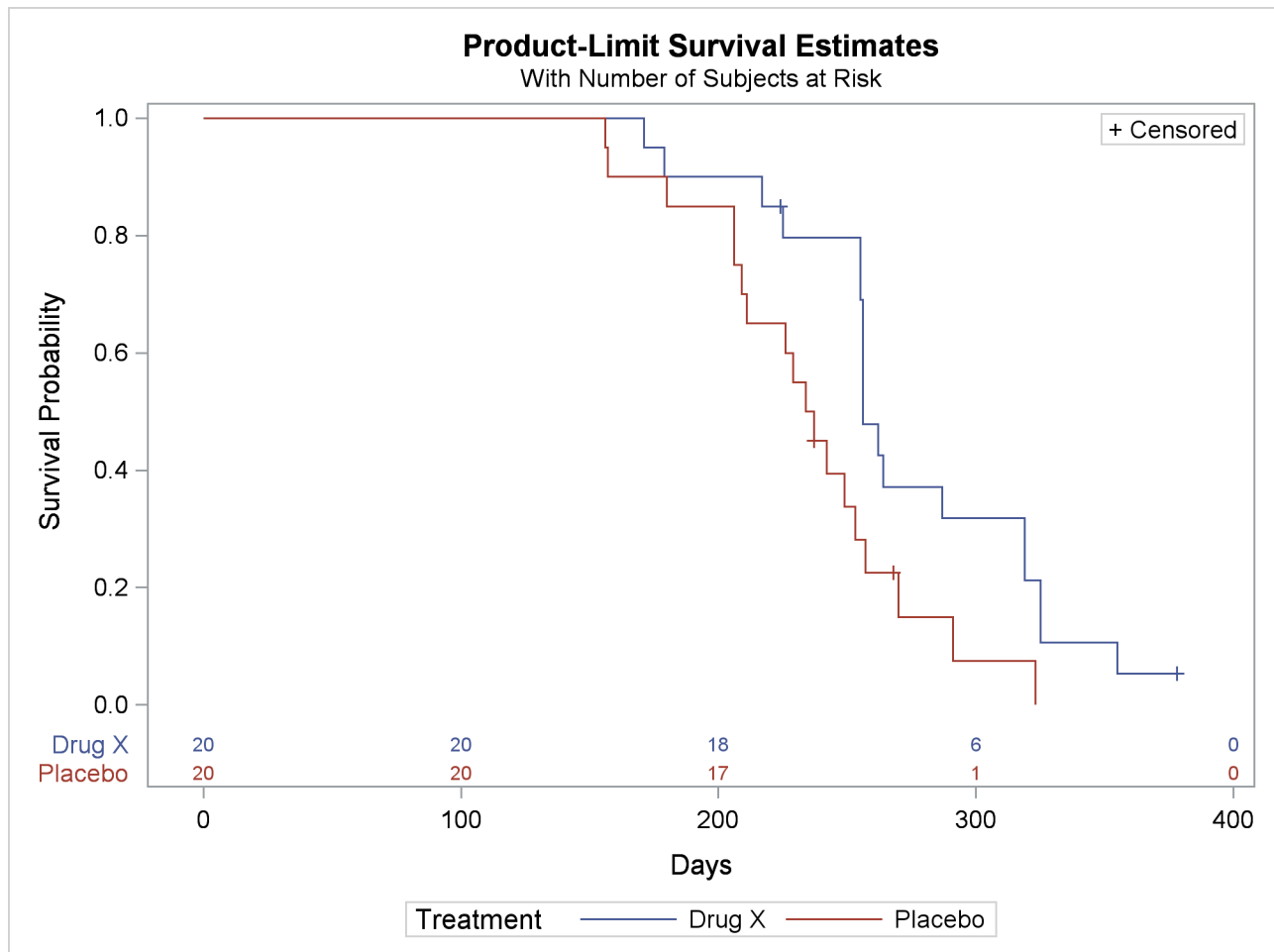
Figure 72.6 Plot of Estimated Survivor Functions
