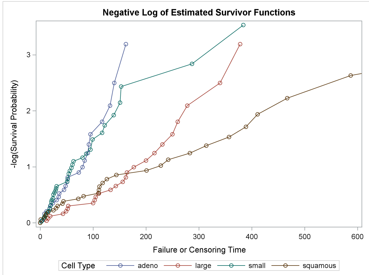
Output 72.1.7 Graph of Negative Log of the Estimated Survivor Functions
