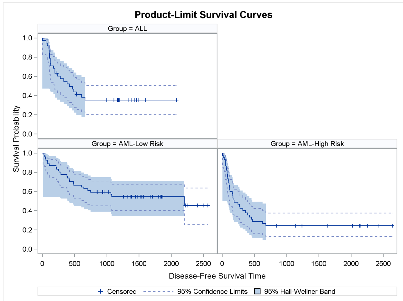
Output 72.2.7 Estimated Disease-Free Survivor Functions with Confidence Limits
