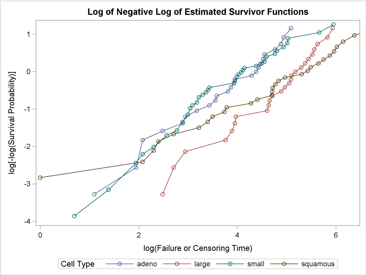
Output 72.1.8 Graph of Log of the Negative Log of the Estimated Survivor Functions
