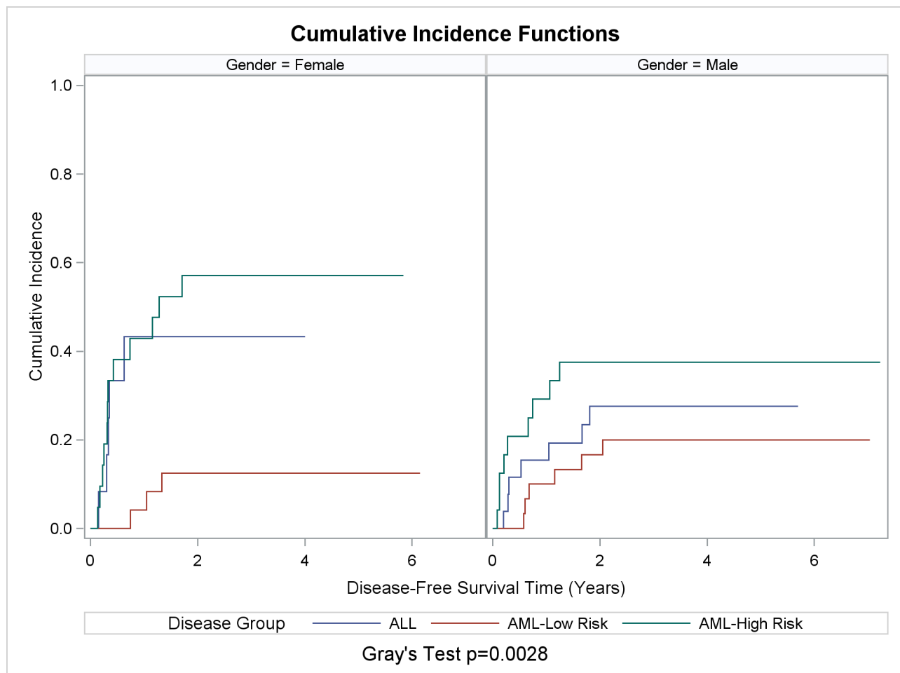
Output 72.4.10 Panel Plots of CIFs for Relapse
