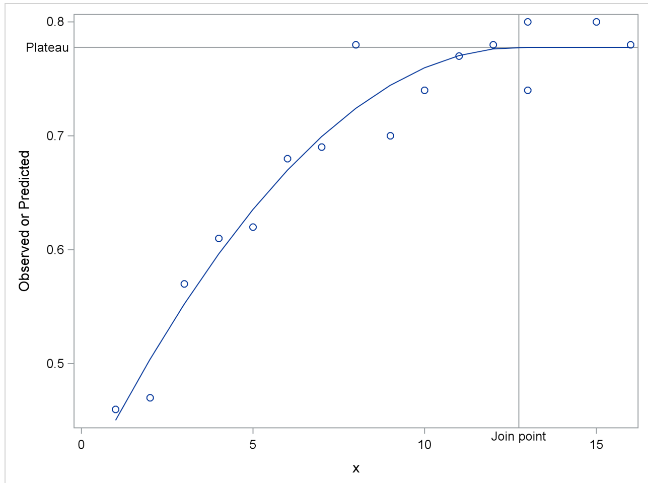
Output 58.1.4 Observed and Predicted Values for the Quadratic Model
