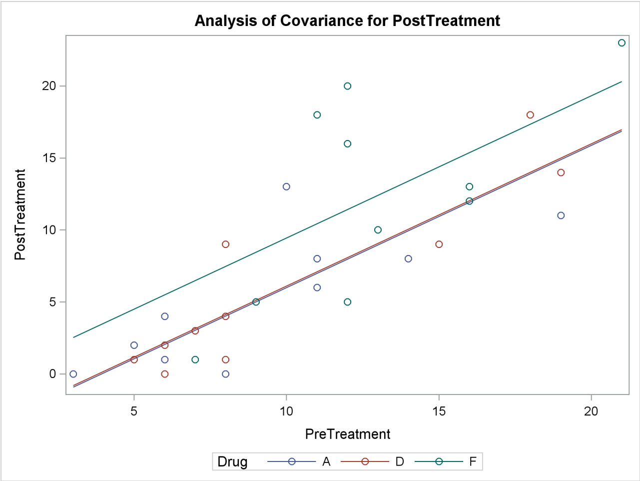
Output 48.4.6 Analysis of Covariance Plot of PostTreatment Score by Drug and PreTreatment Score
