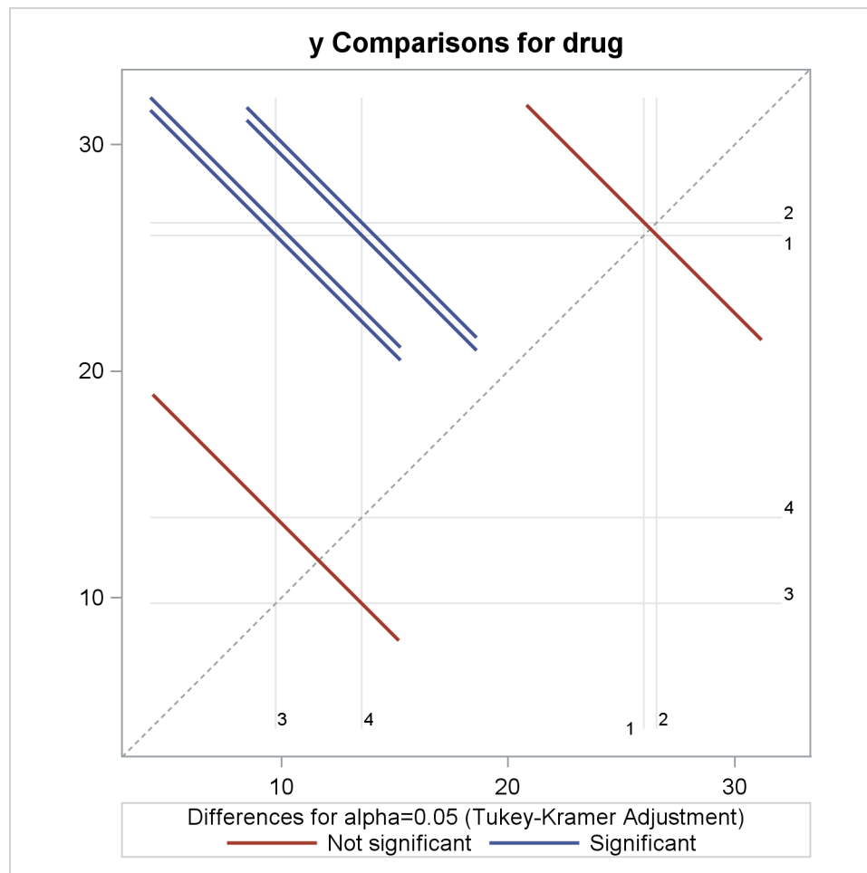
Output 48.3.7 Plot of Response LS-Mean Differences for Drug
