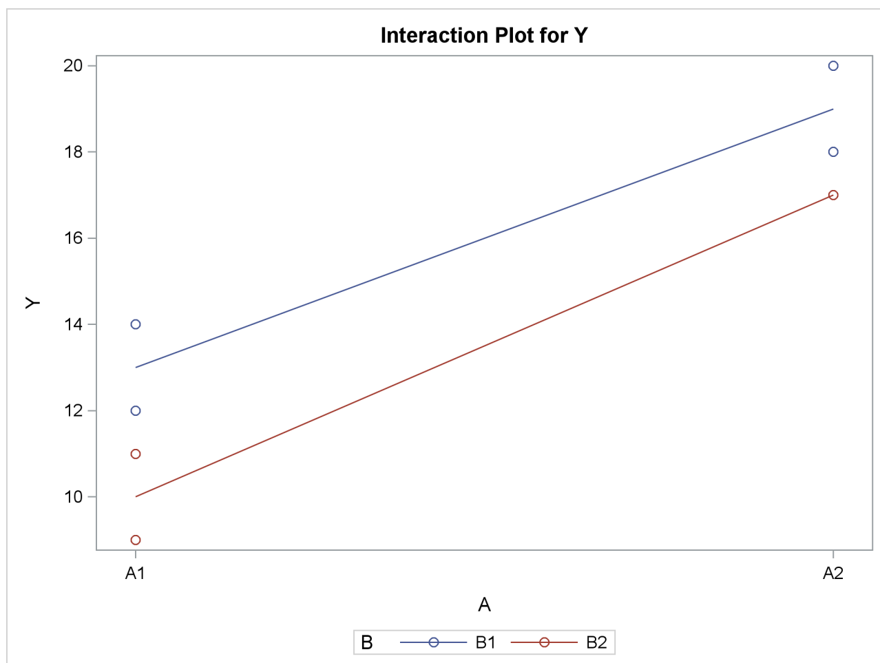
Figure 48.3 Plot of Y by A and B
