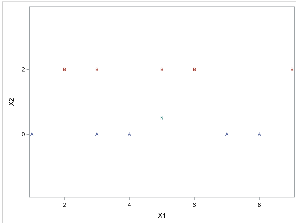
Figure 37.6 Plot of Data with Singular Within-Class Covariance Matrix
