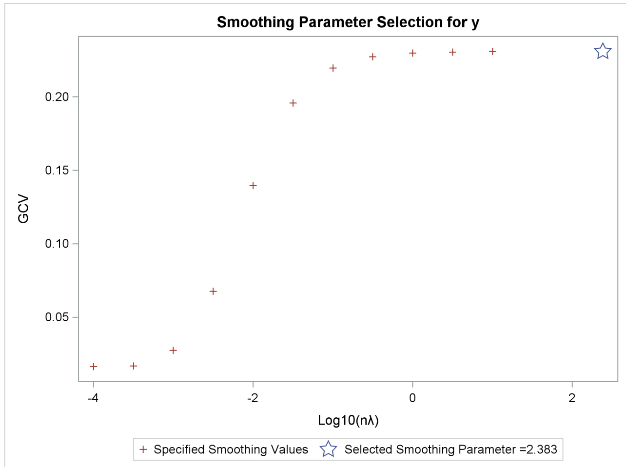
Output 118.2.4 Criterion Plot
