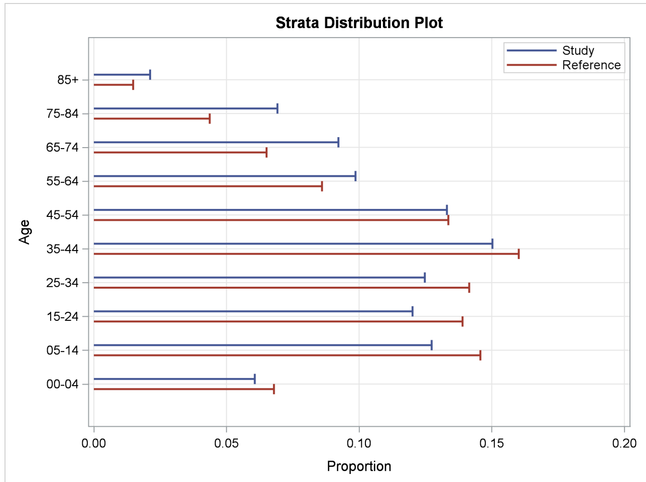
Figure 107.3 Strata Distribution Plot
