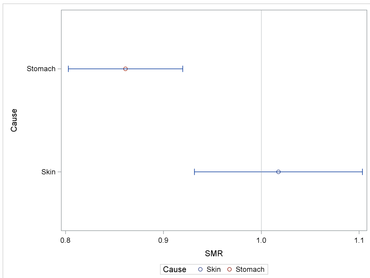
Output 107.4.10 SMR Results
