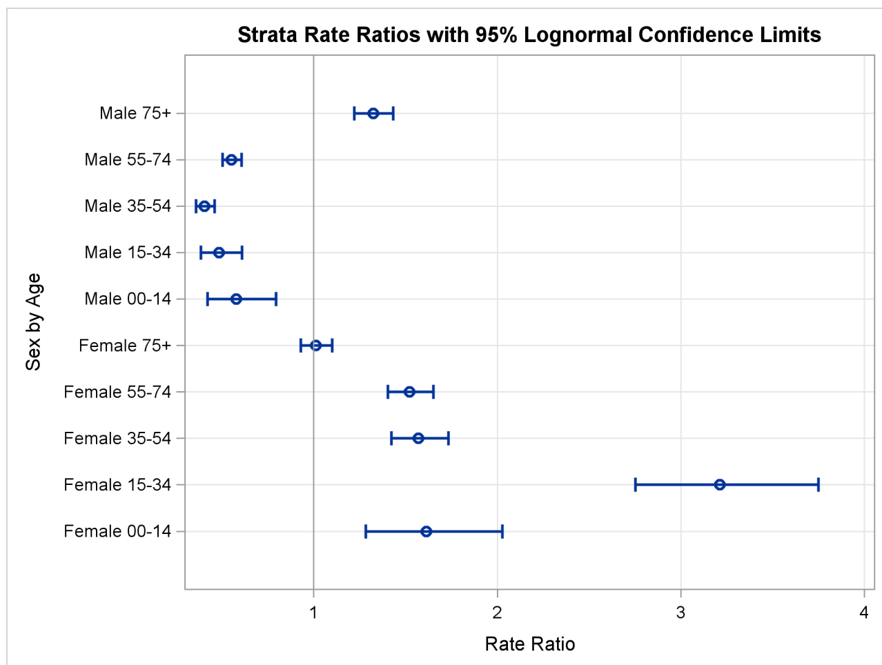
Output 107.1.4 Strata Effect Measure Plot
