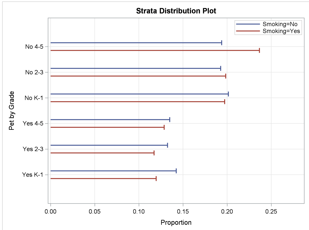
Output 107.2.3 Strata Distribution Plot
