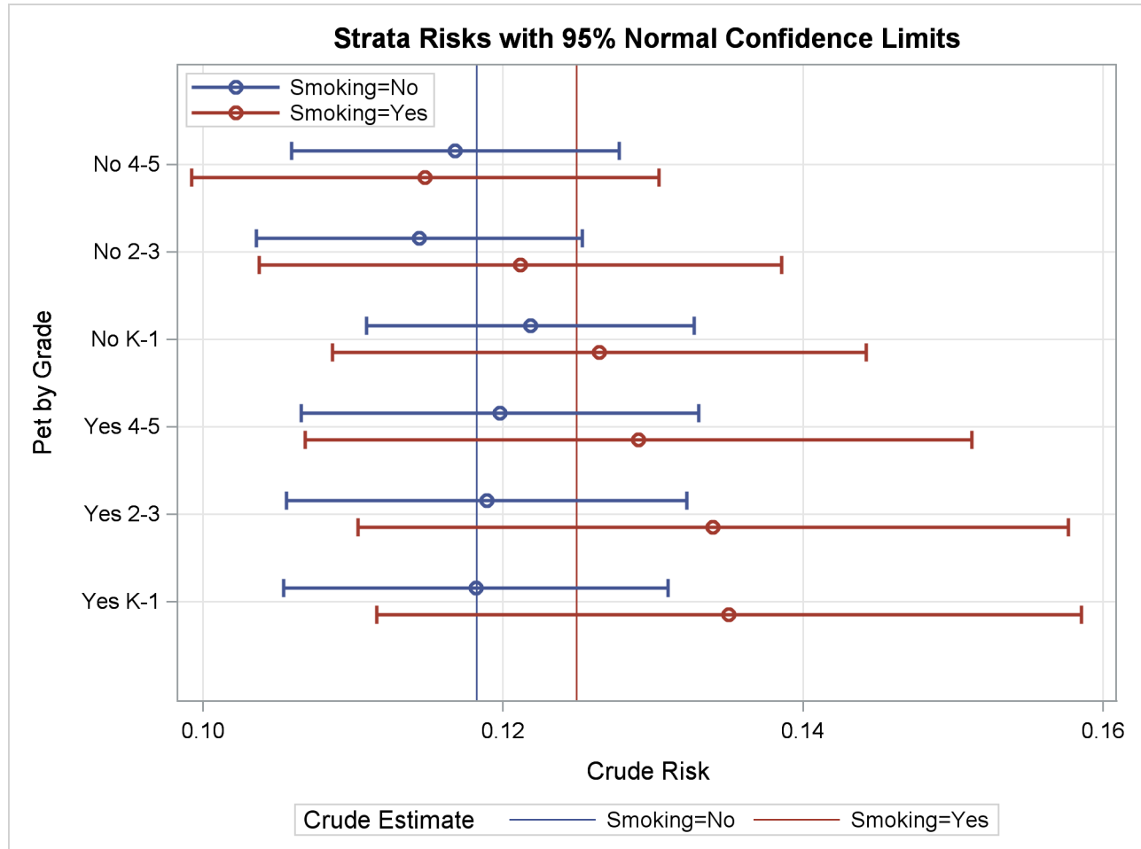
Output 107.2.4 Strata Risk Plot
