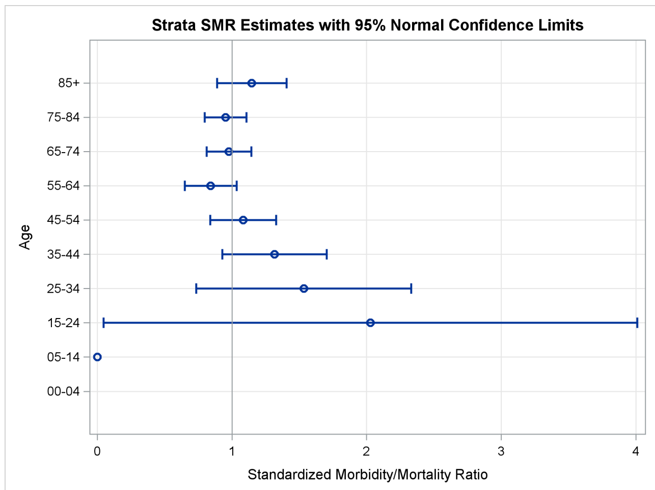
Output 107.4.4 Strata SMR Plot
