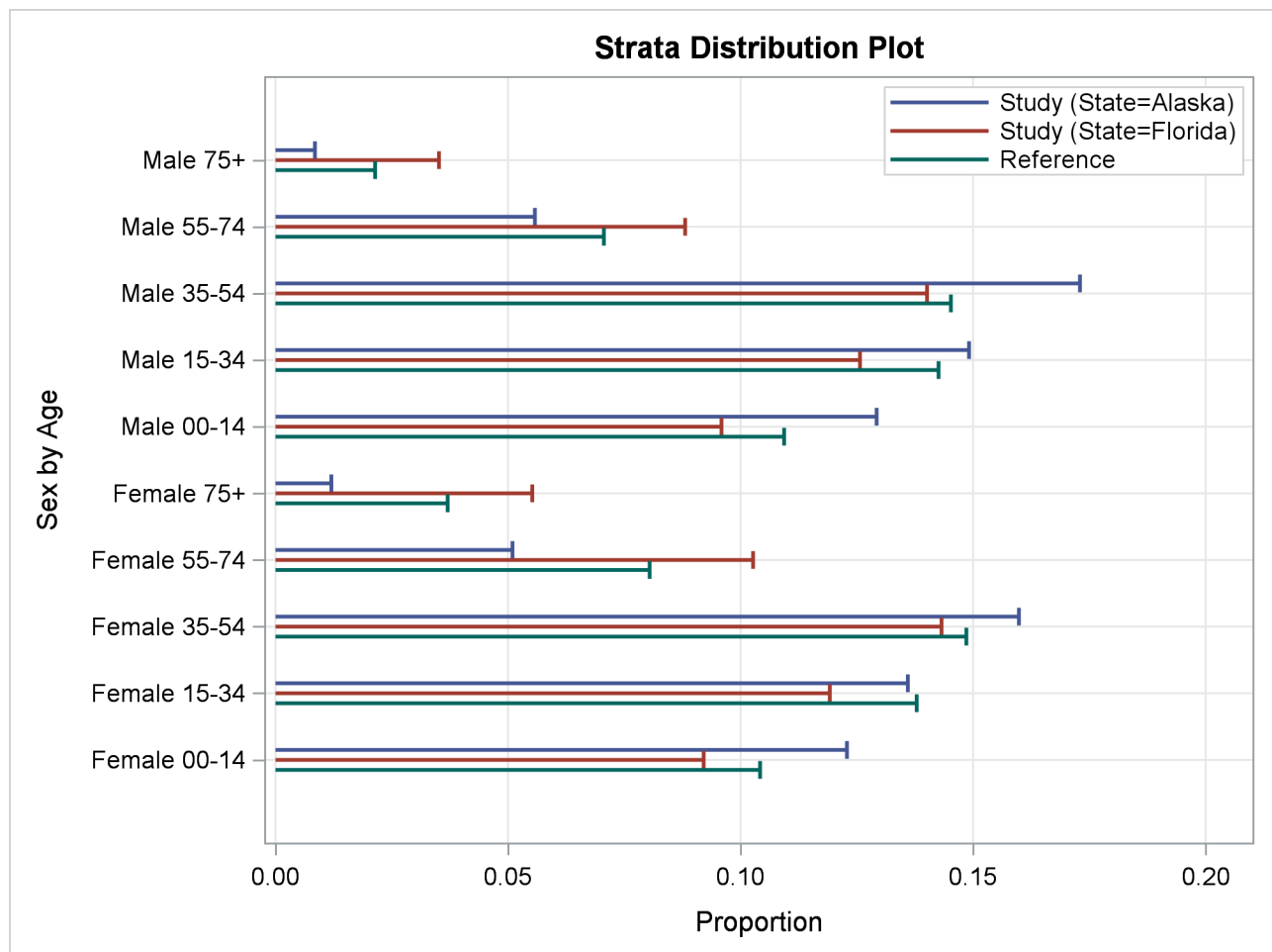
Output 107.1.2 Strata Distribution Plot
