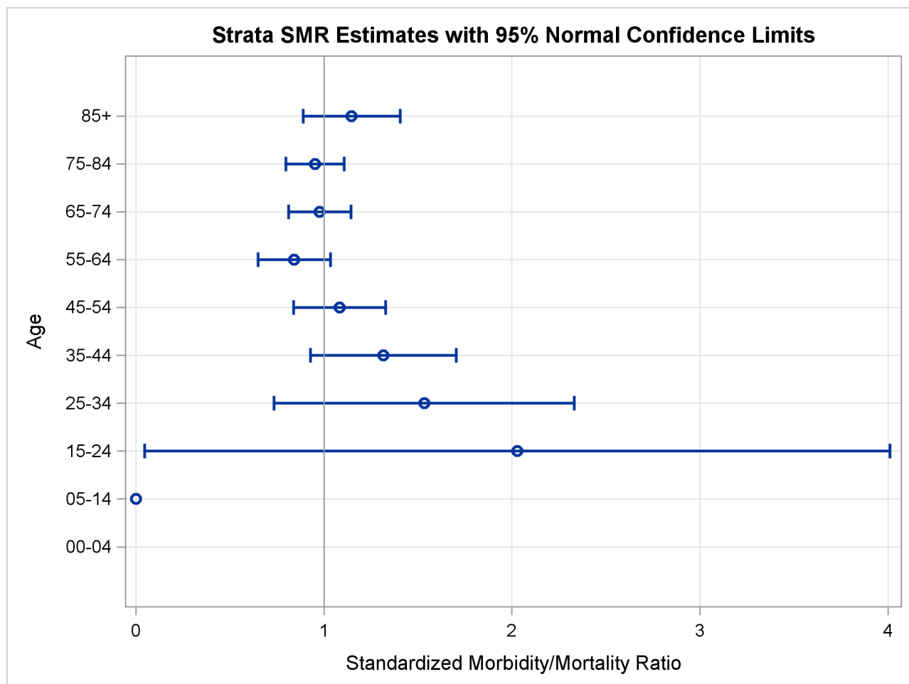
Figure 107.6 Strata SMR Plot
