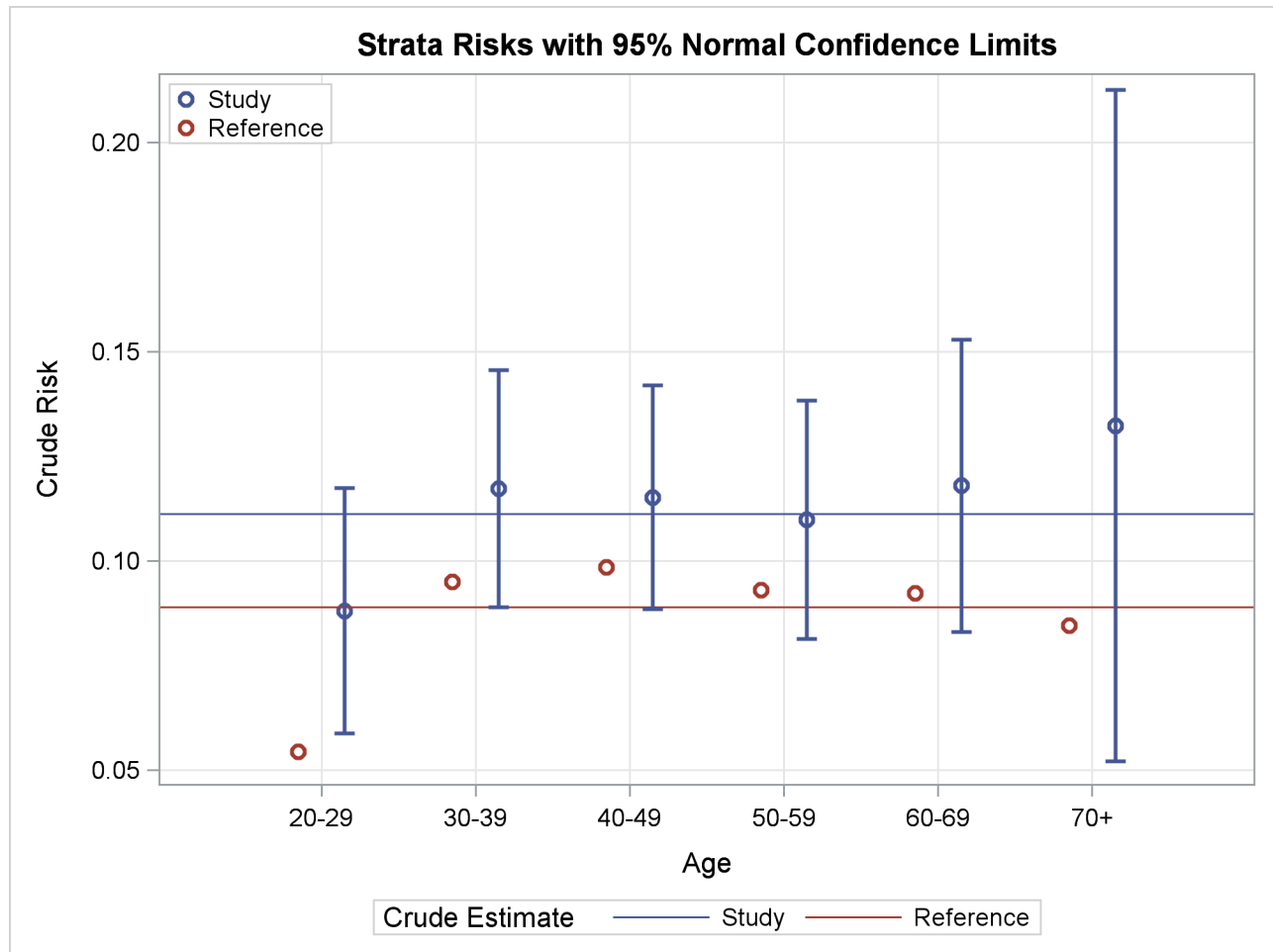
Output 107.3.3 Strata Risk Plot
