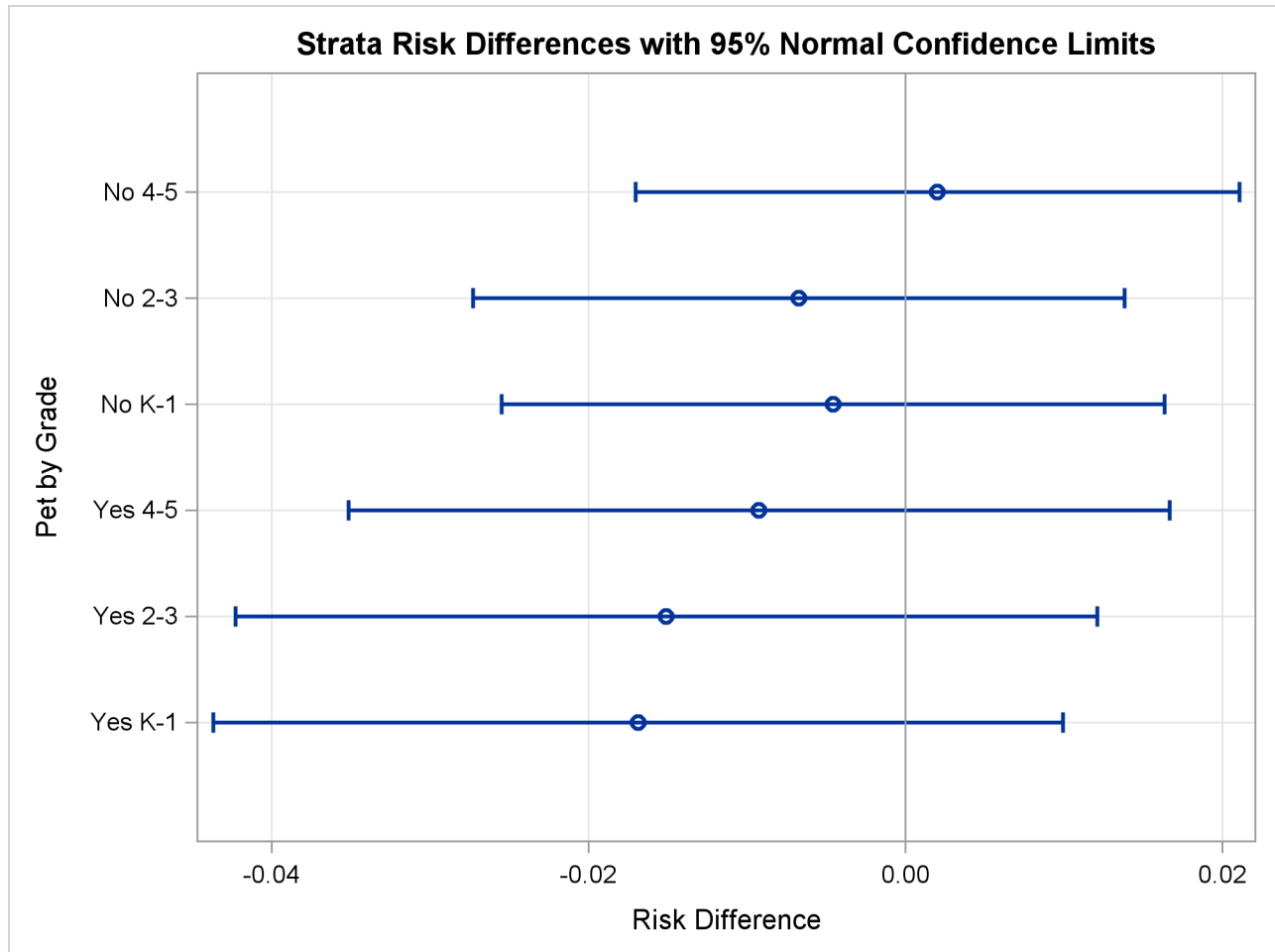
Output 107.2.6 Strata Risk Plot
