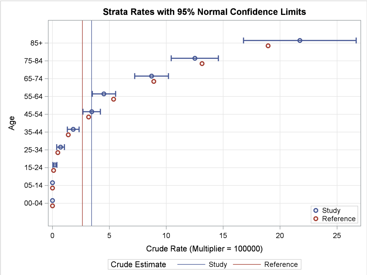
Figure 107.4 Strata Rate Plot
