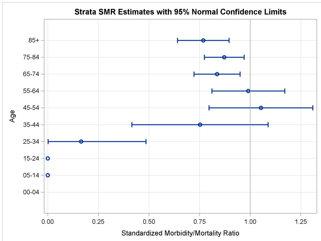
Output 107.4.7 Strata SMR Plot
