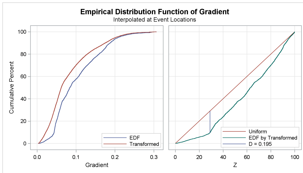
Output 105.2.2 Kolmogorov-Smirnov EDF Test Plot for Gradient
