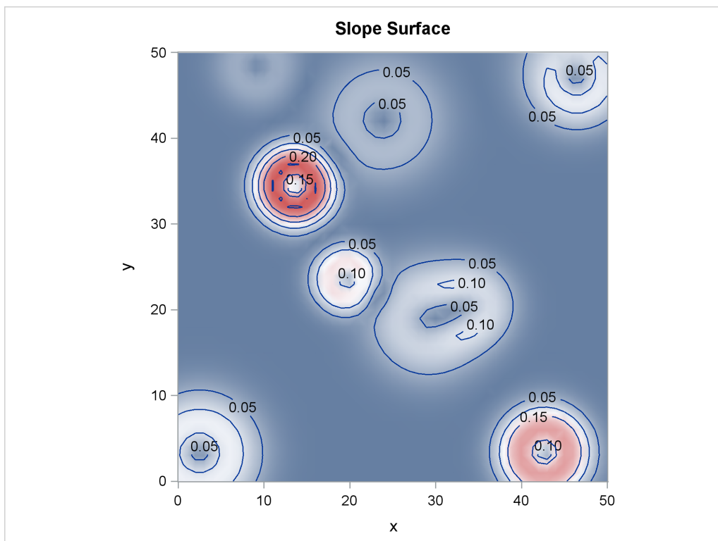
Output 105.3.3 Spatial Covariate Slope
