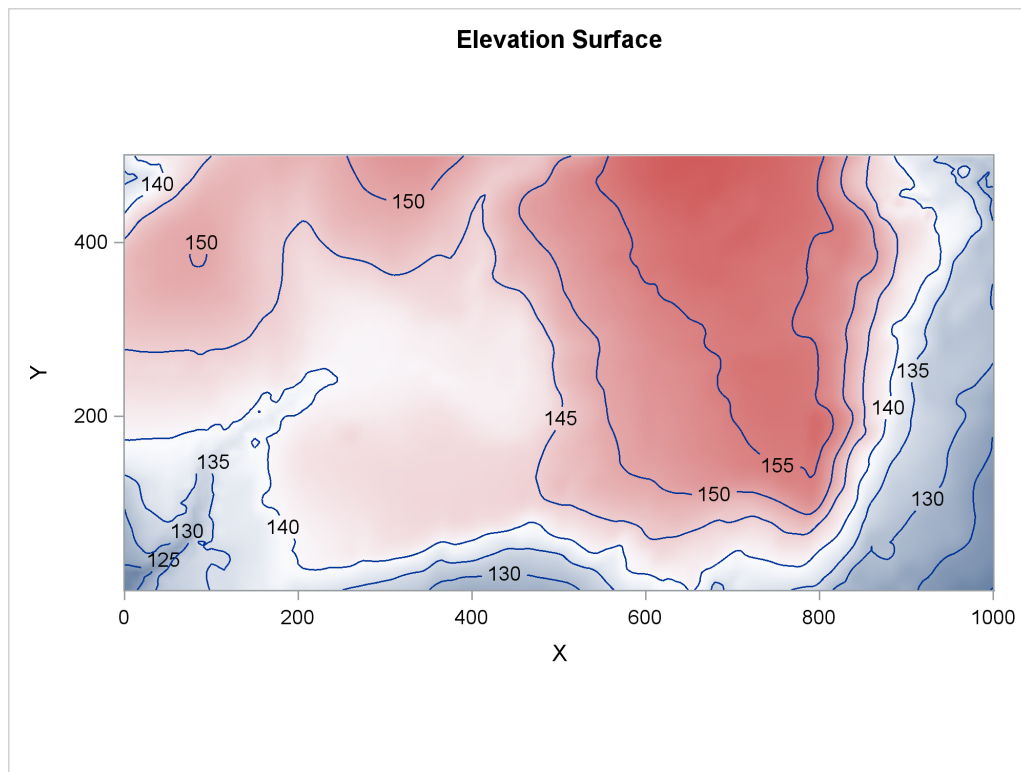
Figure 105.6 Spatial Covariate Elevation
