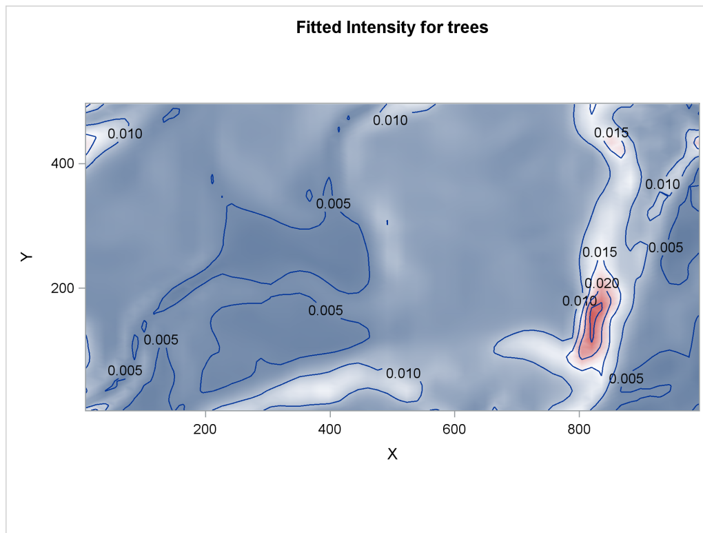
Figure 105.9 Intensity Estimates of Tree presence in Study Area
