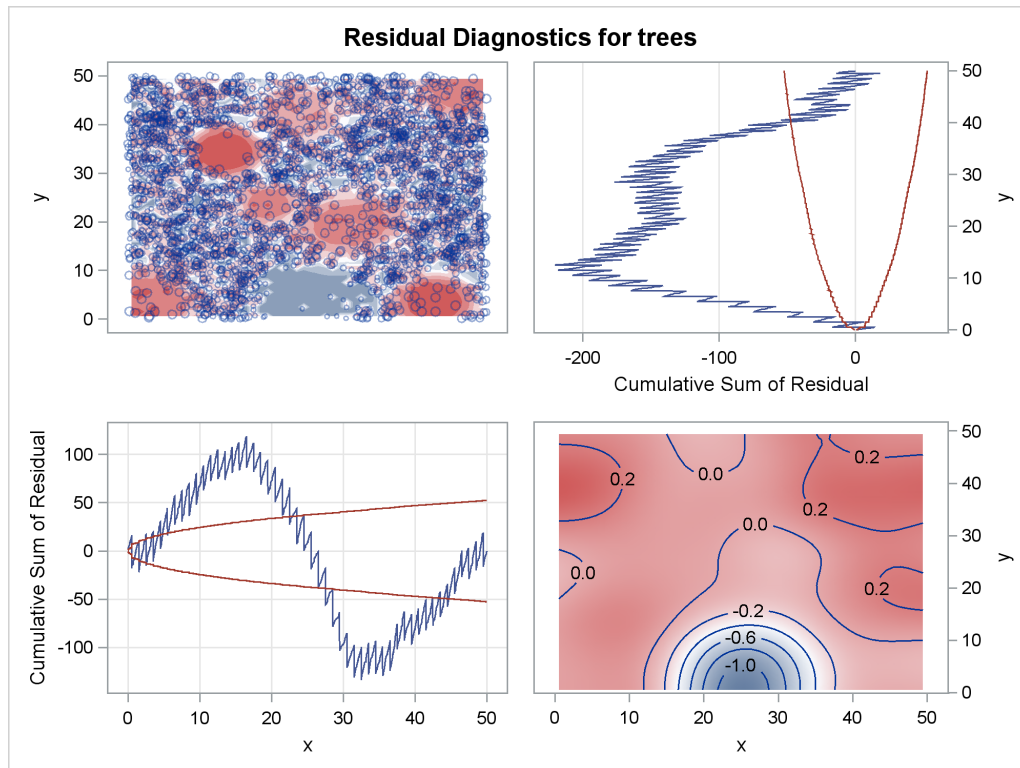
Output 105.3.5 Residual Diagnostics for the Fitted Model
