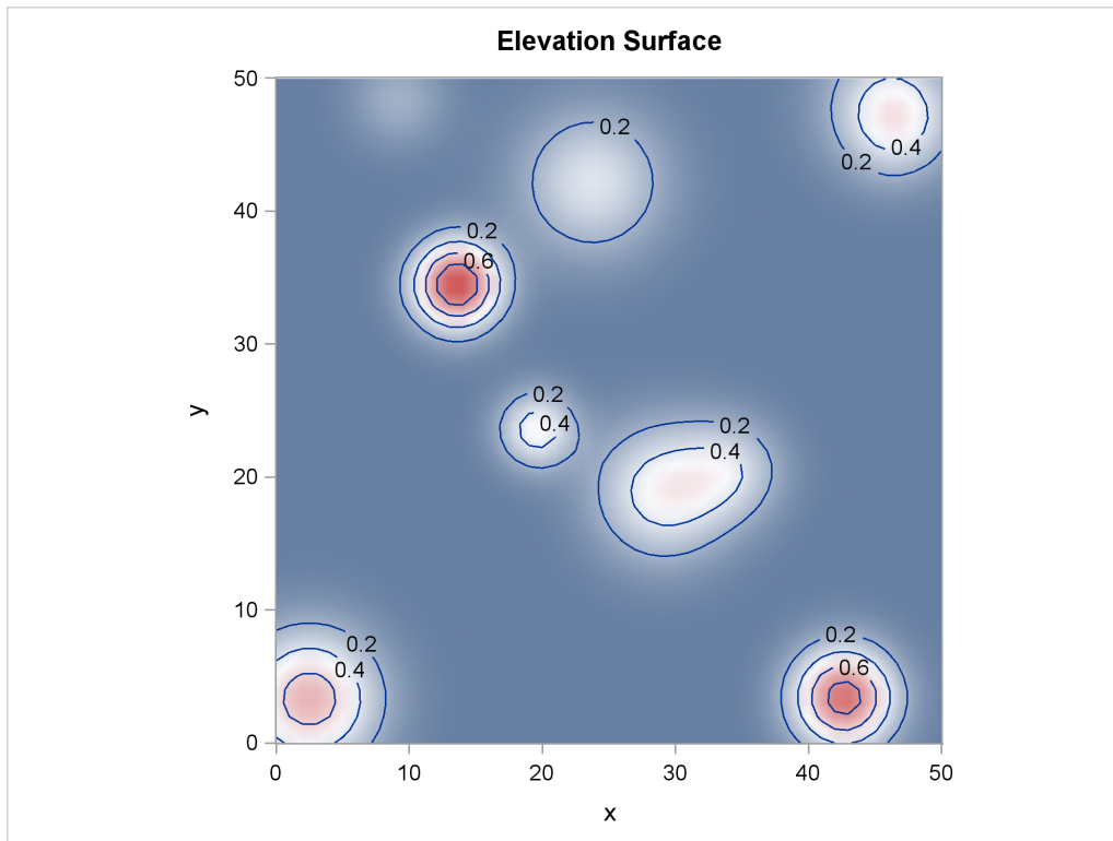
Output 105.3.2 Spatial Covariate Elevation
