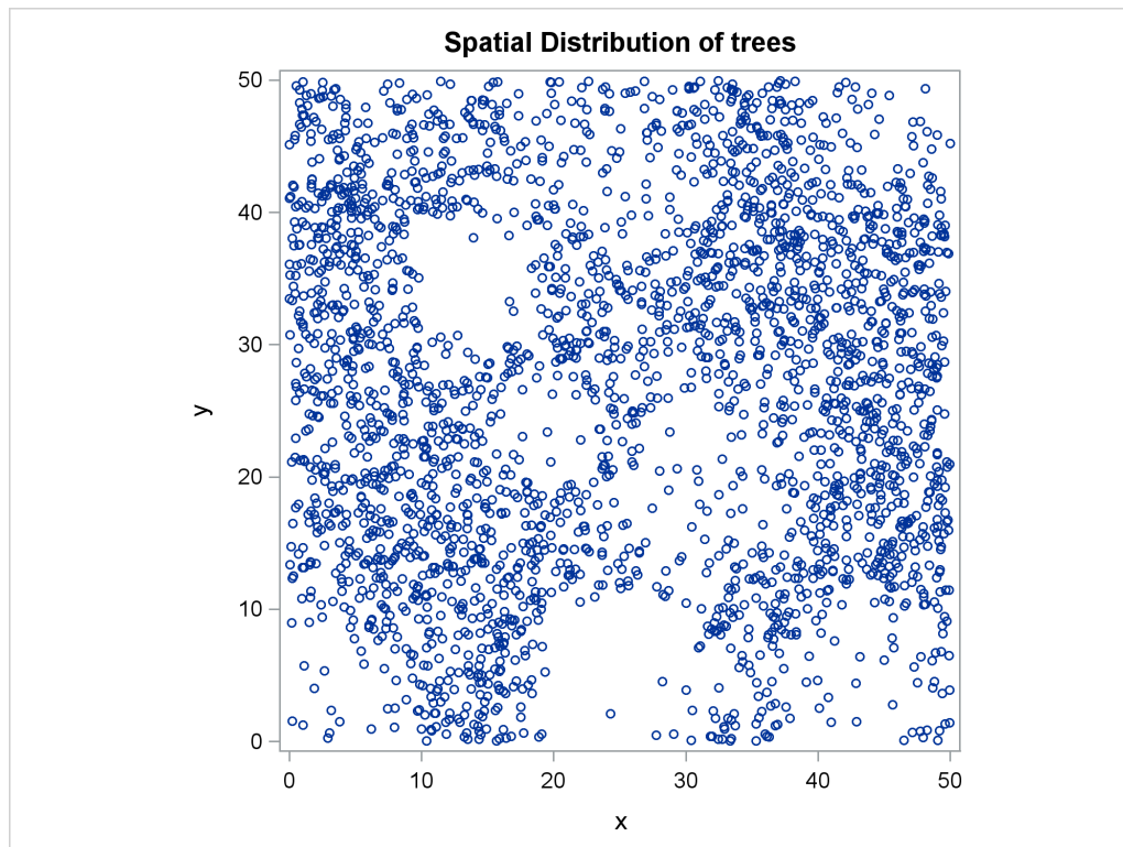
Output 105.3.1 Spatial Point Pattern of Simulated Flowers
