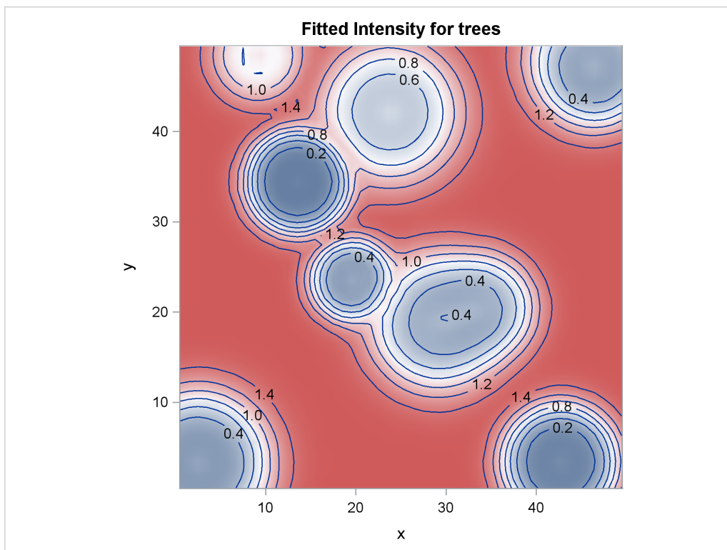
Output 105.3.4 Fitted Intensity Estimate for the Simulated Point Pattern
