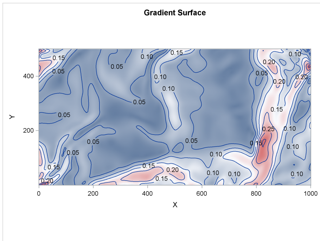
Figure 105.5 Spatial Covariate Gradient
