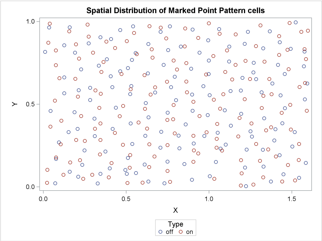
Output 105.1.1 Amacrine Cell Types
