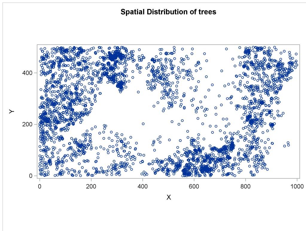
Figure 105.4 Spatial Point Pattern of Tropical Rain forest Trees
