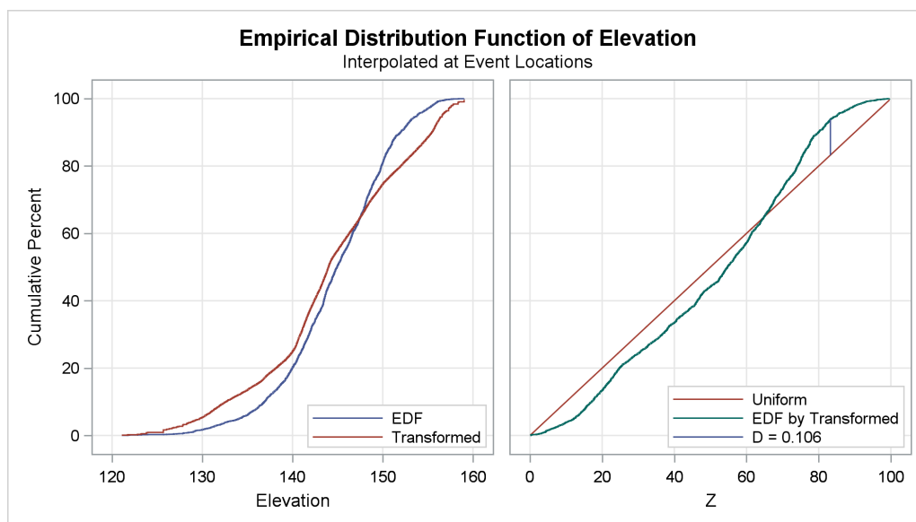
Output 105.2.3 Kolmogorov-Smirnov EDF Test Plot for Elevation
