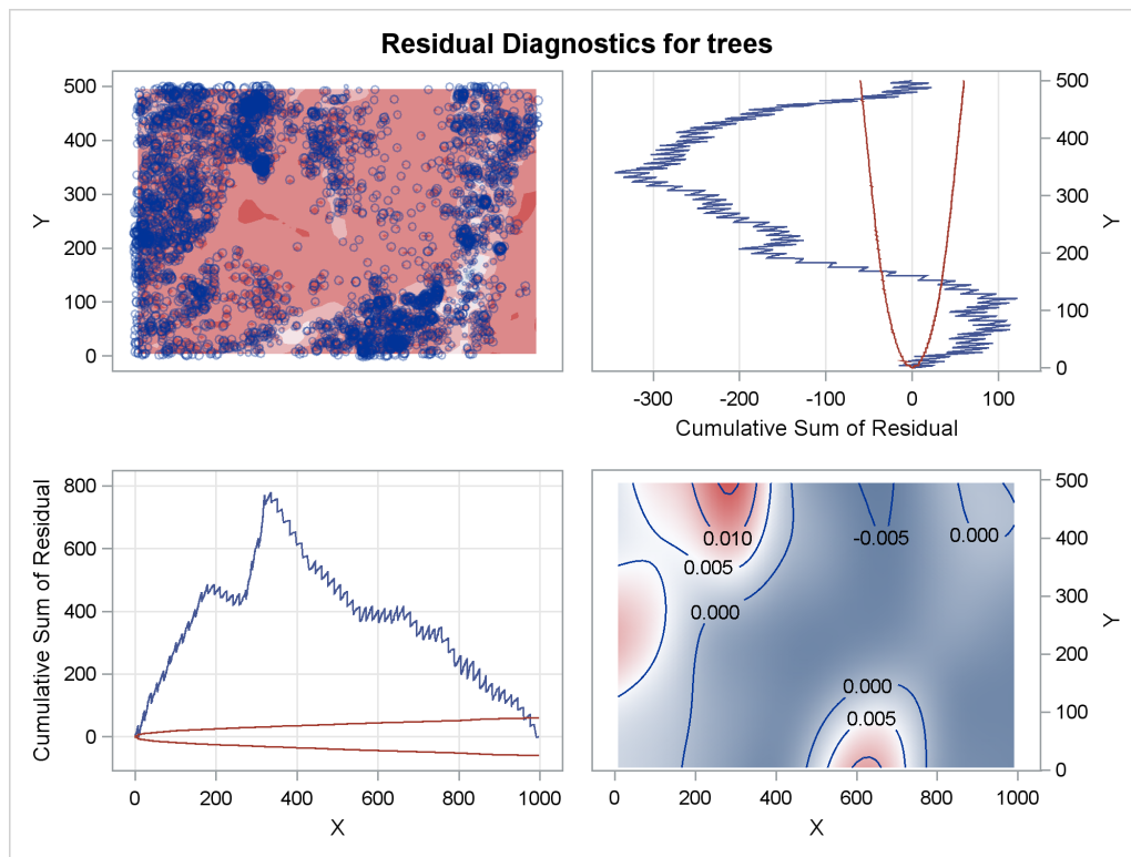
Figure 105.10 Residual Diagnostics for Fitted Log-Intensity Model
