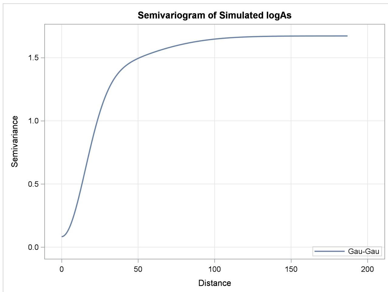
Output 103.3.6 Gaussian-Gaussian Semivariogram Model Used in Simulation
