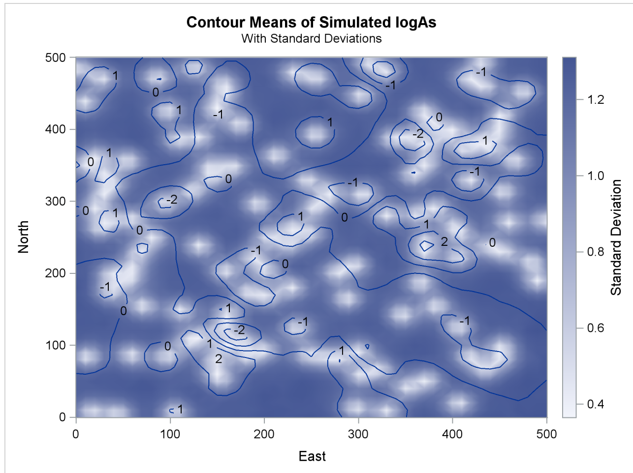
Output 103.3.7 Simulated Arsenic Logarithm Values with Gaussian-Gaussian Covariance
