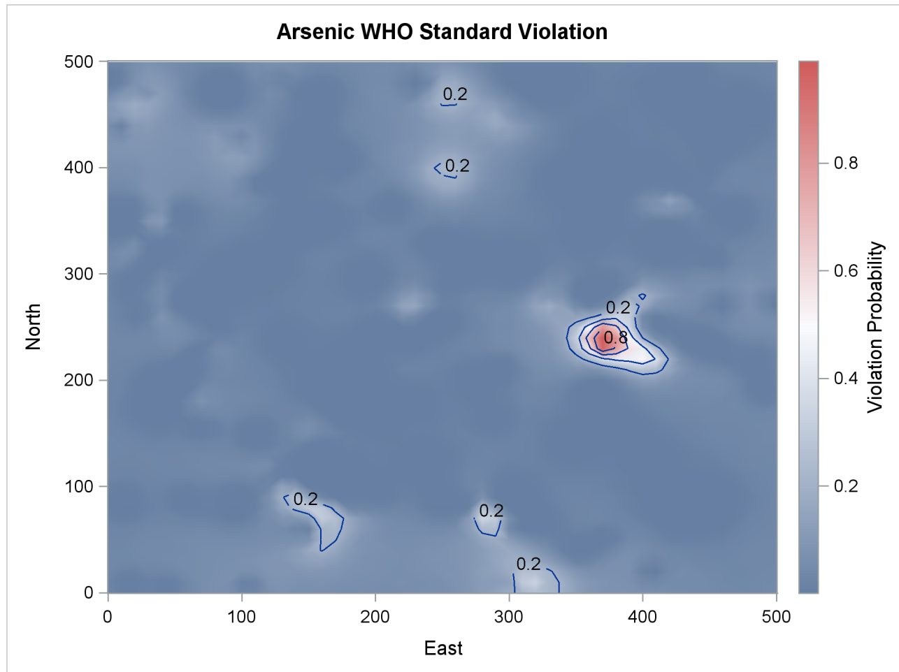
Output 103.3.9 Map of Violation of the Arsenic WHO Standard Probability
