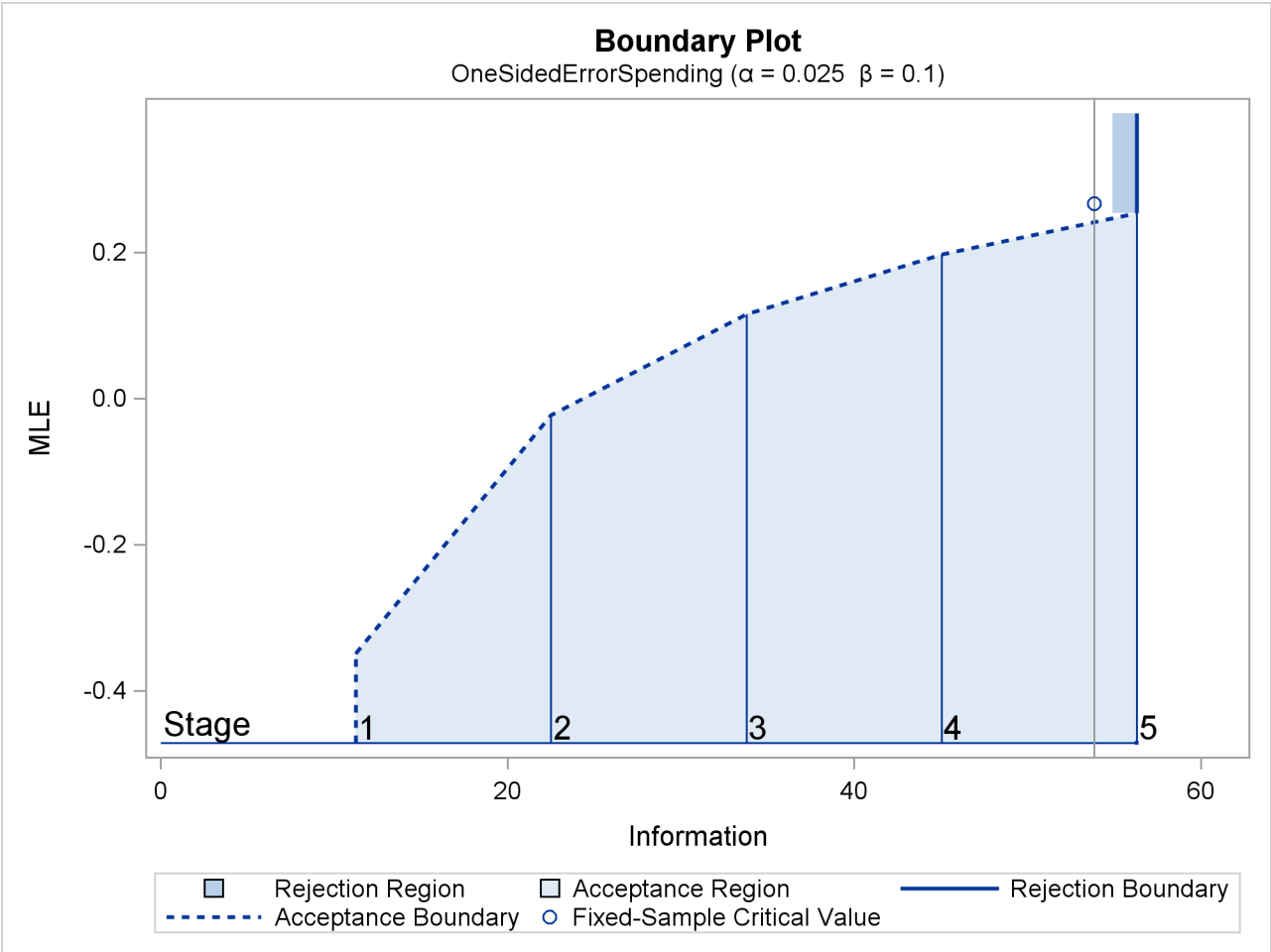
Output 102.5.3 Boundary Plot
