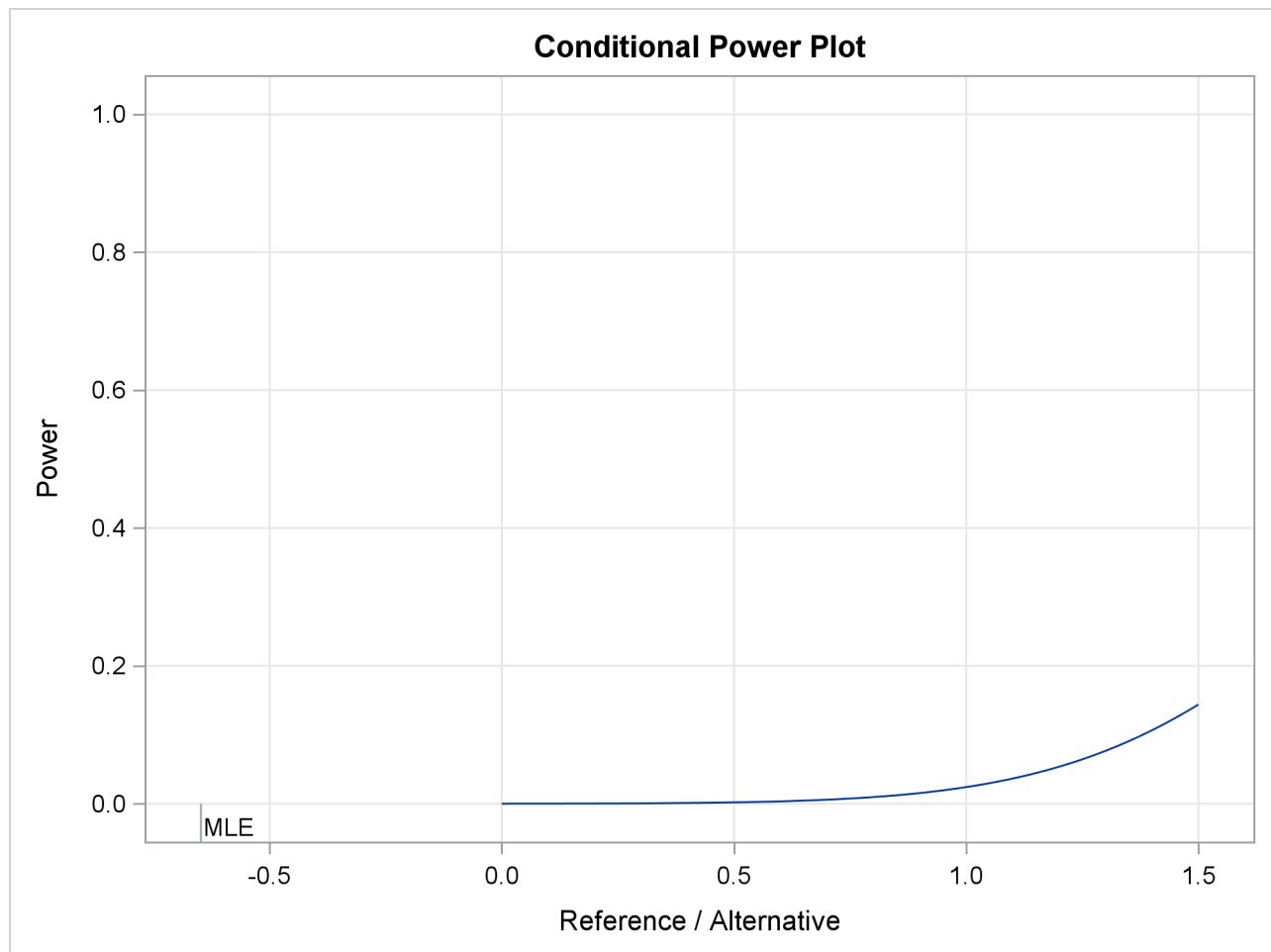
Output 102.4.16 Conditional Power Plot
