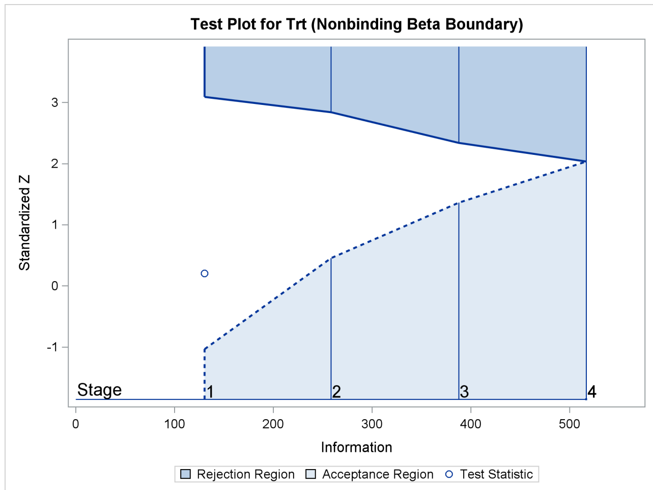
Output 102.9.13 Sequential Test Plot
