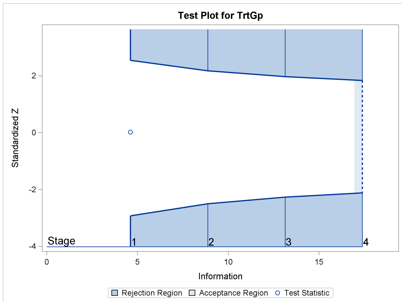
Output 102.7.12 Sequential Test Plot
