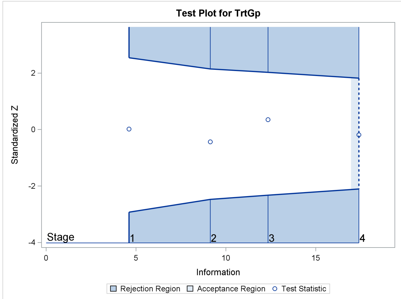
Output 102.7.16 Sequential Test Plot
