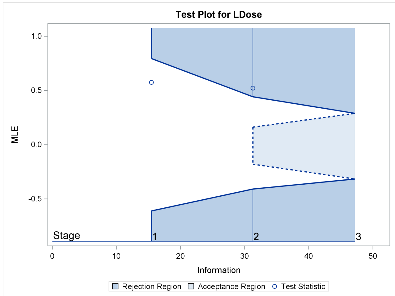
Output 102.8.14 Sequential Test Plot
