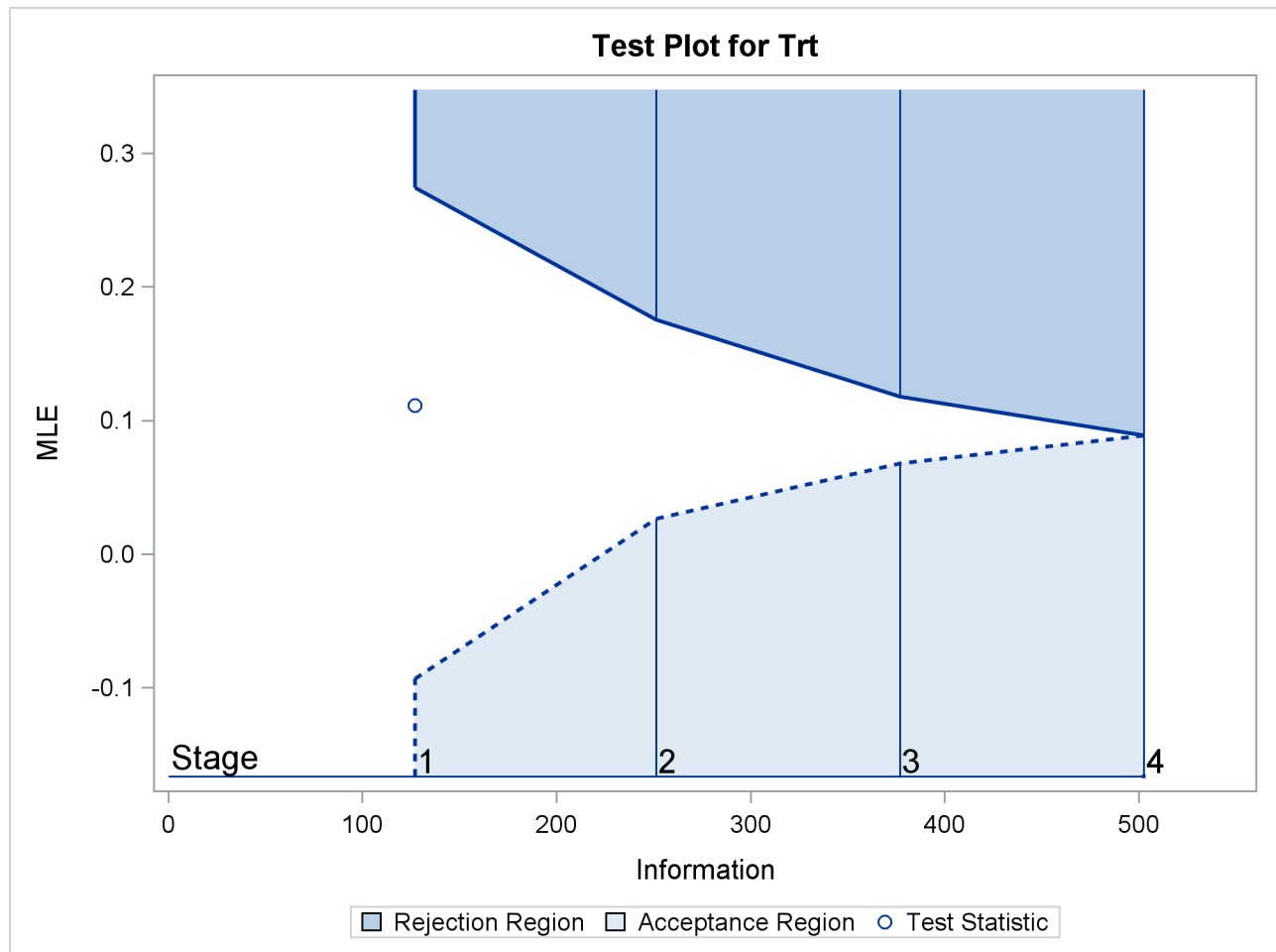
Output 102.1.13 Sequential Test Plot
