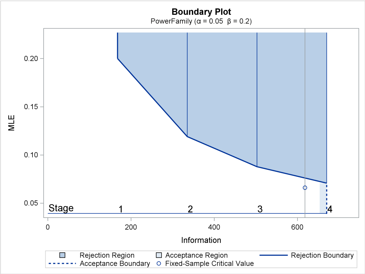
Output 102.4.3 Boundary Plot
