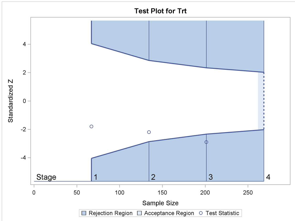
Figure 102.1 Sequential Plot for Two-Sided Test
