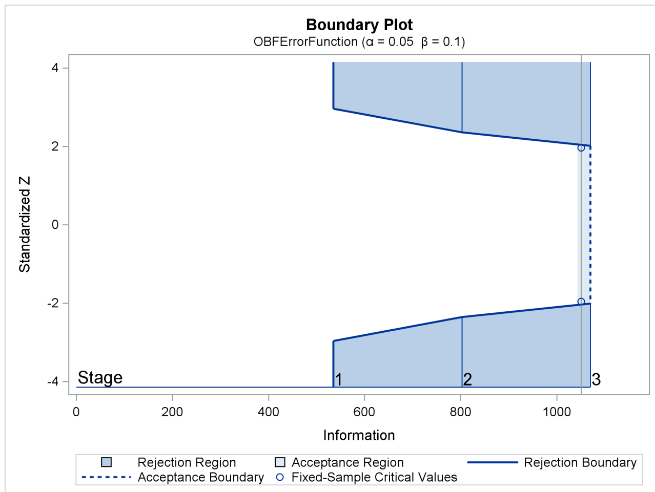
Output 102.2.3 Boundary Plot
