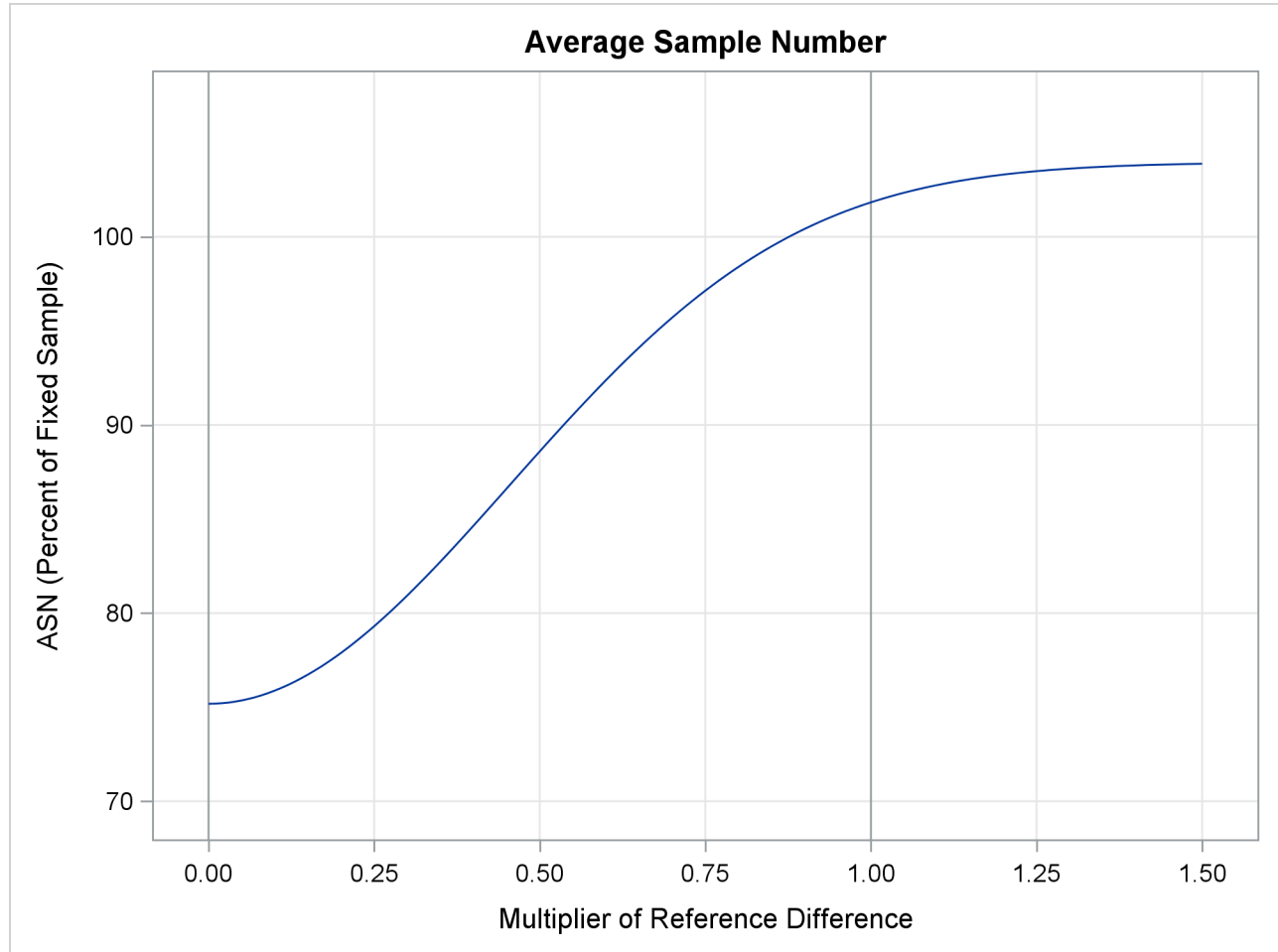
Output 102.3.15 ASN Plot
