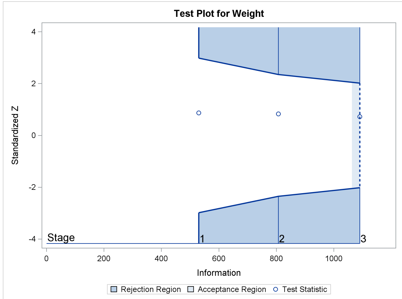
Output 102.2.19 Sequential Test Plot
