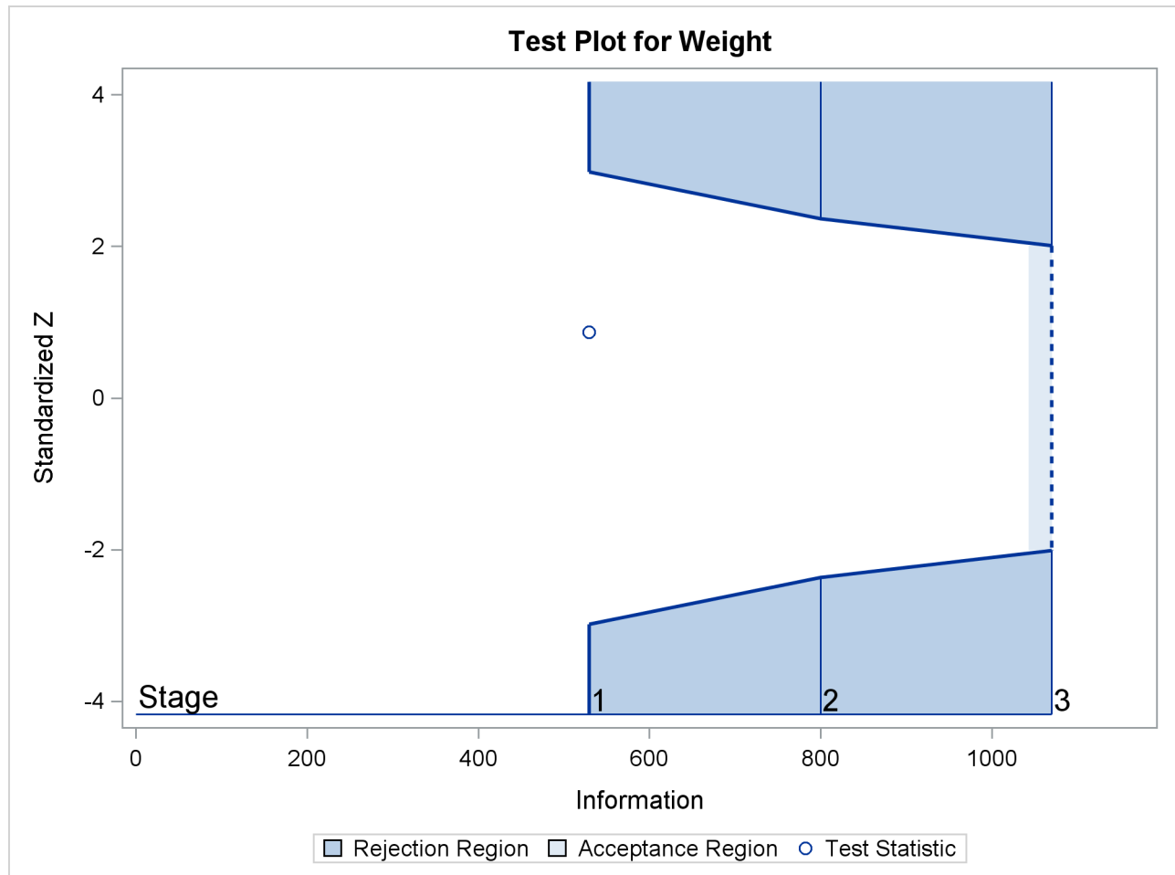
Output 102.2.11 Sequential Test Plot
