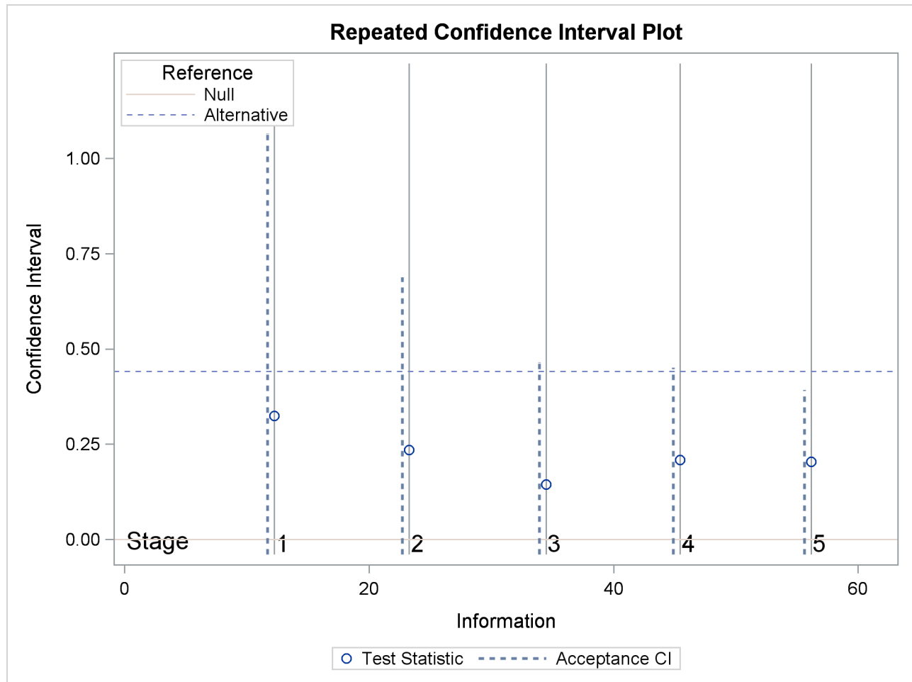
Output 102.5.18 Repeated Confidence Intervals Plot
