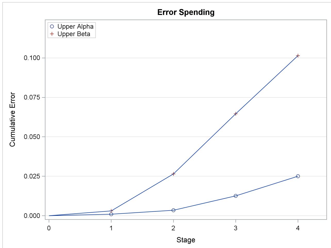
Output 102.1.11 Error Spending Plot
