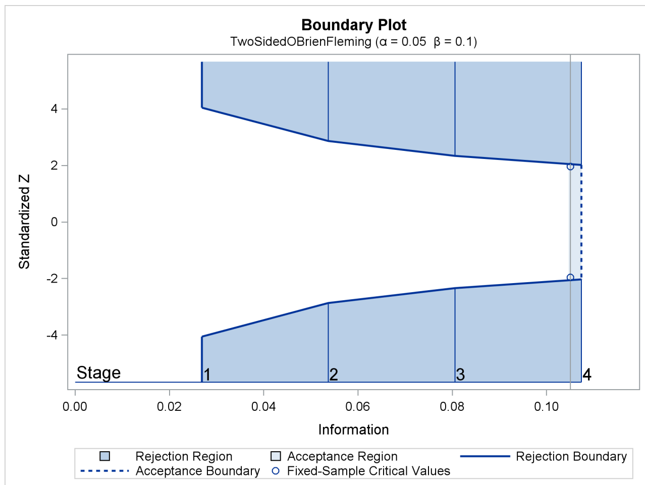
Figure 102.5 O'Brien-Fleming Boundary Plot
