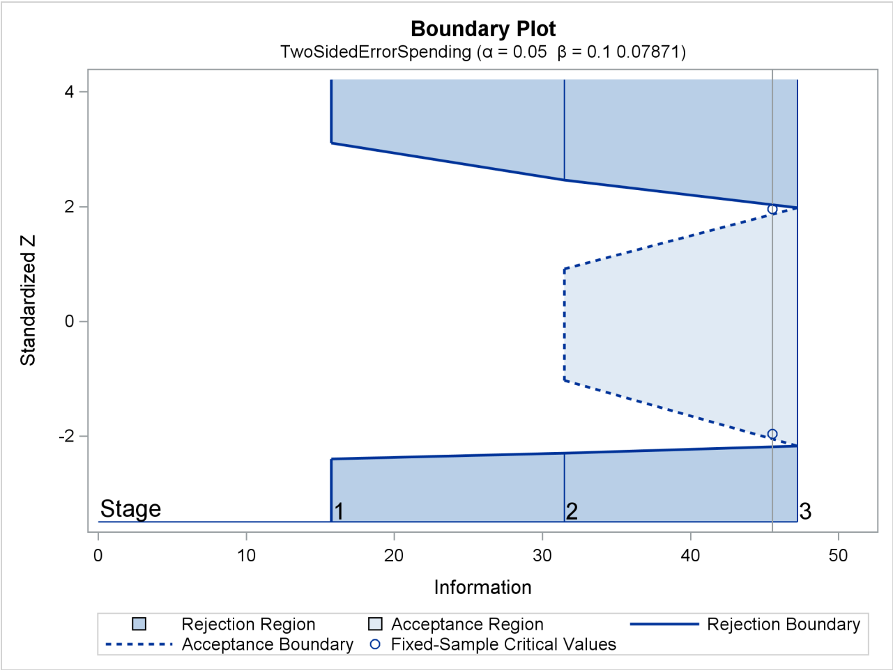
Output 102.8.3 Boundary Plot
