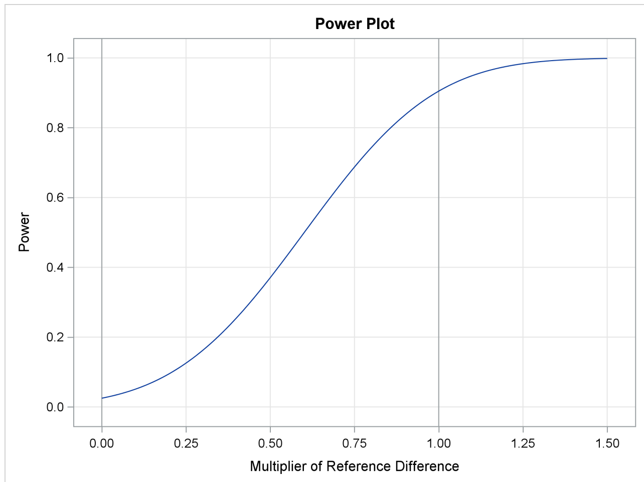
Output 102.2.17 Power Plot
