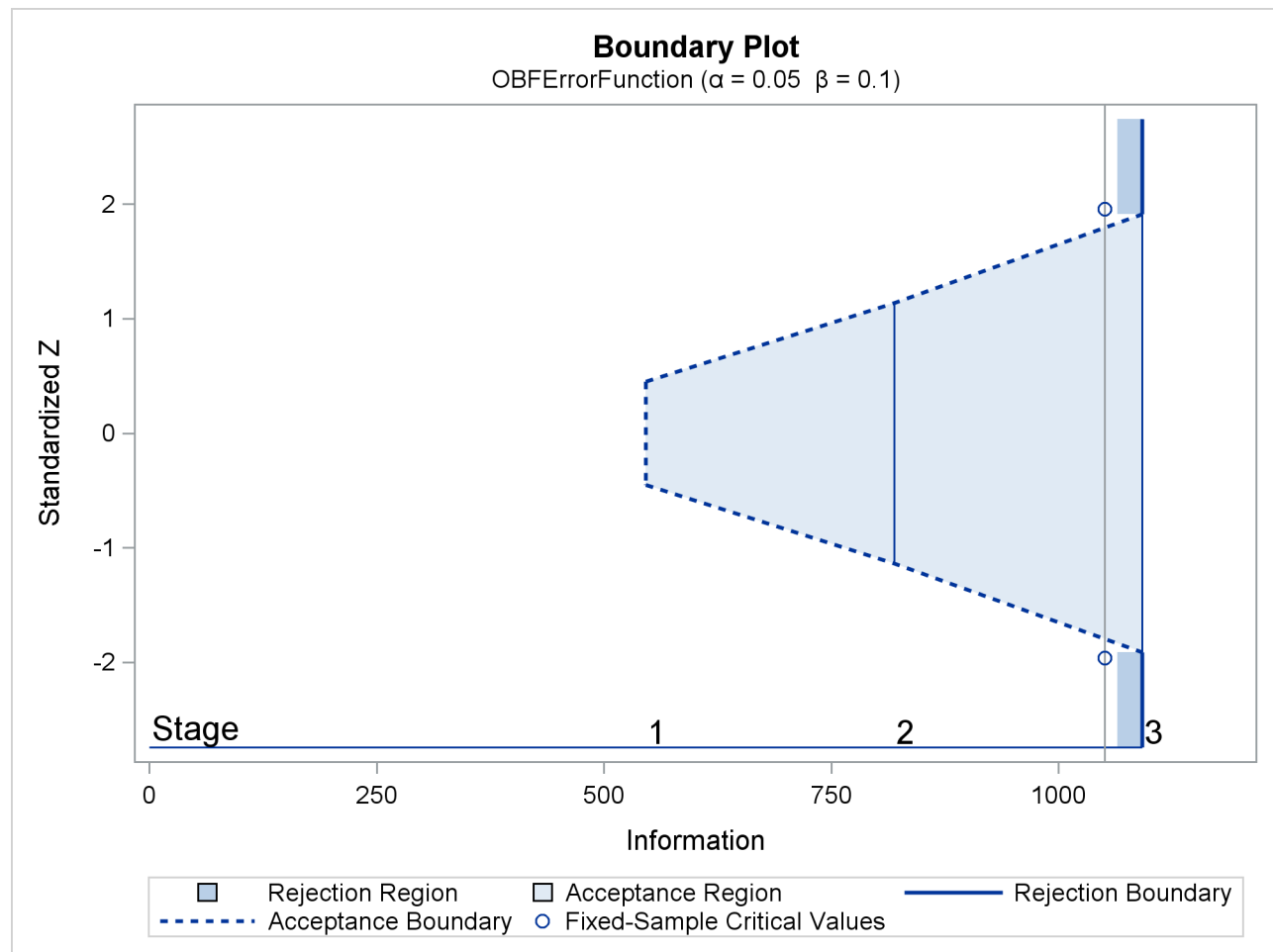
Output 102.3.3 Boundary Plot
