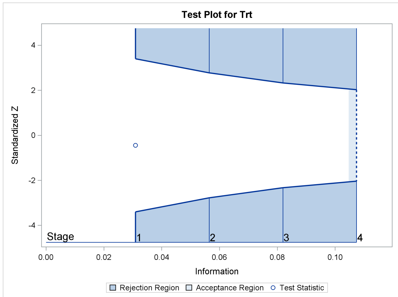
Figure 102.12 Sequential Test Plot
