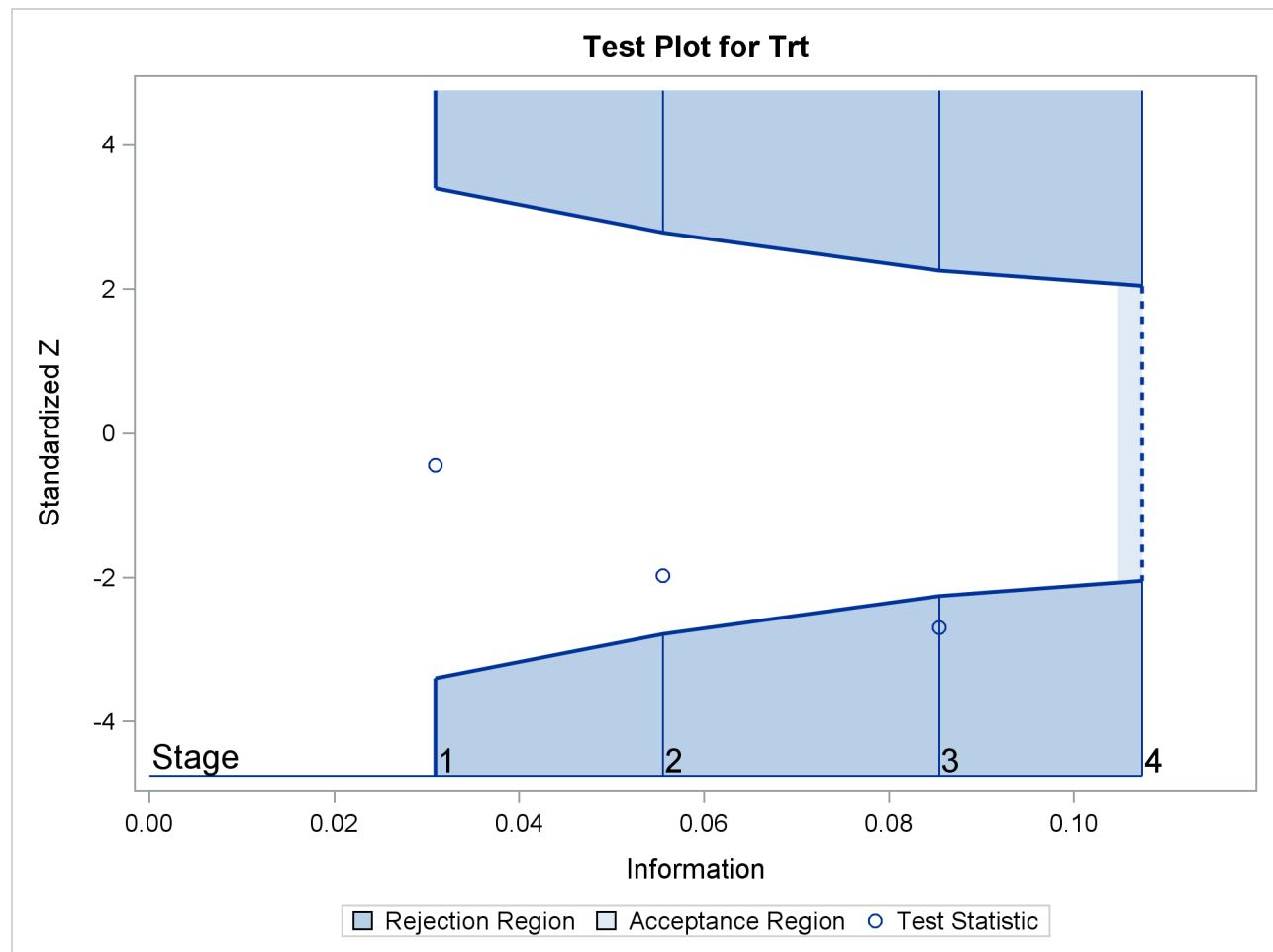
Figure 102.17 Sequential Test Plot
