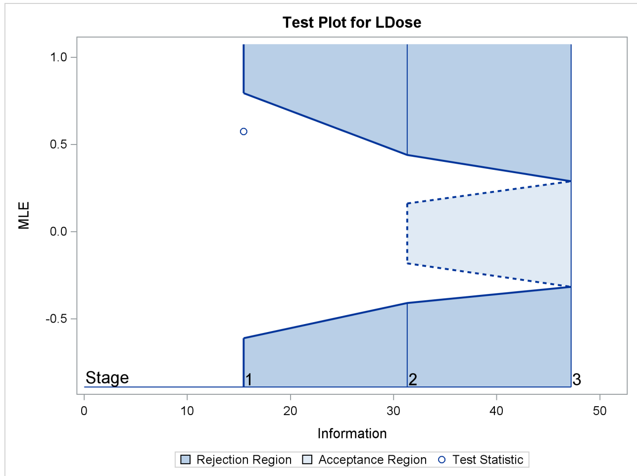
Output 102.8.10 Sequential Test Plot
