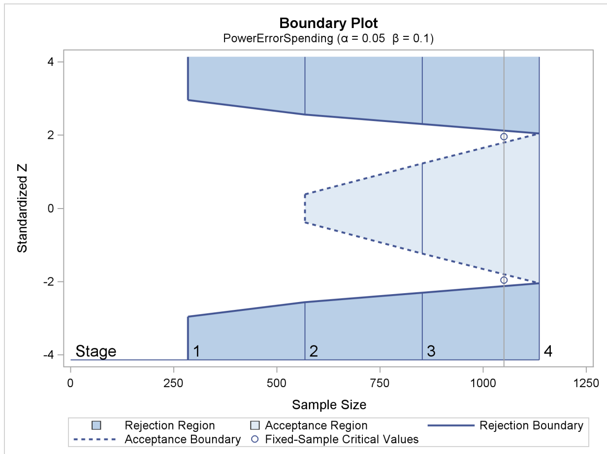
Figure 102.20 Boundary Plot for Two-Sided Test
