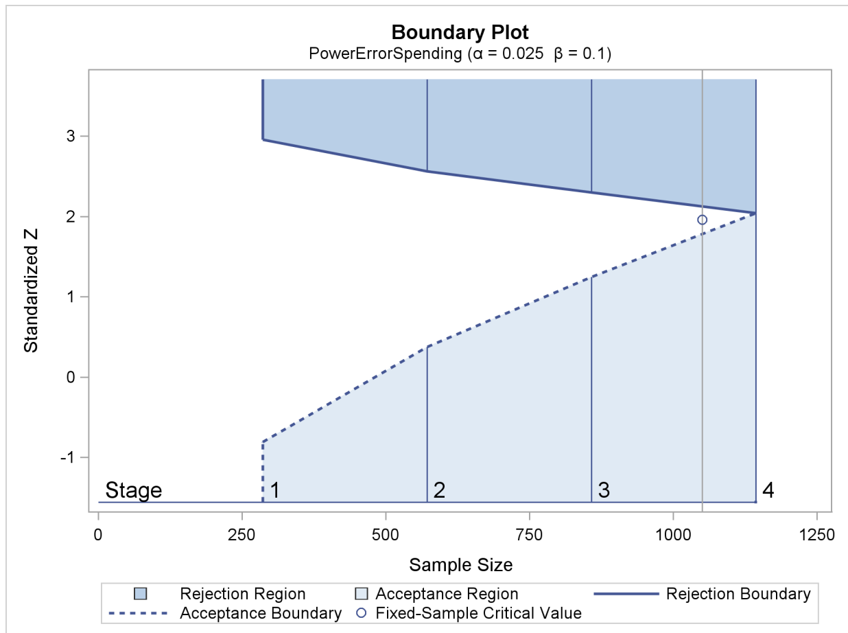
Figure 102.19 Boundary Plot for One-Sided Test
