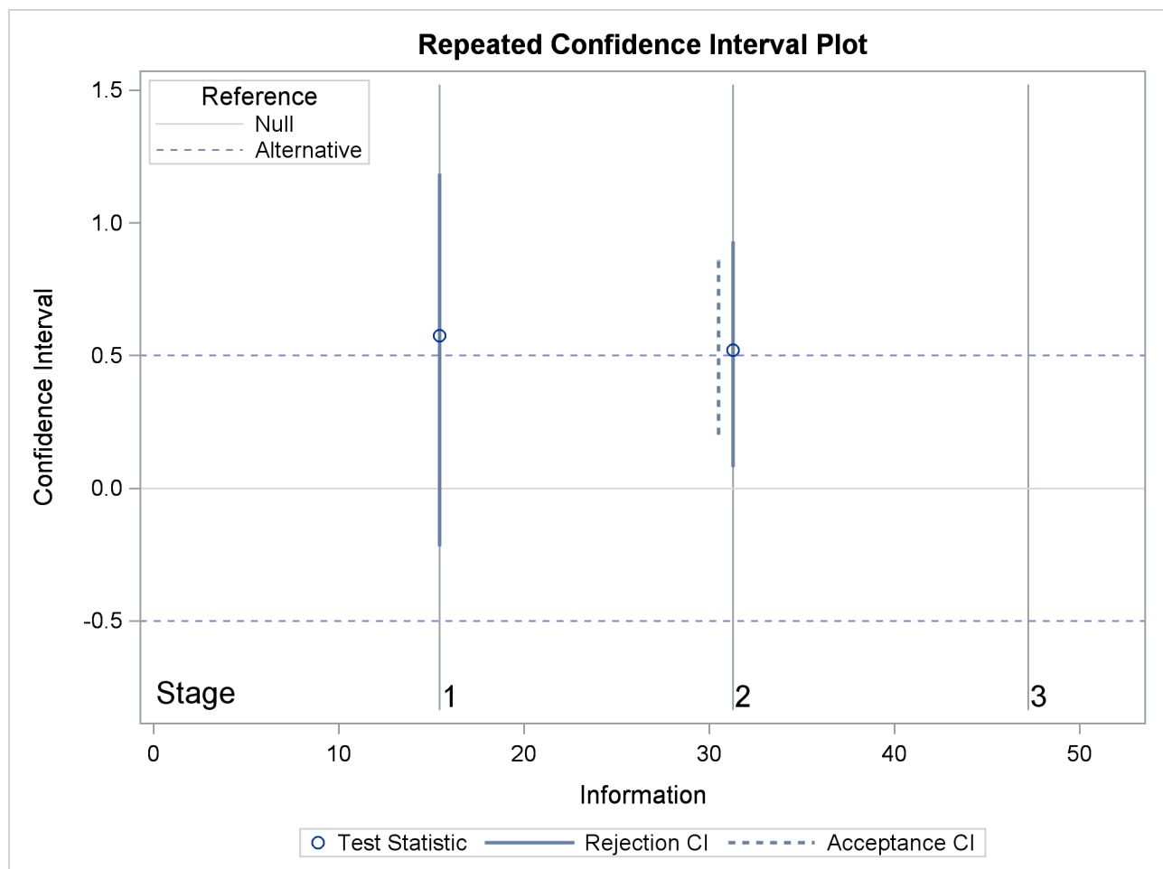
Output 102.8.17 Repeated Confidence Intervals Plot
