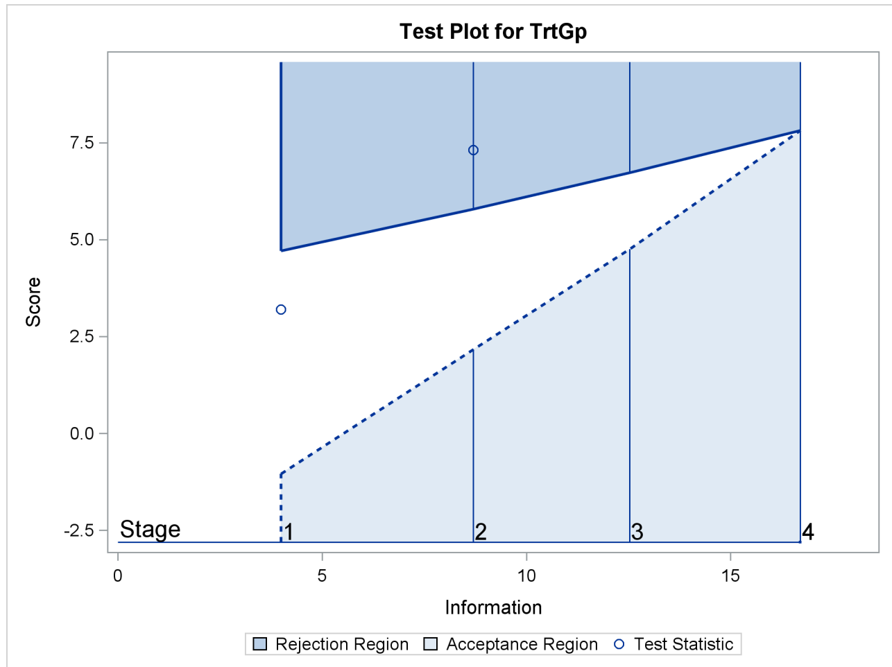
Output 102.6.16 Sequential Test Plot
