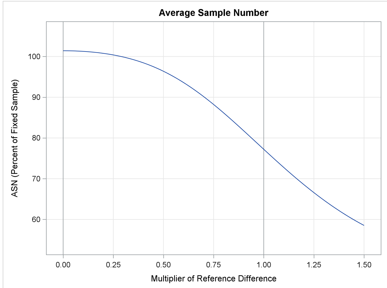
Output 102.2.16 ASN Plot
