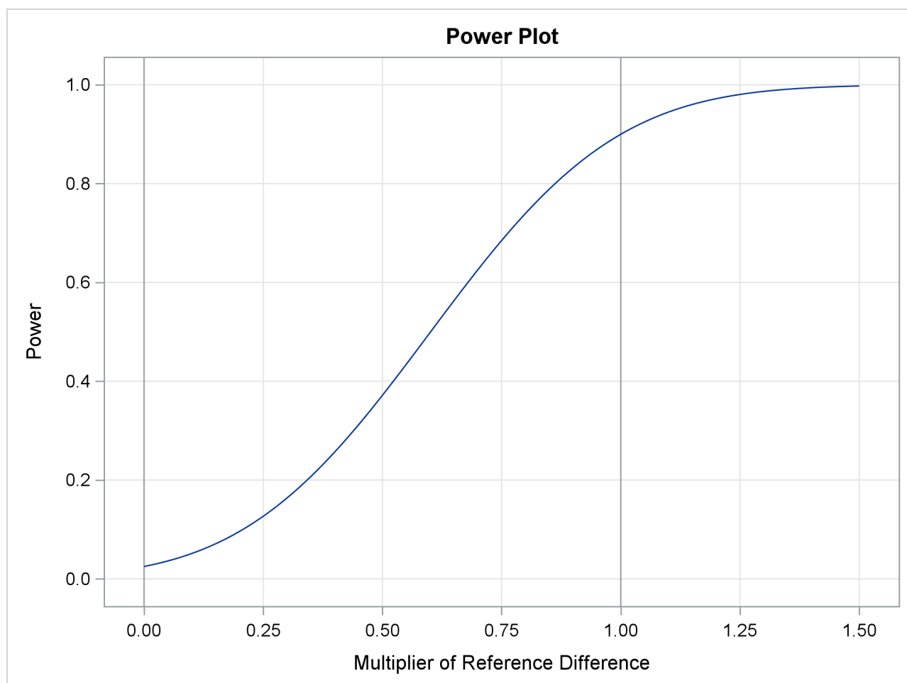
Output 102.3.16 Power Plot
