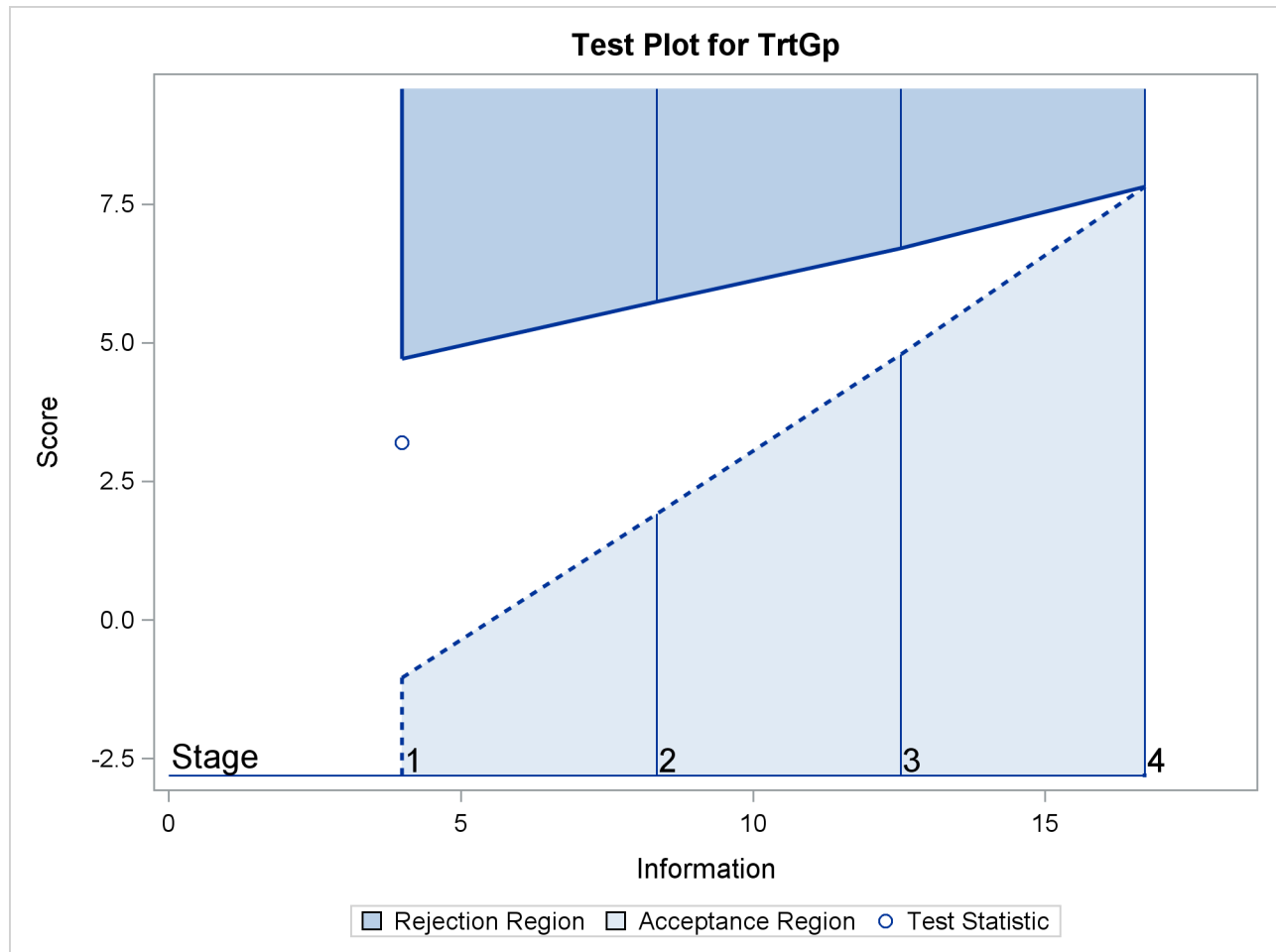
Output 102.6.12 Sequential Test Plot
