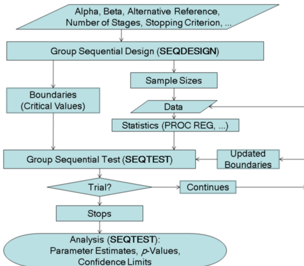
Figure 102.2 Group Sequential Trial
