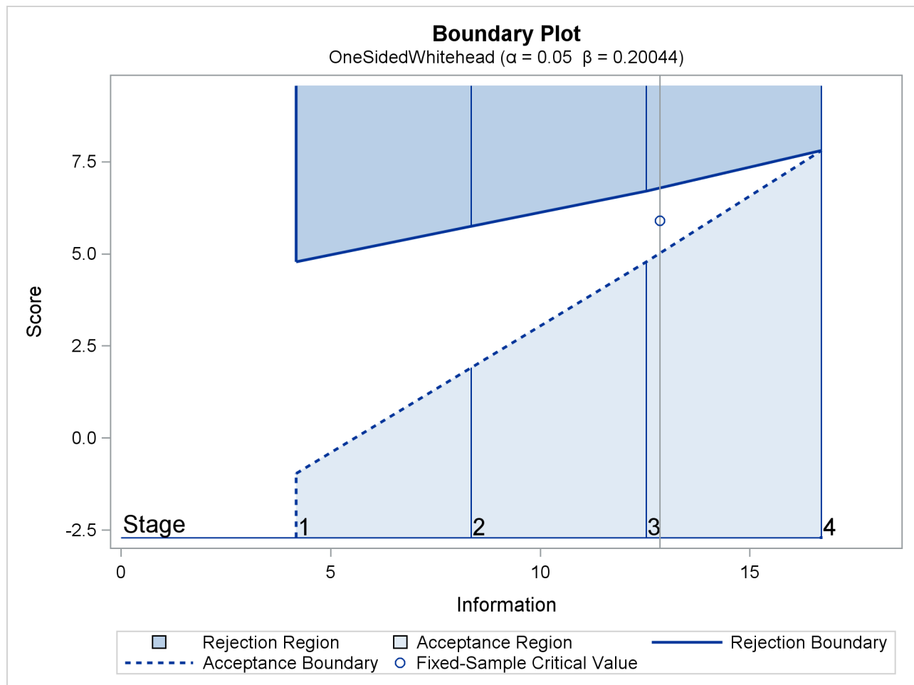
Output 102.6.3 Boundary Plot
