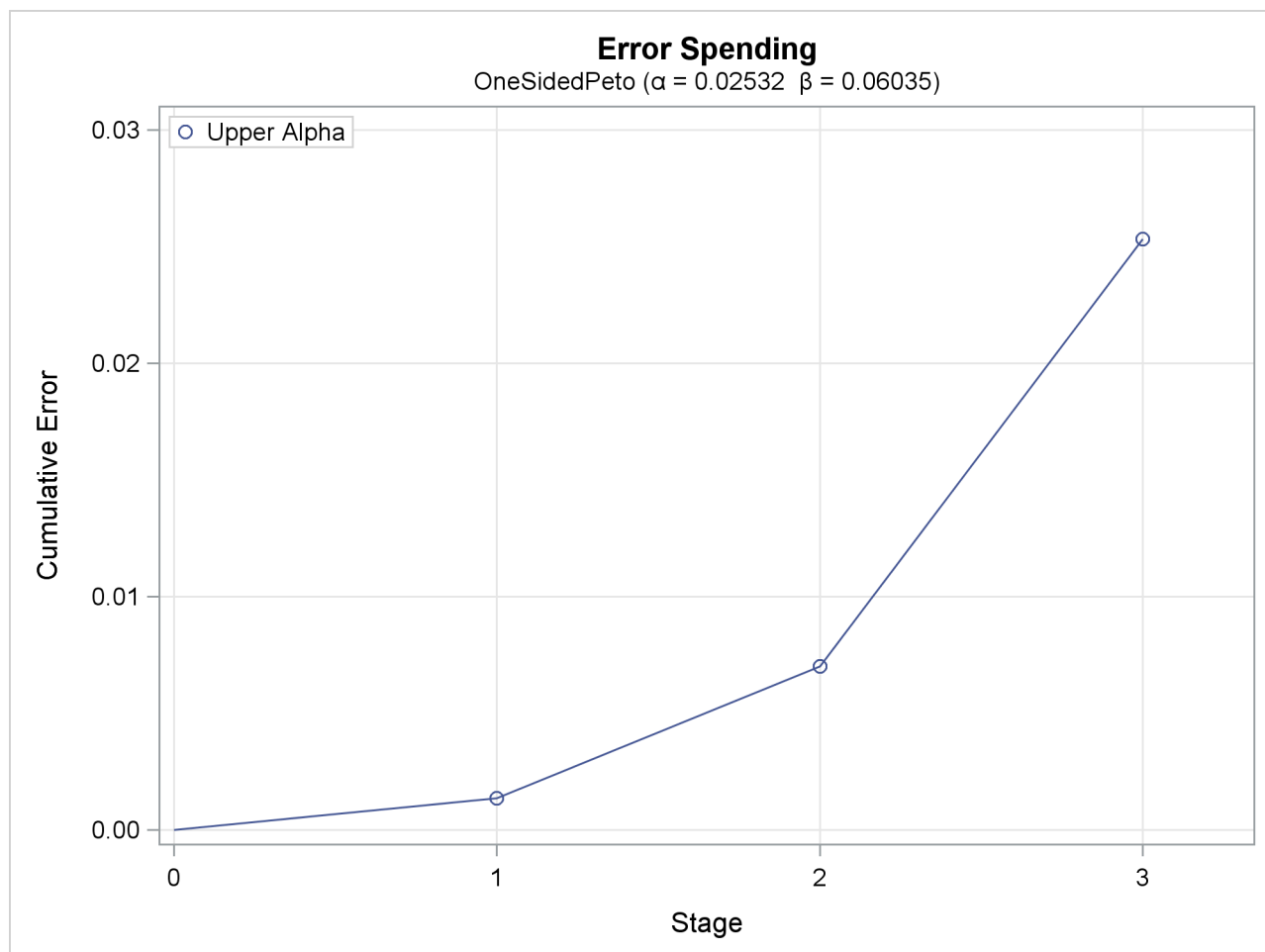
Output 101.5.14 Error Spending Plot
