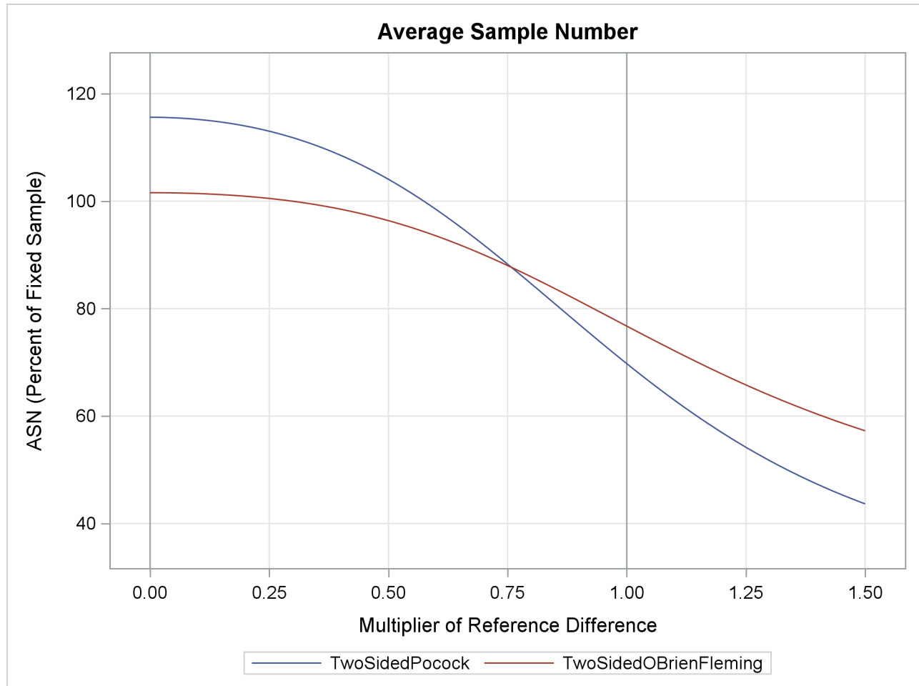
Output 101.4.3 ASN Plot
