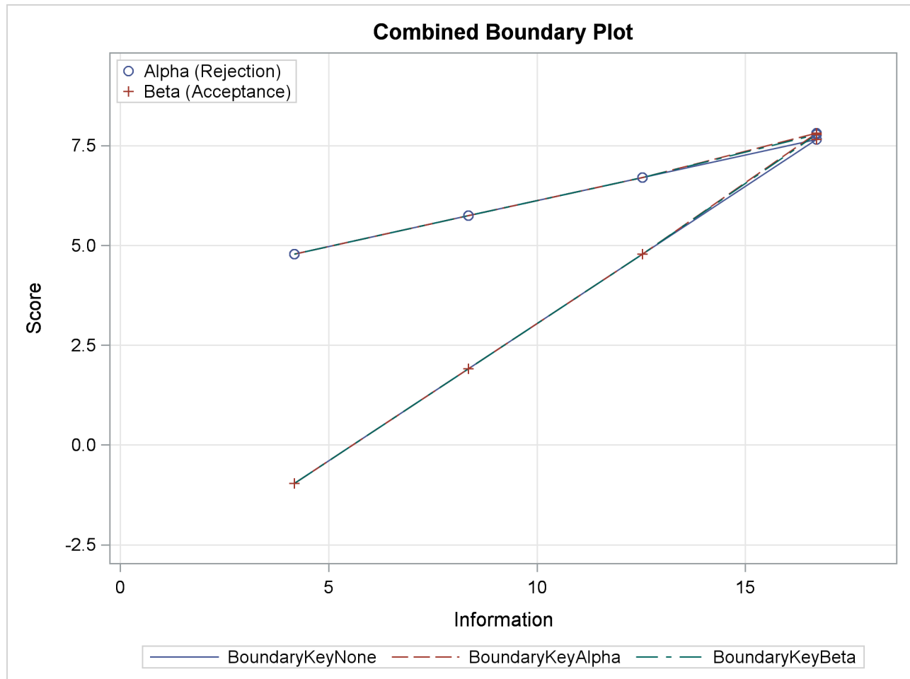
Output 101.7.13 Combined Boundary Plot
