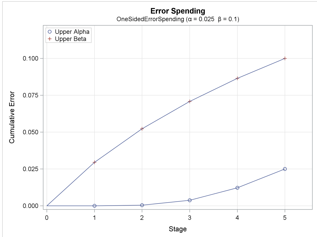
Output 101.8.10 Error Spending Plot
