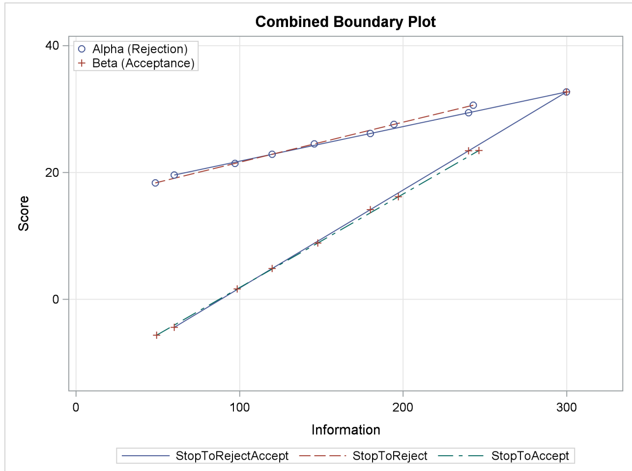
Output 101.6.16 Combined Boundary Plot with Score Scale
