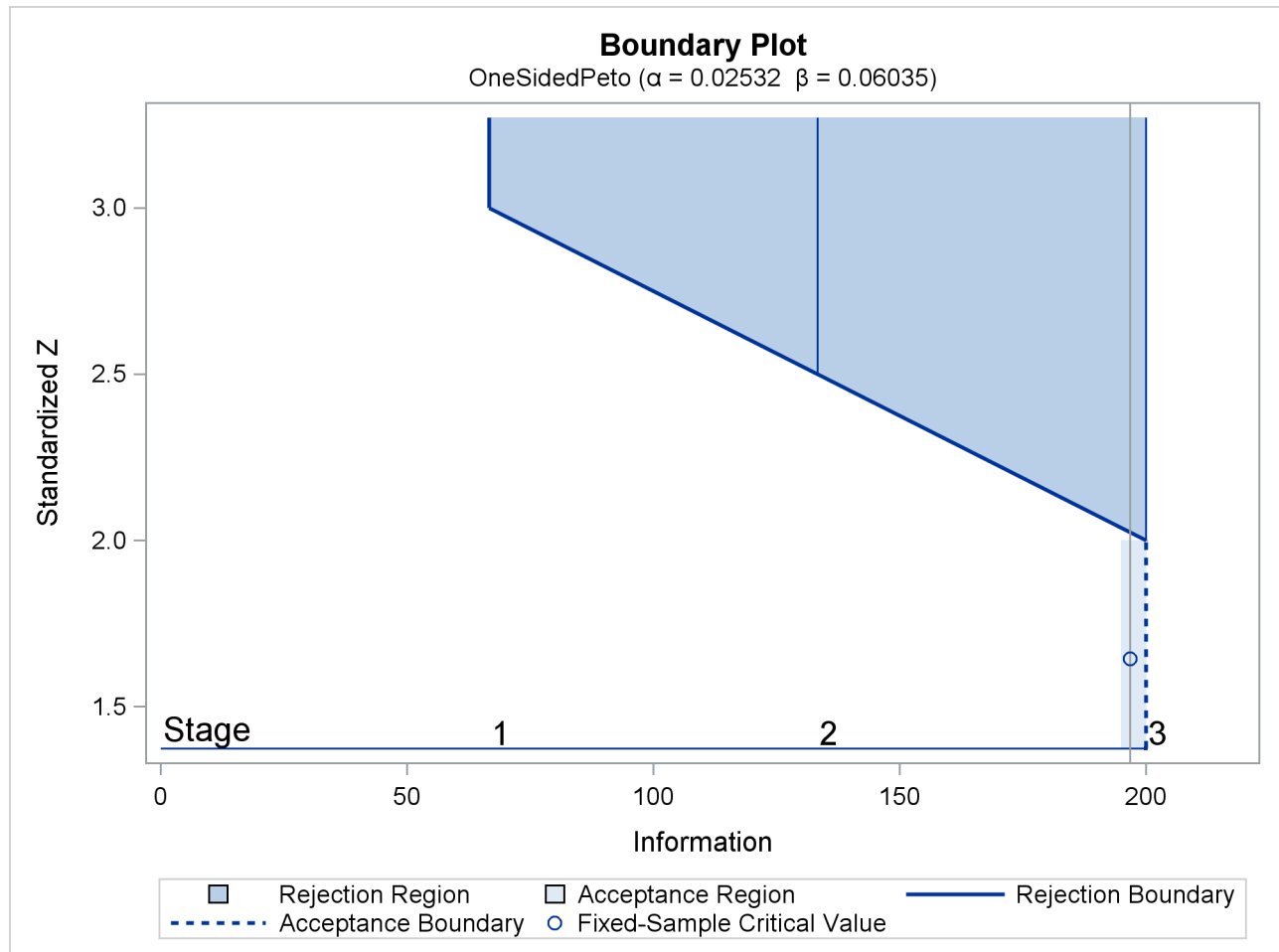
Output 101.5.13 Boundary Plot
