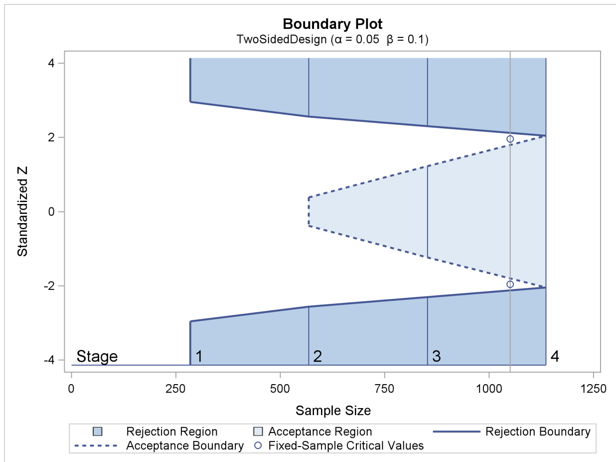
Figure 101.11 Boundary Plot for Two-Sided Test
