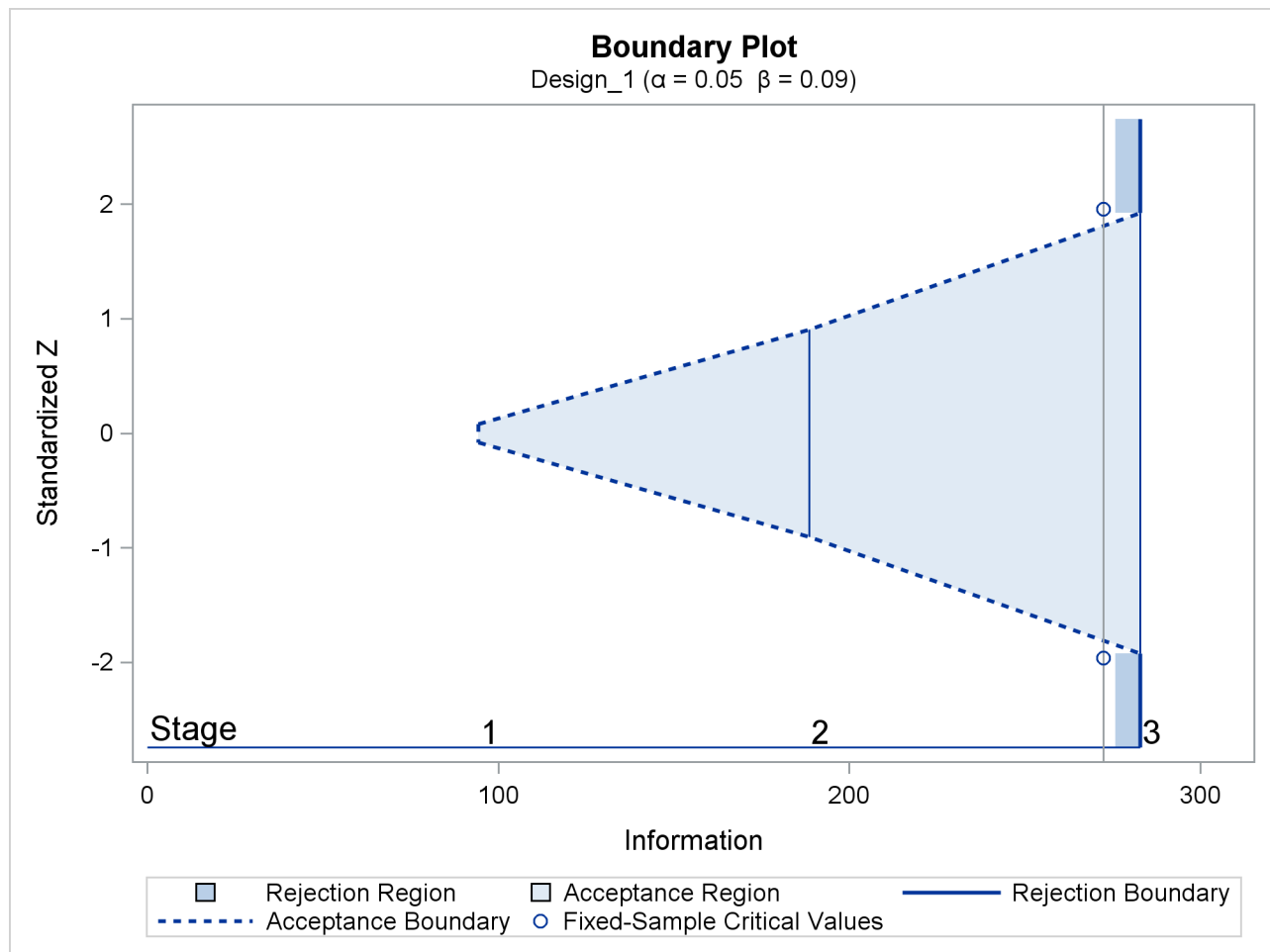
Output 101.10.4 Boundary Plot
