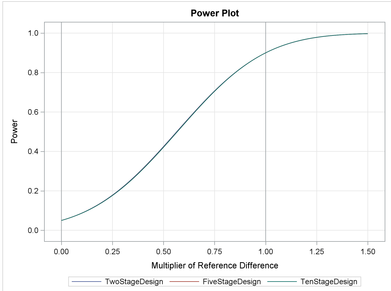
Output 101.9.8 Power Plot
