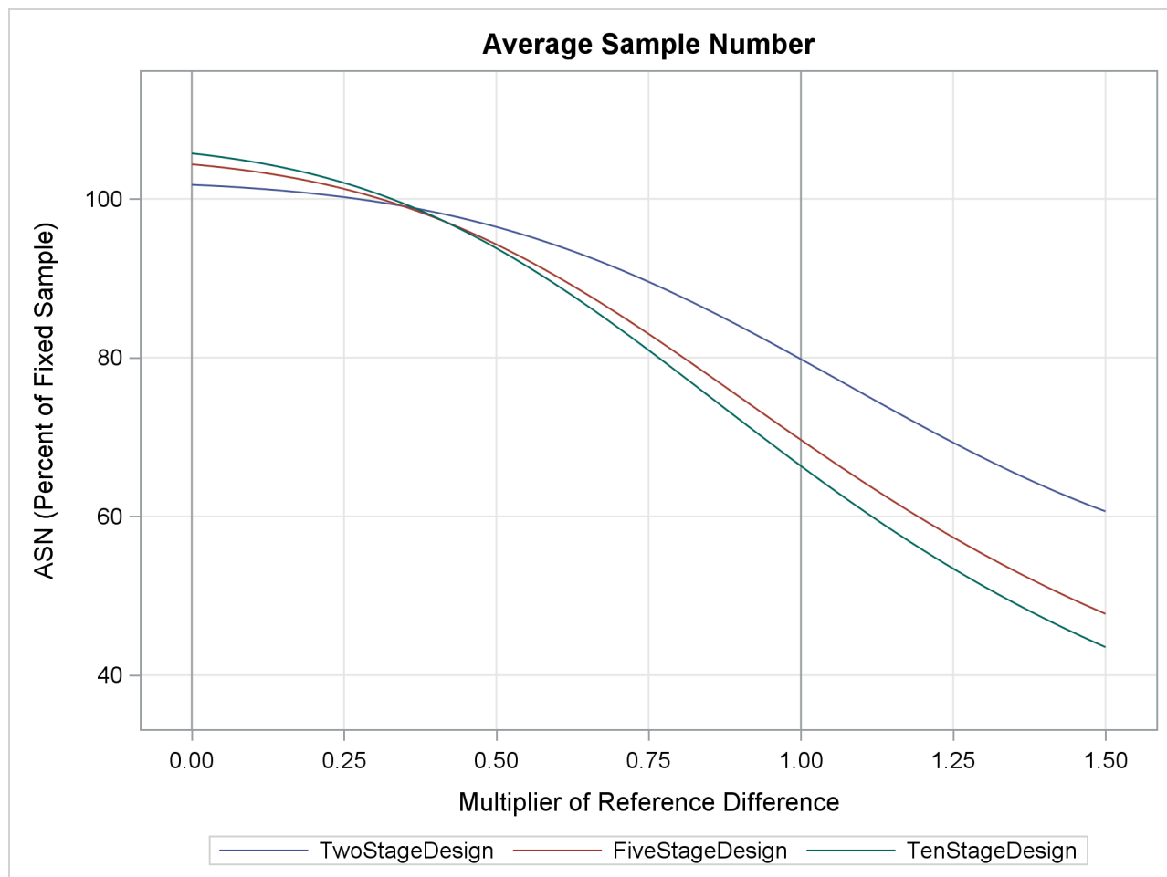
Output 101.9.7 ASN Plot
