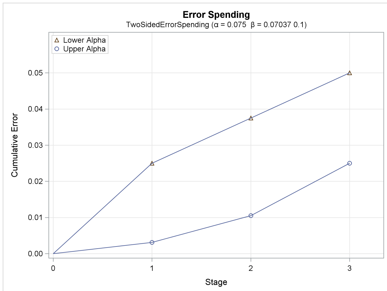
Output 101.11.10 Error Spending Plot
