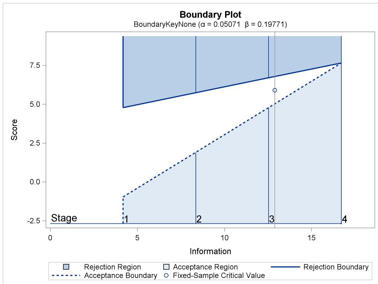
Output 101.7.4 Boundary Plot
