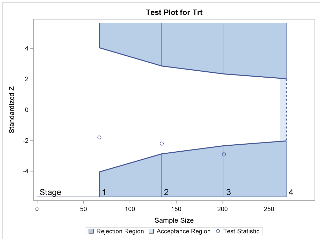
Figure 101.1 Sequential Plot for Two-Sided Test
