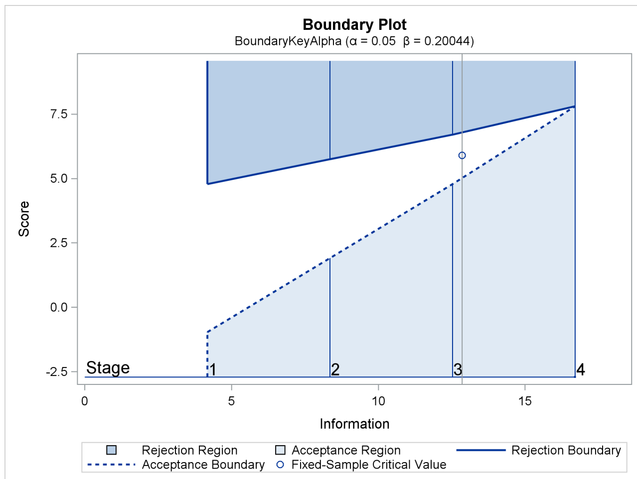
Output 101.7.8 Boundary Plot
