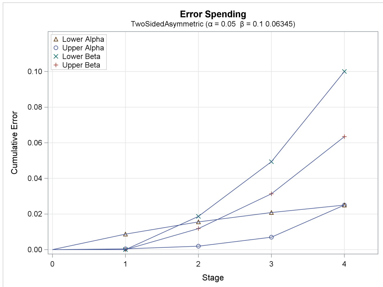
Output 101.12.10 Error Spending Plot
