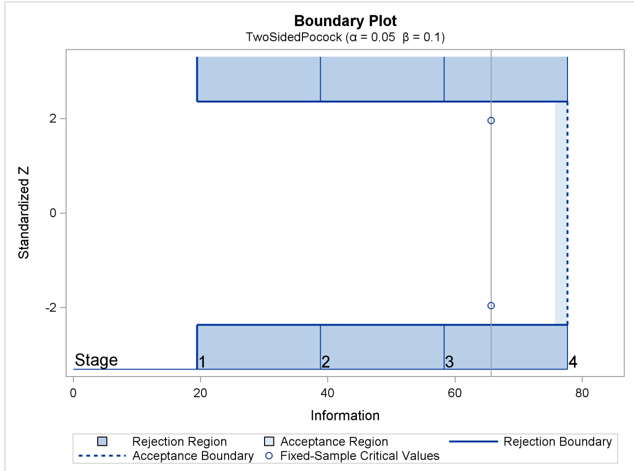
Output 101.4.1 Pocock Boundary Plot
