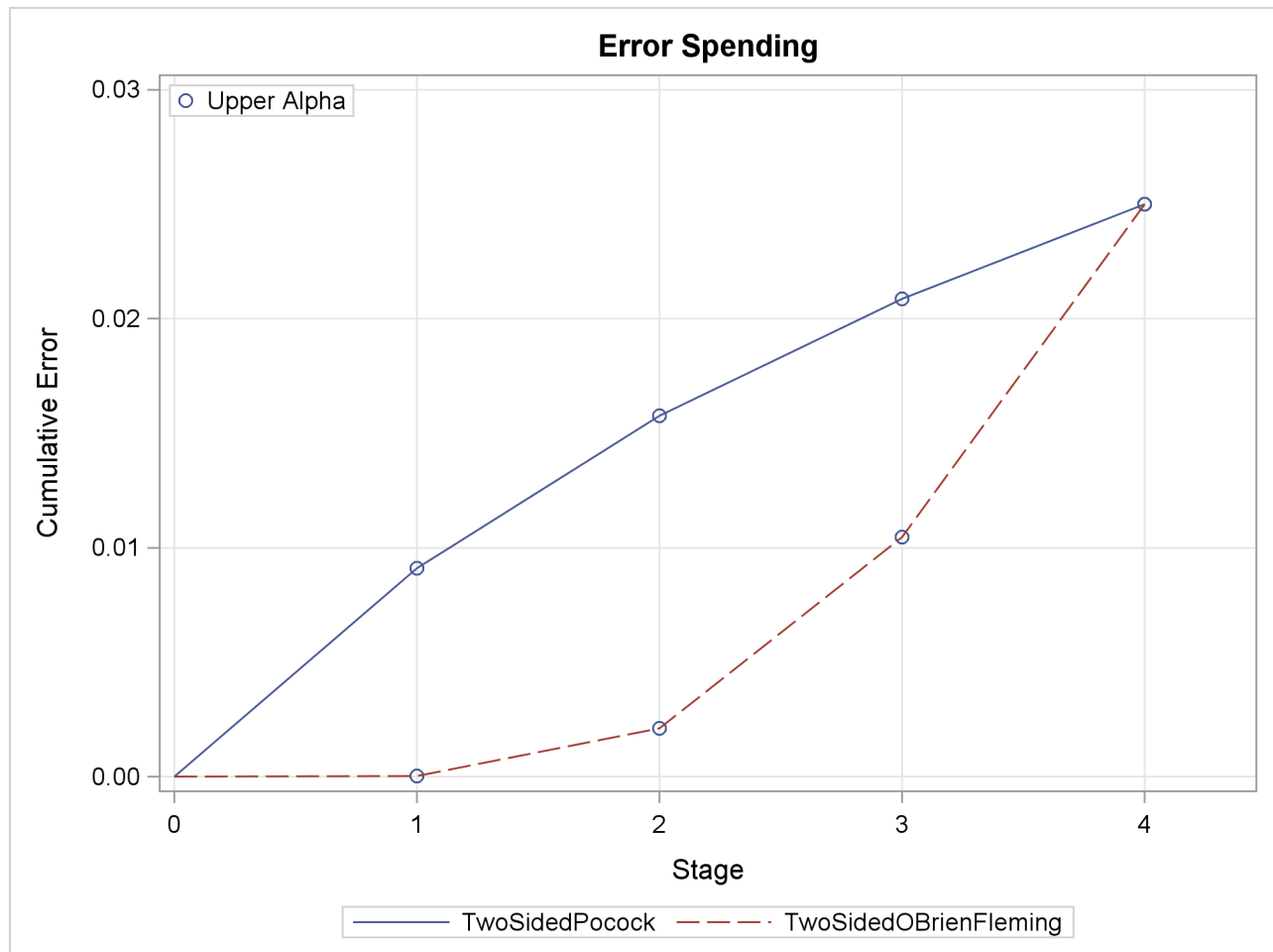
Output 101.4.6 Error Spending Plot
