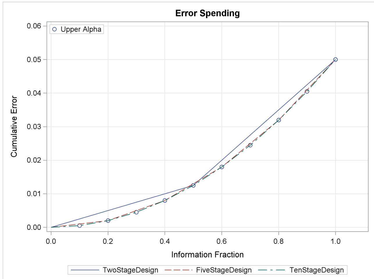
Output 101.9.10 Error Spending Plot
