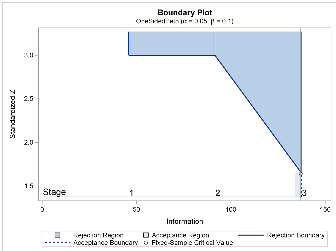
Output 101.5.6 Boundary Plot
