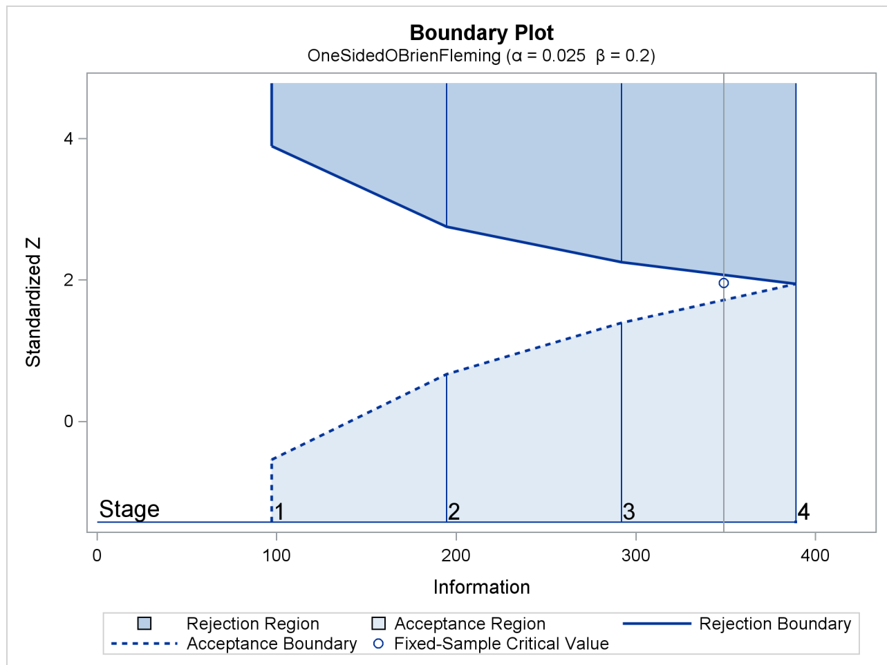
Output 101.2.4 Boundary Plot
