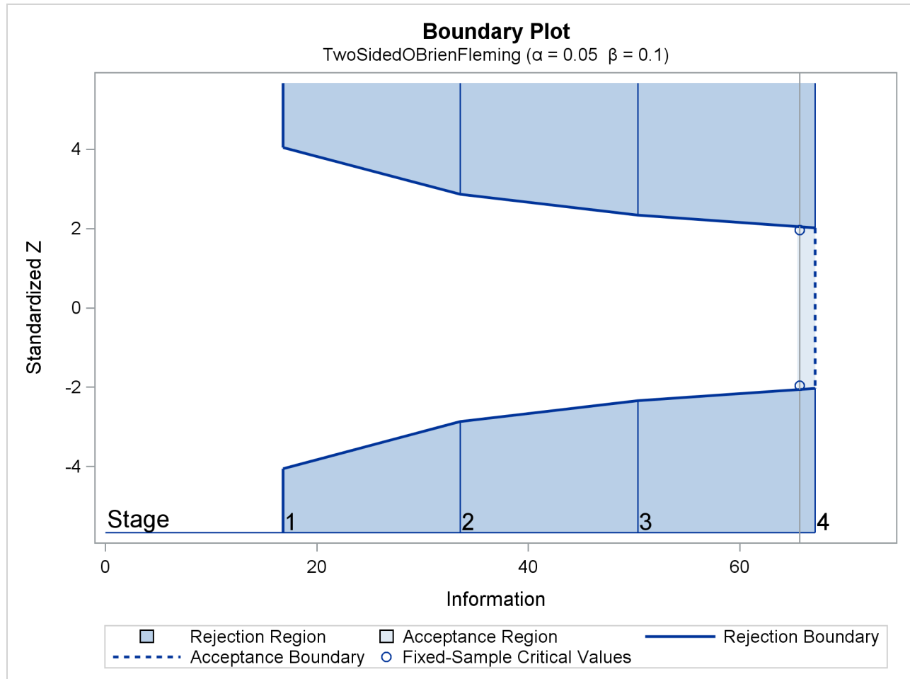
Output 101.4.2 O'Brien-Fleming Boundary Plot
