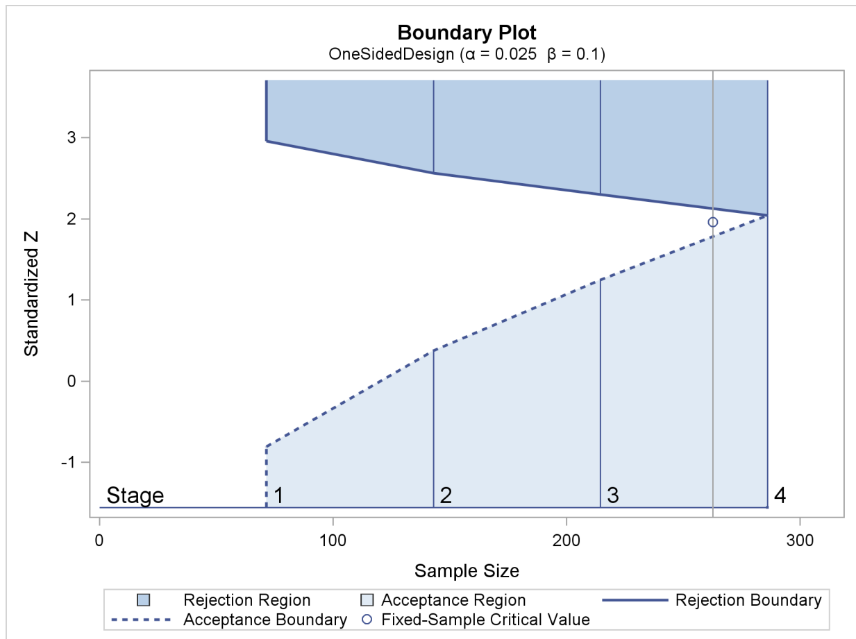
Figure 101.3 Boundary Plot for One-Sided Design
