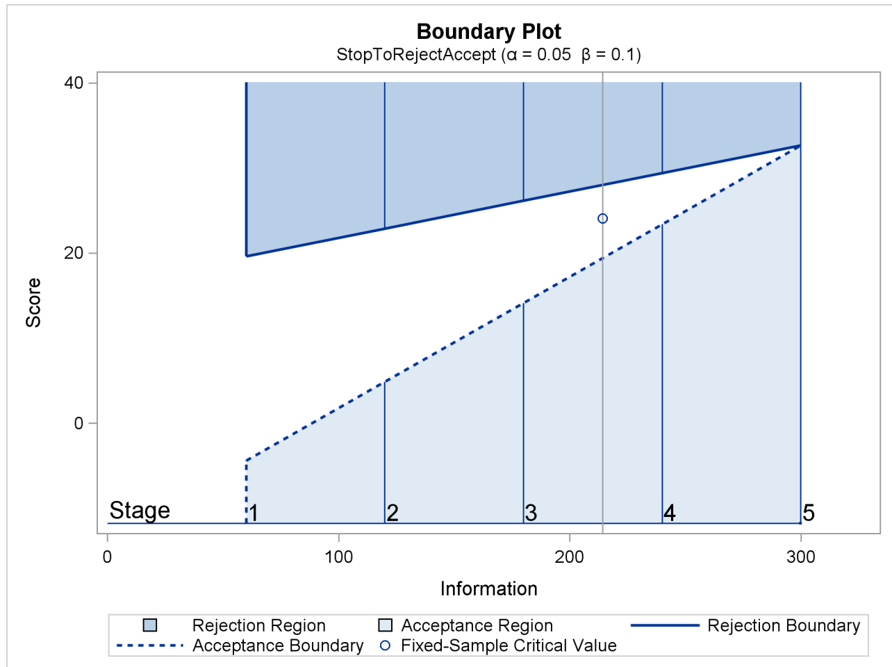
Output 101.6.5 Boundary Plot with Score Statistics
