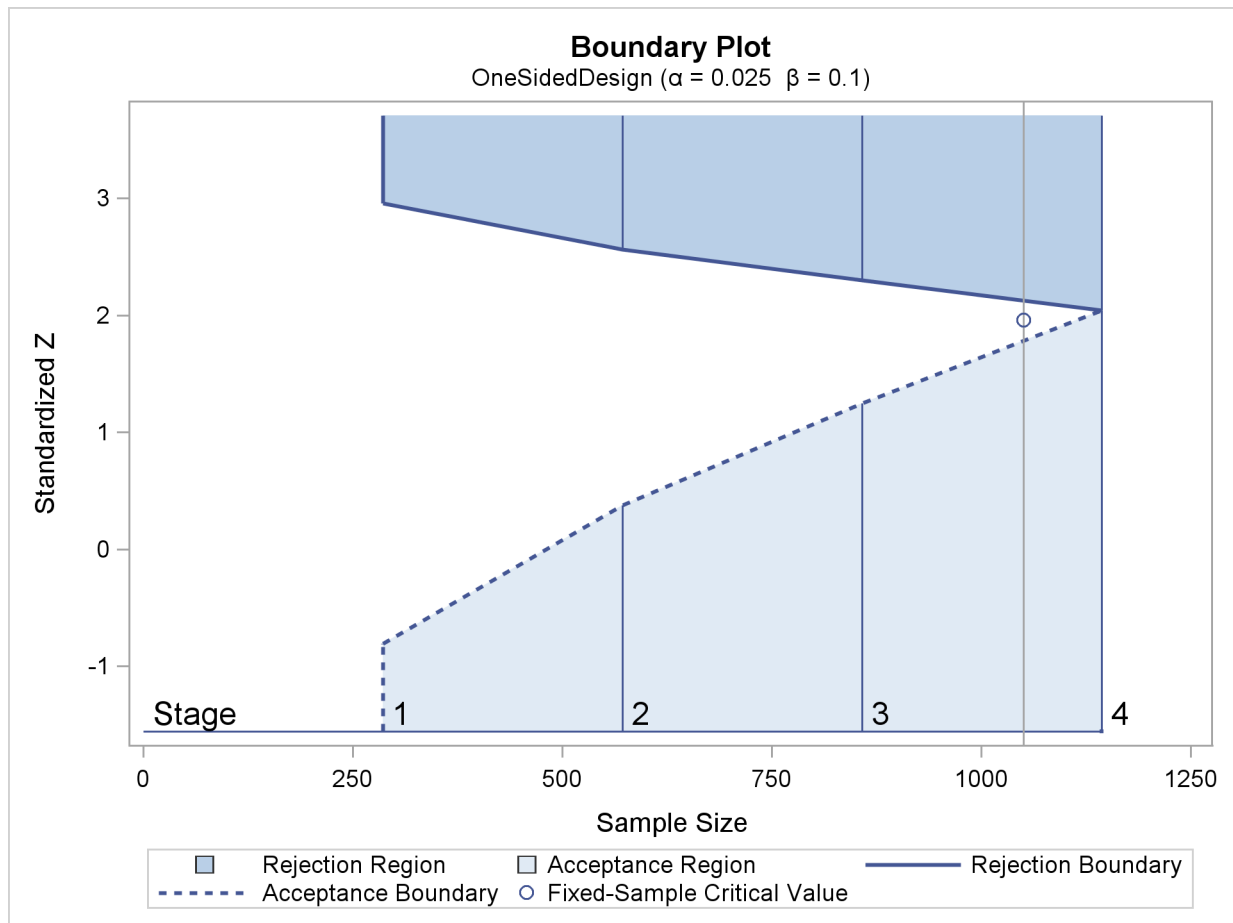
Figure 101.10 Boundary Plot for One-Sided Test
