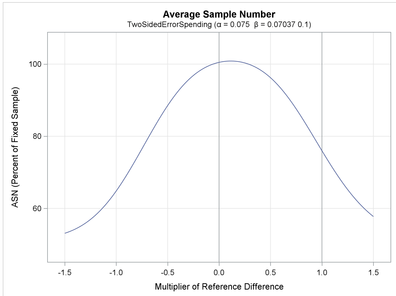
Output 101.11.6 ASN Plot
