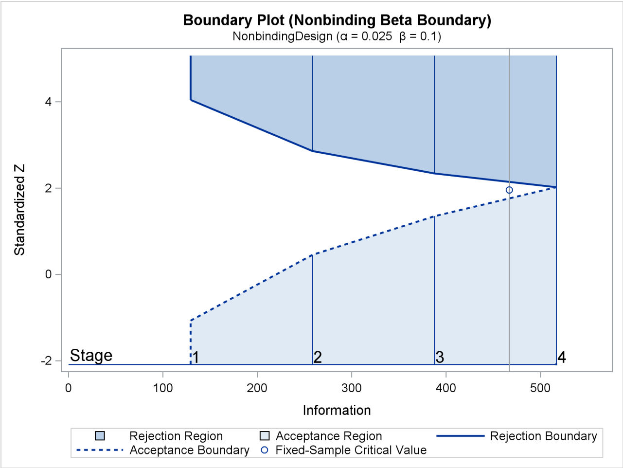
Output 101.13.4 Boundary Plot
