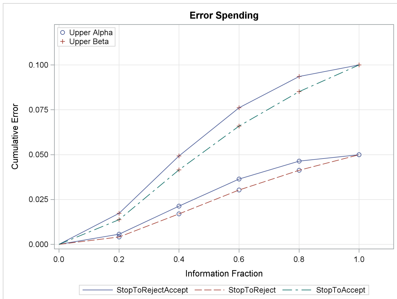
Output 101.6.17 Error Spending Plot
