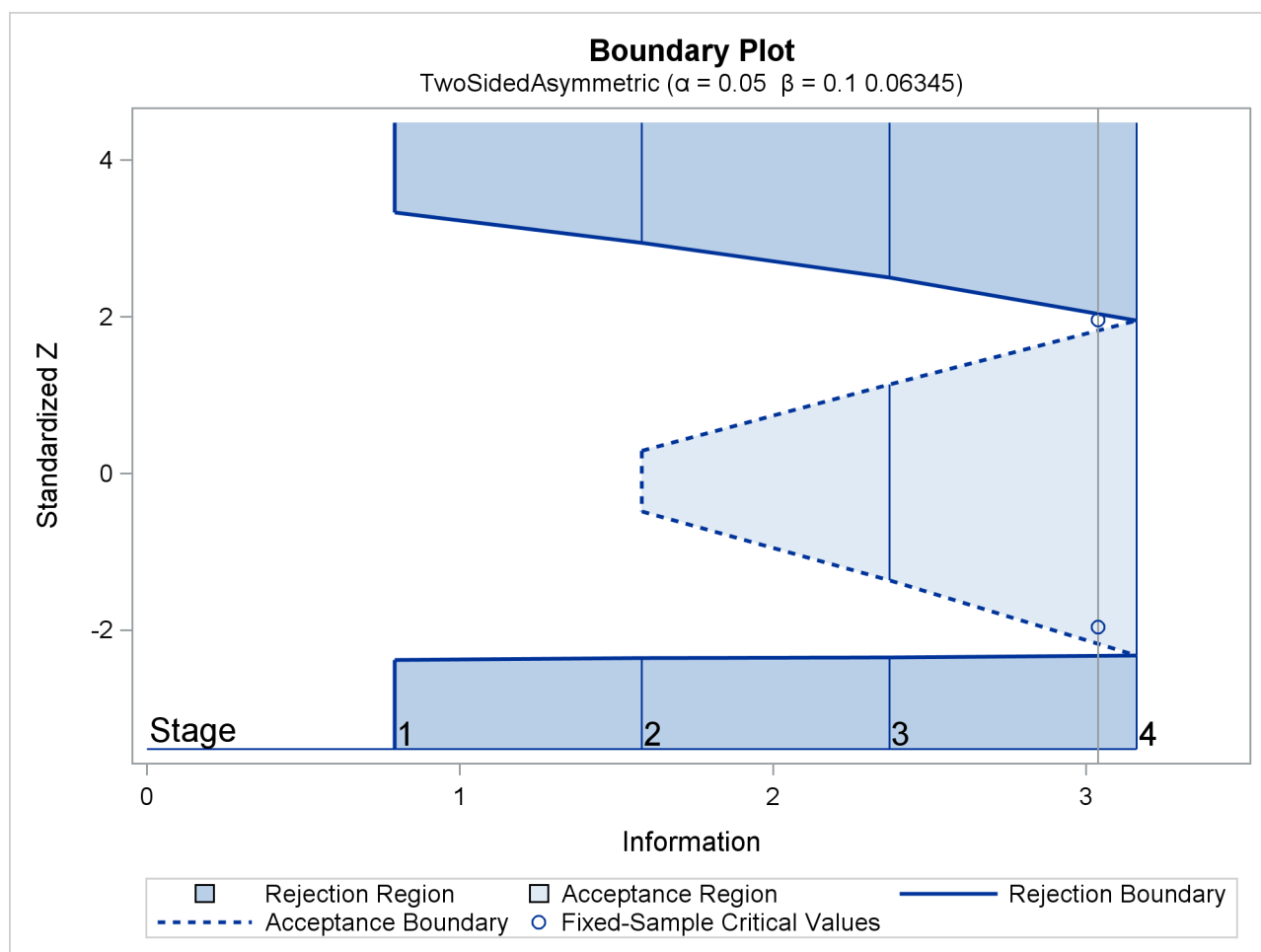
Output 101.12.8 Boundary Plot
