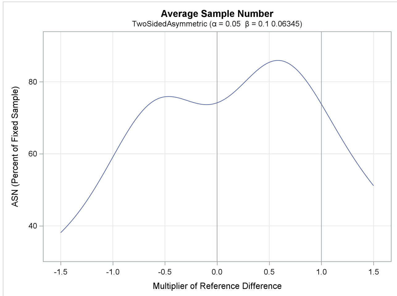
Output 101.12.6 ASN Plot
