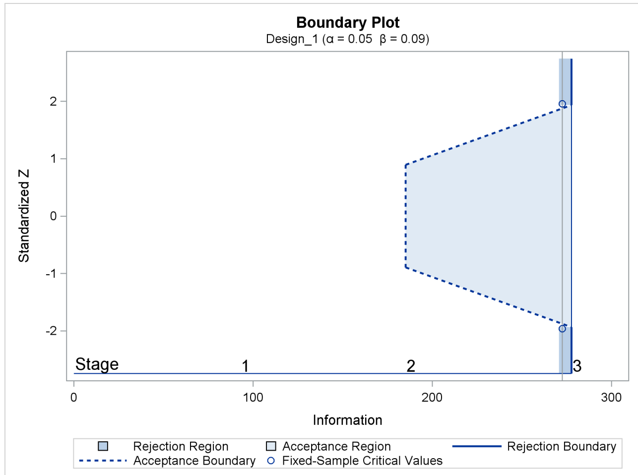
Output 101.10.8 Boundary Plot
