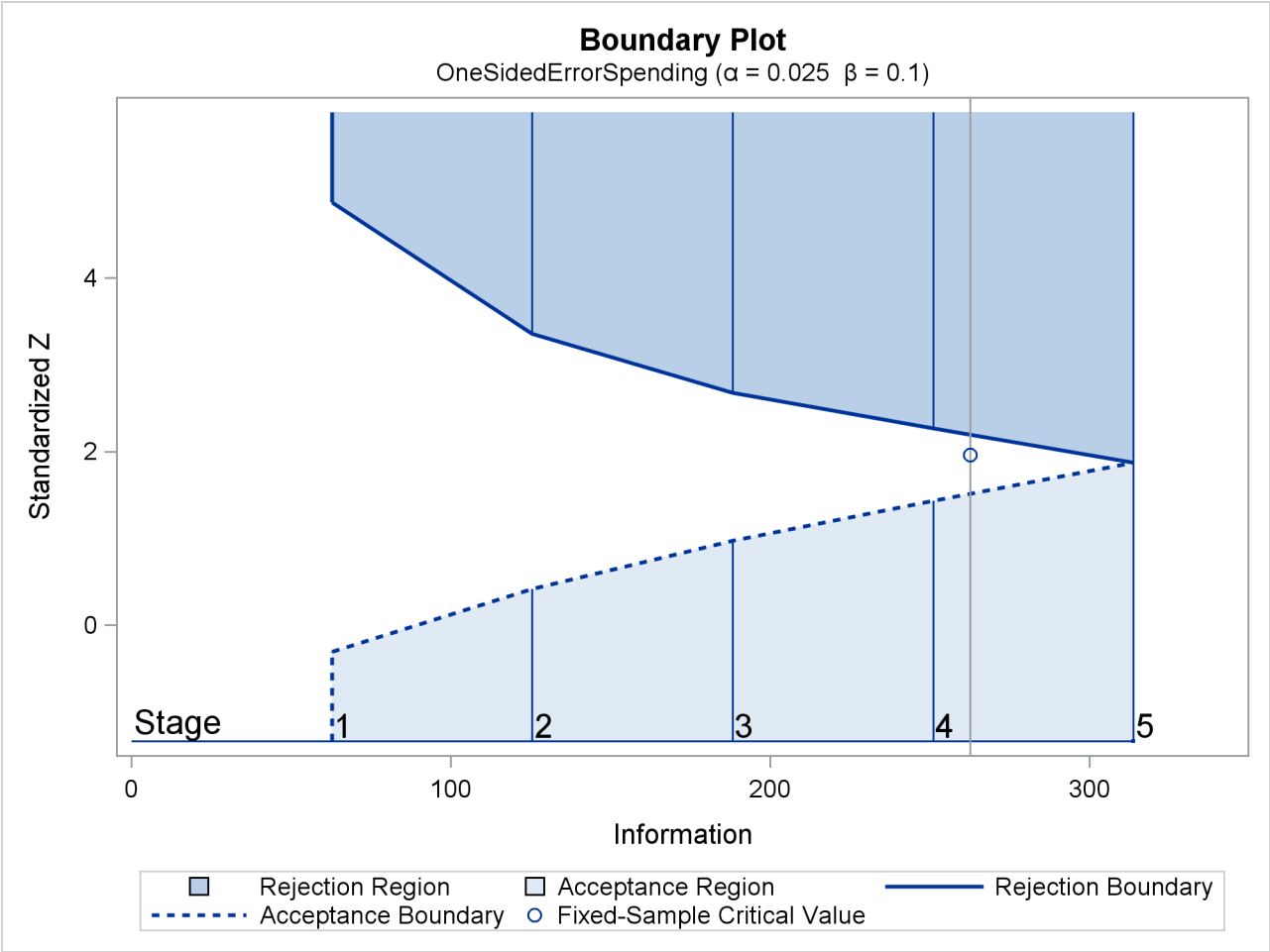
Output 101.8.8 Boundary Plot
