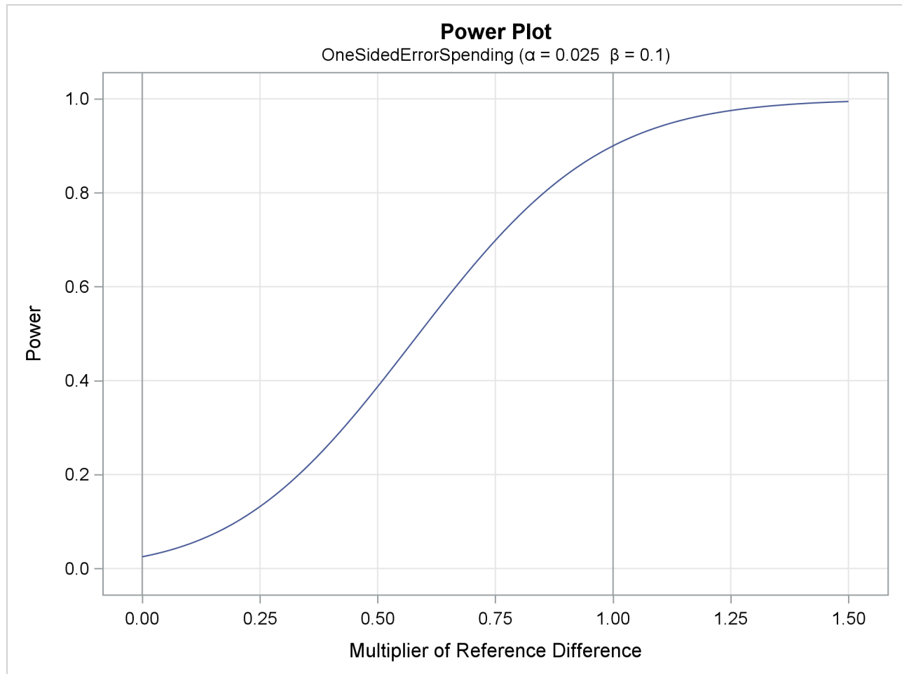
Output 101.8.6 Power Plot
