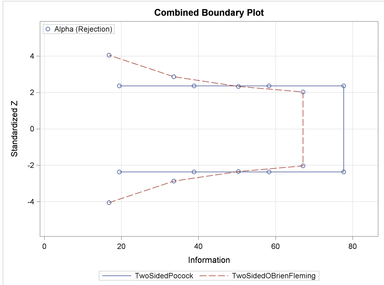
Output 101.4.5 Combined Boundary Plot
