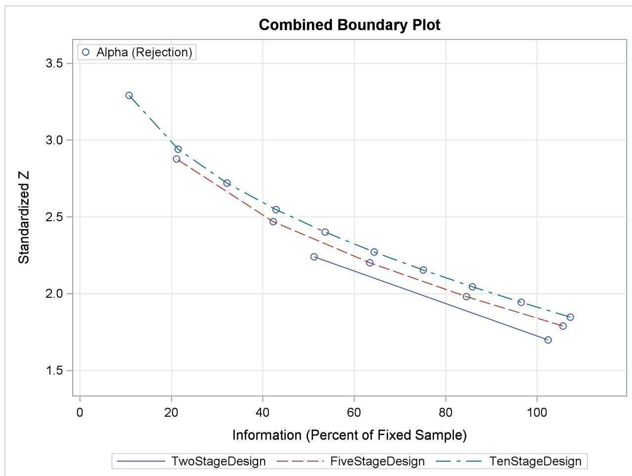
Output 101.9.9 Combined Boundary Plot
