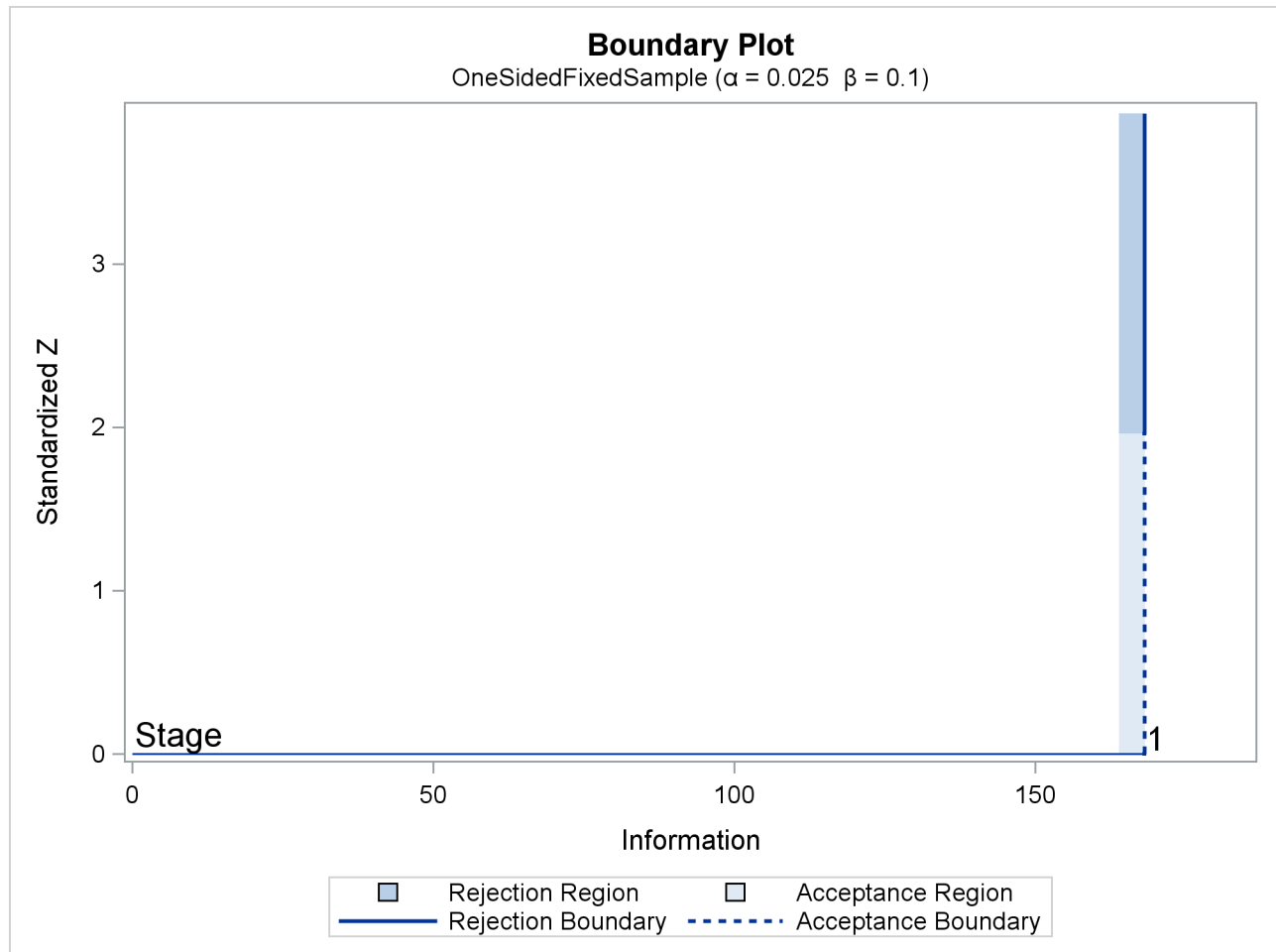
Output 101.1.4 Boundary Plot
