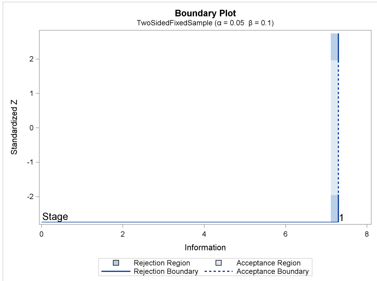
Output 101.1.10 Boundary Plot
