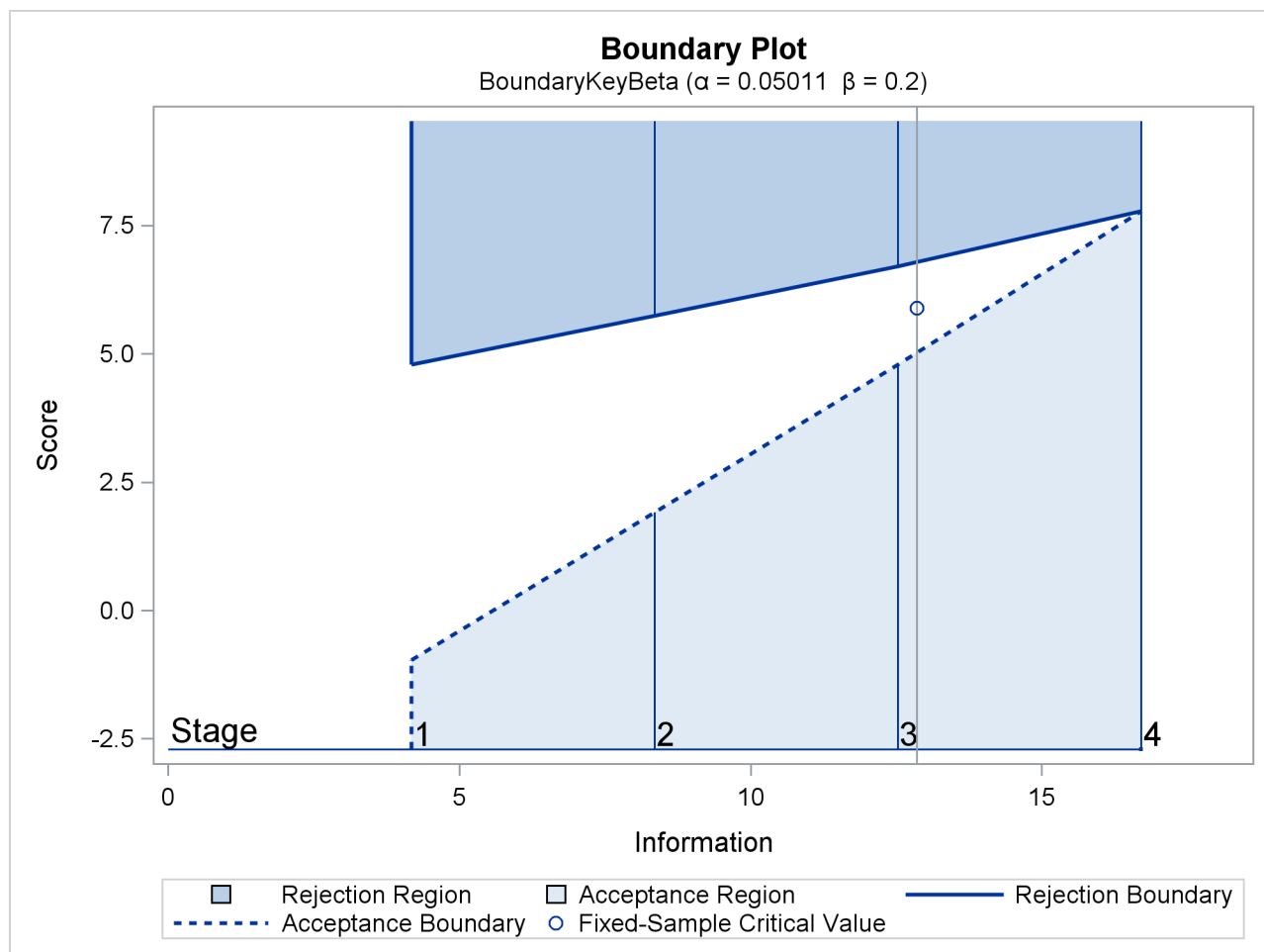
Output 101.7.12 Boundary Plot
