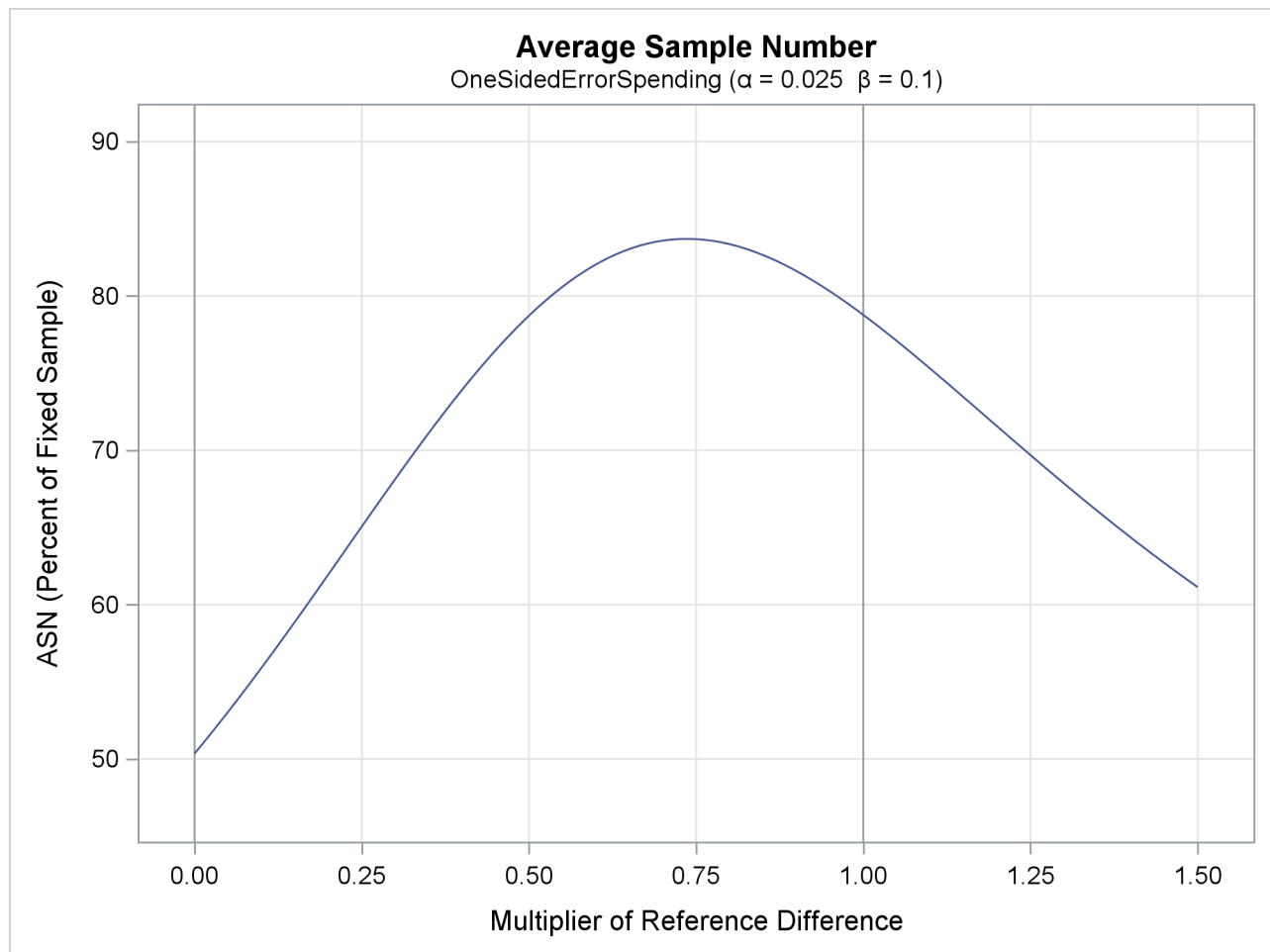
Output 101.8.5 ASN Plot
