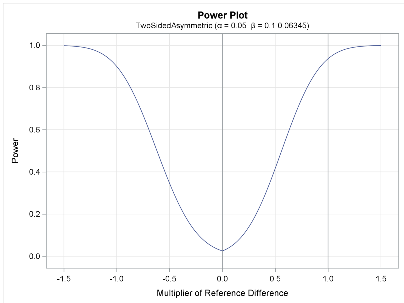
Output 101.12.5 Power Plot
