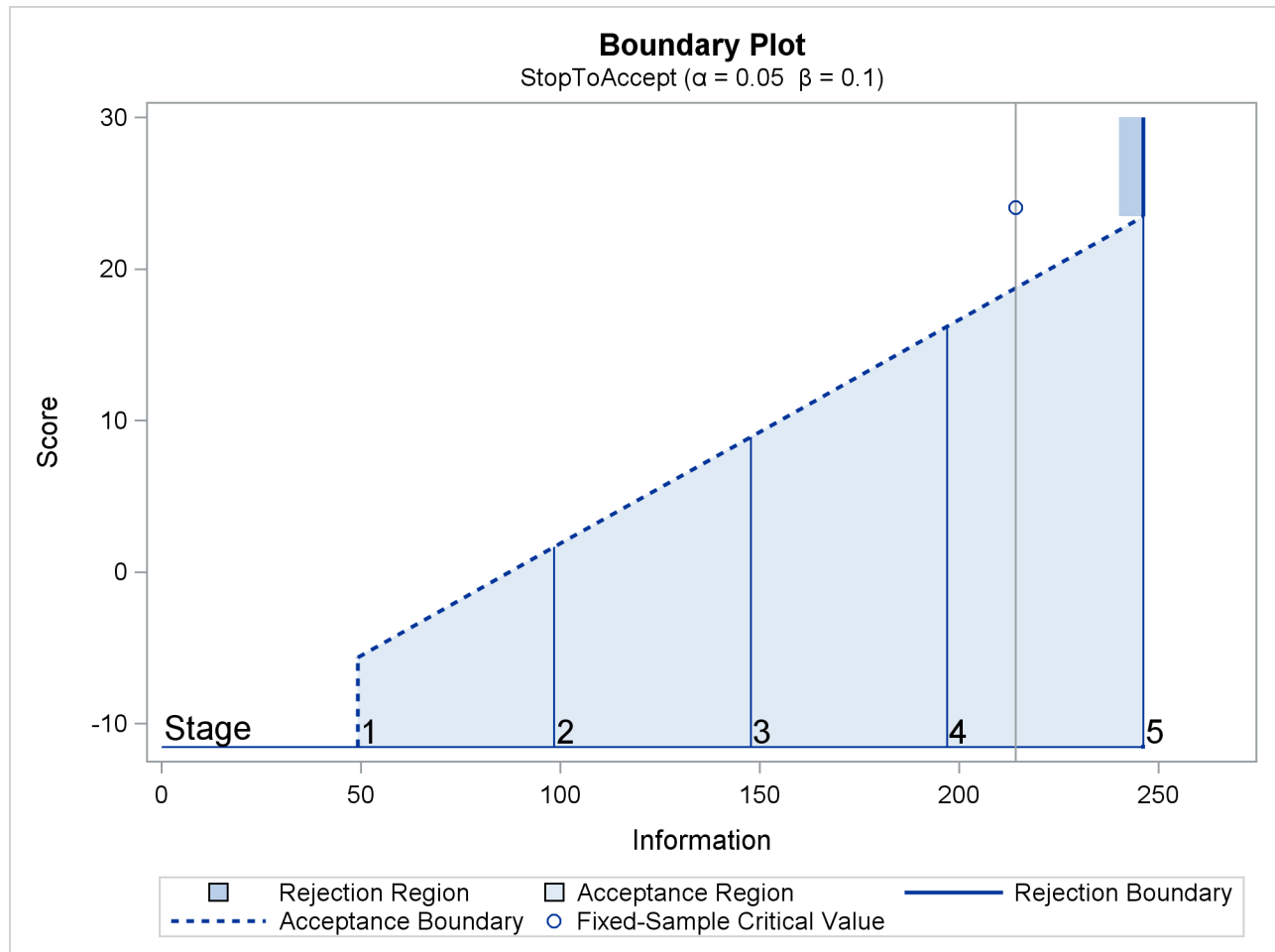
Output 101.6.15 Boundary Plot with Score Scale
