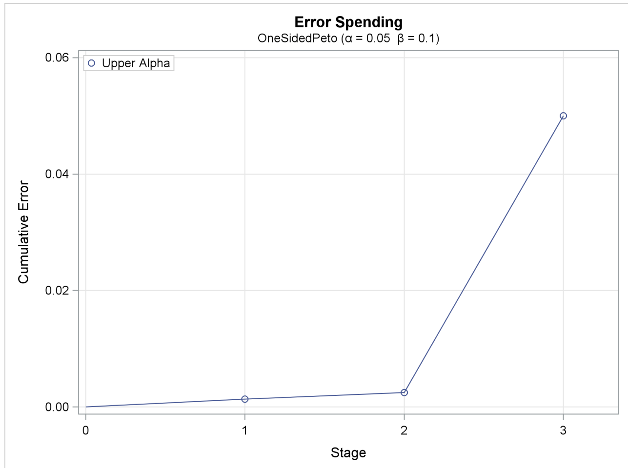
Output 101.5.7 Error Spending Plot
