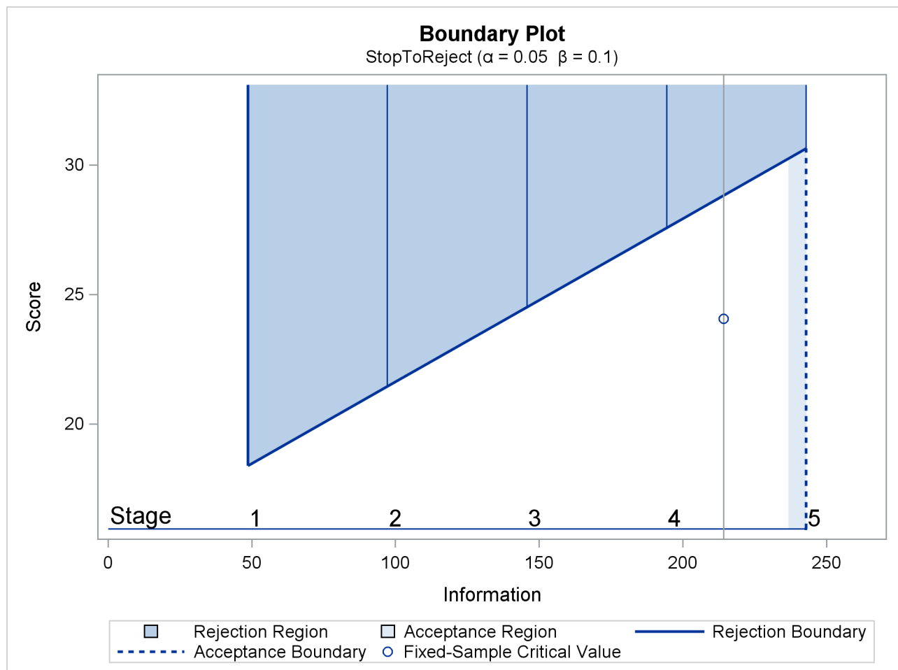
Output 101.6.10 Boundary Plot with Score Statistics
