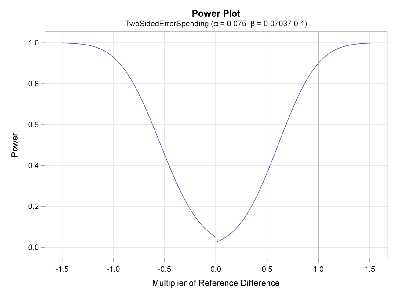
Output 101.11.5 Power Plot
