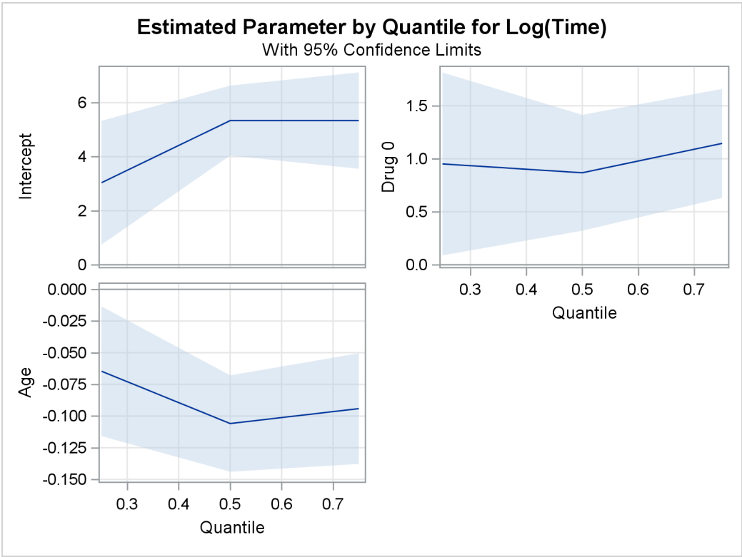
Figure 94.3 Estimated Parameters
