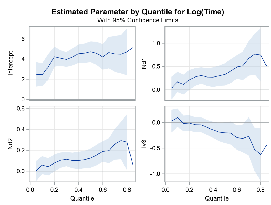
Output 94.2.2 Quantile Processes with 95% Confidence Bands
