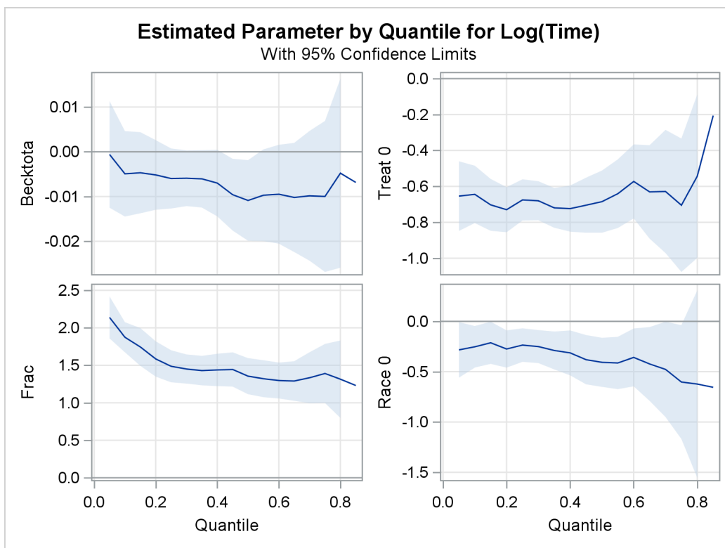
Output 94.2.3 Quantile Processes with 95% Confidence Bands
