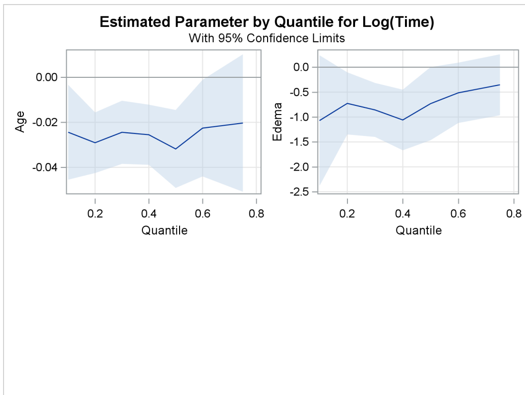
Output 94.1.5 Quantile Processes with 95% Confidence Bands
