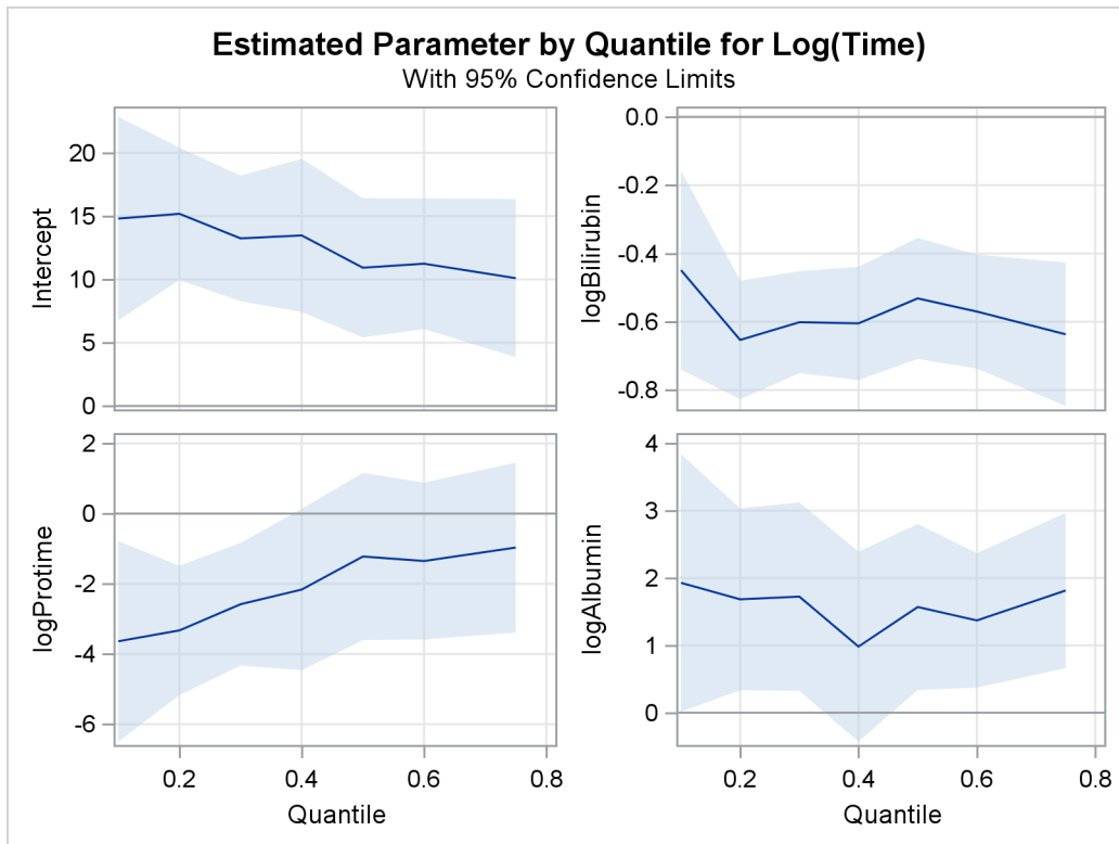
Output 94.1.4 Quantile Processes with 95% Confidence Bands
