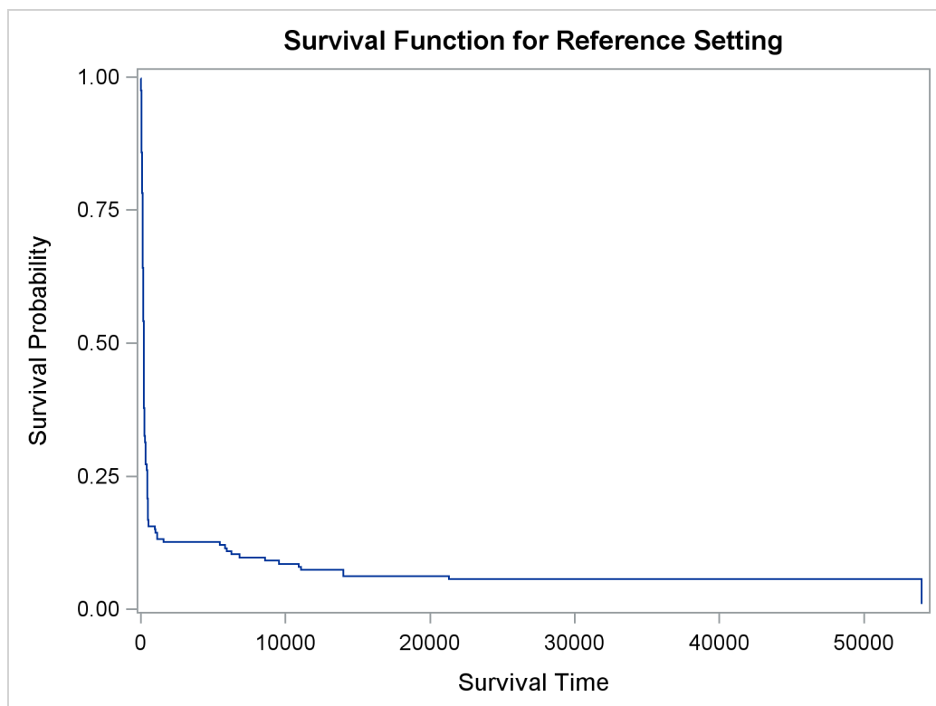
Output 94.2.5 Survival Function
