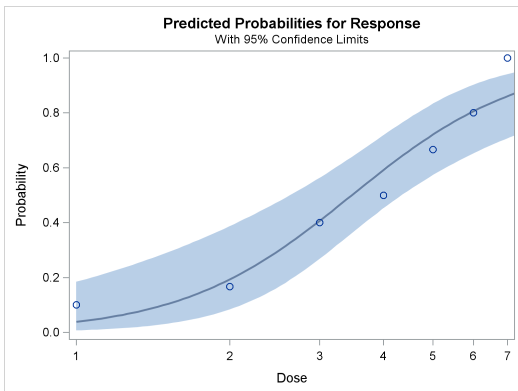
Output 93.1.7 Plot of Observed and Fitted Probabilities
