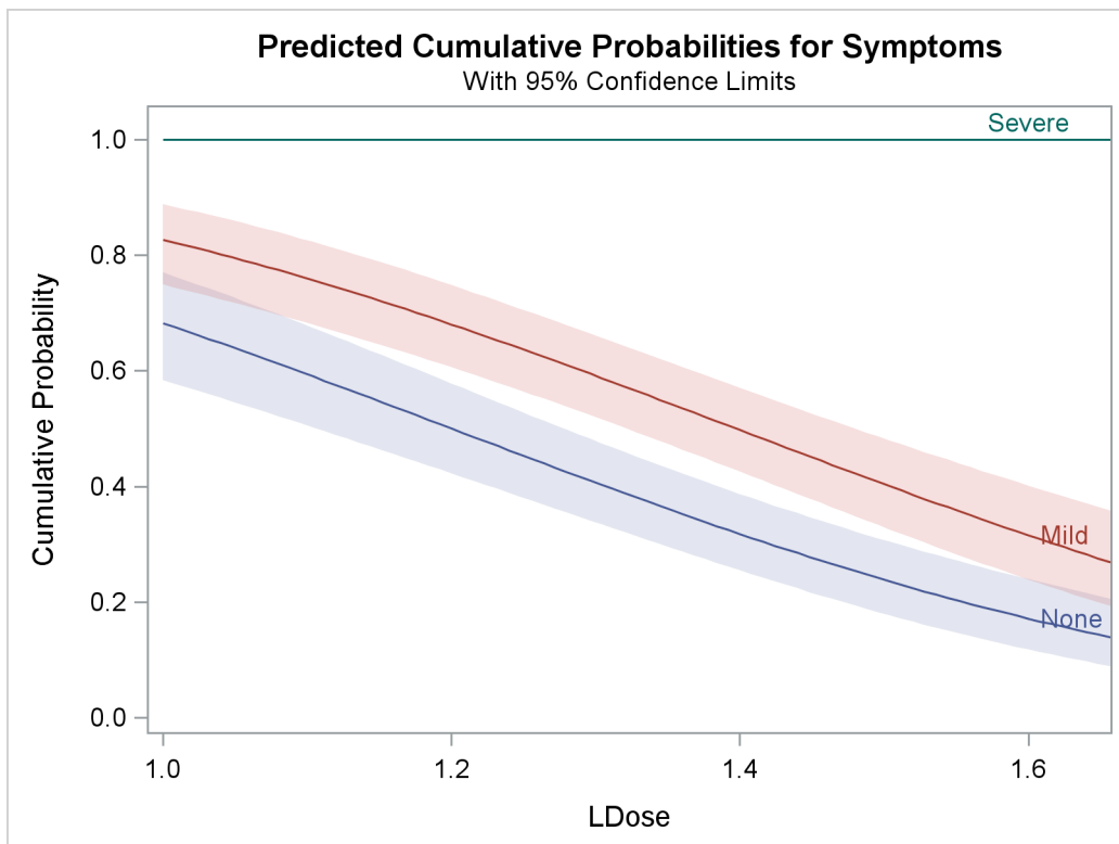
Output 93.2.6 Plot of Predicted Cumulative Probabilities for the Standard Preparation Group
