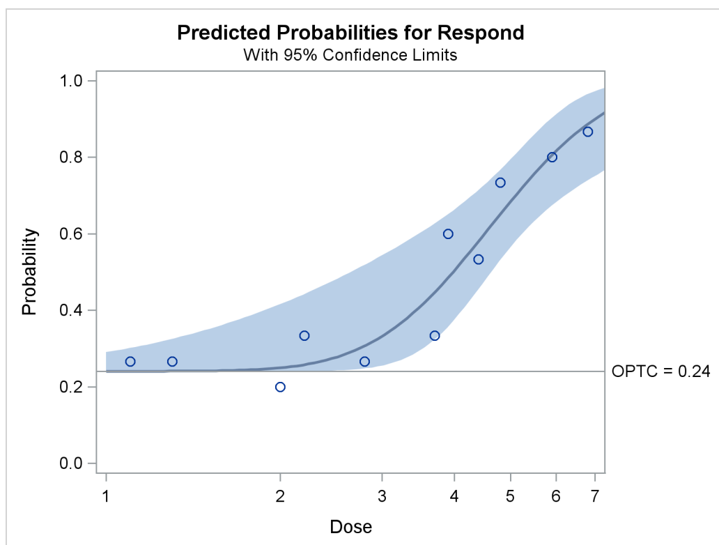
Figure 93.4 Plot of Observed and Fitted Probabilities versus Dose Level
