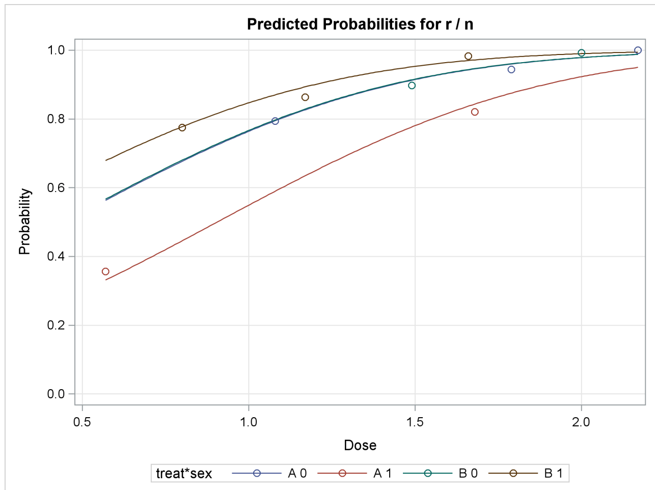
Output 93.5.3 Predicted Probability versus Dose Level by treat*sex
