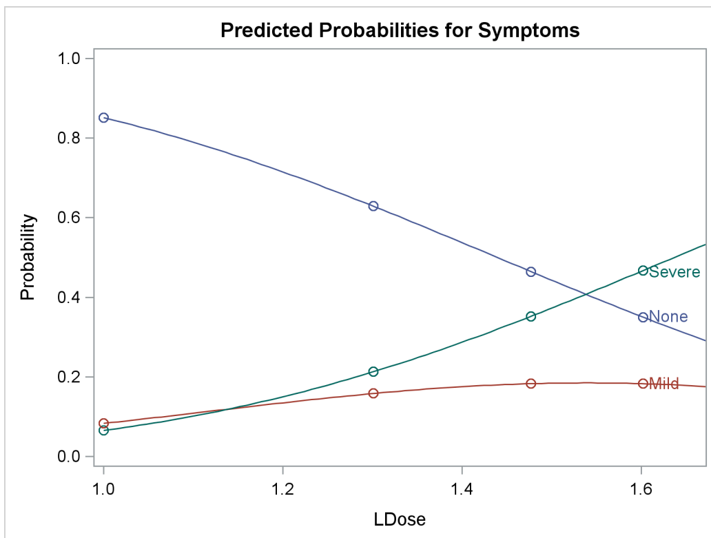
Output 93.2.3 Plot of Predicted Probabilities for the Test Preparation Group
