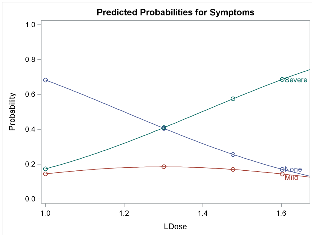
Output 93.2.5 Plot of Predicted Probabilities for the Standard Preparation Group
