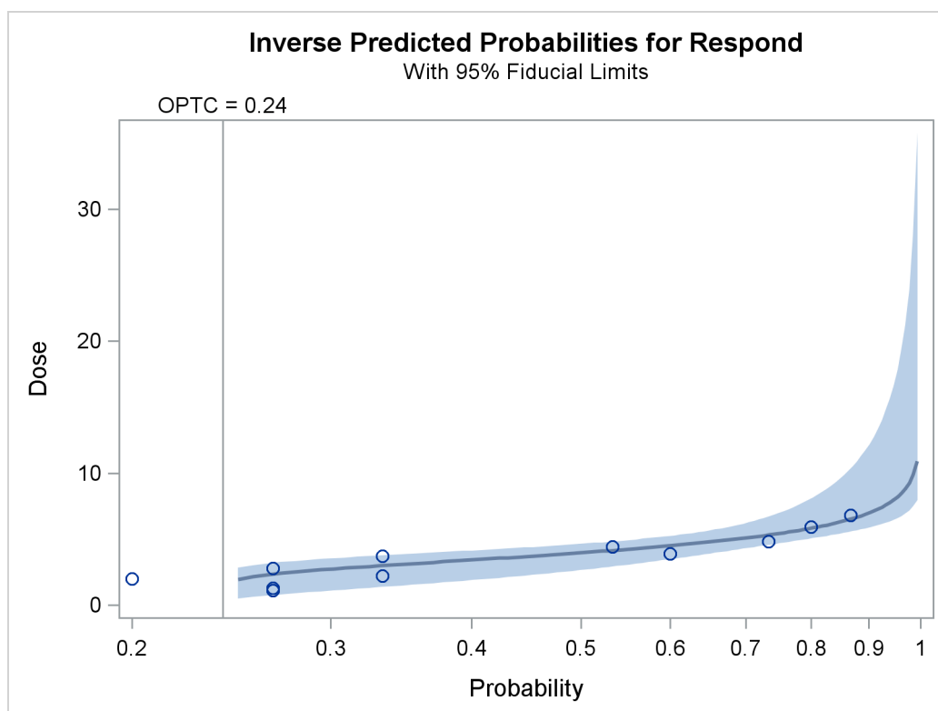
Figure 93.5 Inverse Predicted Probability Plot with Fiducial Limits
