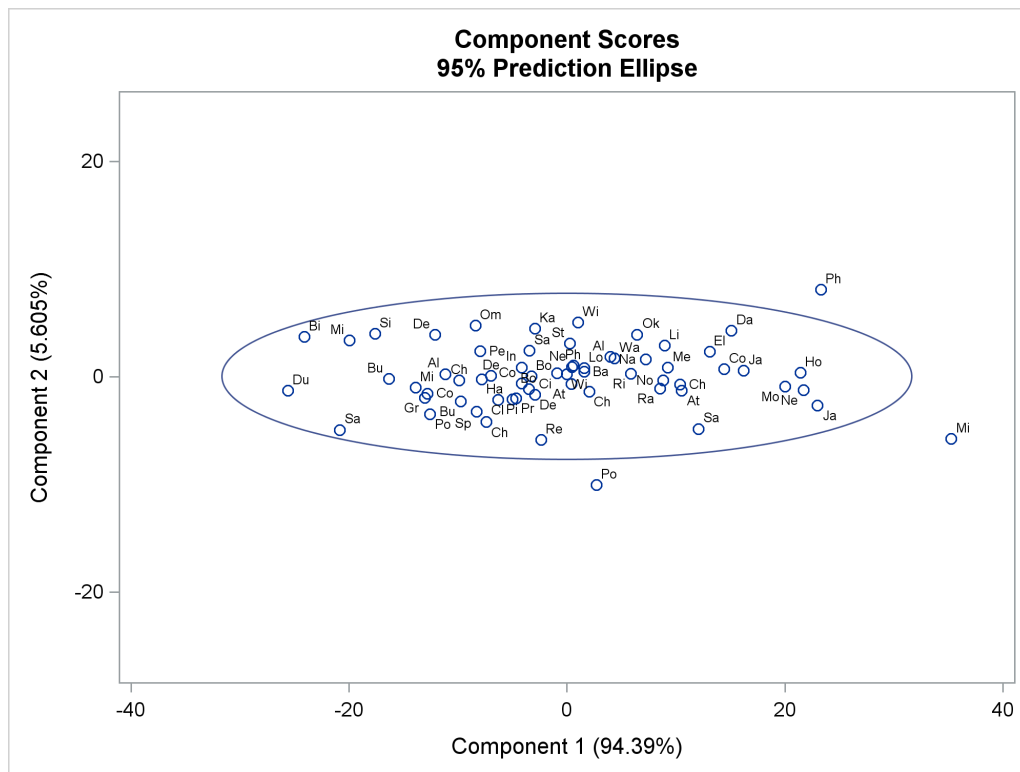
Output 91.1.3 Plot of Component 2 by Component 1
