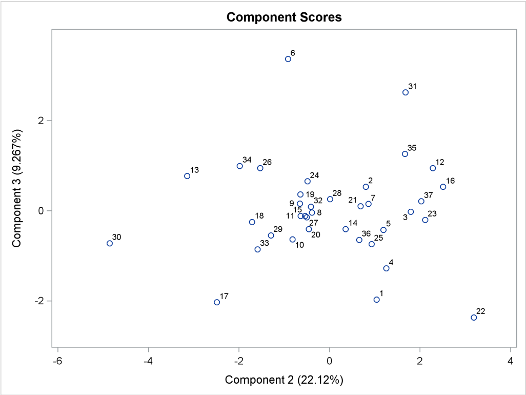
Output 91.3.11 Component 3 versus Component 2
