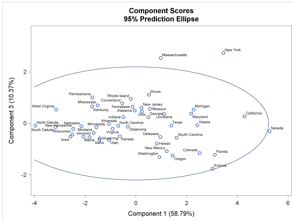
Figure 91.5 Plot of the First and Third Component Scores
