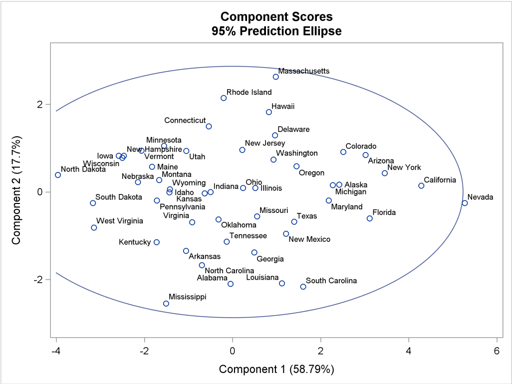
Figure 91.4 Plot of the First Two Component Scores
