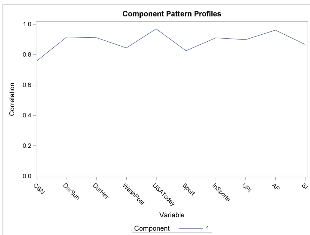
Output 91.2.3 Pattern Profile Plot
