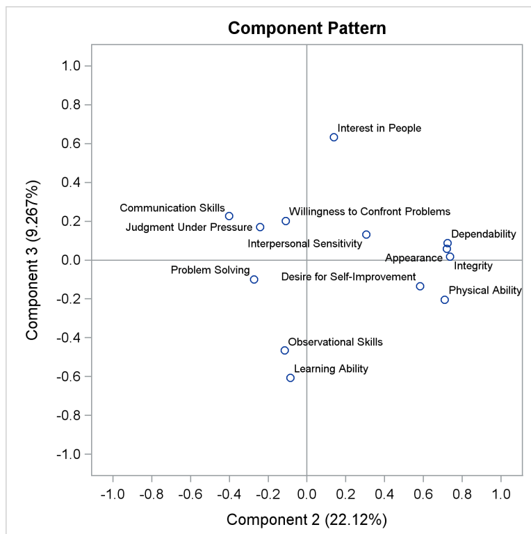
Output 91.3.7 Pattern Plot of Component 3 by Component 2
