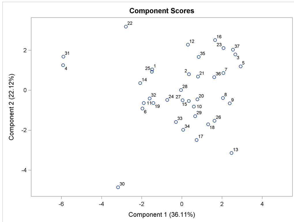
Output 91.3.9 Component 2 versus Component 1
