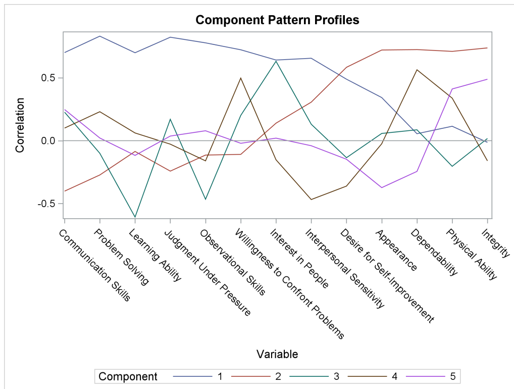
Output 91.3.8 Component Pattern Profile Plot from Using PROC PRINCOMP
