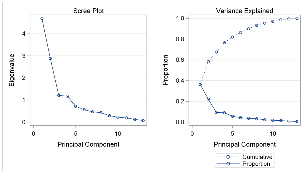
Output 91.3.3 Scree Plot from Using PROC PRINCOMP
