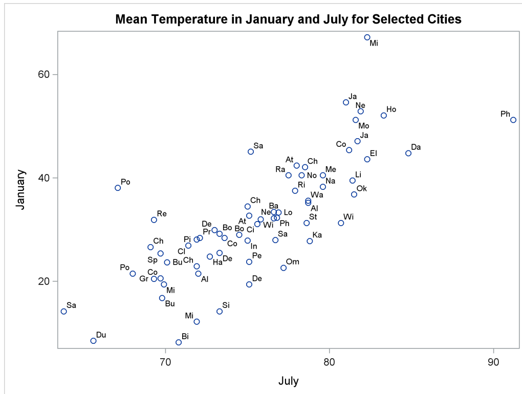
Output 91.1.1 Plot of Raw Data
