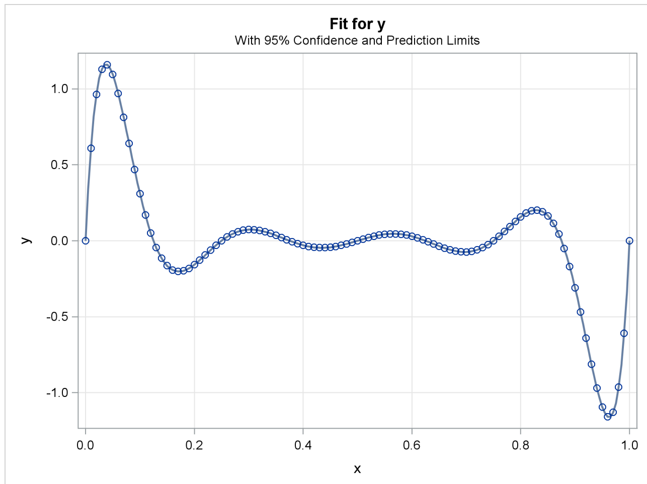
Output 84.3.2 PROC ORTHOREG Fit Plot for Ninth-Degree Polynomial
