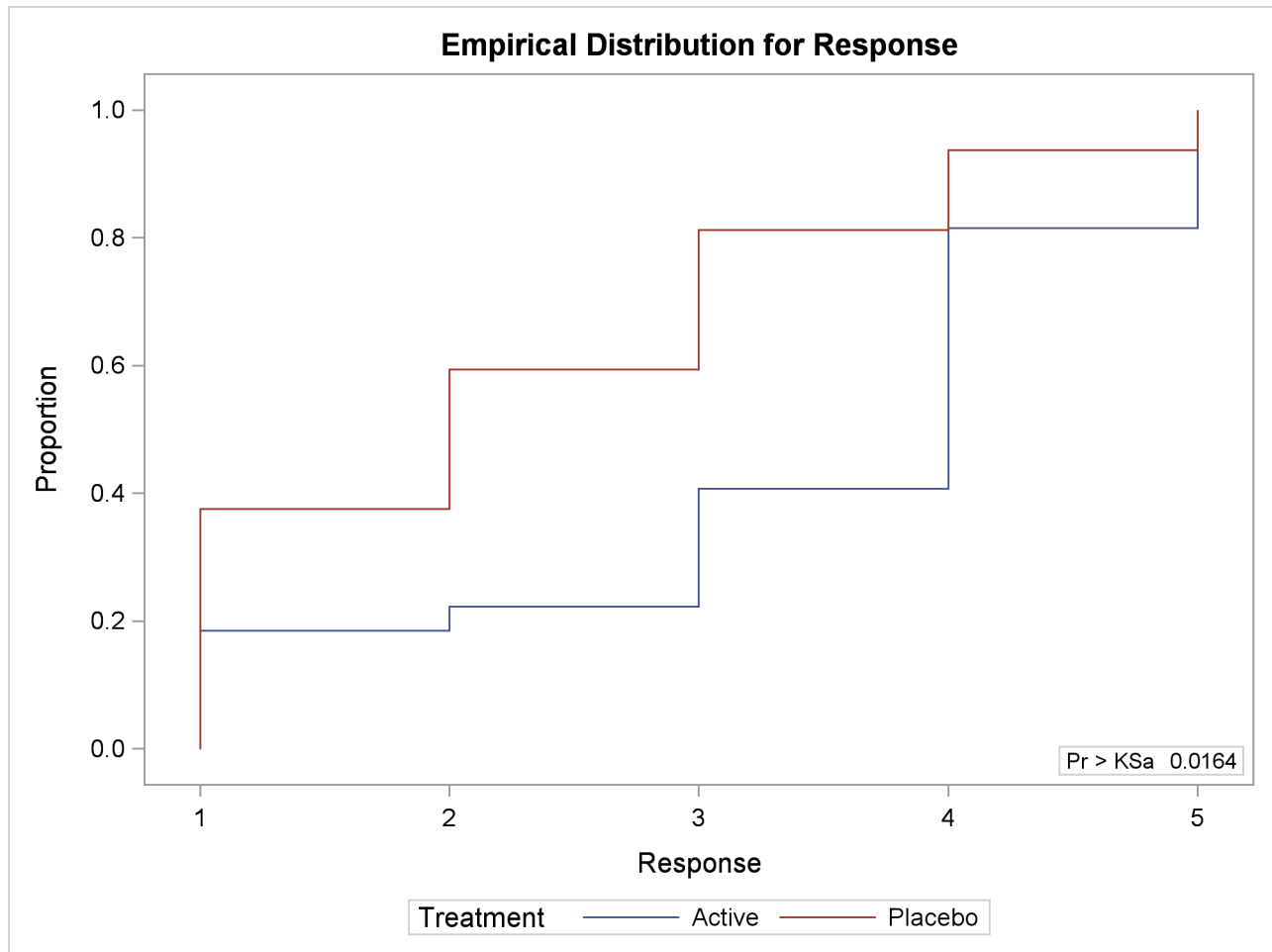
Output 83.2.2 Empirical Distribution Function Plot
