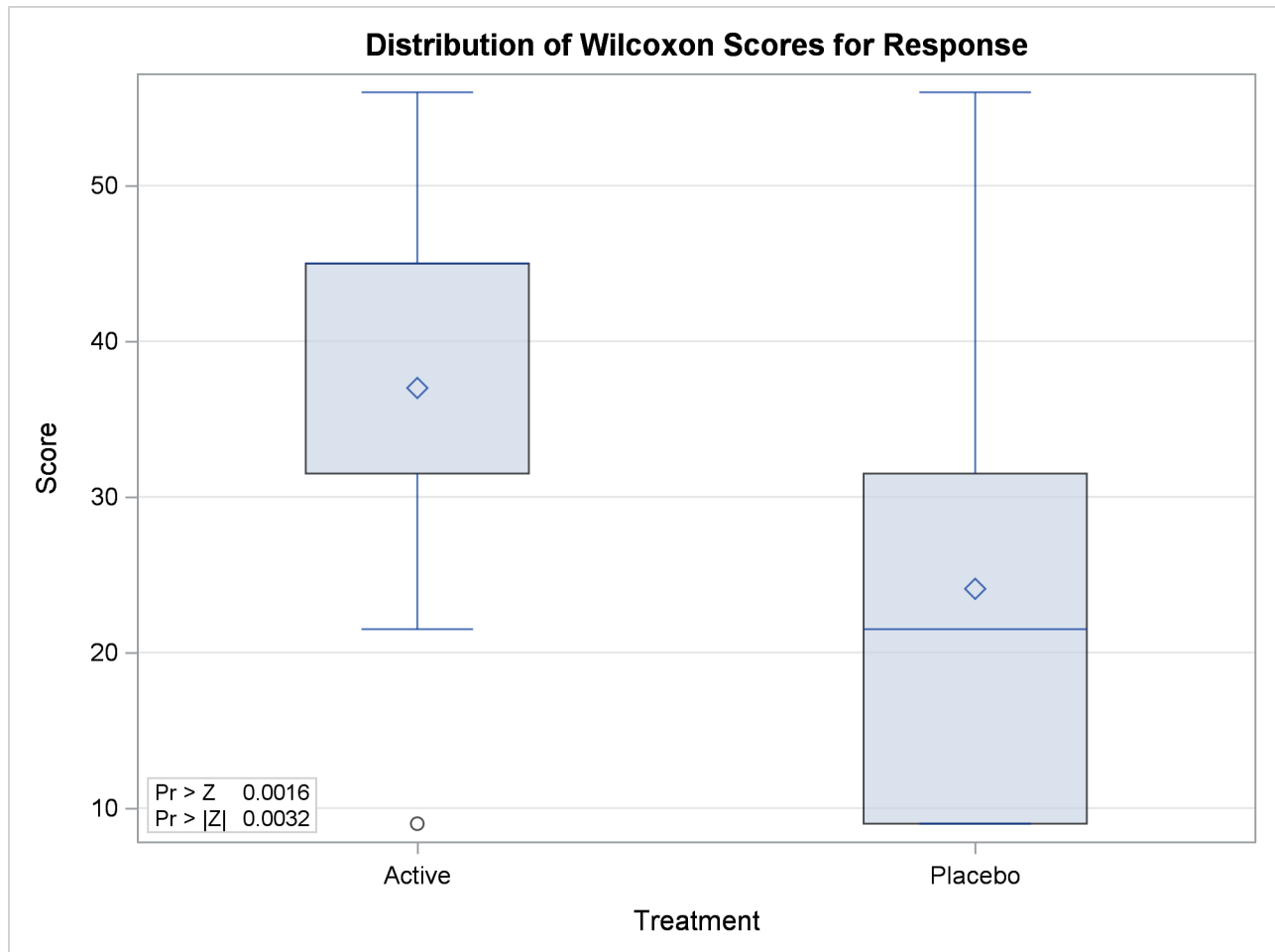
Output 83.1.2 Box Plot of Wilcoxon Scores
