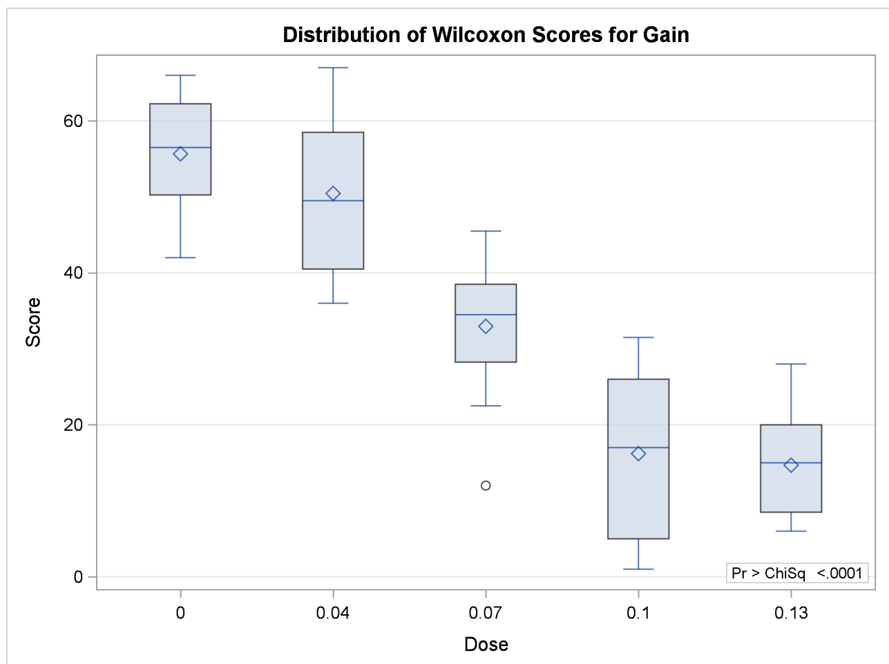
Figure 83.7 Box Plot of Wilcoxon Scores
