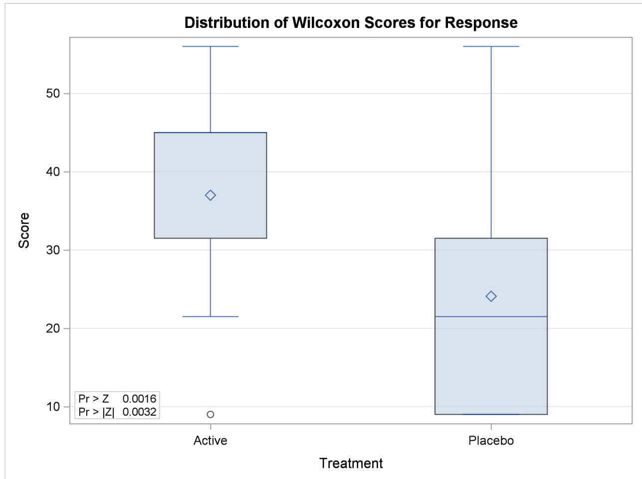
Output 83.1.2 Box Plot of Wilcoxon Scores
