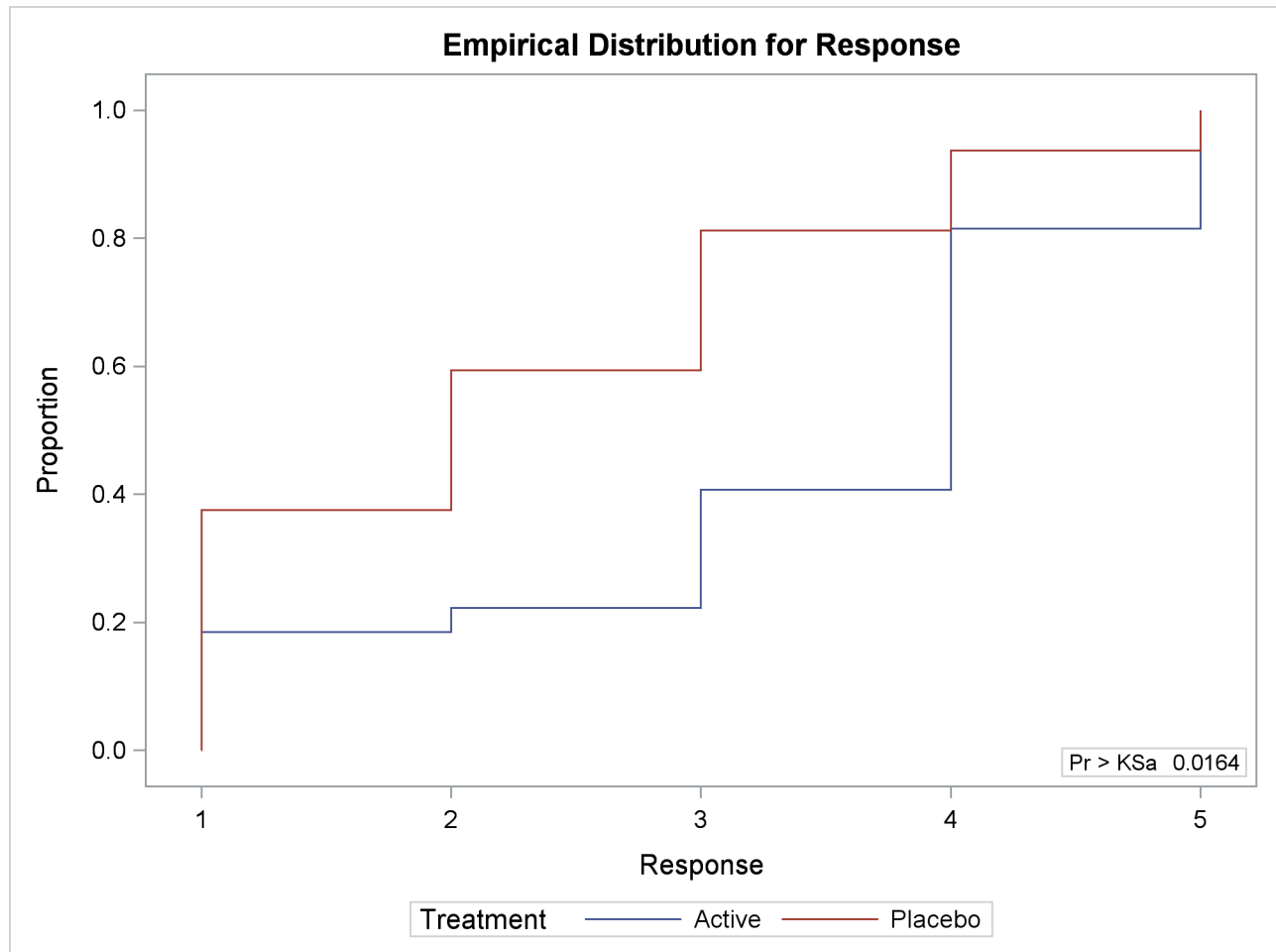
Output 83.2.2 Empirical Distribution Function Plot
