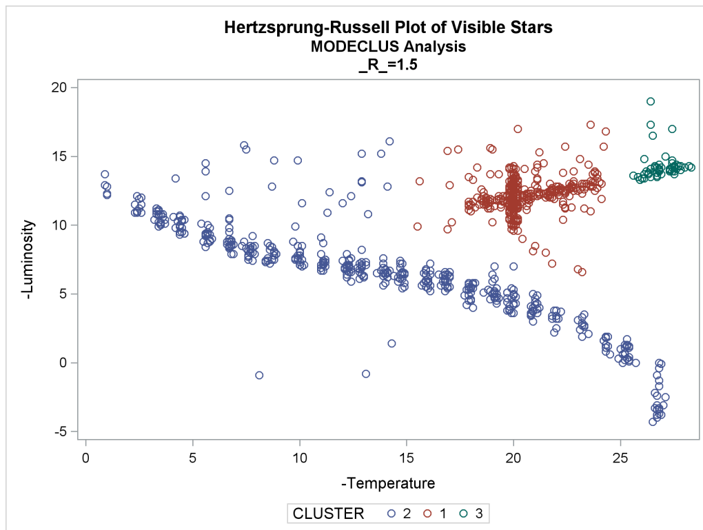
Output 78.4.4 Scatter Plots of Cluster Memberships by \_R_=1.5
