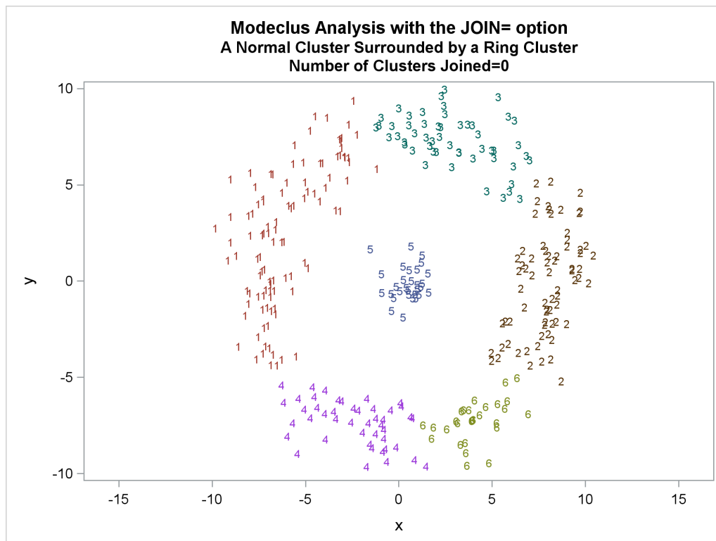
Output 78.3.3 Cluster Memberships When Number of Clusters Joined=0
