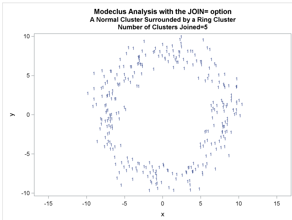
Output 78.3.8 Cluster Memberships When Number of Clusters Joined=5
