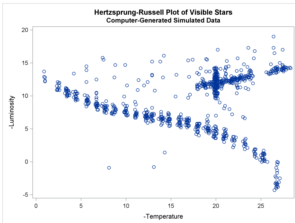
Output 78.4.1 Scatter Plot of Data
