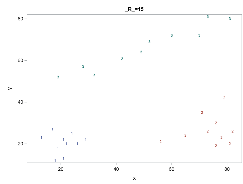
Figure 78.7 Scatter Plots of Cluster Memberships with _R_=15
