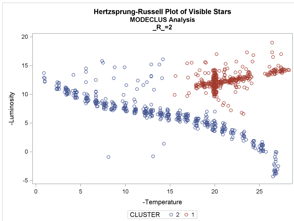
Output 78.4.5 Scatter Plots of Cluster Memberships by \_R_=2
