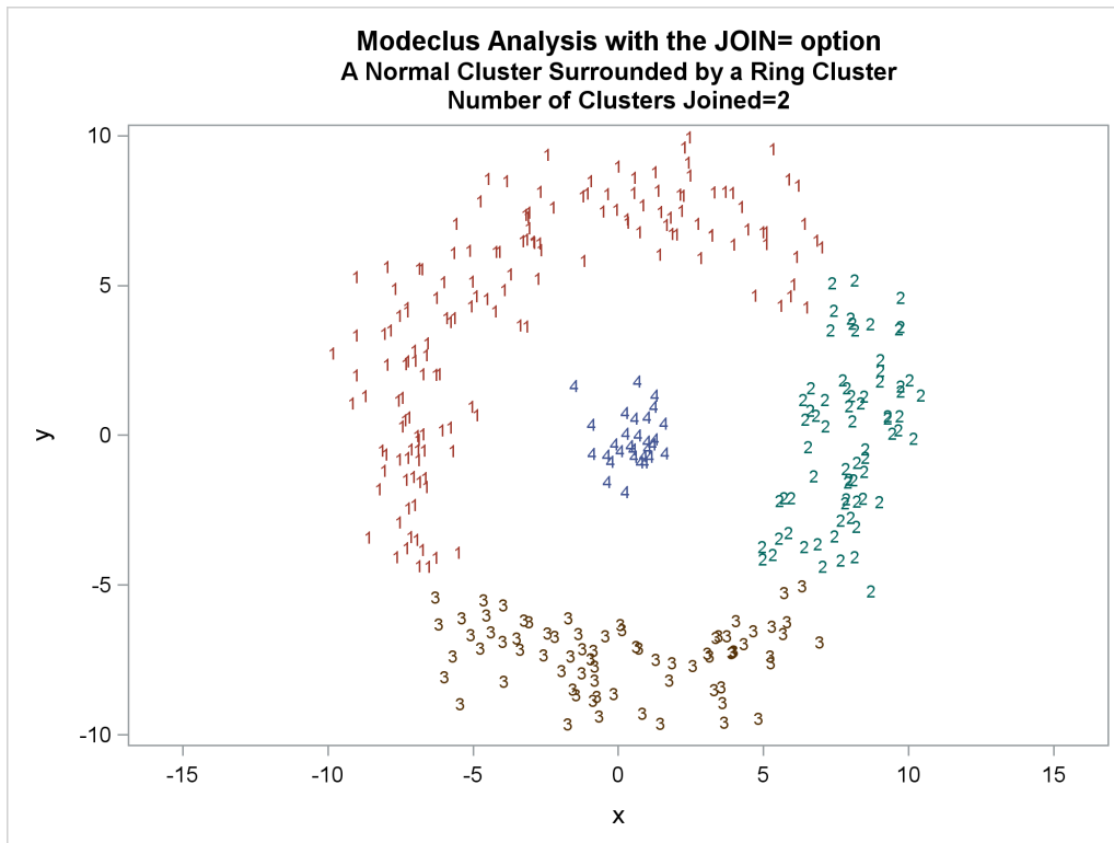
Output 78.3.5 Cluster Memberships When Number of Clusters Joined=2
