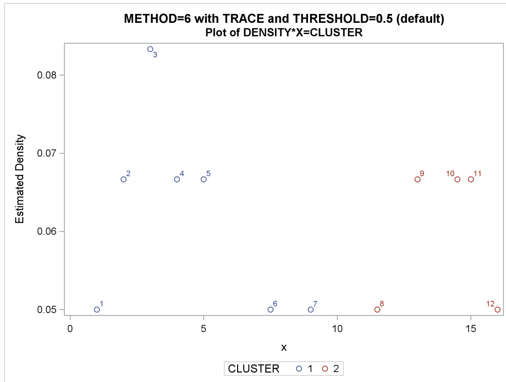
Output 78.5.2 Density Plot
