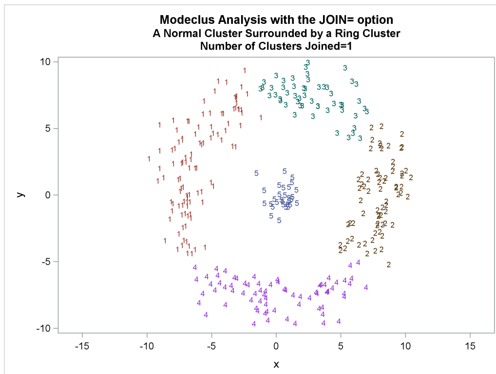
Output 78.3.4 Cluster Memberships When Number of Clusters Joined=1
