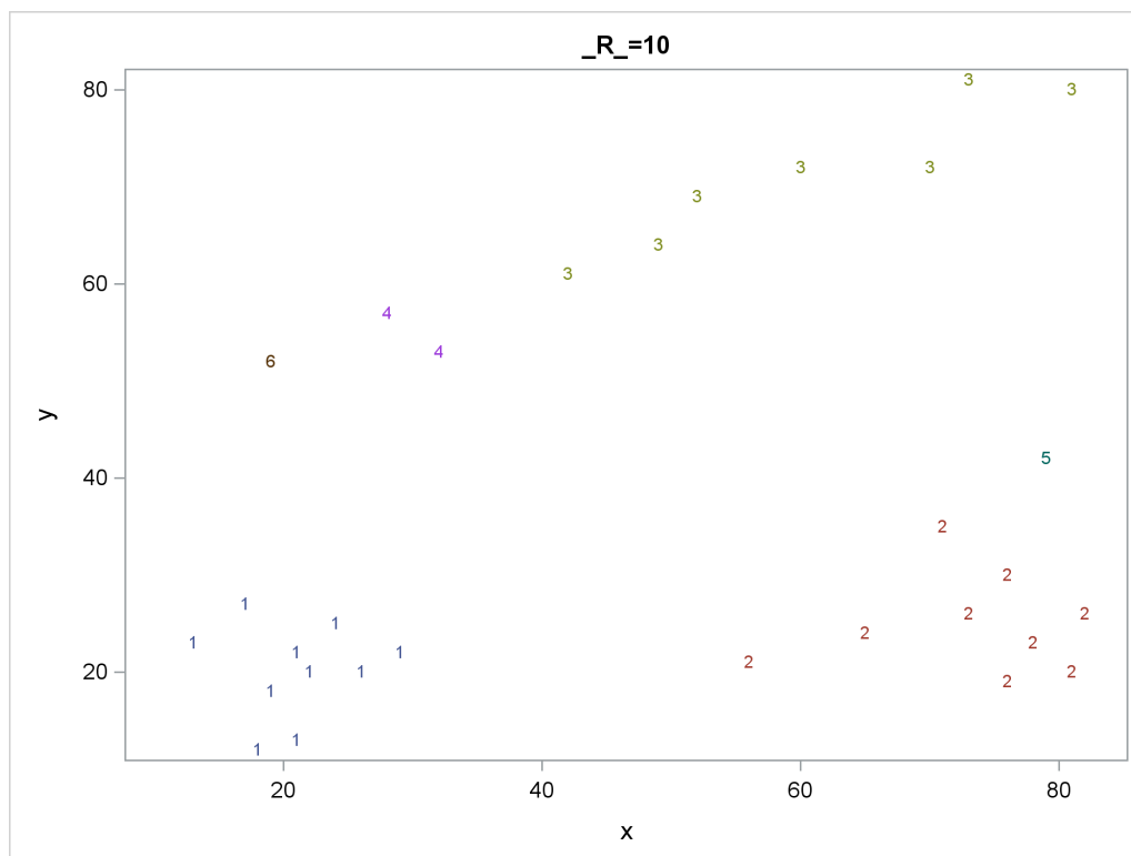
Figure 78.6 Scatter Plots of Cluster Memberships with _R_=10
