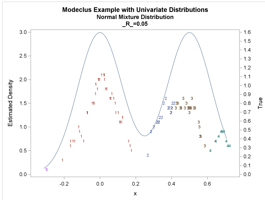
Output 78.1.16 True Density, Estimated Density, and Cluster Membership by Various \_R\_ = Values
