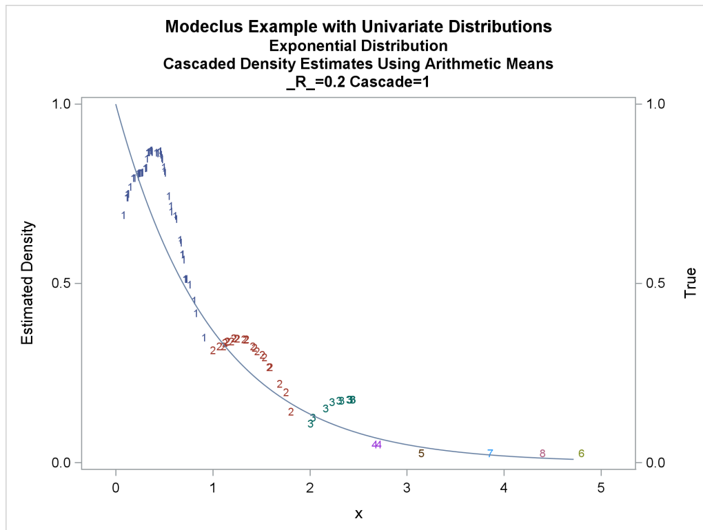
Output 78.1.12 True Density, Estimated Density, and Cluster Membership by \_R_=0.2 with Various \_CASCAD\_ Values
