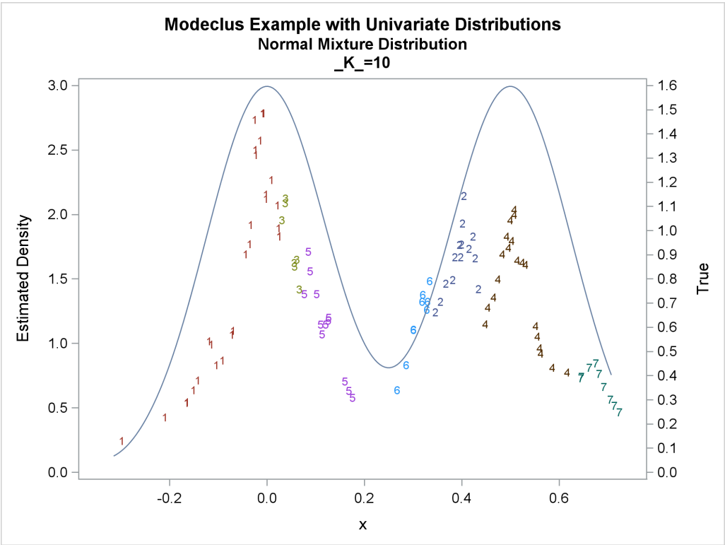
Output 78.1.14 True Density, Estimated Density, and Cluster Membership by Various _K_ Values
