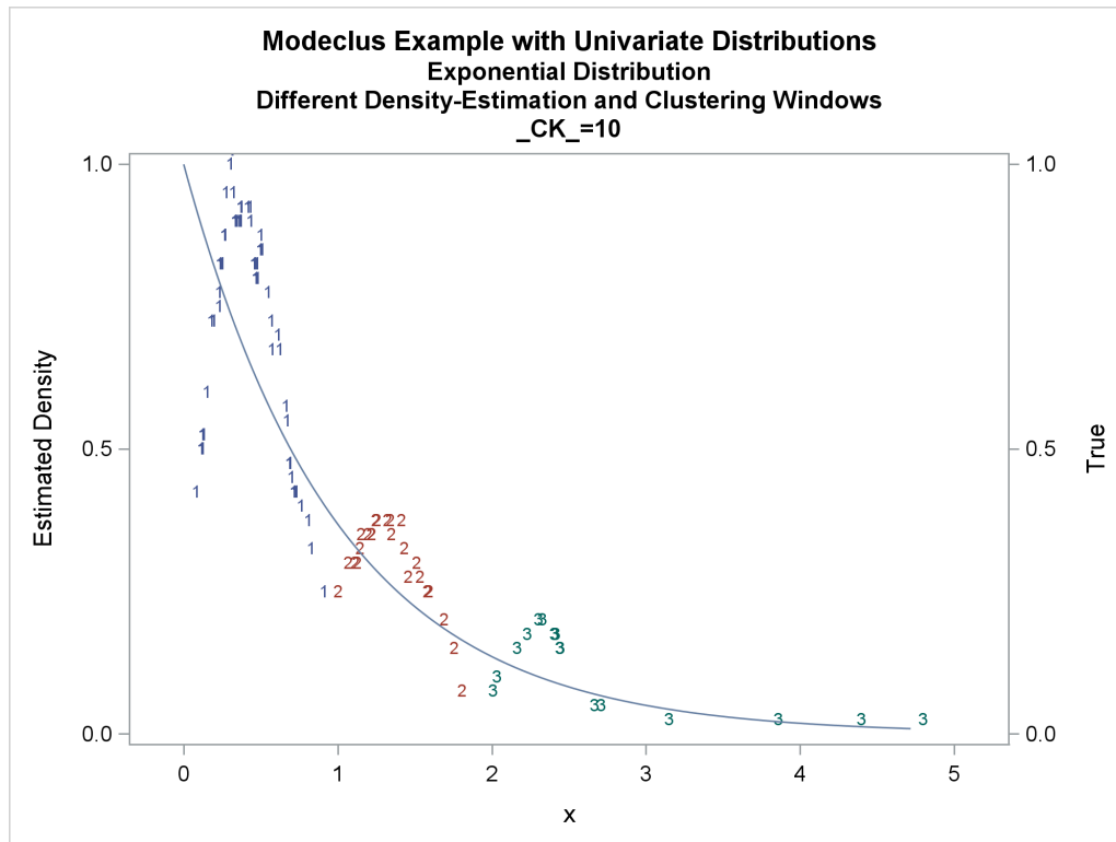
Output 78.1.10 True Density, Estimated Density, and Cluster Membership by \_R_=0.2 with Various \_CK\_ Values
