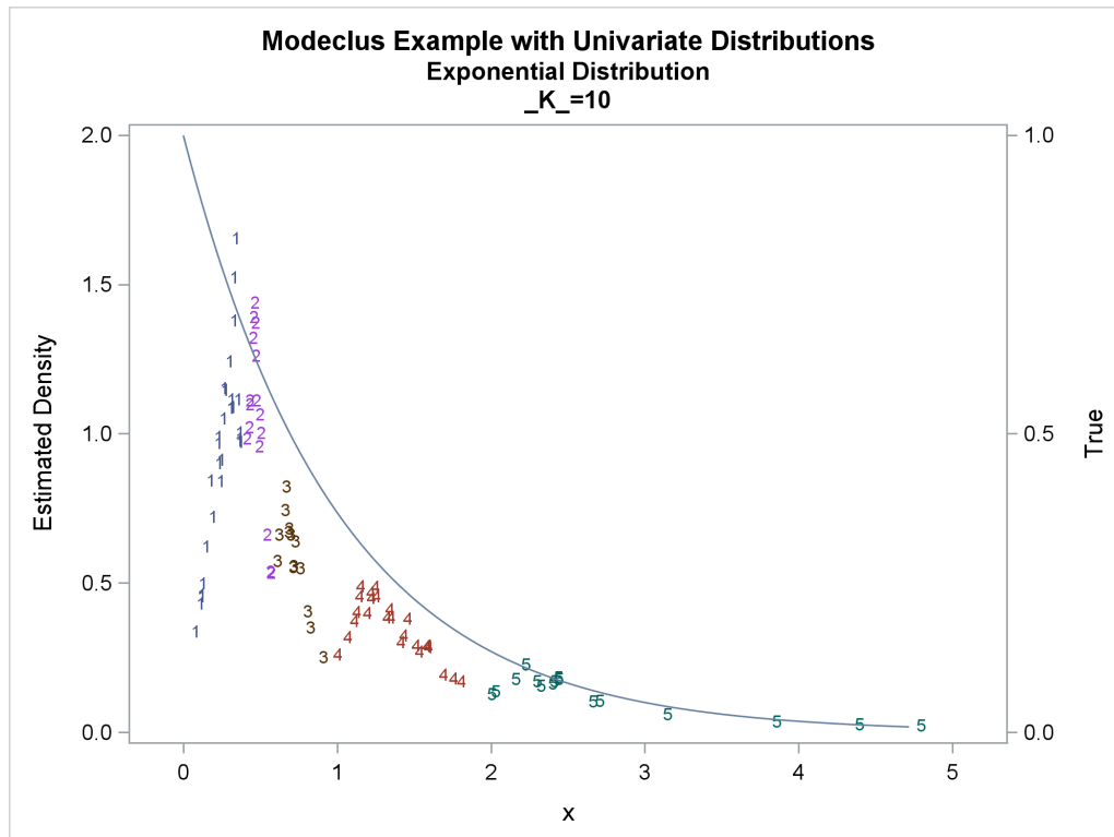
Output 78.1.6 True Density, Estimated Density, and Cluster Membership by Various _K_ Values
