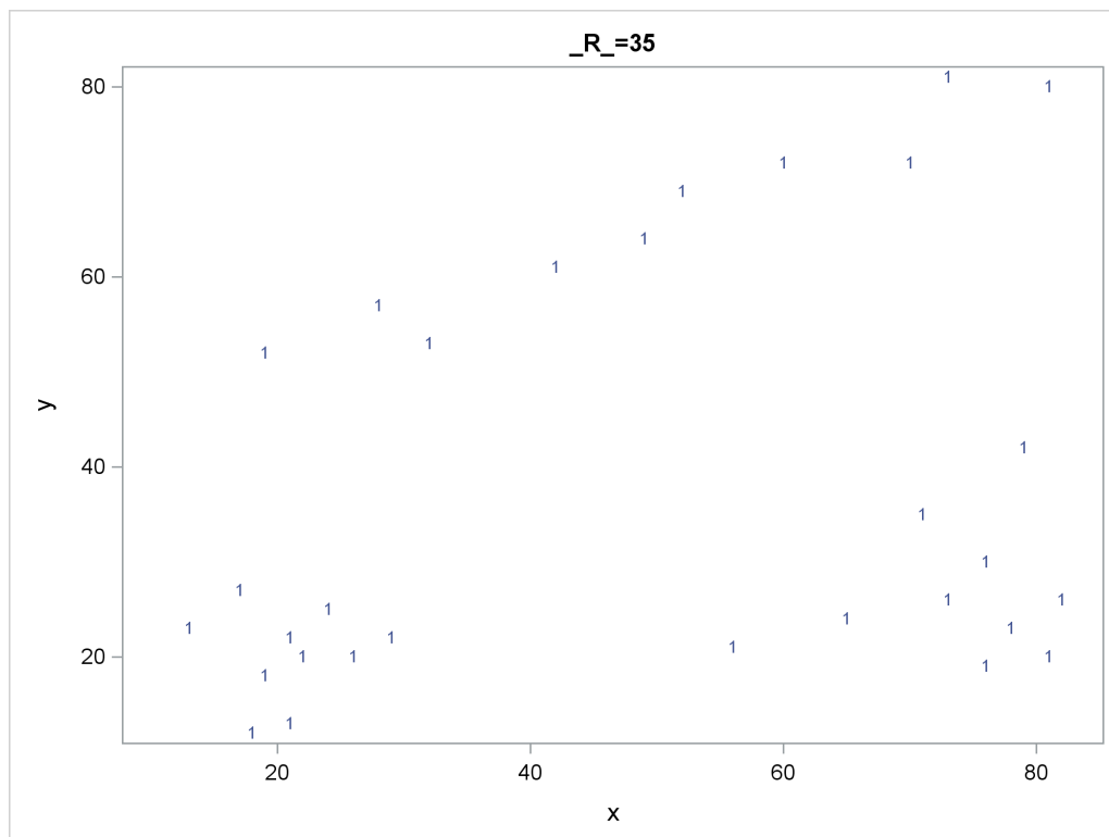
Figure 78.8 Scatter Plots of Cluster Memberships with _R_=35
