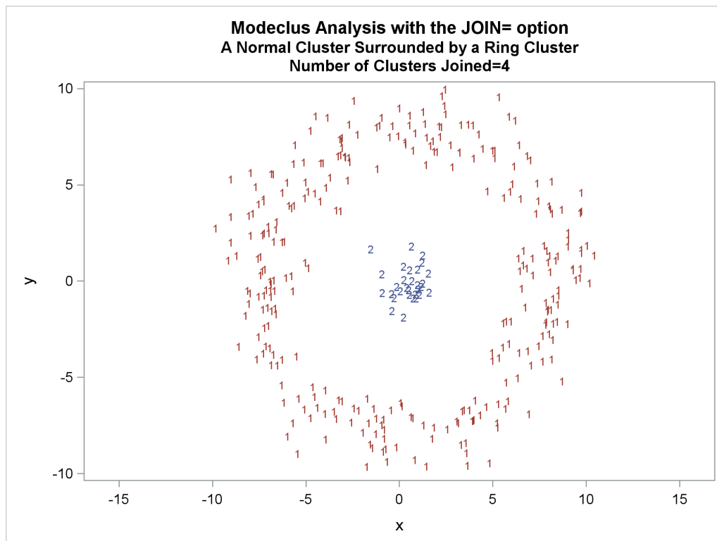
Output 78.3.7 Cluster Memberships When Number of Clusters Joined=4
