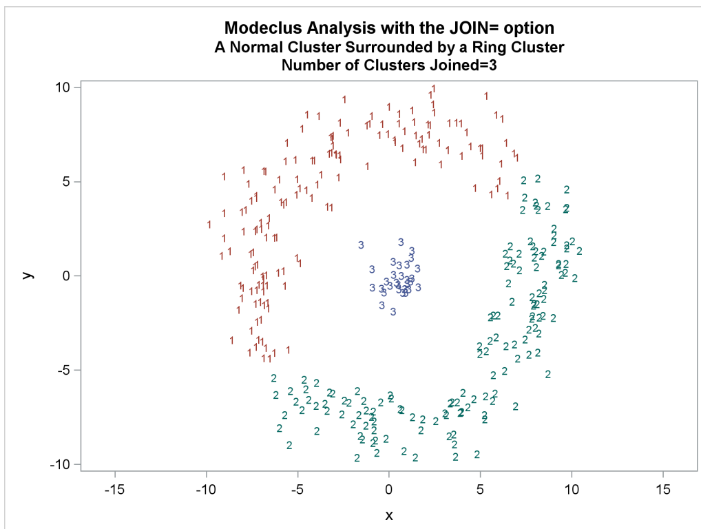
Output 78.3.6 Cluster Memberships When Number of Clusters Joined=3
