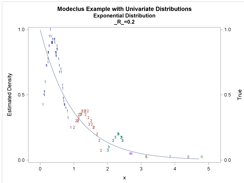
Output 78.1.8 True Density, Estimated Density, and Cluster Membership by Various \_R\_ Values
