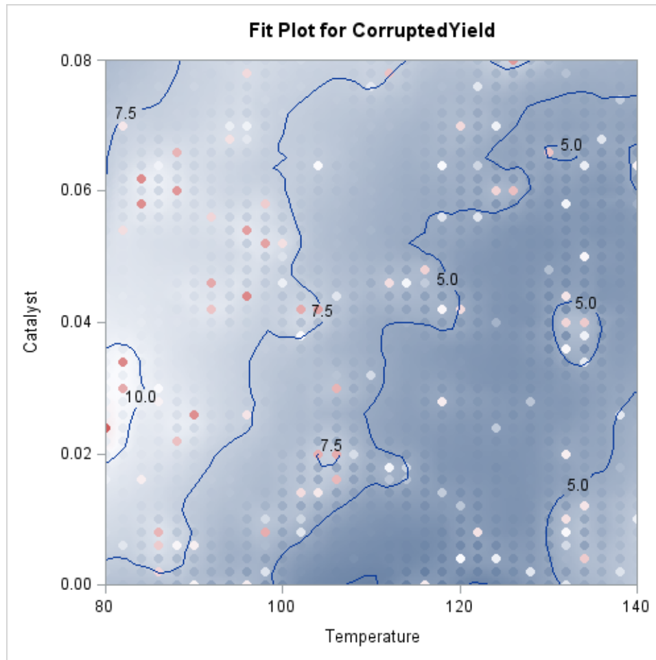
Output 71.3.4 Fit for CorruptedYield
