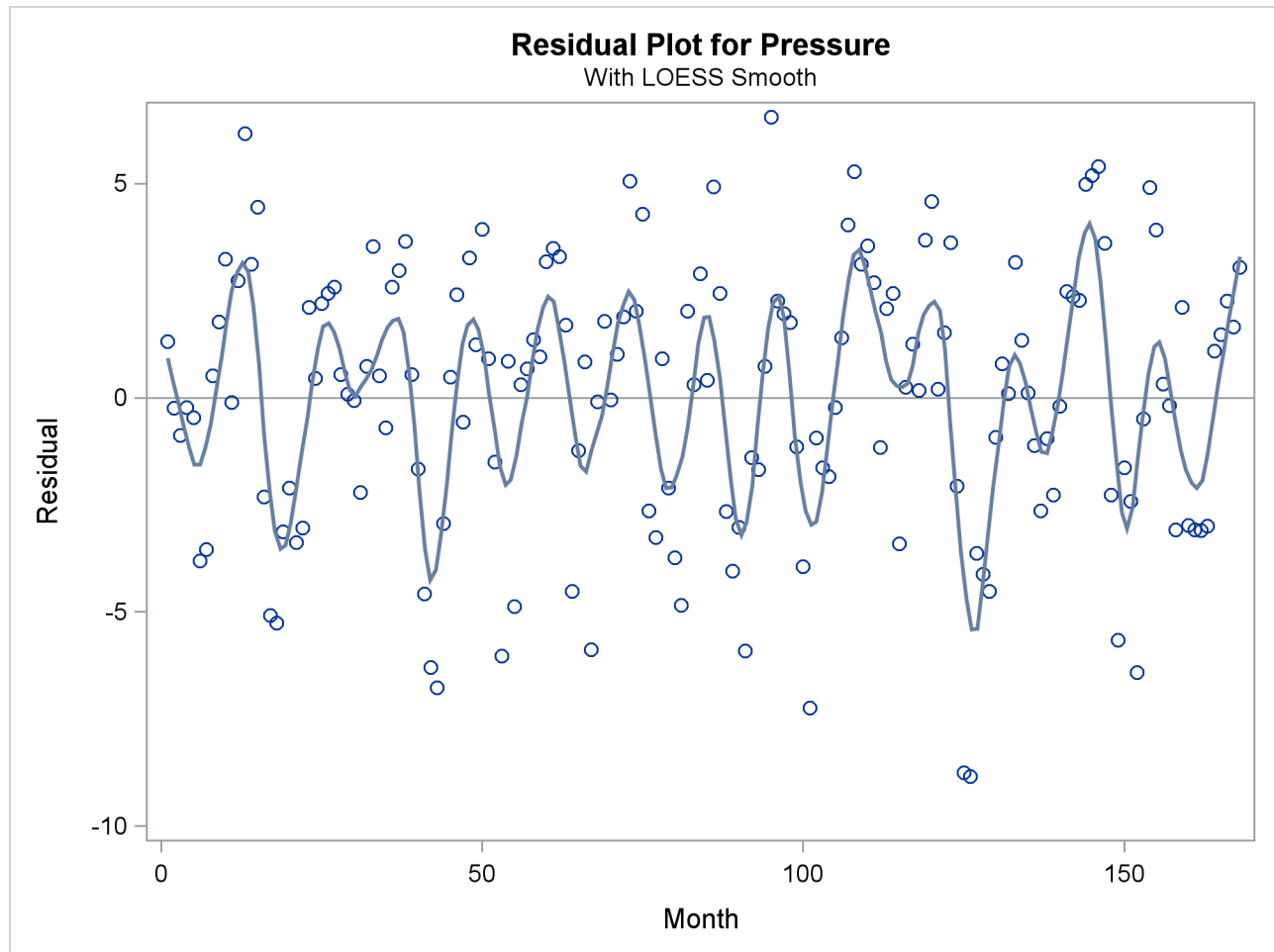
Output 71.4.4 Residuals for the Loess Fit for the ENSO Data
