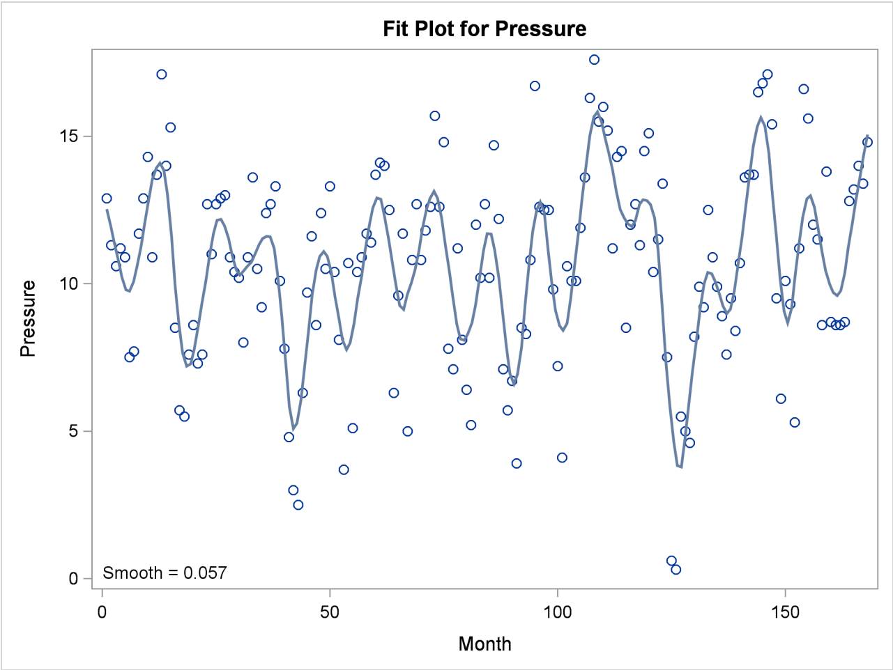
Output 71.4.8 Loess Fit Showing an Annual Cycle
