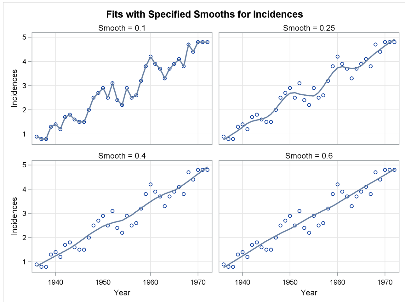
Figure 71.9 Loess Fits for a Range of Smoothing Parameters
