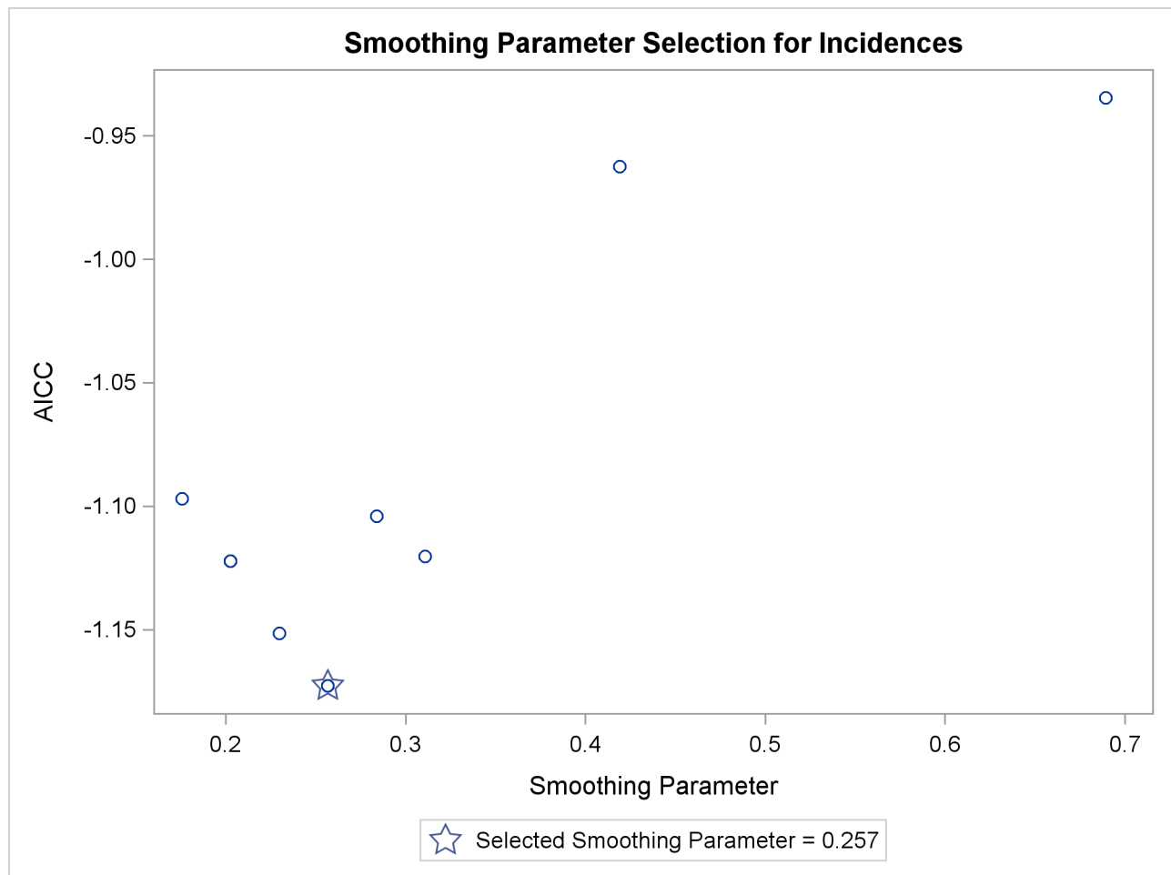
Figure 71.6 AICC Criterion by Smoothing Parameter
