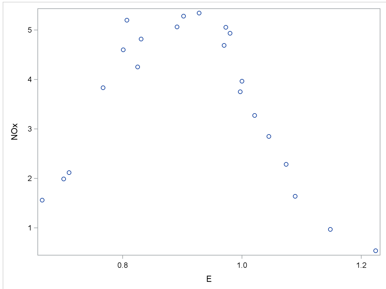
Output 71.1.1 Scatter Plot of the Gas Data
