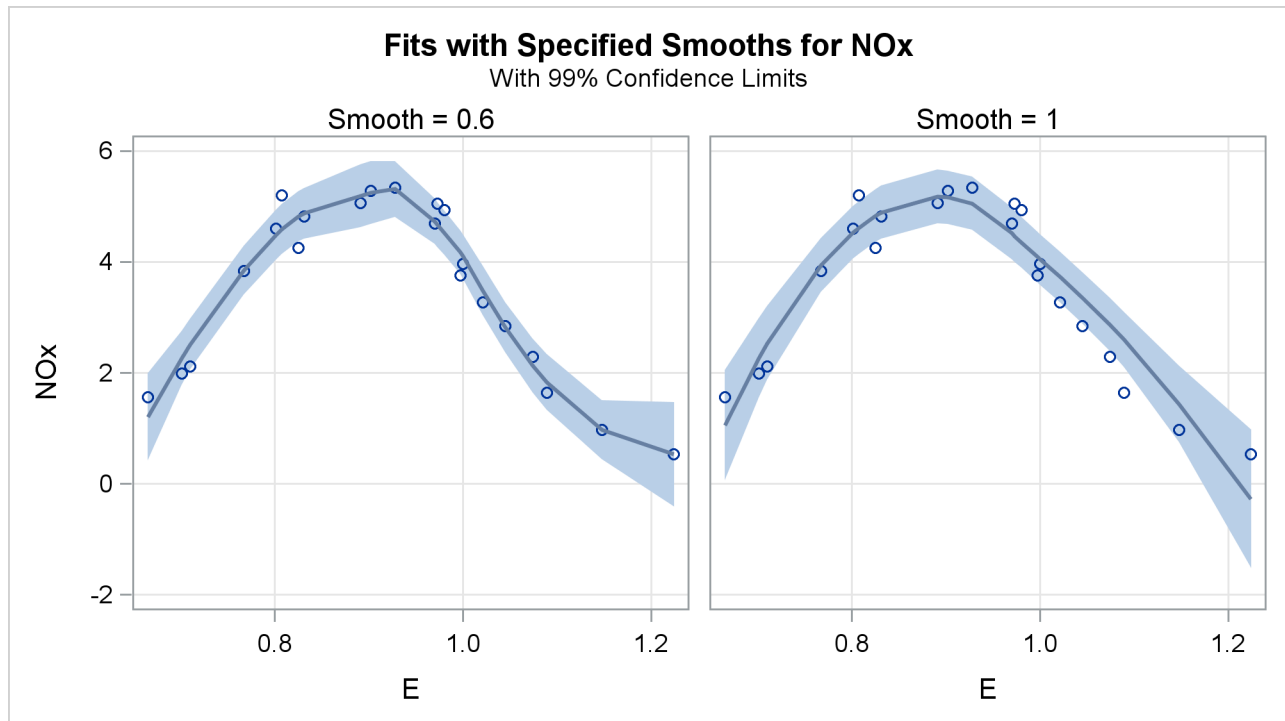
Output 71.1.5 Loess Fits with 99% Confidence Limits for the Gas Data
