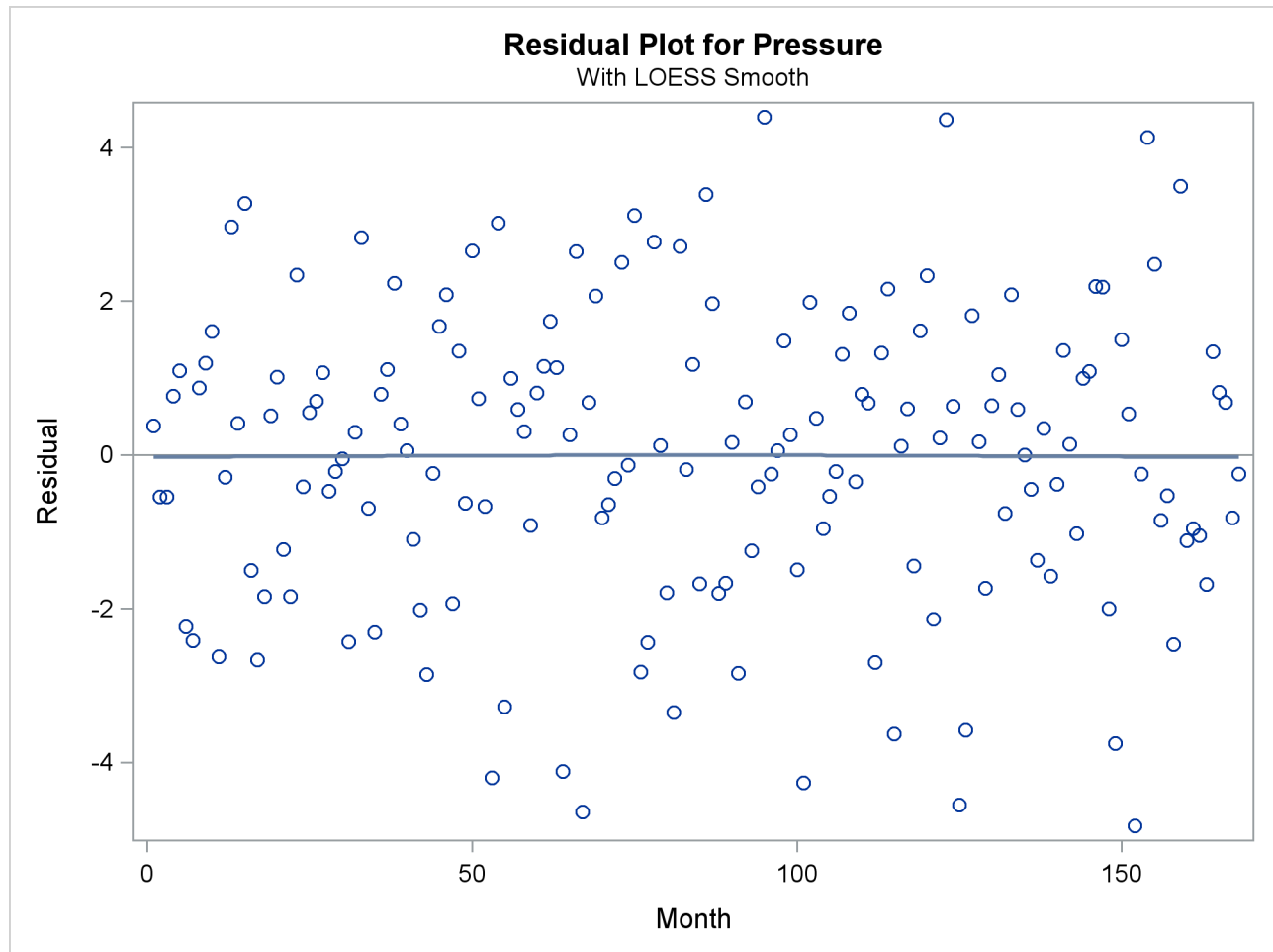
Output 71.4.9 Residuals of the Selected Model
