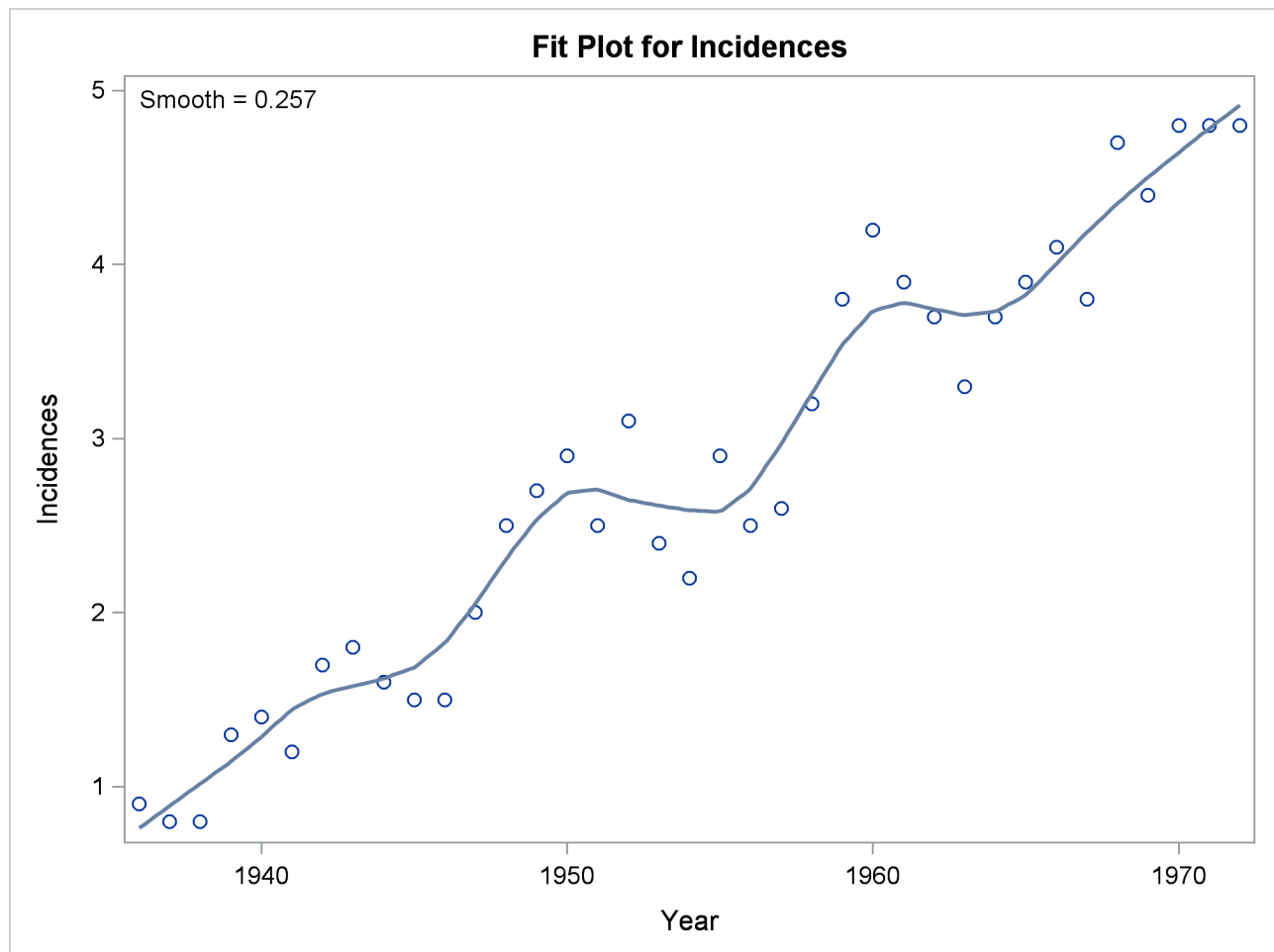
Figure 71.2 Default Loess Fit for the Melanoma Data
