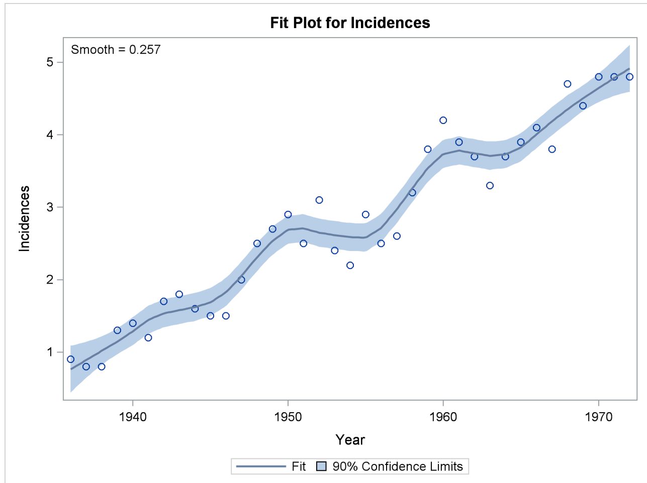
Figure 71.13 Loess Fit of Melanoma Data with 90% Confidence Limits
