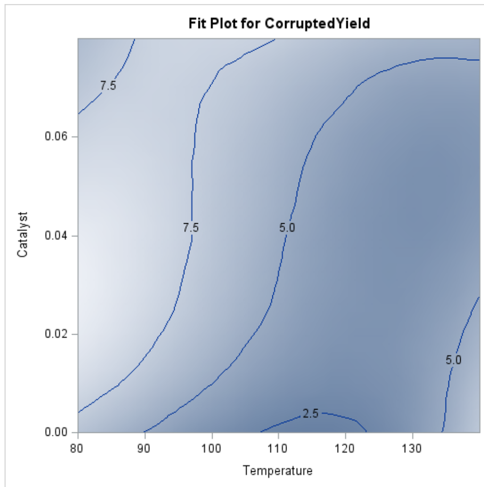
Output 71.3.6 Robust Fit for CorruptedYield with Observations Suppressed
