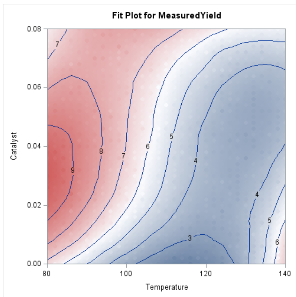
Output 71.3.3 Fit for MeasuredYield
