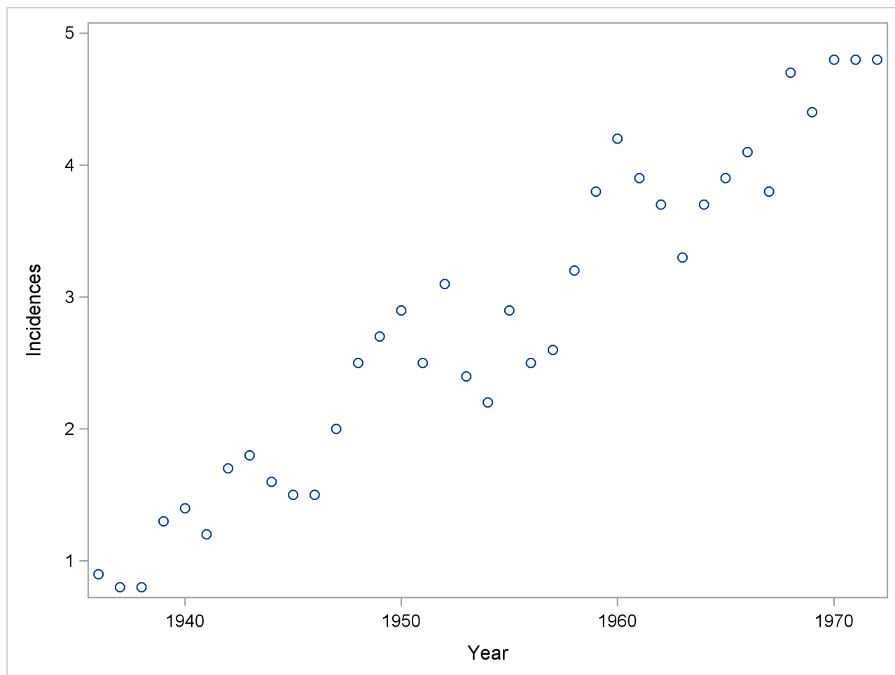
Figure 71.1 Scatter Plot of the Melanoma Data
