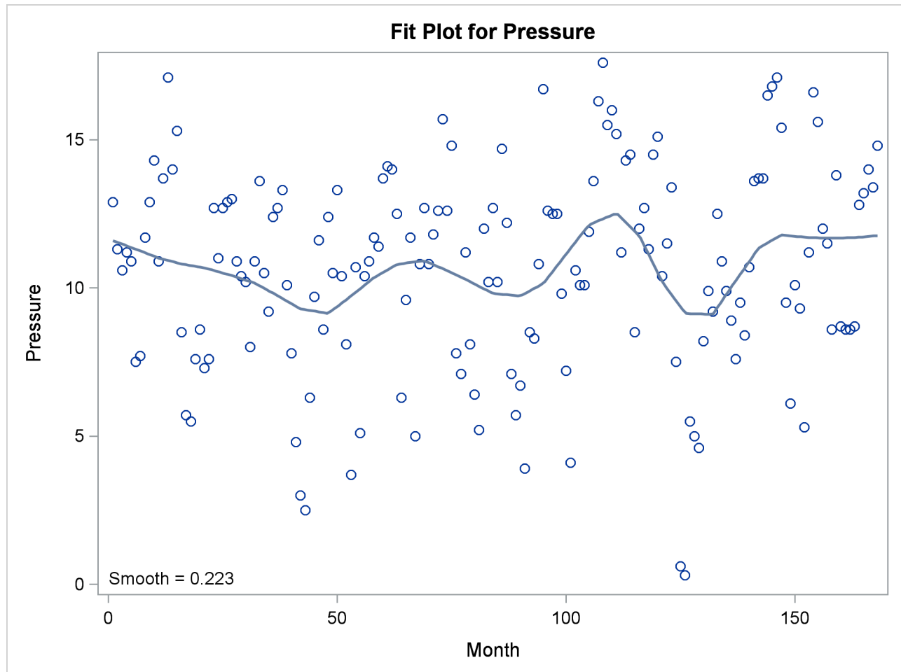
Output 71.4.3 Oversmoothed Loess Fit for the ENSO Data
