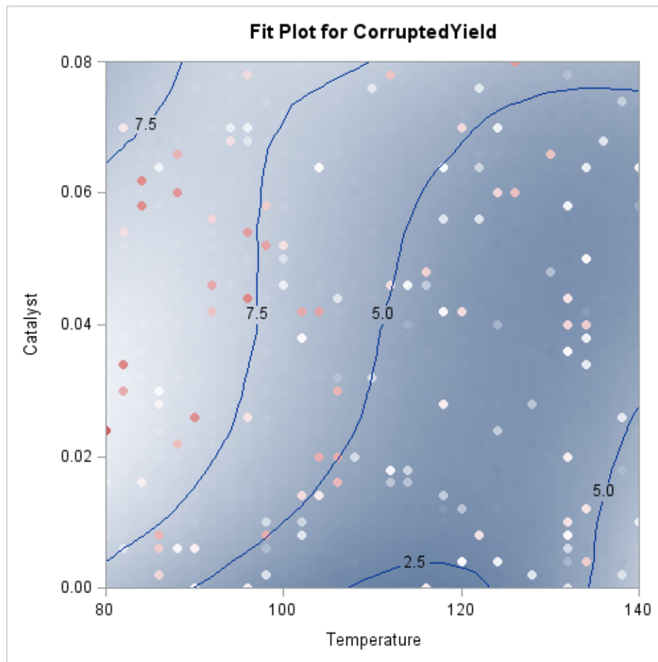
Output 71.3.5 Robust Fit for CorruptedYield
