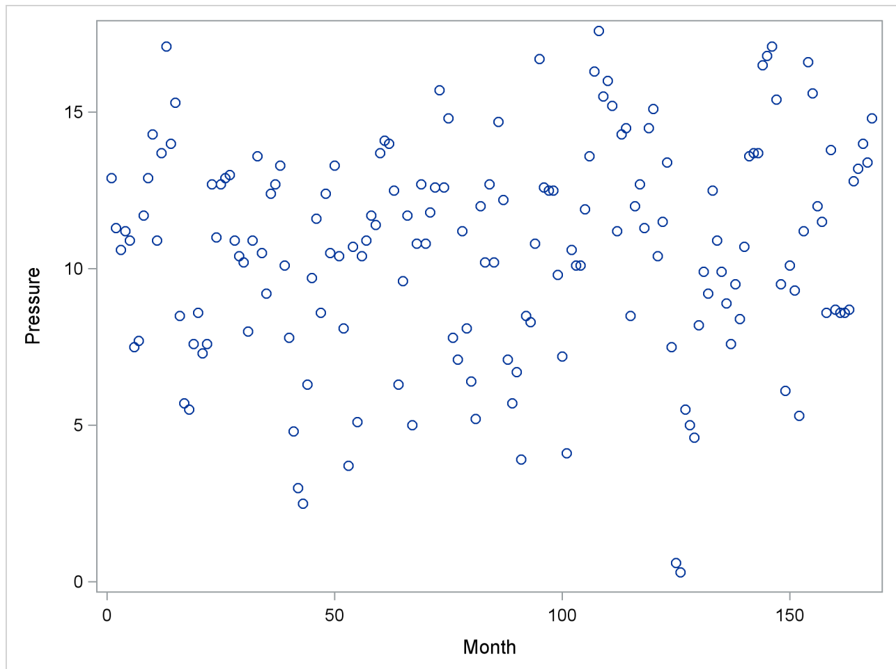
Output 71.4.1 Scatter Plot of ENSO Data
