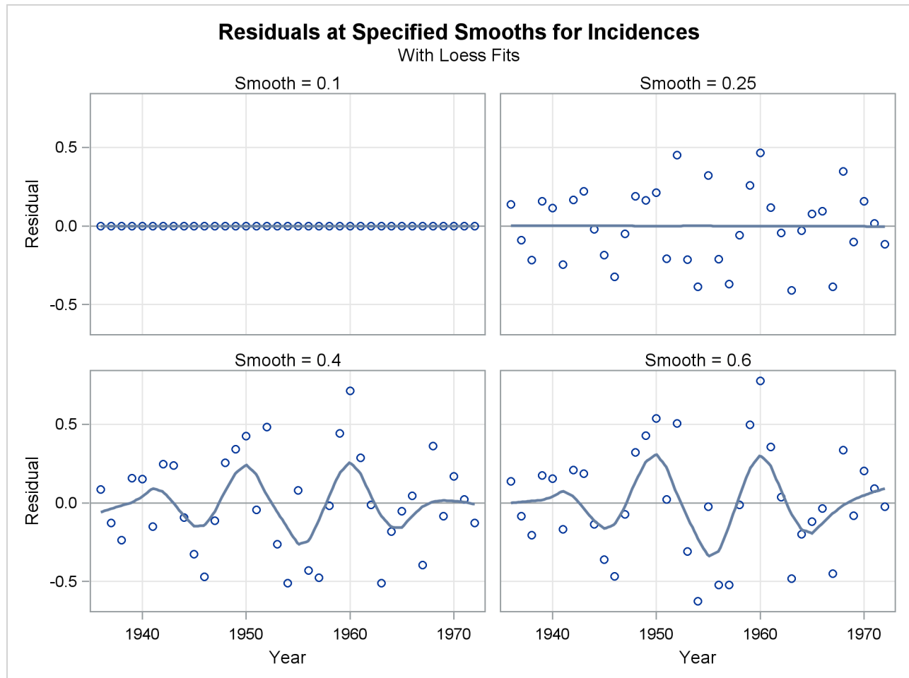
Figure 71.11 Residuals with Superimposed Loess Fits
