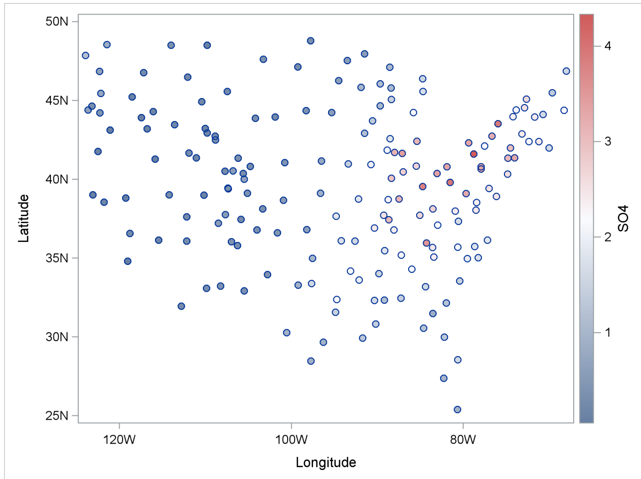
Output 71.2.1 Sulfate Measurements
