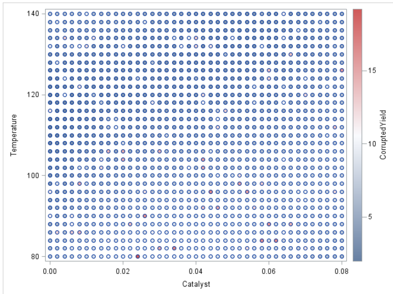
Output 71.3.1 Scatter Plot of Experiment Data Colored by CorruptedYield
