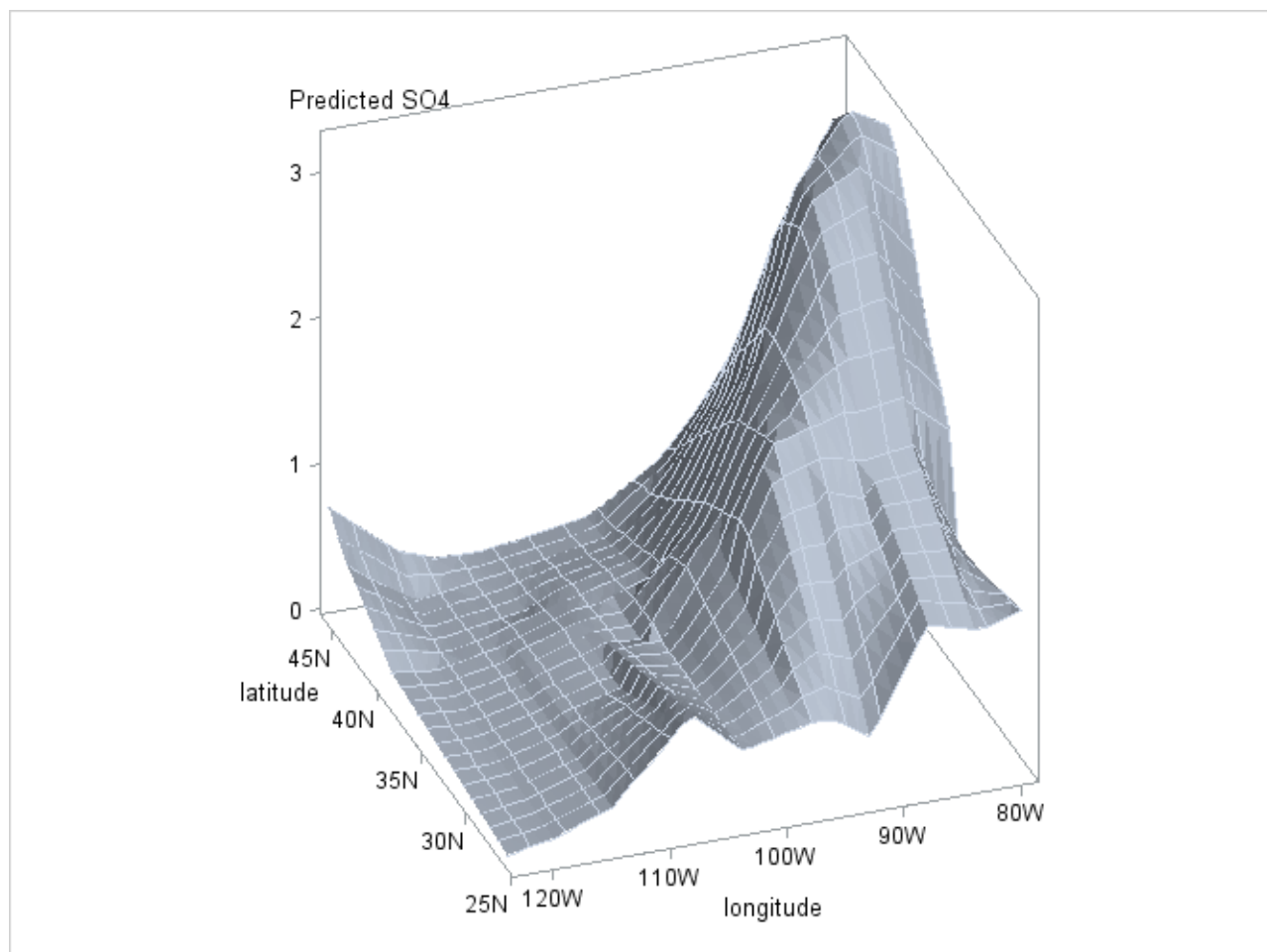
Output 71.2.3 Loess Fit of SO 4 Surface
