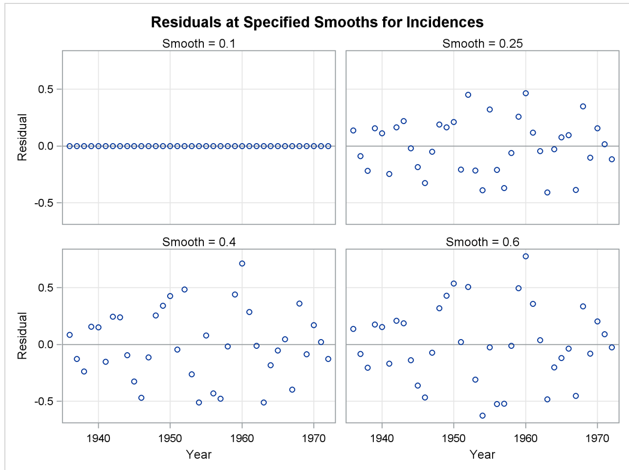
Figure 71.10 Residuals of Loess Fits for a Range of Smoothing Parameters
