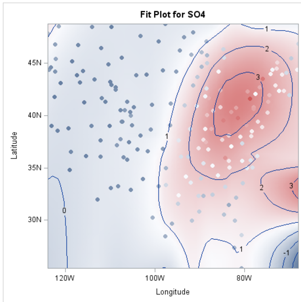
Output 71.2.2 Fit Plot for the SO 4 Data
