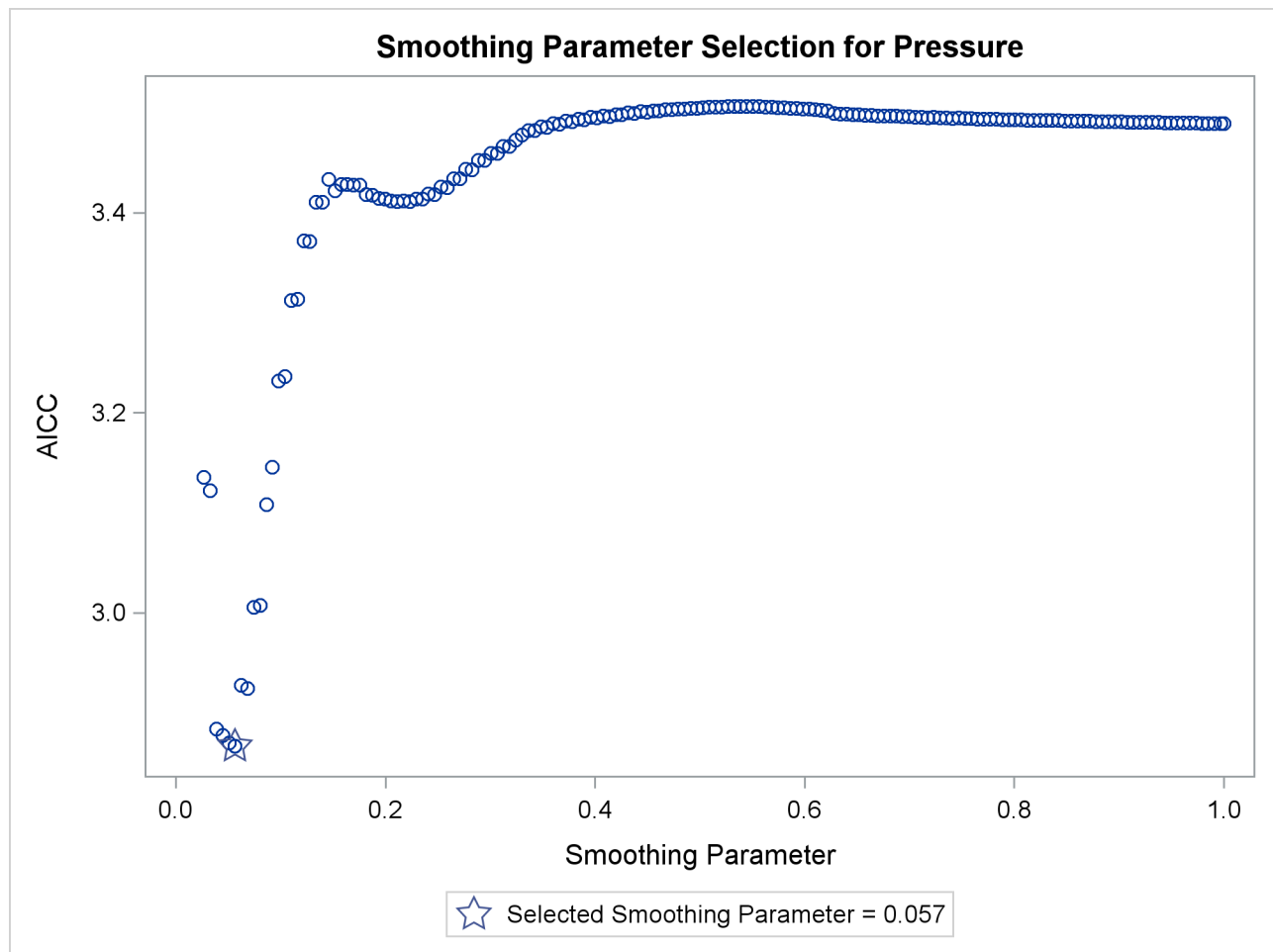
Output 71.4.5 AICC versus Smoothing Parameter Showing Local Minima
