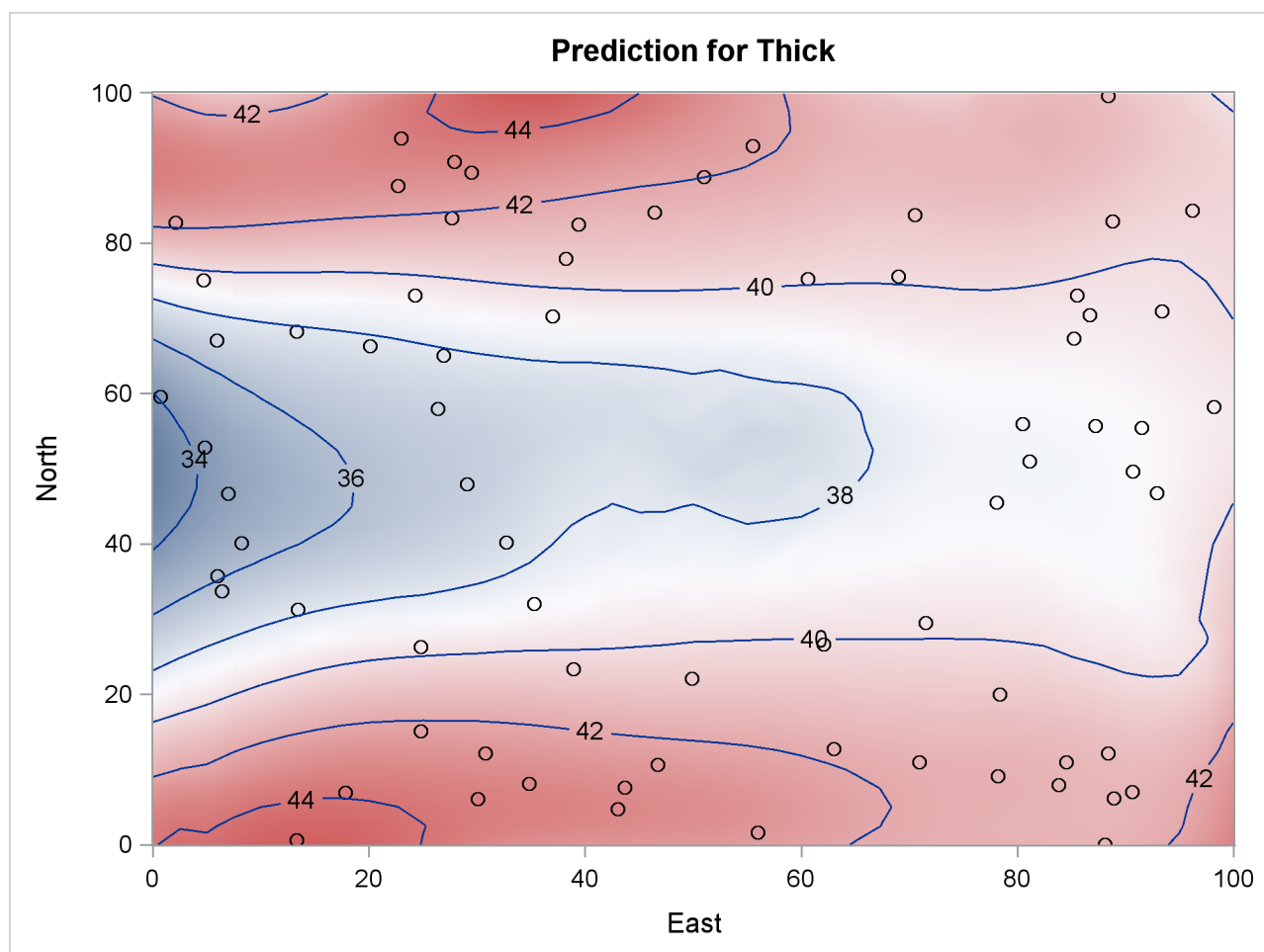
Output 67.3.3 Surface Plot and Contours of Kriged Coal Seam Thickness
