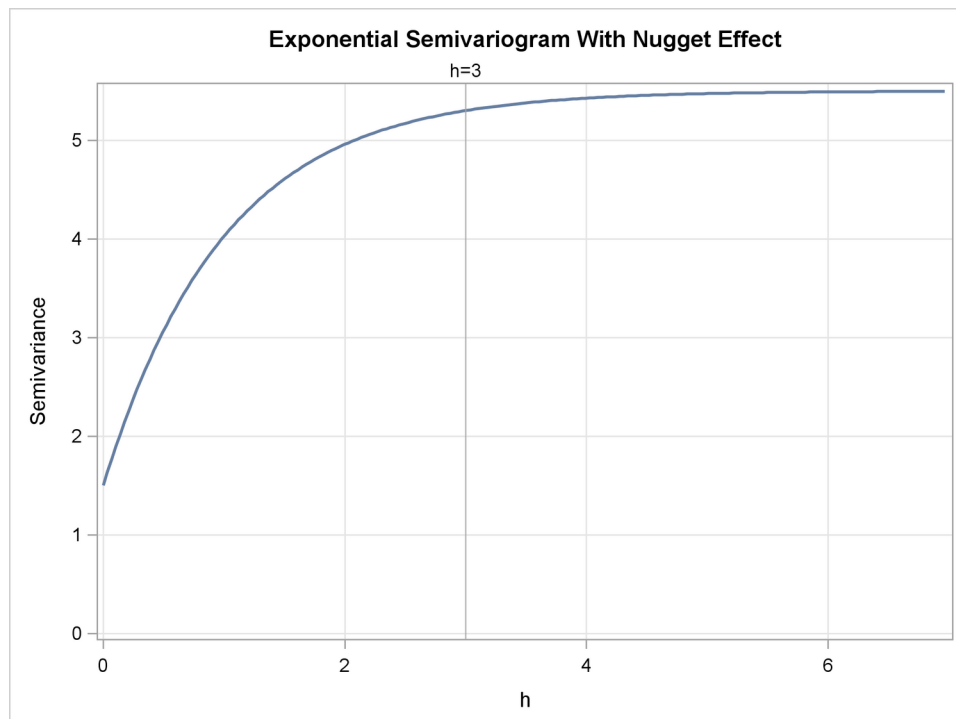
Figure 67.11 Exponential Semivariogram Model with a Nugget Effect c_n = 1.5
