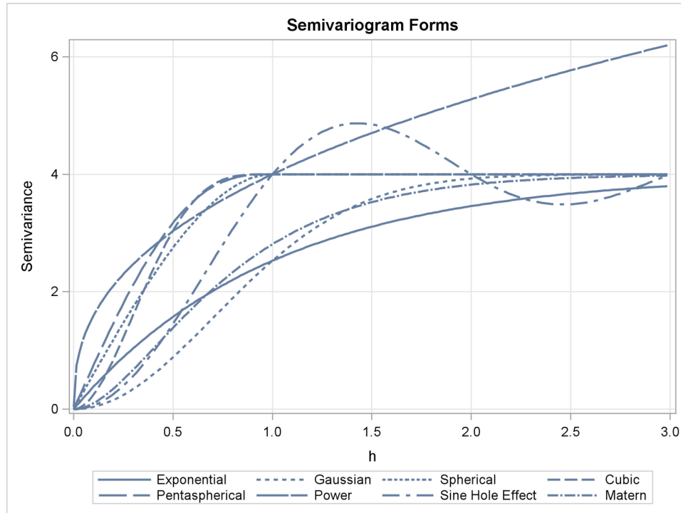
Figure 67.9 Semivariogram Forms Used in PROC KRIGE2D
