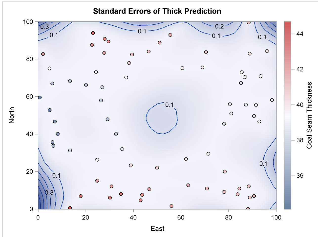
Output 67.3.4 Surface Plot and Contours of Prediction Standard Errors
