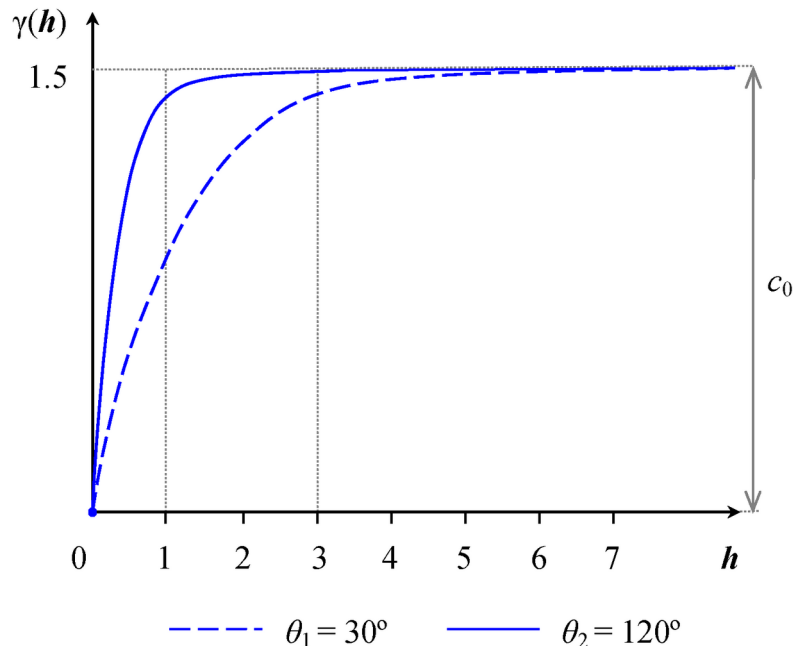
Figure 67.12 Geometric Anisotropy with Major Axis in the Direction \theta_1 = 30^\circ
