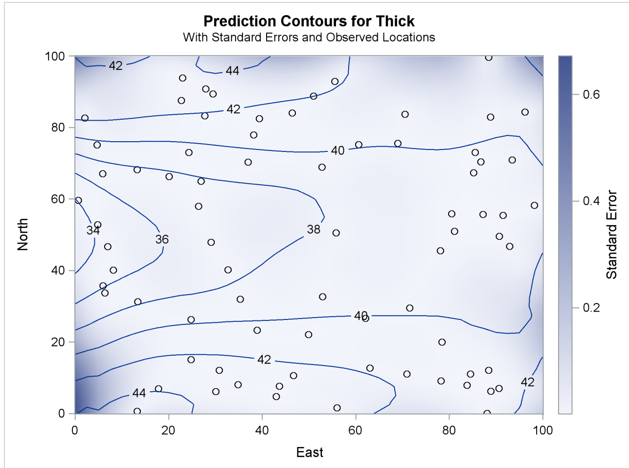
Figure 67.4 Contour Plot of Kriged Coal Seam Thickness
