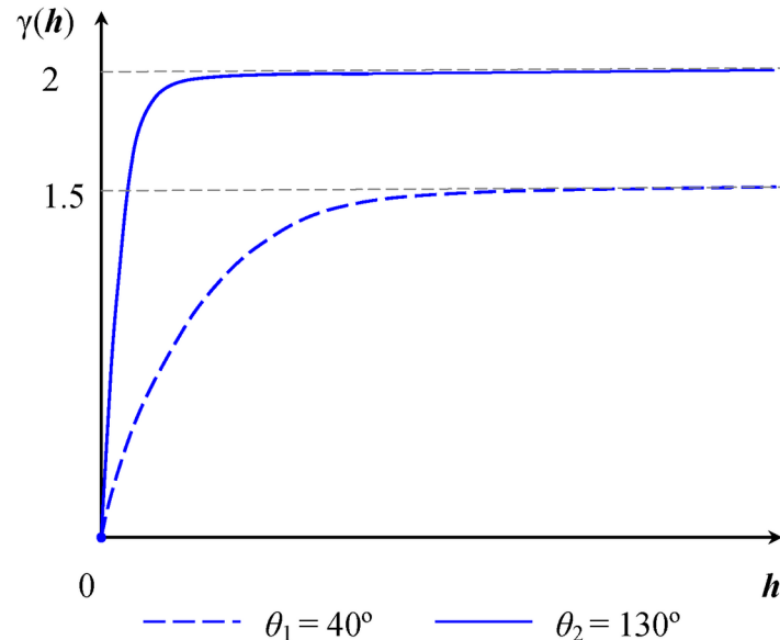
Figure 67.14 Zonal Anisotropy in Two Directions
