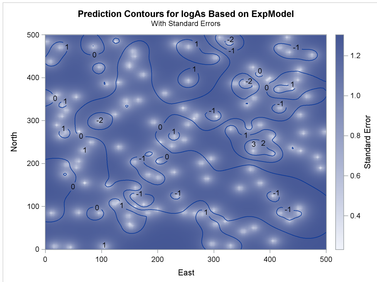
Output 67.1.10 Predicted Arsenic Logarithm Values with Exponential Covariance
