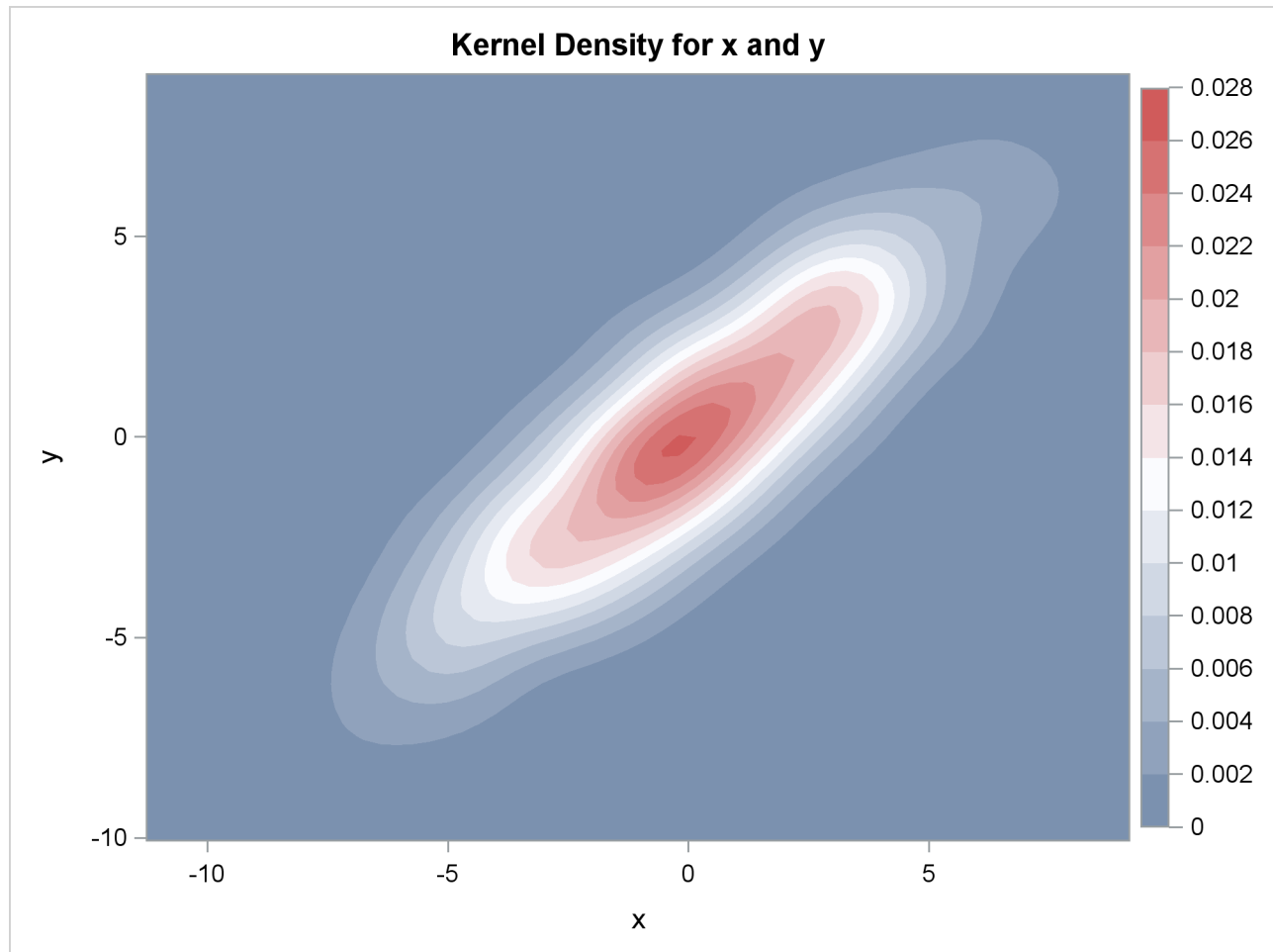
Figure 66.1 Contour Plot of Estimated Density
