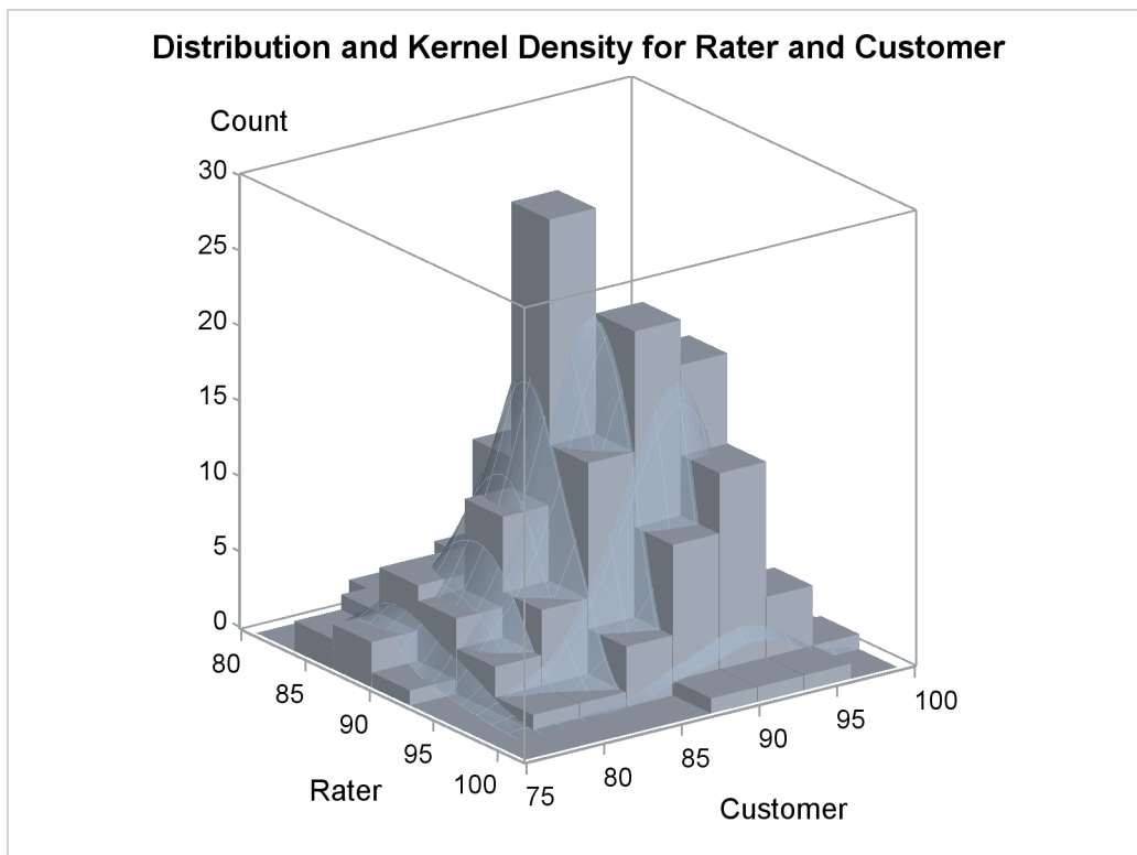
Output 66.6.6 Bivariate Histogram with Overlaid Surface Plot
