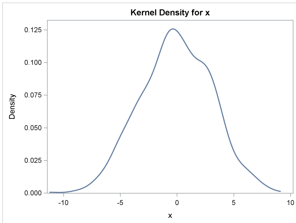
Output 66.5.1 Kernel Density Estimate
