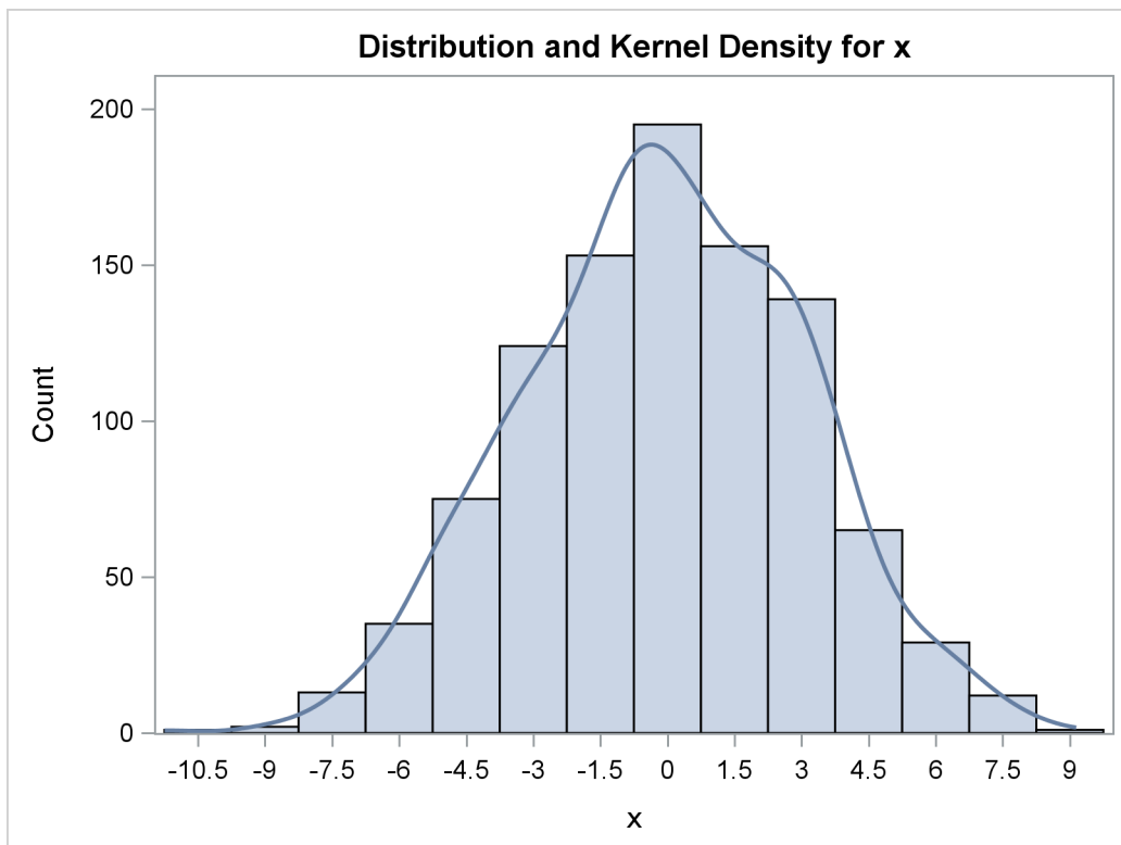
Output 66.5.3 Histogram with Overlaid Kernel Density Estimate
