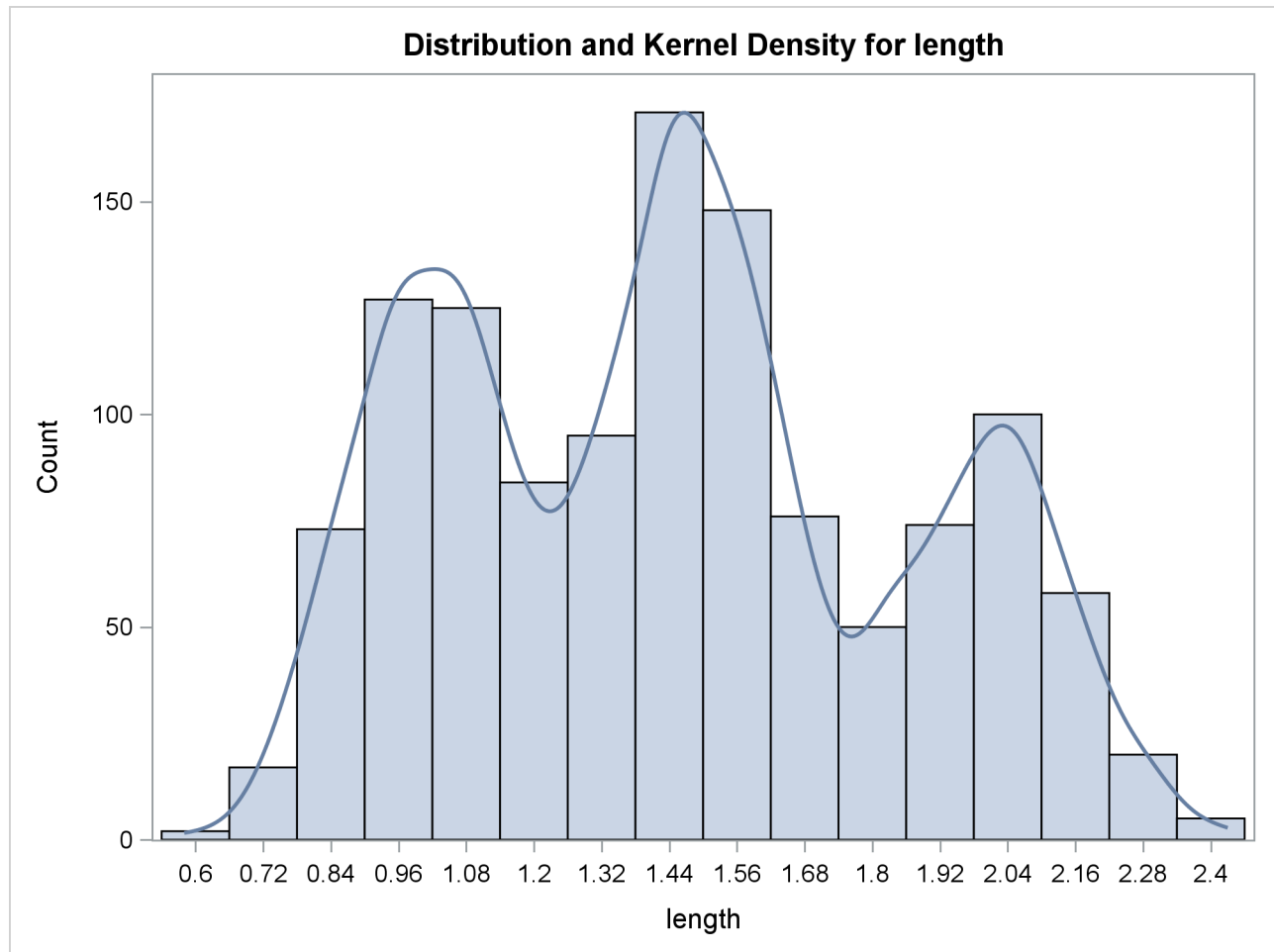
Output 66.1.1 Histogram with Overlaid Kernel Density Estimate
