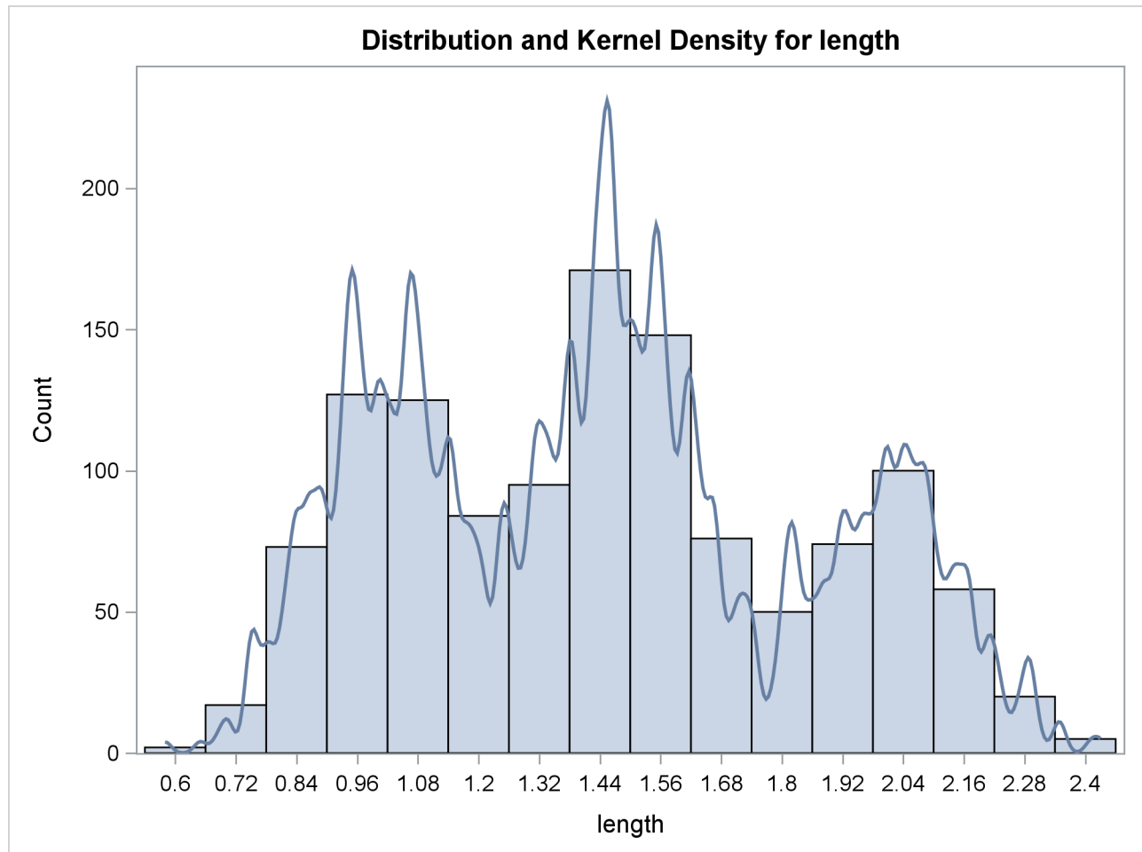
Output 66.2.2 Histogram with Undersmoothed Kernel Density Estimate
