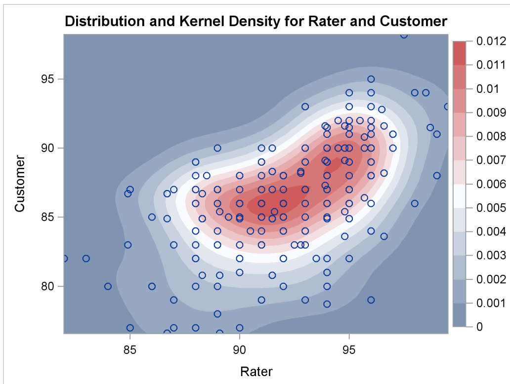
Output 66.6.4 Contour Plot with Overlaid Scatter Plot
