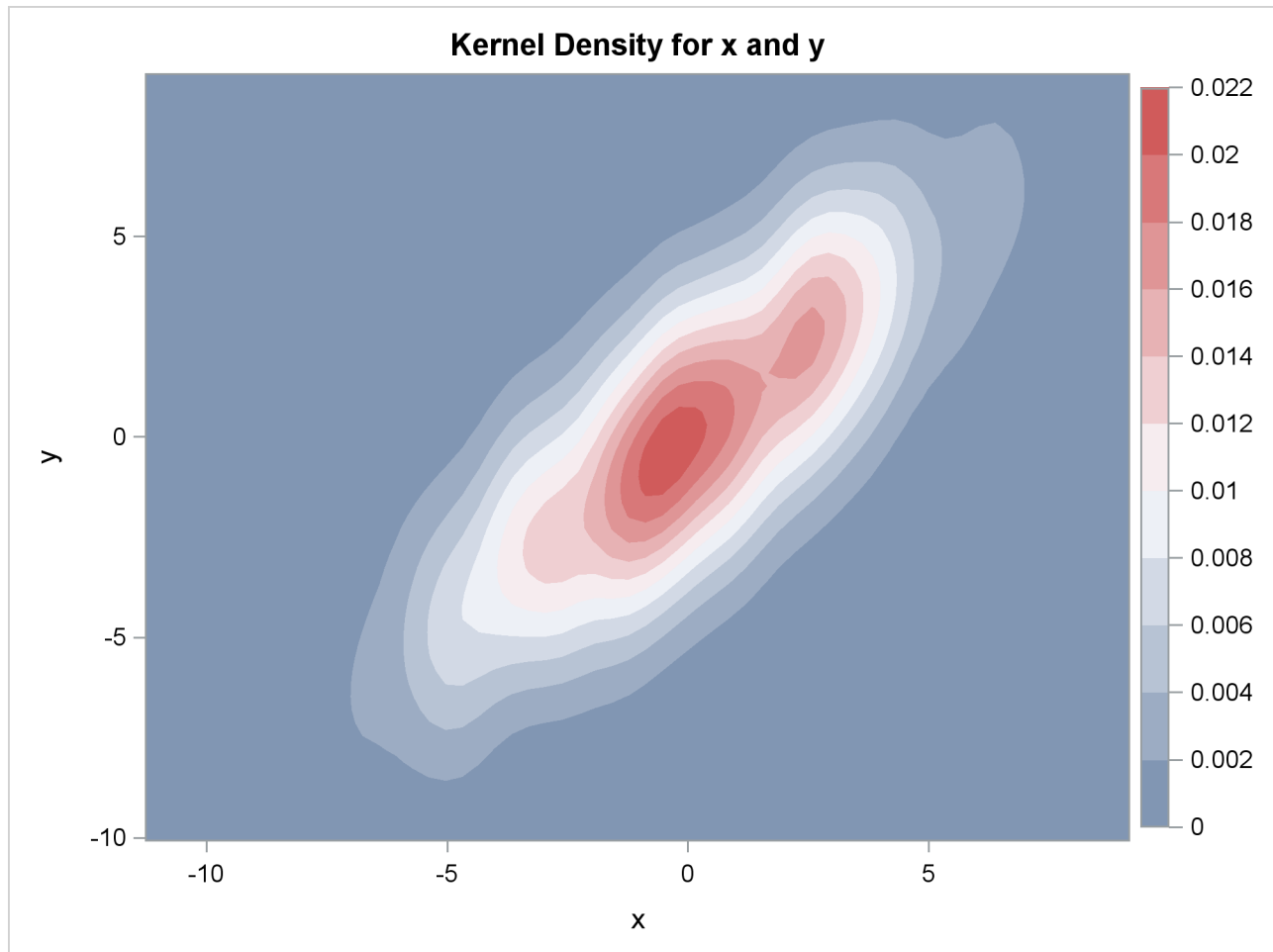
Output 66.3.2 Contour Plot of Estimated Density with Different Smoothing for x and y
