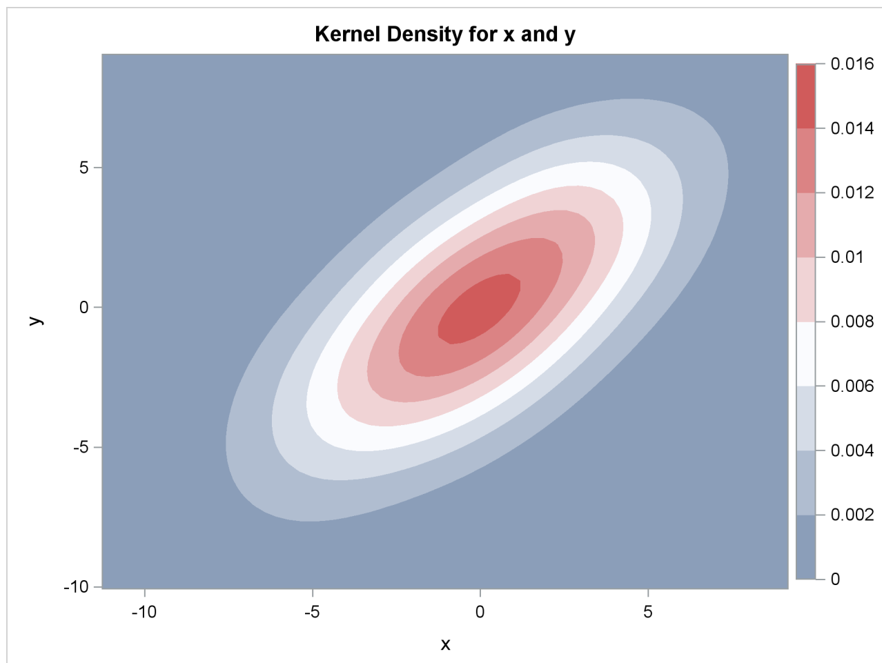
Output 66.3.1 Contour Plot of Estimated Density with Additional Smoothing
