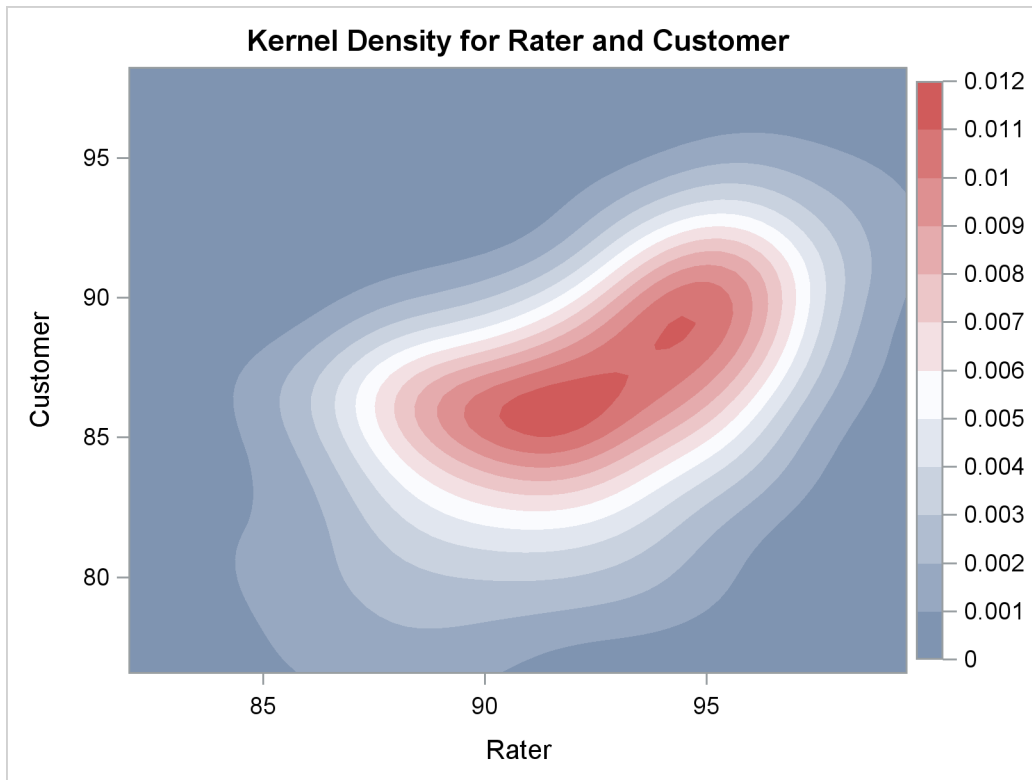
Output 66.6.3 Contour Plot
