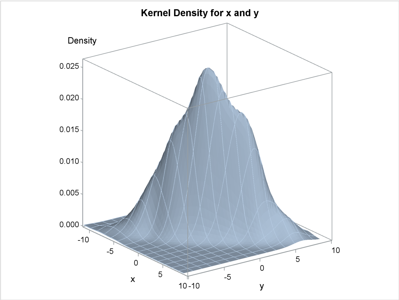
Figure 66.2 Surface Plot of Estimated Density
