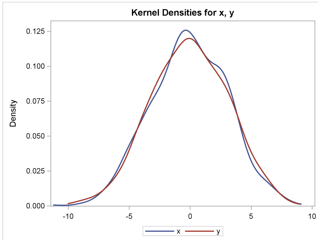
Output 66.5.4 Overlaid Kernel Density Estimates
