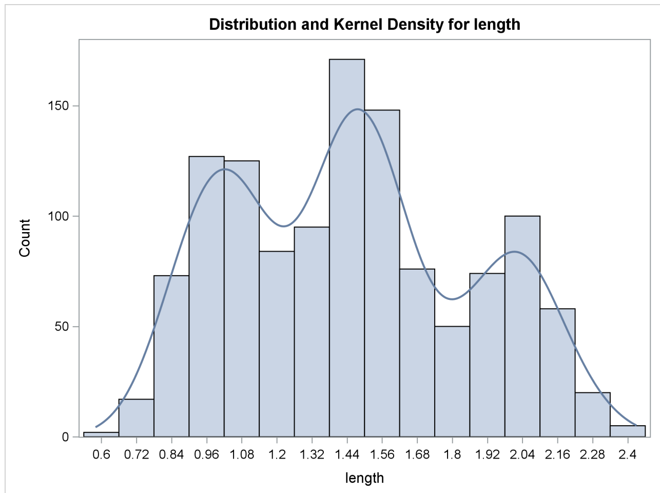
Output 66.2.1 Histogram with Oversmoothed Kernel Density Estimate
