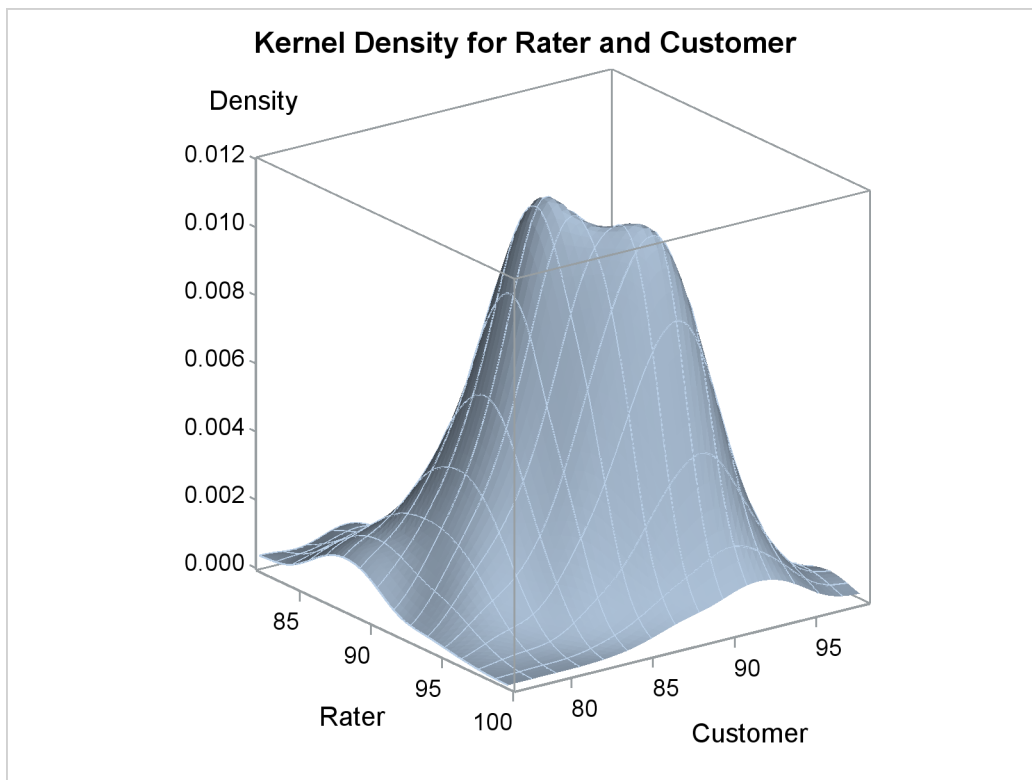
Output 66.6.5 Surface Plot
