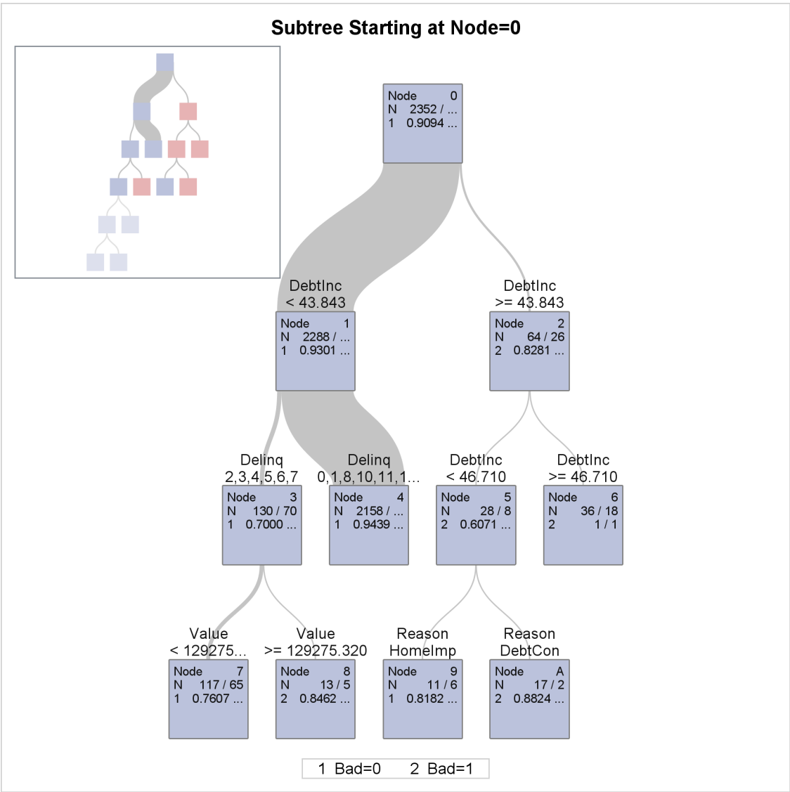
Output 61.4.3 Detailed Tree Diagram
