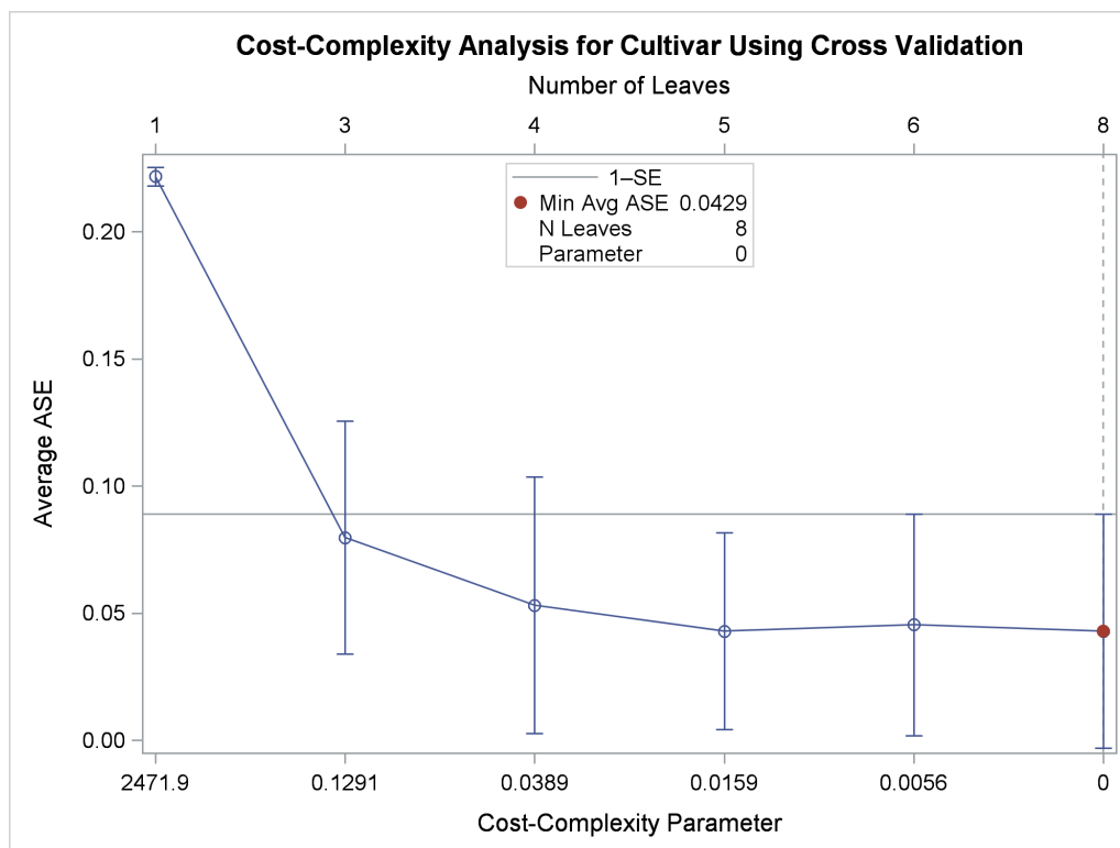
Output 61.6.2 Cost-Complexity Pruning Plot of Average ASE
