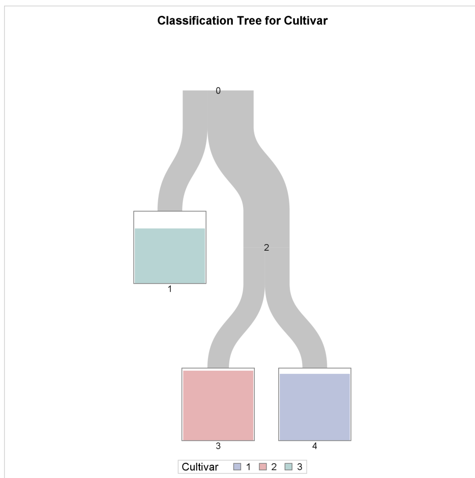
Figure 61.7 Overview Diagram of Final Tree
