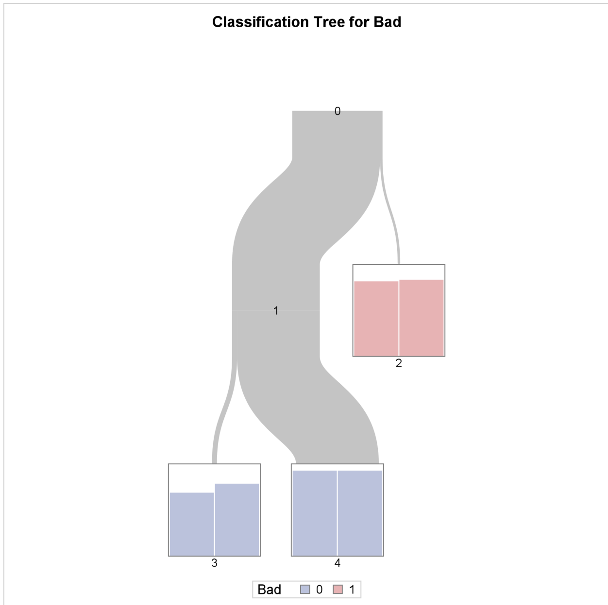
Figure 61.11 First Two Splits for Hmeq Data Set
