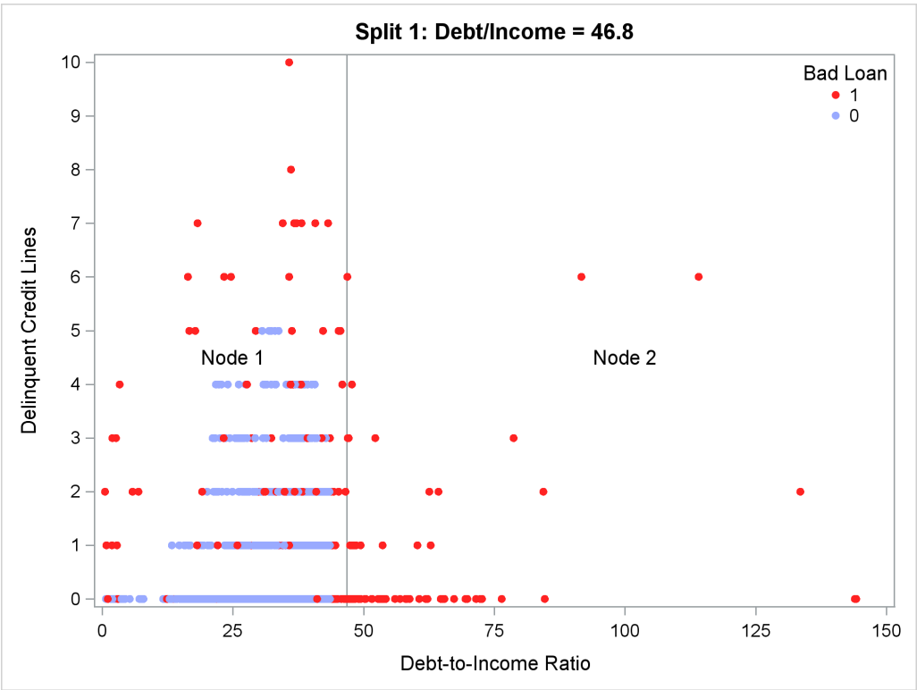
Figure 61.12 Scatter Plot of the Predictor Space for the First Split
