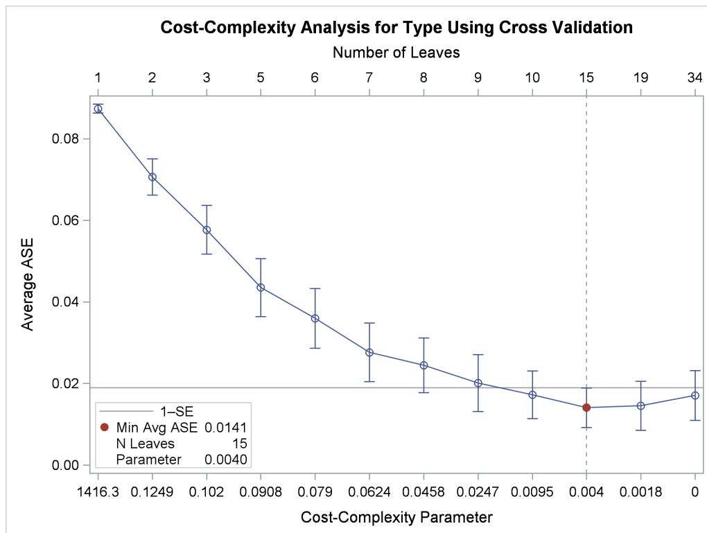
Output 61.2.1 Plot of Cross Validated ASE by Cost-Complexity Pruning Parameter
