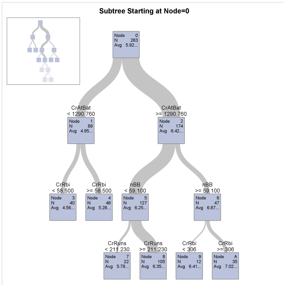
Output 61.3.2 Detailed Diagram of Regression Tree
