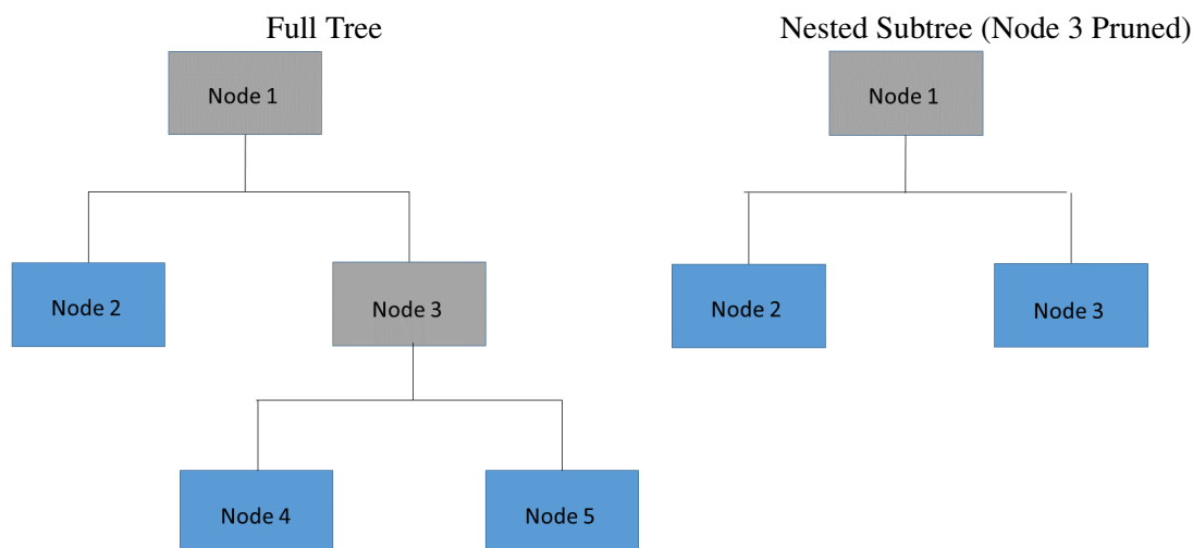
Figure 61.14 Tree and Pruned Subtree
