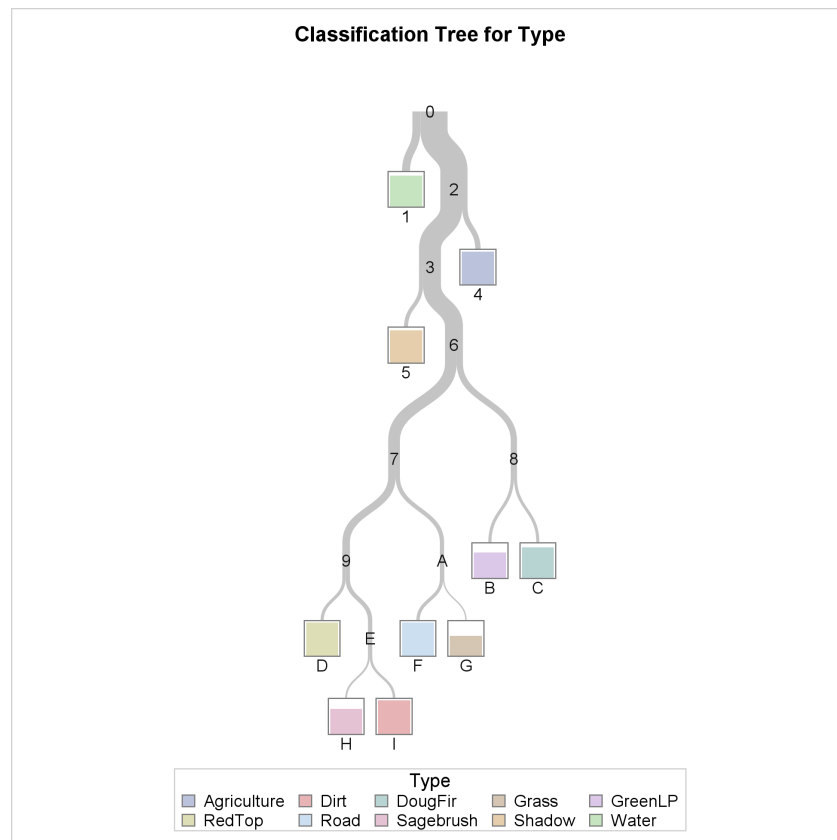
Output 61.2.2 Diagram of 10-Leaf Tree Selected Using 1-SE Rule
