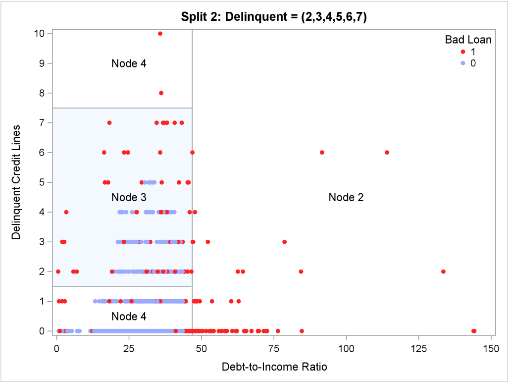
Figure 61.13 Scatter Plot of the Predictor Space for the Second Split
