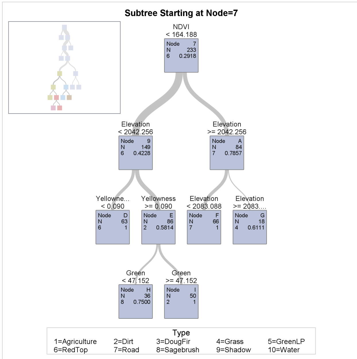
Output 61.2.3 Detailed Diagram of 10-Leaf Tree
