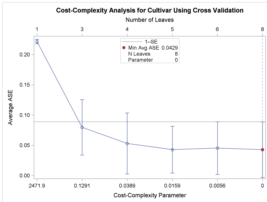
Figure 61.6 Cost-Complexity Plot
