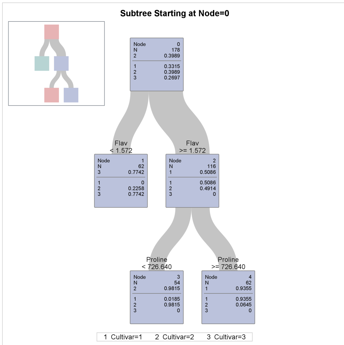
Figure 61.8 Detailed Tree Diagram
