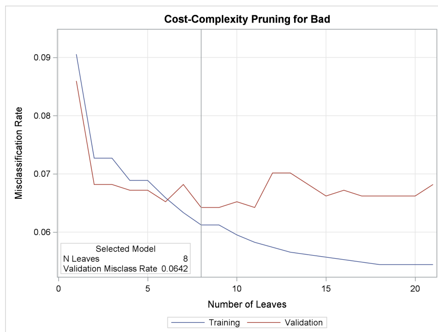
Output 61.4.7 Pruning Plot
