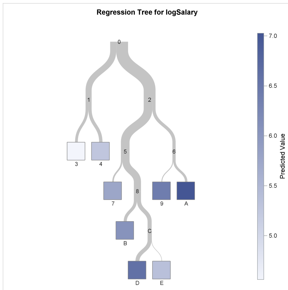
Output 61.3.1 Overview Diagram of Regression Tree
