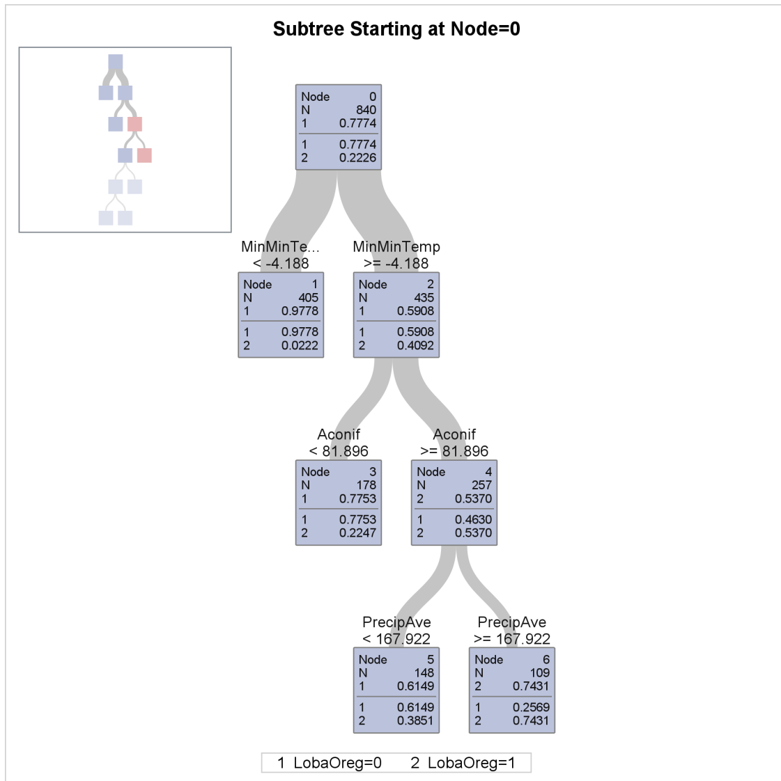
Output 61.1.4 First Four Levels of Fitted Tree
