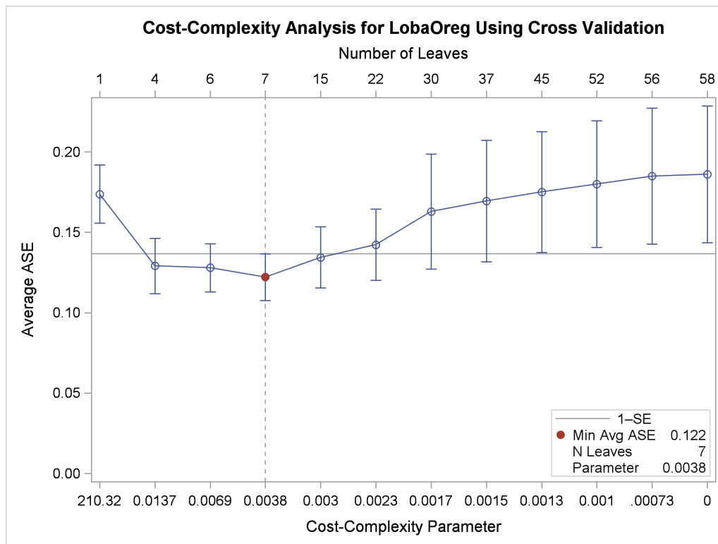
Output 61.1.2 ASE as a Function of Cost-Complexity Parameter
