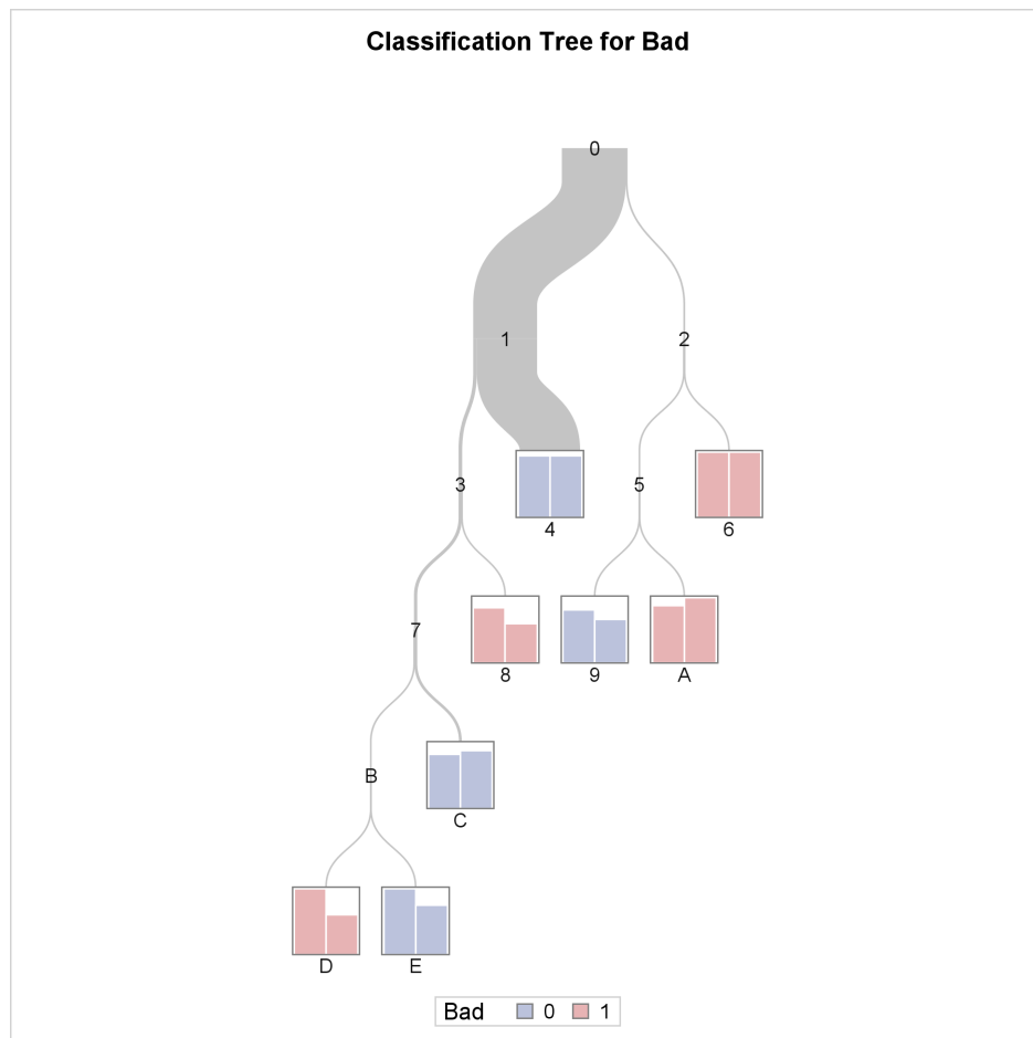
Output 61.4.2 Overview Diagram of Final Tree
