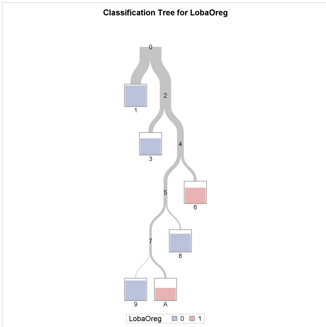
Output 61.1.3 Overview of Fitted Tree
