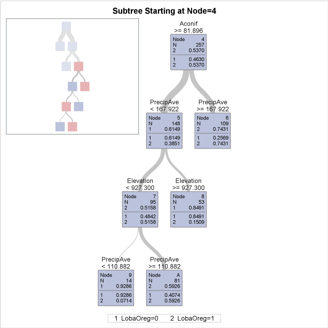
Output 61.1.5 Bottom Four Levels of Fitted Tree
