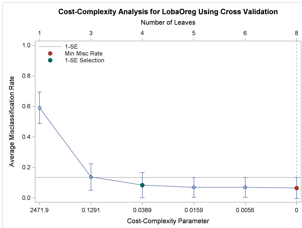
Output 61.6.3 Cost-Complexity Analysis Based on Misclassification Rate
