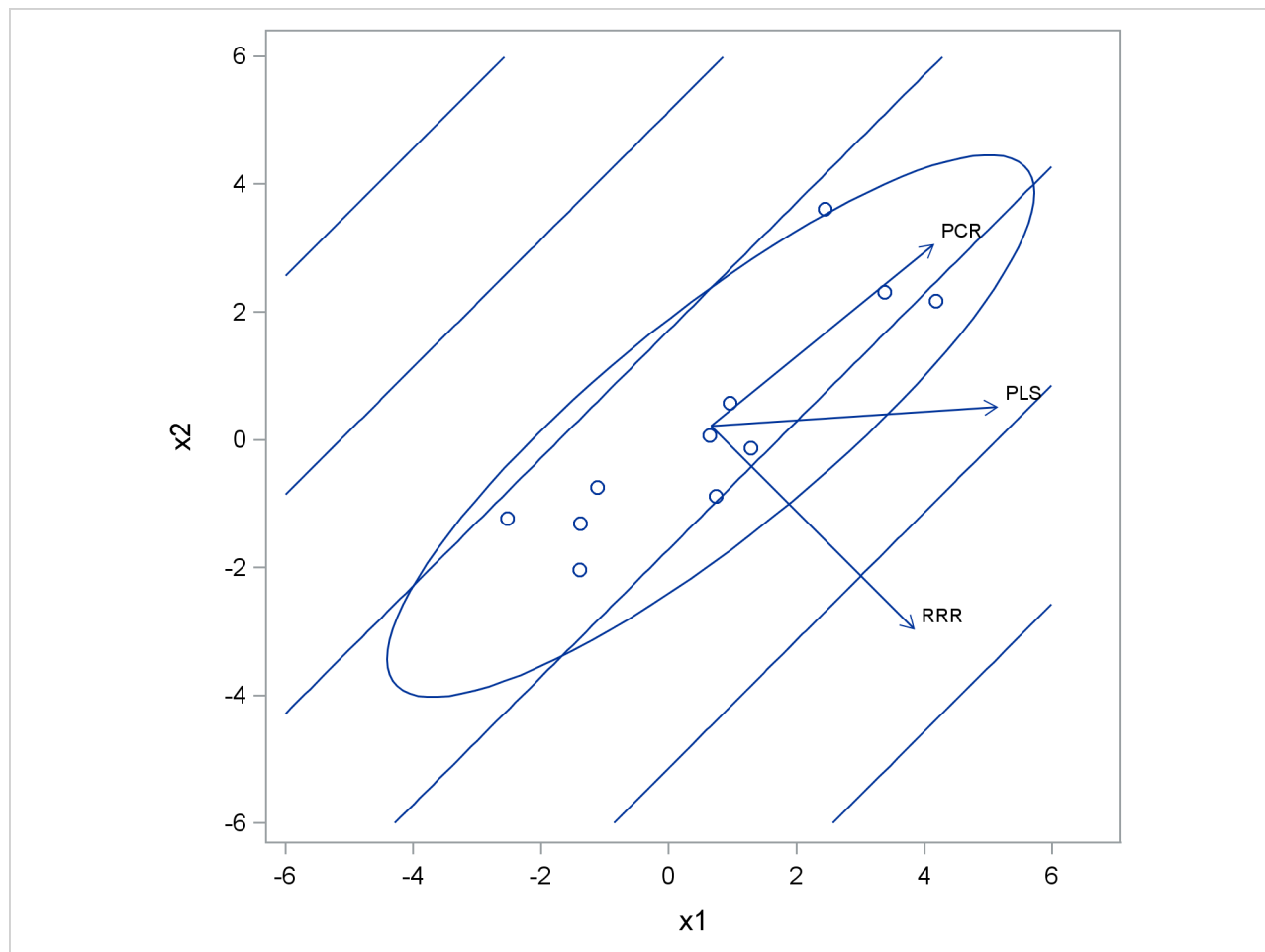
Figure 57.14 Depiction of the First Factors for Three Different Regression Methods
