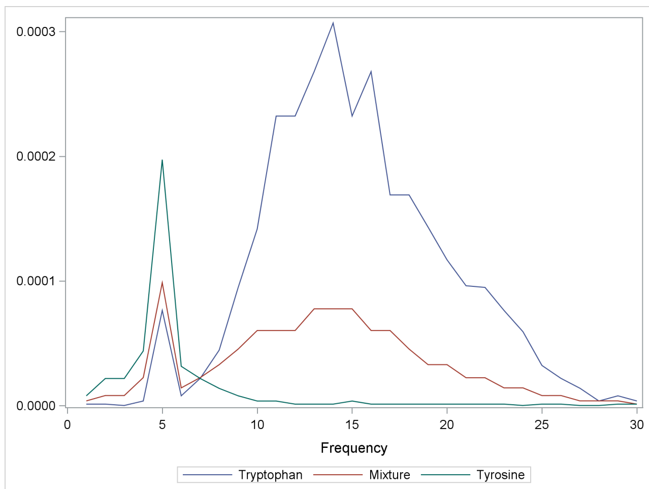
Output 57.1.1 Spectra for Three Samples of Tyrosine and Tryptophan
