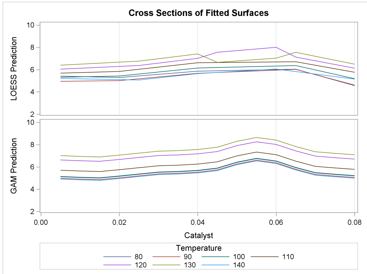
Output 41.3.3 Cross Sections of Fitted Regression Surfaces
