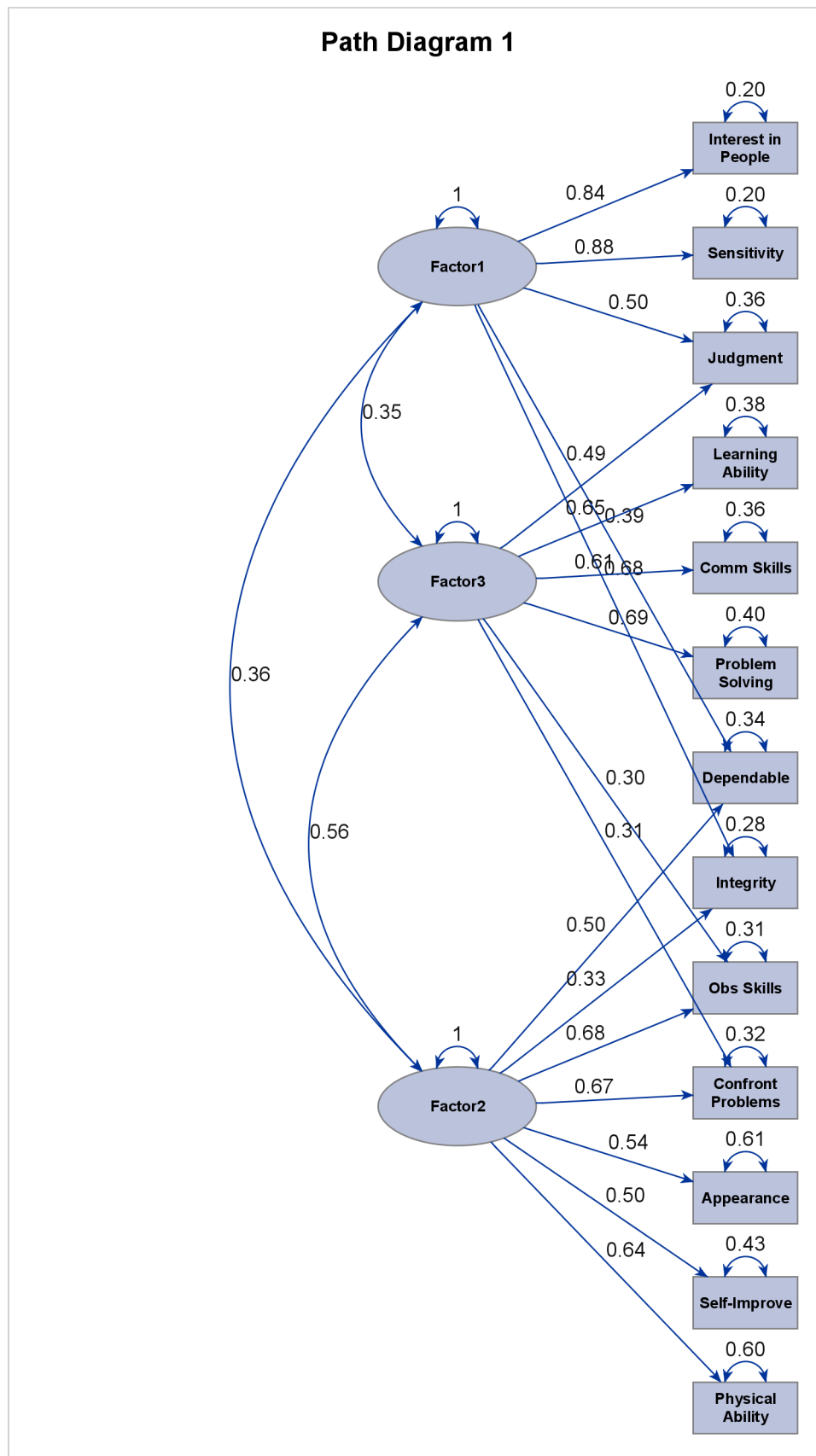
Output 37.5.3 Default Path Diagram for the Quartimin-Rotated Solution
