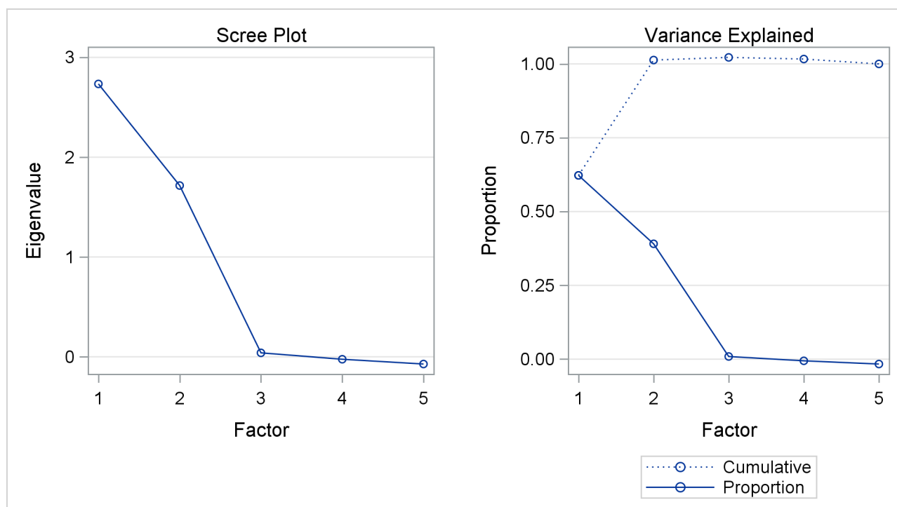
Output 37.2.3 Scree and Variance Explained Plots
