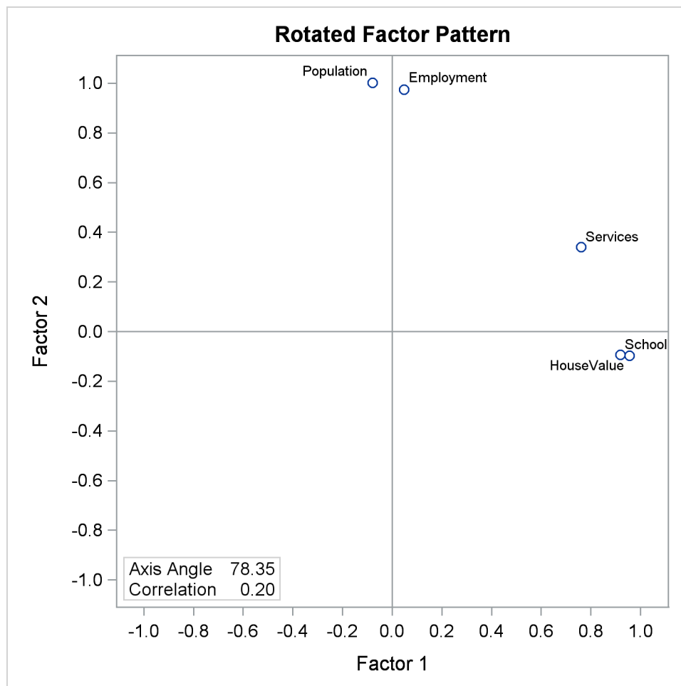
Output 37.2.12 Promax Rotation: Factor Loading Plot
