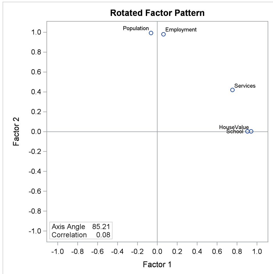
Output 37.2.20 Harris-Kaiser Rotation: Factor Loading Plot
