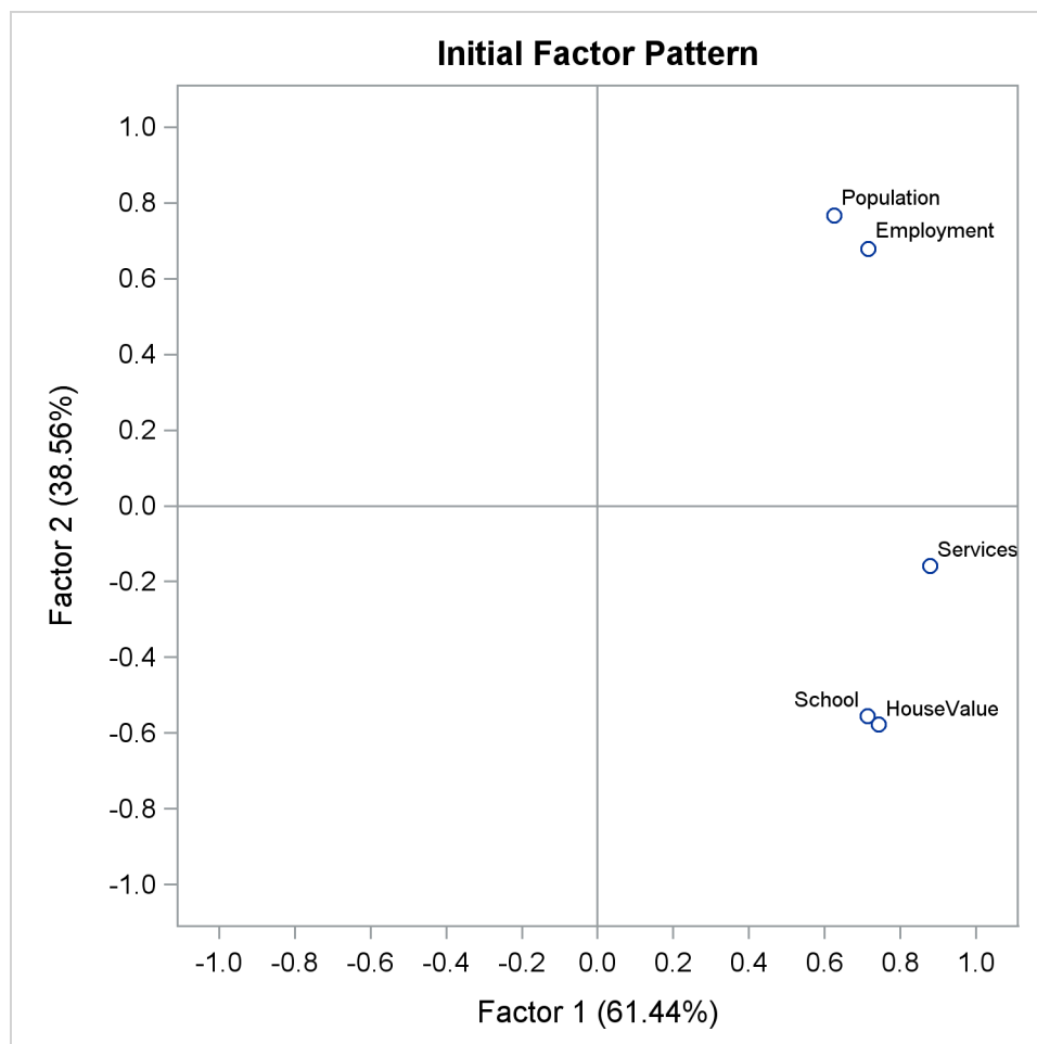
Output 37.2.6 Unrotated Factor Loading Plot
