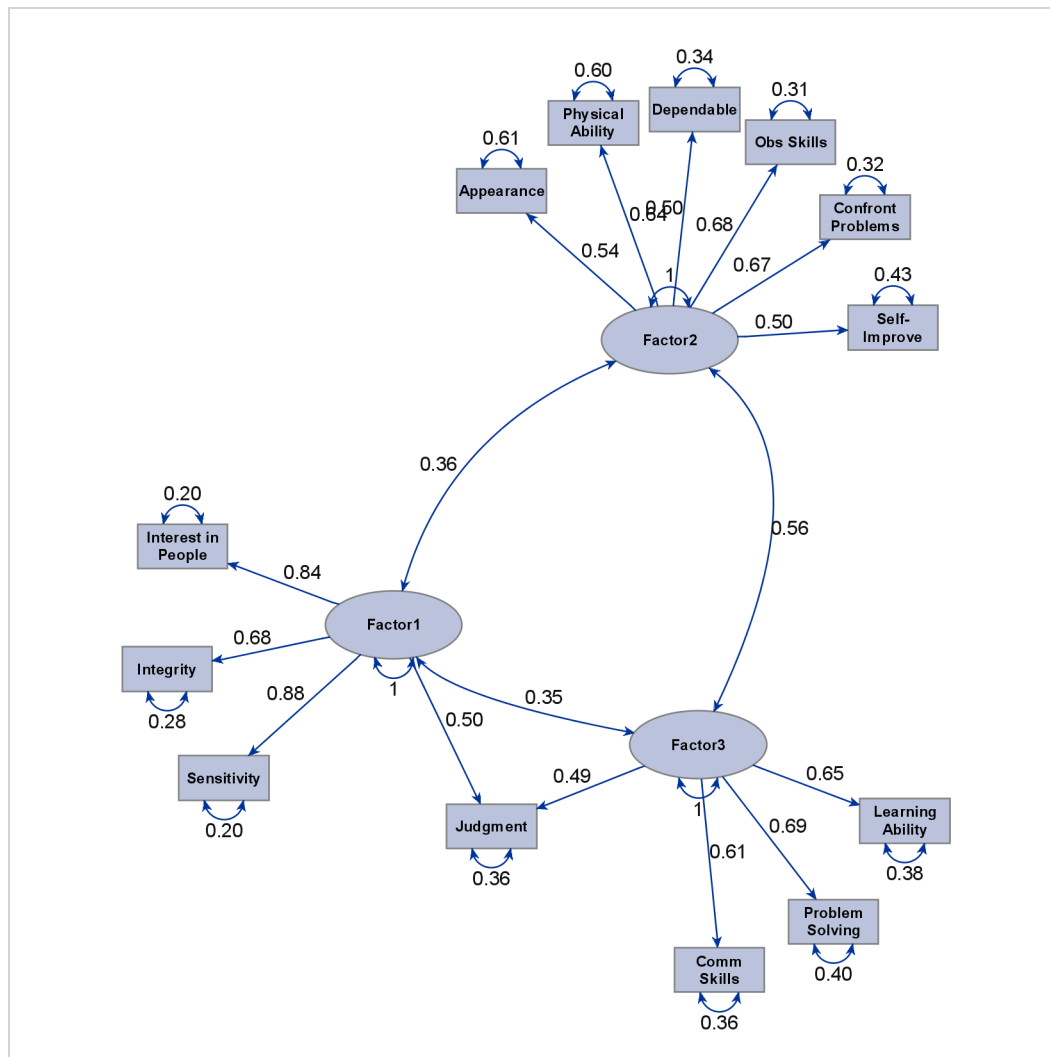
Output 37.5.5 Path Diagram Showing Strong Links by Using the ARRANGE=GRIP Algorithm
