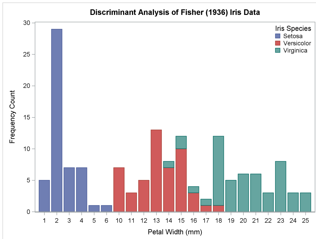
Output 35.1.1 Sample Distribution of Petal Width in Three Species
